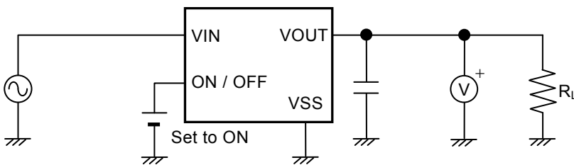
Figure 7 Test Circuit 5
