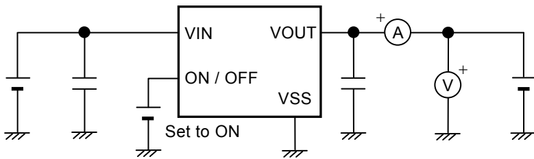
Figure 5 Test Circuit 3
