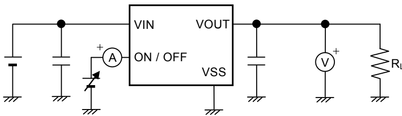
Figure 6 Test Circuit 4
