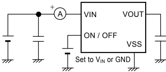
Figure 4 Test Circuit 2
