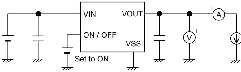
Figure 3 Test Circuit 1
