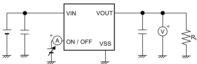
Figure 8 Test Circuit 4
