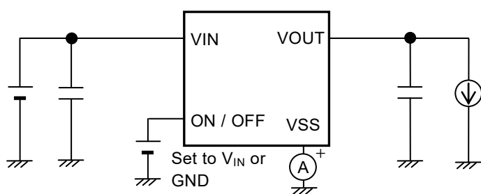
Figure 6 Test Circuit 2
