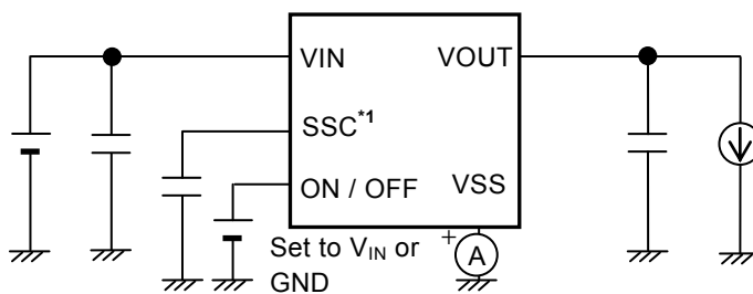
Figure 10 Test Circuit 2
