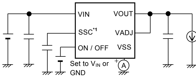
Figure 17 Test Circuit 9
