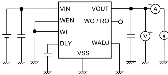
Figure 7 Test Circuit 1
