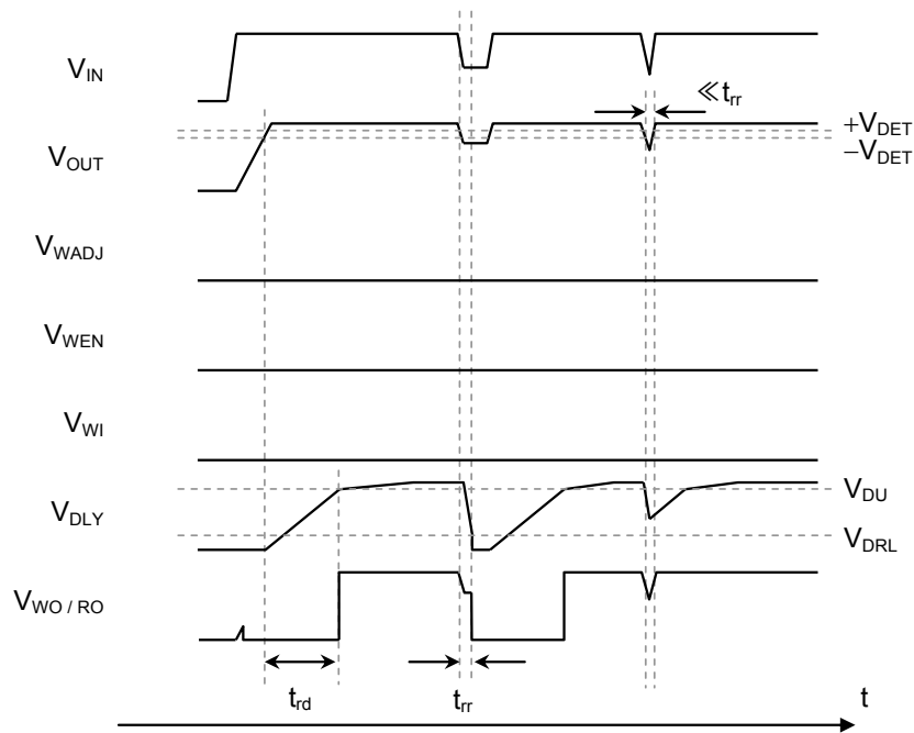
Figure 48 Example of Detector Operation
