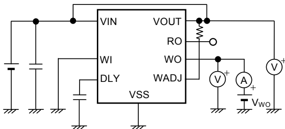
Figure 31 Test Circuit 14
