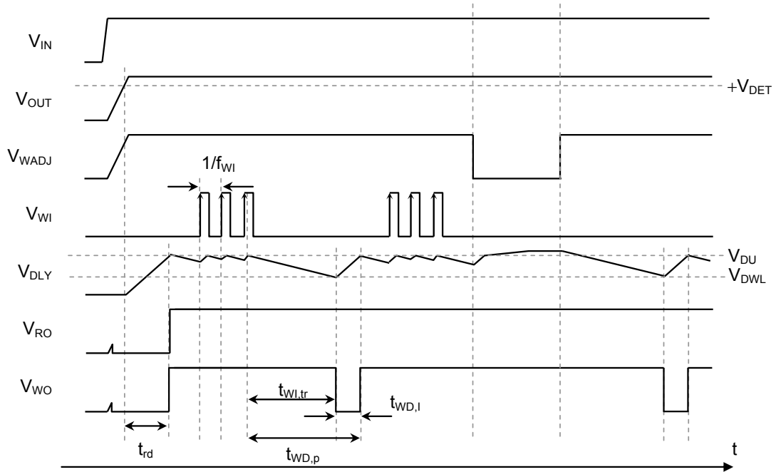
Figure 49 Example of Watchdog Timer Monitoring Operation
