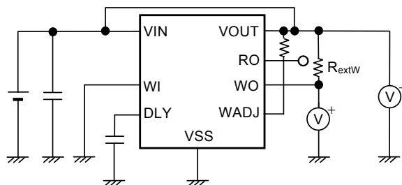
Figure 30 Test Circuit 13
