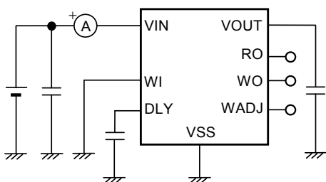
Figure 29 Test Circuit 12
