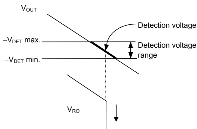
Figure 34 Detection Voltage
