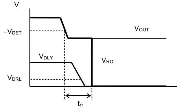
Figure 37 Reset Reaction Time
