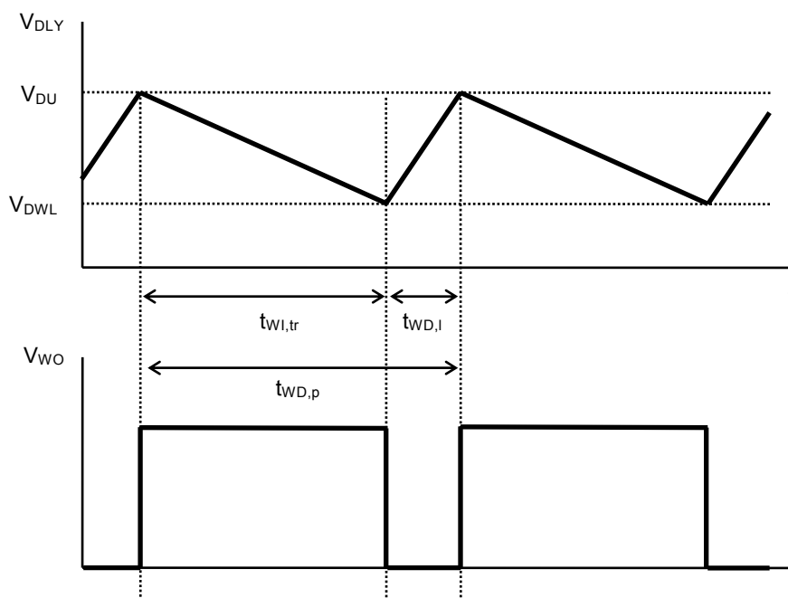
Figure 38 Watchdog Trigger Time
