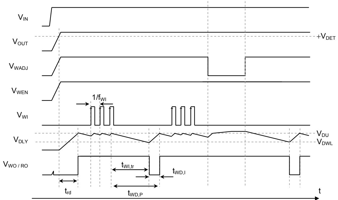
Figure 47 Example of Watchdog Timer Monitoring Operation
