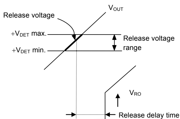
Figure 35 Release Voltage
