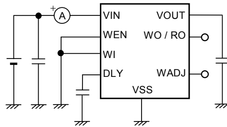
Figure 18 Test Circuit 12
