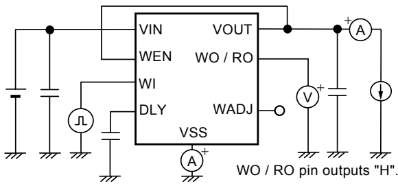
Figure 17 Test Circuit 11
