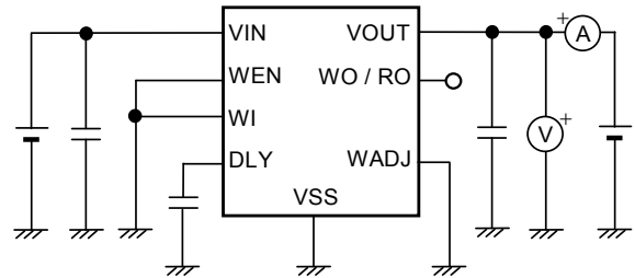
Figure 8 Test Circuit 2
