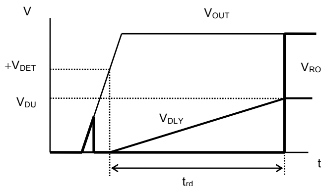
Figure 36 Release Delay Time
