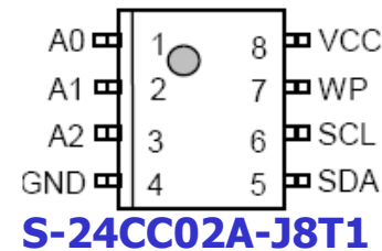
8-Pin SOP (JEDEC) Top view
