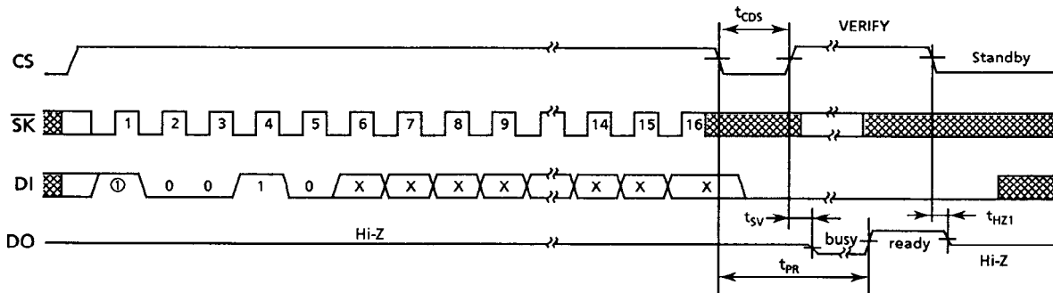
Figure 8 ERAL Timing
