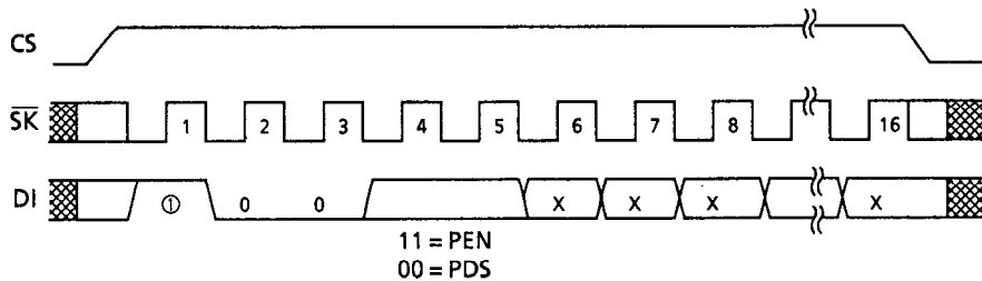
Figure 9 PEN/PDS Timing
