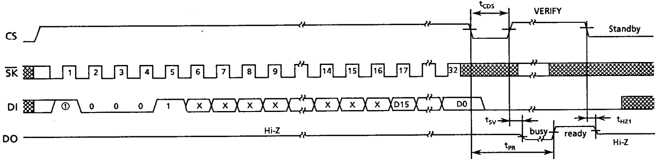
Figure 7 WRAL Timing
