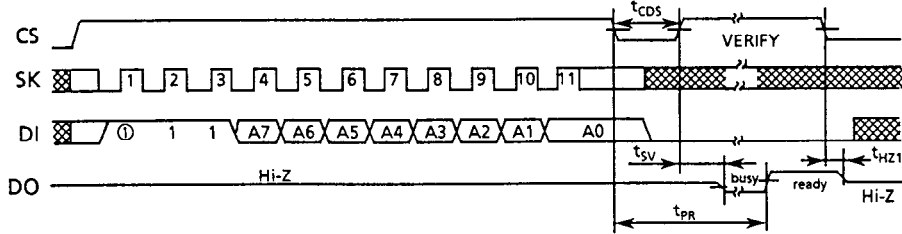
Figure 12 ERASE Timing (S-29L331A)
