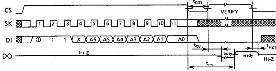
Figure 11 ERASE Timing (S-29L221A)
