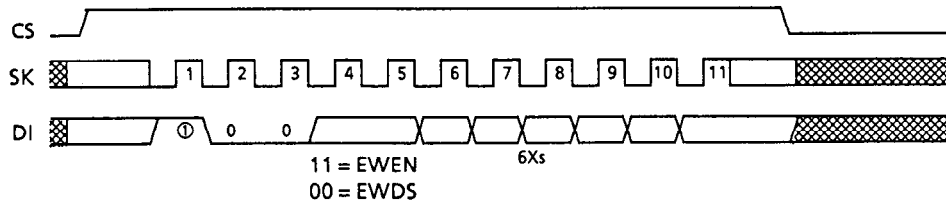
Figure 14 EWEN/EWDS Timing (S-29L221A)
