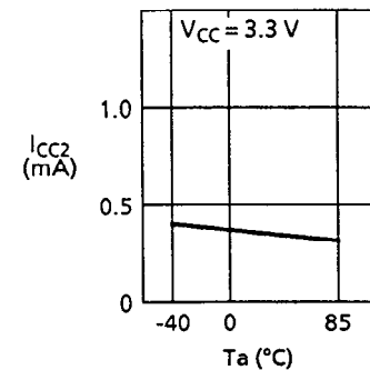
1.8 Current consumption (PROGRAM) I_{CC2} — Ambient temperature T_a
