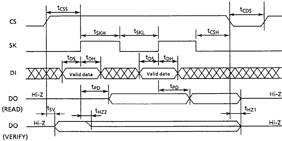
Figure 3 Timing Chart
