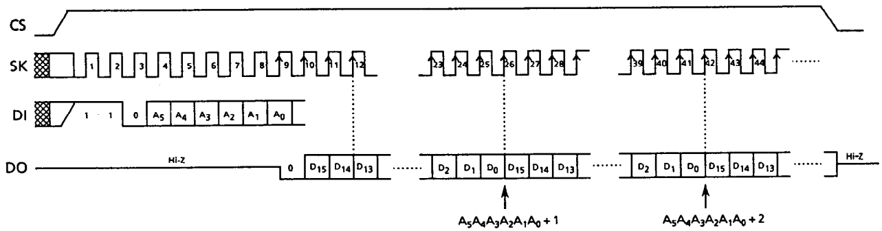
Figure 4 Read Timing (S-29L130A)
