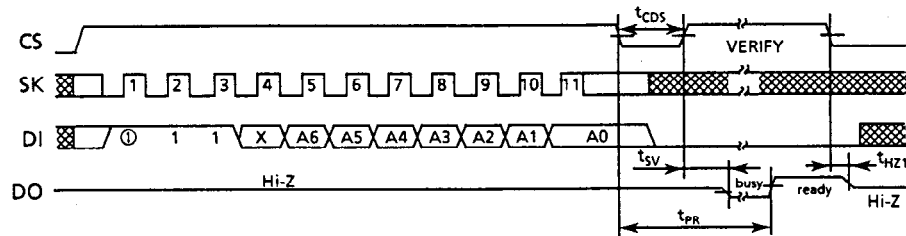
Figure 11 ERASE Timing (S-29L220A)
