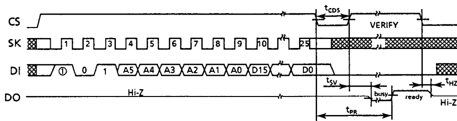
Figure 7 WRITE Timing (S-29L130A)
