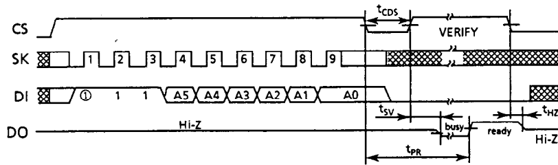
Figure 10 ERASE Timing (S-29L130A)
