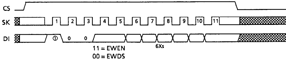
Figure 15 EWEN/EWDS Timing (S-29L330A)
