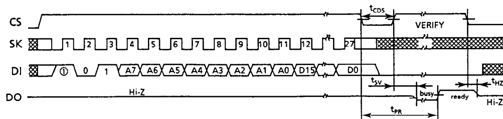
Figure 9 WRITE Timing (S-29L330A)
