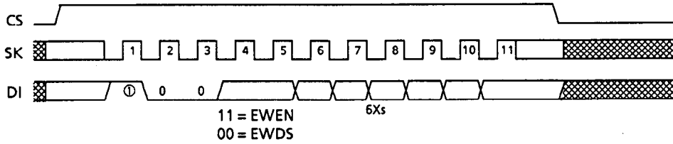
Figure 14 EWEN/EWDS Timing (S-29L220A)
