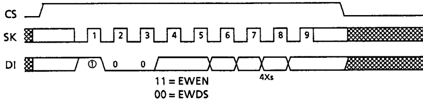
Figure 13 EWEN/EWDS Timing (S-29L130A)
