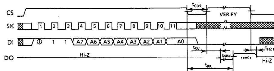
Figure 12 ERASE Timing (S-29L330A)
