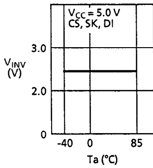
1.27 Input voltage V_{IN} ( V_{IL} , V_{IH} ) – Ambient temperature T_a
