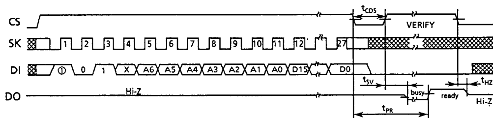
Figure 8 WRITE Timing (S-29L220A)
