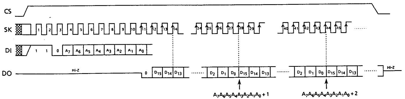
Figure 6 Read Timing (S-29L330A)
