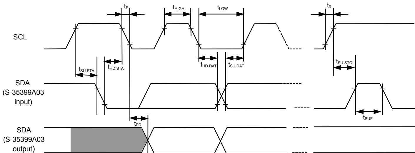
Figure 7 Bus Timing ABLIC Inc.
