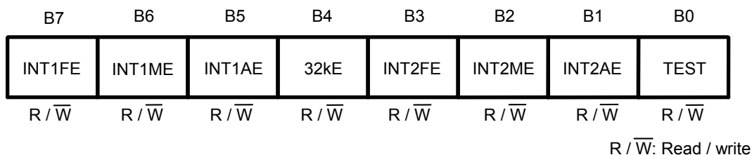
Figure 11 Status Register 2
