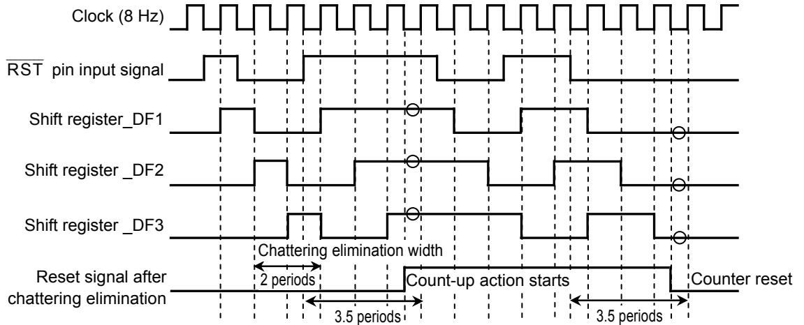
Figure 34 Timing Chart of Chattering Elimination
