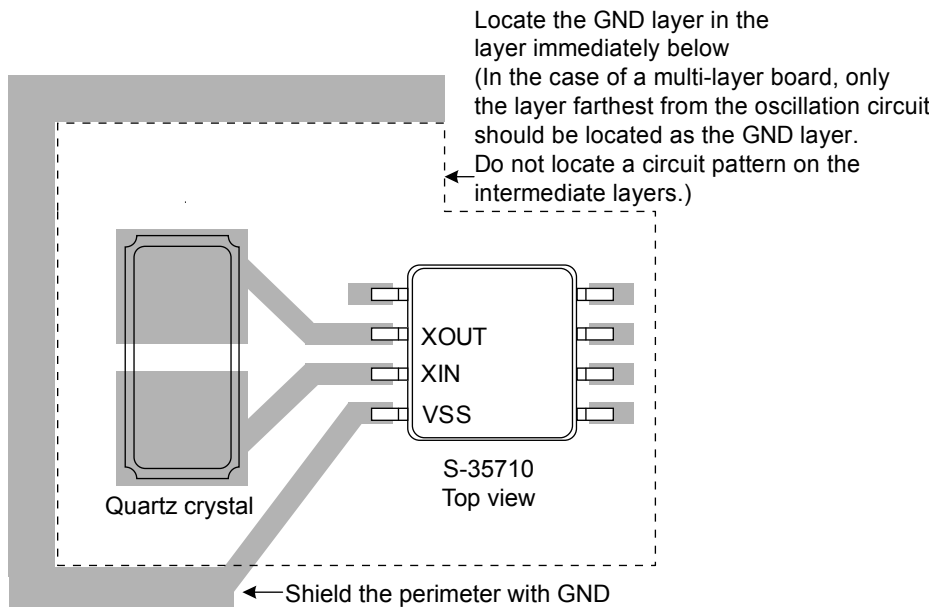
Figure 38 Example of Recommended Connection Pattern Diagram
