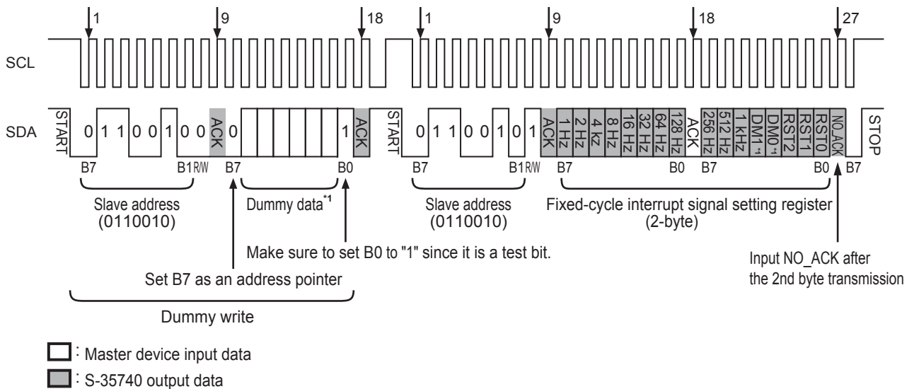
Figure 25 Read Timing of Fixed-cycle Interrupt Signal Setting Register
