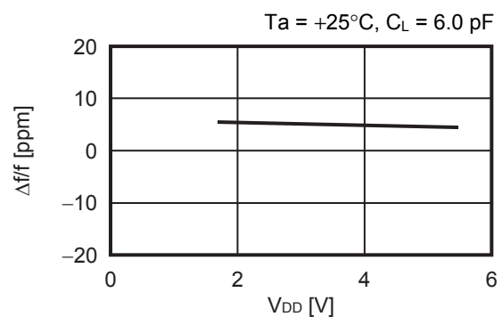
8. Oscillation frequency vs. Power supply voltage characteristics
