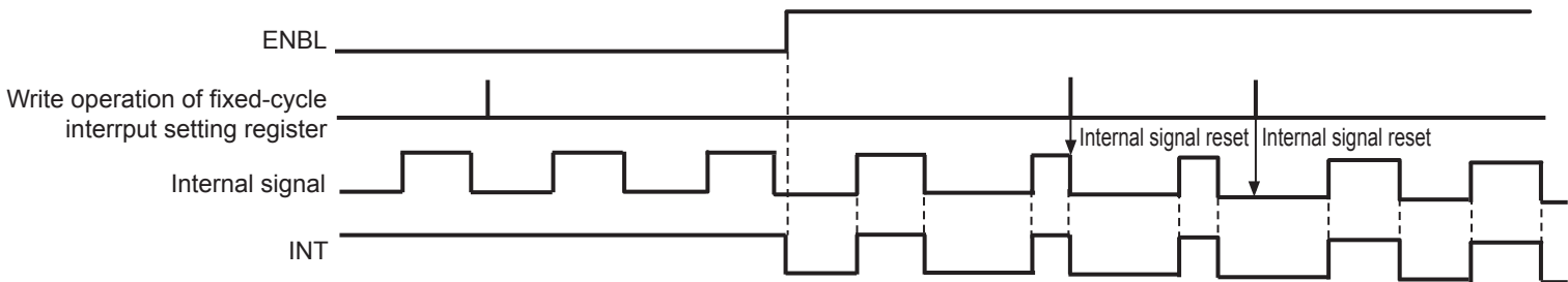
Figure 16 INT Pin Output Timing Example 2 (CMOS Output)
