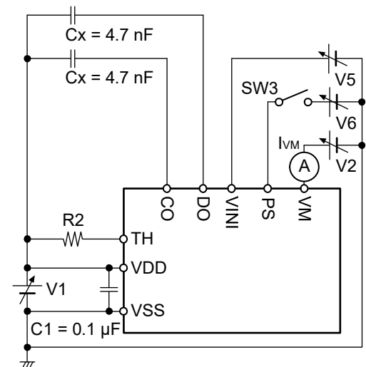
Figure 8 Test Circuit 4
