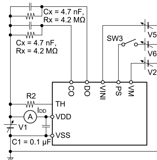
Figure 7 Test Circuit 3
