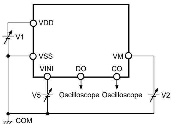
Figure 7 Test Circuit 5
