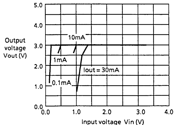
(b) Input voltage – Output voltage characteristics
