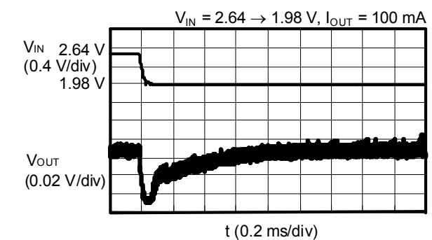
S-8340C33AFT, f_{OSC} = 300 kHz
