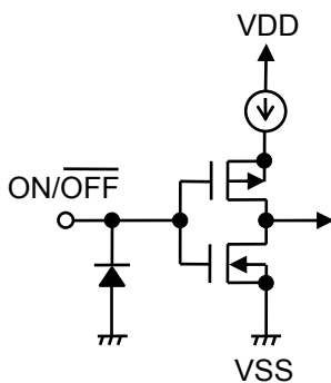
Figure 11 ON/OFF Pin Structure
