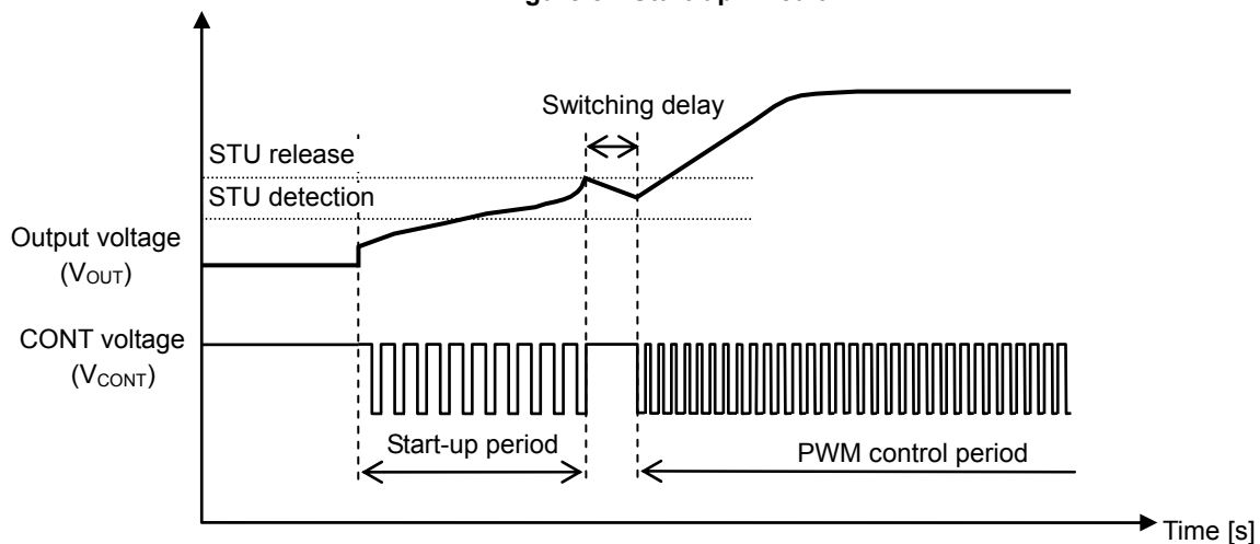
Figure 9 Start-up Sequence
