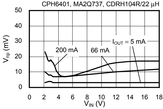
(33) S-8460B00AFT ( V_{OUT} = 3.3\text{ V} )
