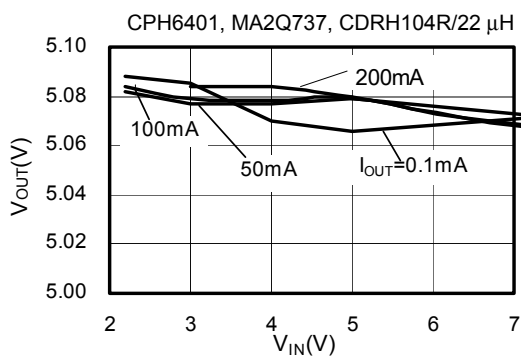
(30) S-8460B00AFT ( V_{OUT} = 5.0\text{ V} )
