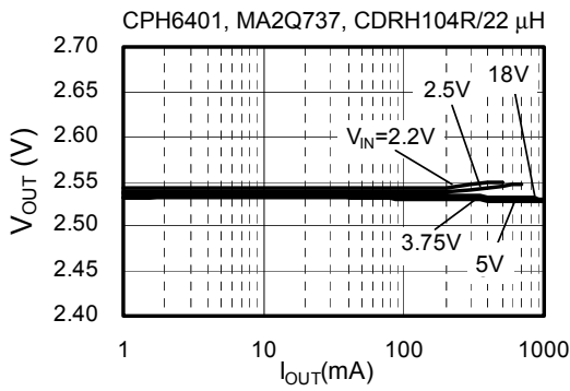
(26) S-8460B00AFT ( V_{OUT} = 2.5\text{ V} )
