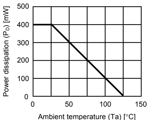
Figure 3 Power Dissipation of Packages (Before Mounting)
