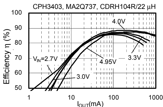
(5) S-8460B00AFT ( V_{OUT} = 3.3\text{ V} )
