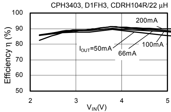
(22) S-8460B00AFT ( V_{OUT} = 3.3\text{ V} )
