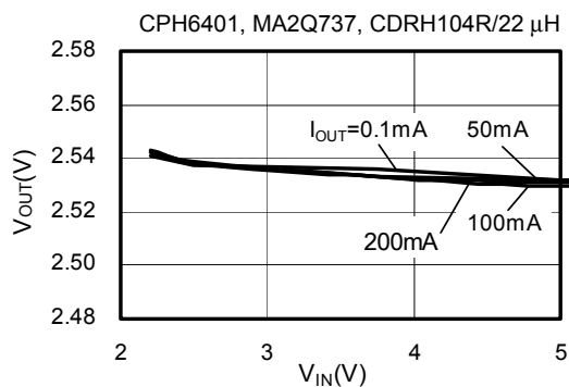
(29) S-8460B00AFT ( V_{OUT} = 2.5\text{ V} )
