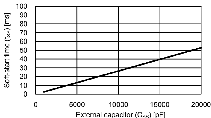
Figure 11 Soft-Start Time
