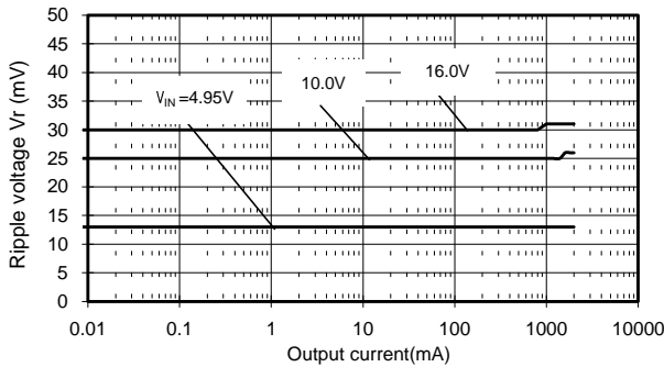
(33)S-8532B15AFT
