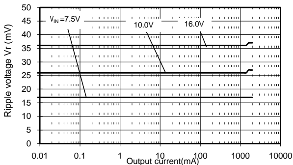
(33)S-8532B15AFT
