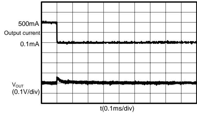
(6) S-8532B50AFT ( V_{IN} : 7.5V)
