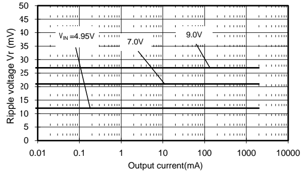
(32)S-8532B15AFT
