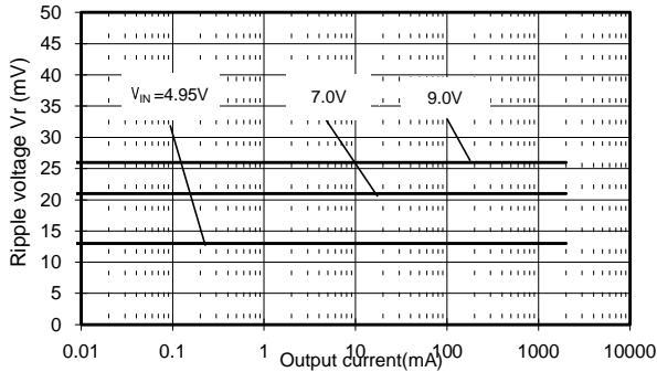
(31)S-8532B15AFT
