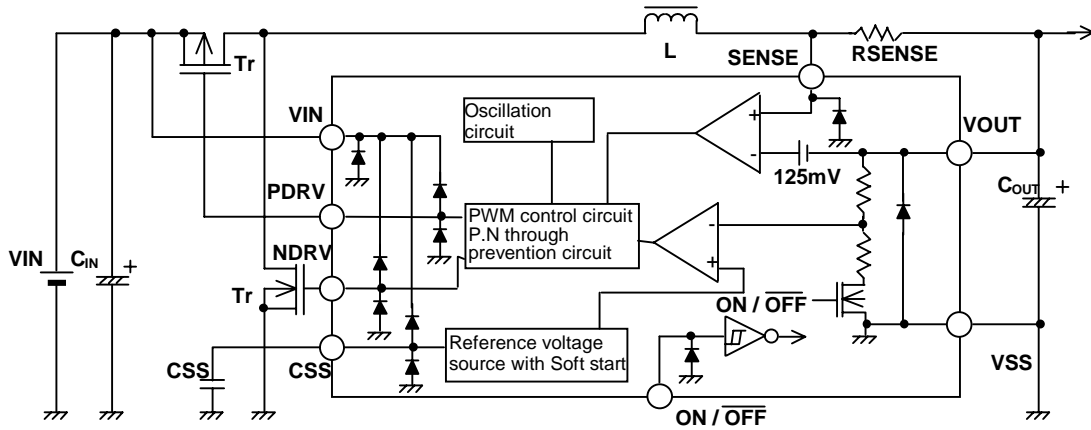
Figure 1 Block diagram
