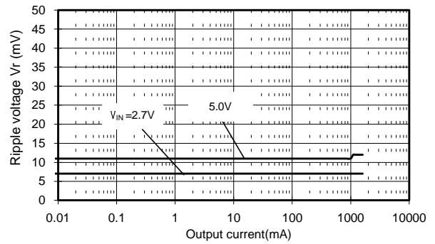
(30)S-8532B15AFT
