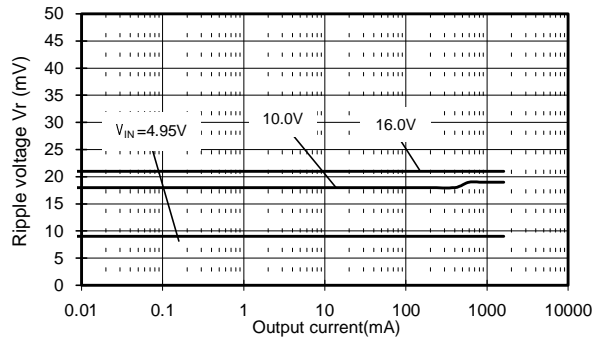
(34)S-8532B15AFT
