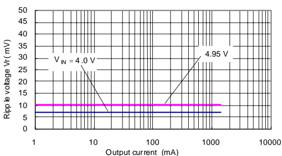
(32) S-8533A33AFT (Si3454DV/Si3455DV)
