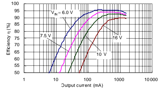
(24) S-8533A50AFT (Si3454DV/Si3455DV)
