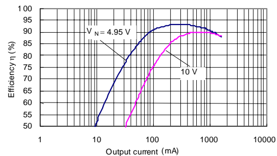
(24) S-8533A50AFT (Si3454DV/Si3455DV)
