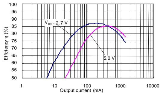
(12) S-8533A33AFT (Si3441DV/Si3442DV)
