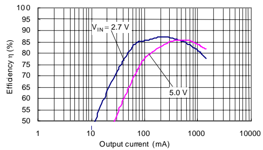
(20) S-8533A33AFT (Si3441DV/Si3442DV)
