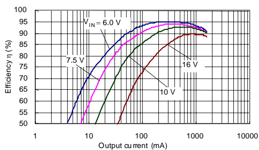
(16) S-8533A50AFT (Si3454DV/Si3455DV)
