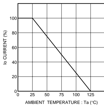
Fig. 4 Derating curve
