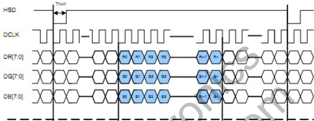
Parallel RGB input timign table
