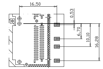
QUAD LIGHT PIPE LED LOCATION
