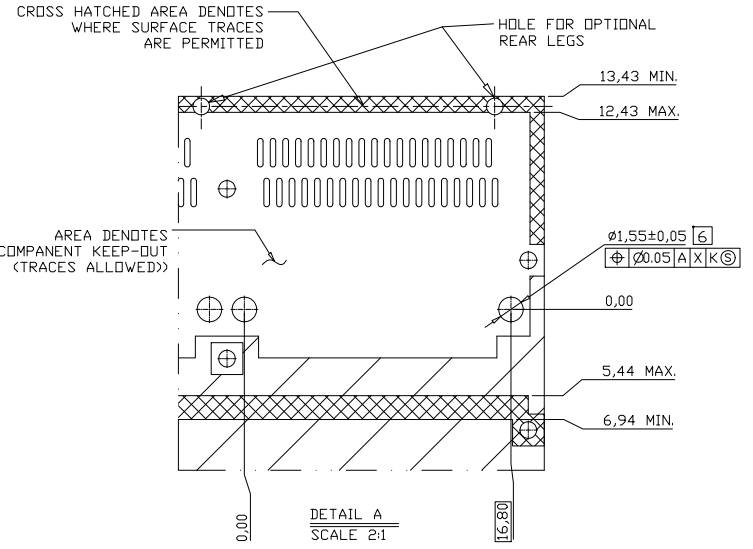
FOR CAGE ASSEMBLIES WITH LIGHT PIPES
