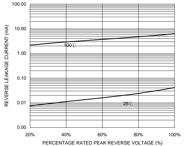
FIG. 4-TYPICAL REVERSE CHARACTERISTICS
