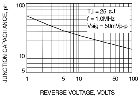
Fig. 4-TYPICAL JUNCTION CAPACITANCE
