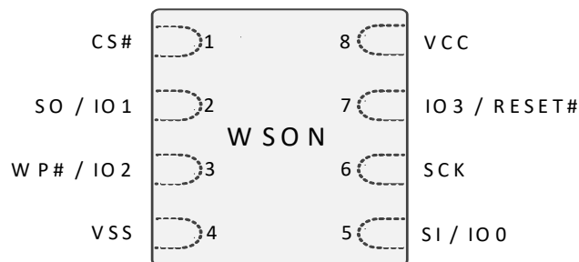
Figure 4. 8-Connector Package (WSO5 5 x 6), Top View [3]
