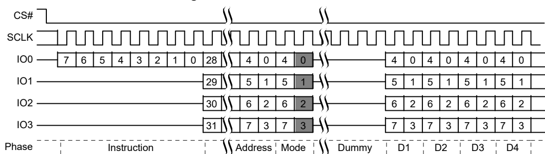
Figure 20. Quad I/O Command [7]
