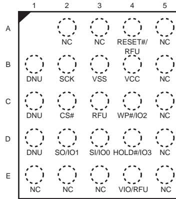
Figure 41. 24-Ball BGA, 5 x 5 Ball Footprint (FAB024), Top View [41]
