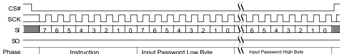
Figure 118. Password Program (PASSP E8h) Command Sequence
