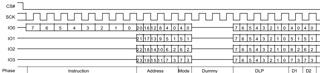
Figure 94. DDR Quad I/O Read Initial Access (3-Byte Address, EDh [ExtAdd=0], HPLC=11b)
