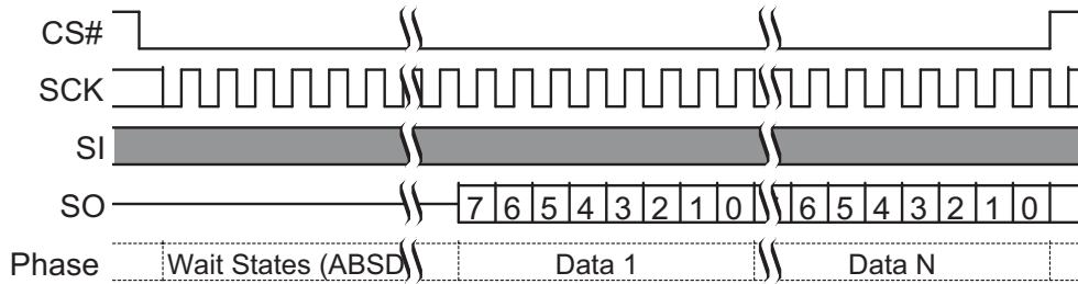
Figure 64. AutoBoot Sequence (CR1[1]=1)
