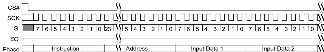
Figure 106. Page Program (OTPP 42h) Command Sequence
