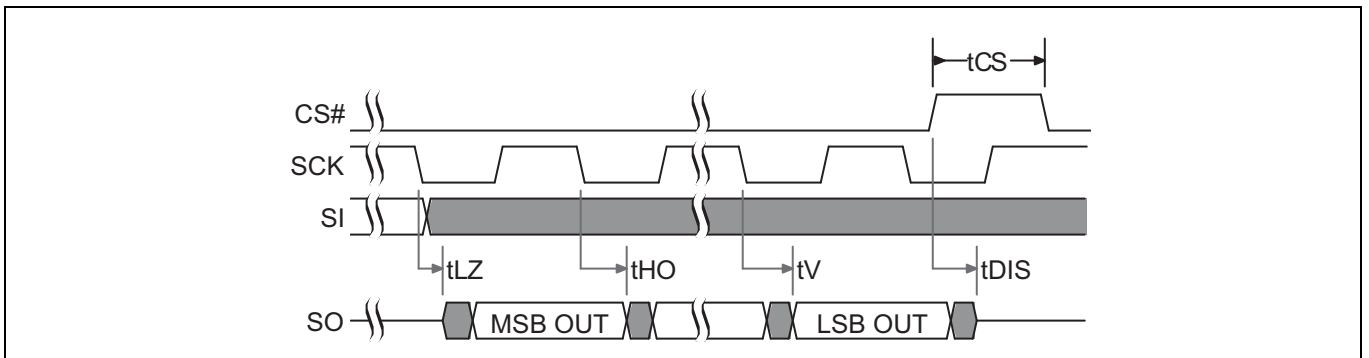
Figure 32 SPI single bit output timing
