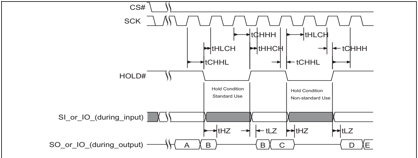
Figure 34 Hold timing
