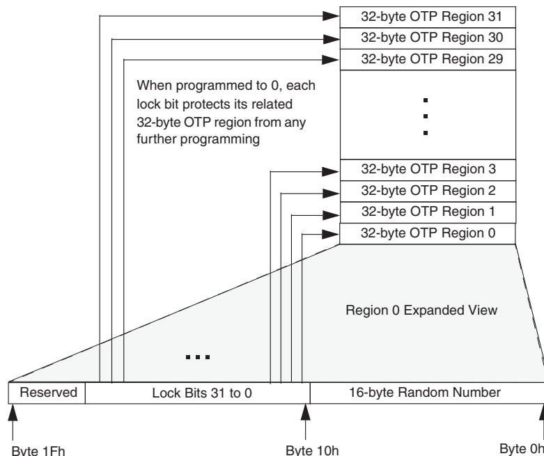
Figure 46. OTP Address Space
