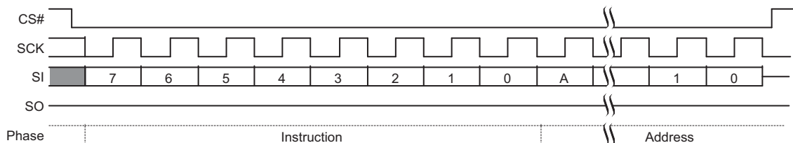
Figure 108. PPBP Command Sequence
