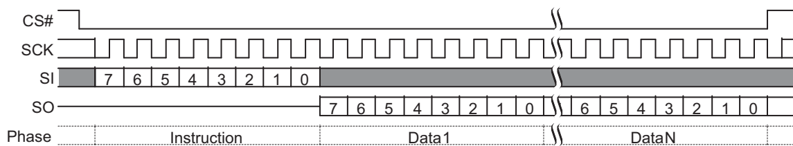
Figure 49. Read Identification (RDID) Command Sequence
