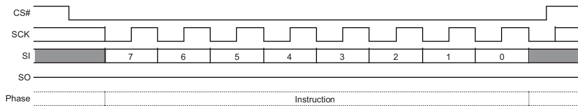
Figure 121. Release from Deep Power-Down Command Sequence
