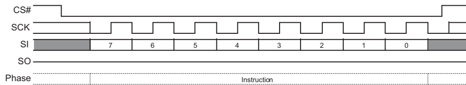
Figure 7. Single Bit Wide Input Command
