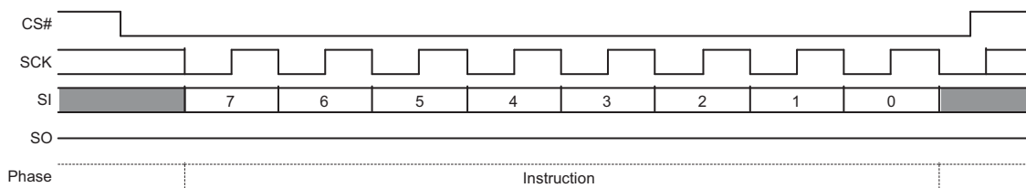
Figure 10.68 PPB Lock Bit Write Command Sequence
