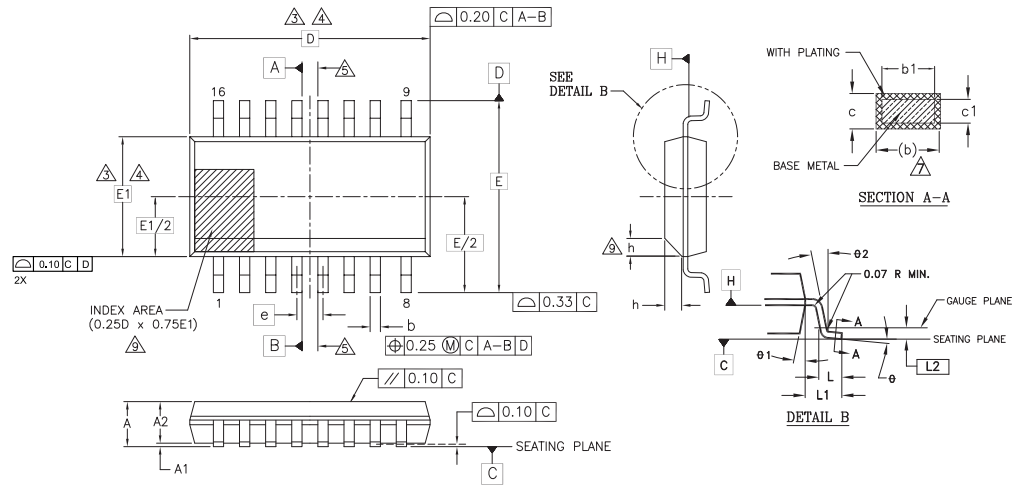
Figure 7.2 SOIC 16-Lead, 300-mil Body Width (SO3016)
