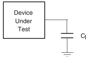
Figure 6.2 Test Setup
