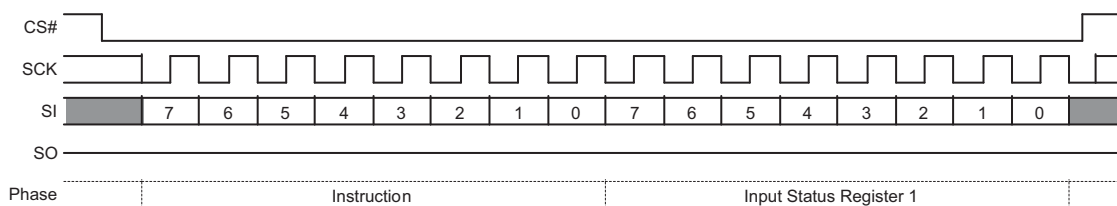
Figure 10.10 Write Registers (WRR) Command Sequence – 8-Data Bits
