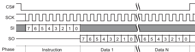
Figure 9.65 Password Read Command Sequence
