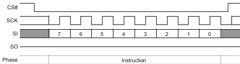
Figure 9.64 PPB Lock Bit Write Command Sequence
