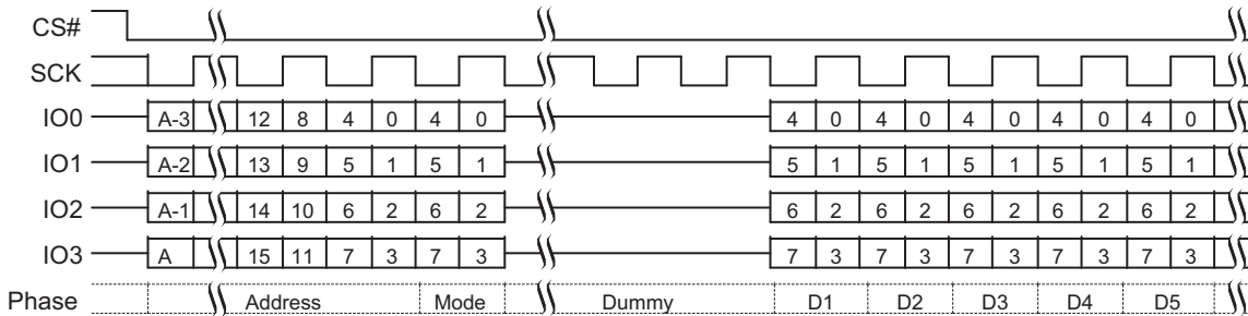
Figure 9.37 Continuous DDR Quad I/O Read Subsequent Access (EDh or EEh)
