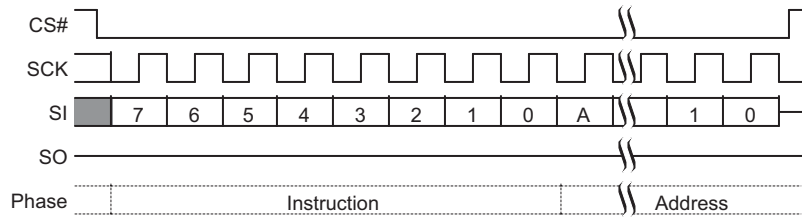
Figure 9.61 PPBP Command Sequence
