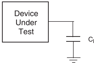
Figure 5.2 Test Setup
