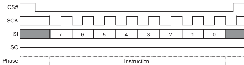
Figure 9.62 PPB Erase Command Sequence
