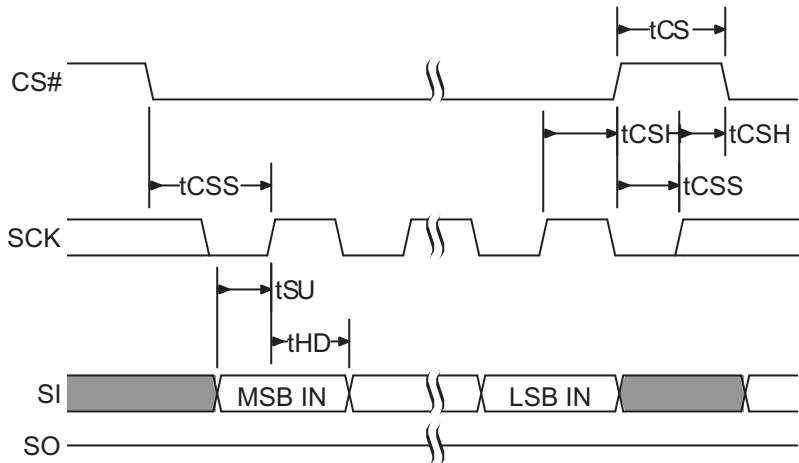
Figure 5.10 SPI Single Bit Input Timing
