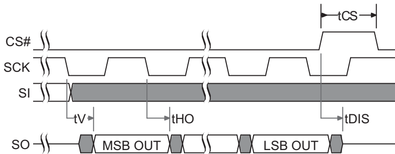
Figure 5.11 SPI Single Bit Output Timing
