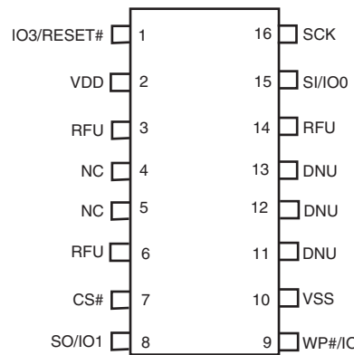
Figure 6.1 16-Lead SOIC Package, Top View
