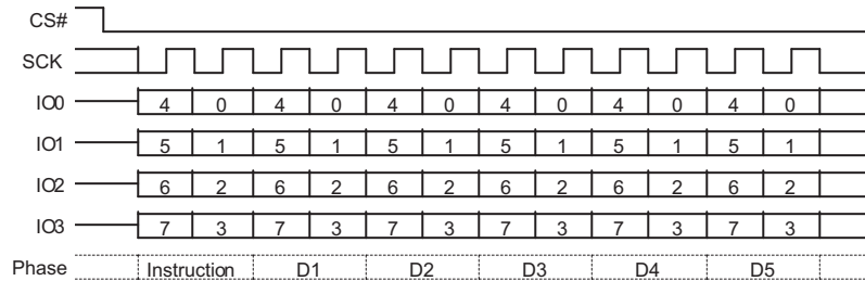
Figure 9.3 Read Quad Identification (RDQID) Command Sequence
