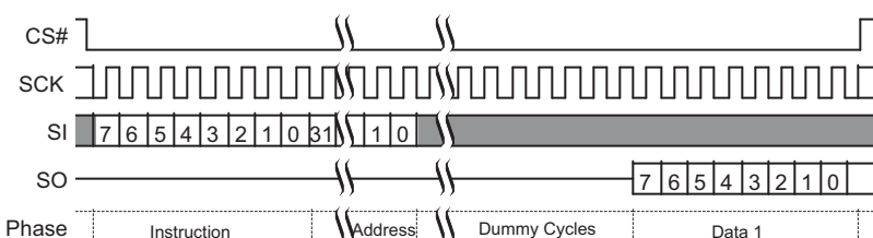
Figure 3.7 Single Bit Wide I/O Command with latency
