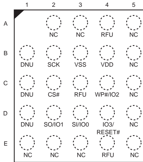
Figure 6.5 24-Ball BGA, 5x5 Ball Footprint (FAB024), Top View
