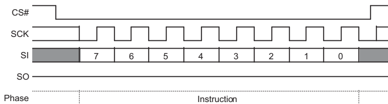
Figure 9.45 Bulk Erase Command Sequence
