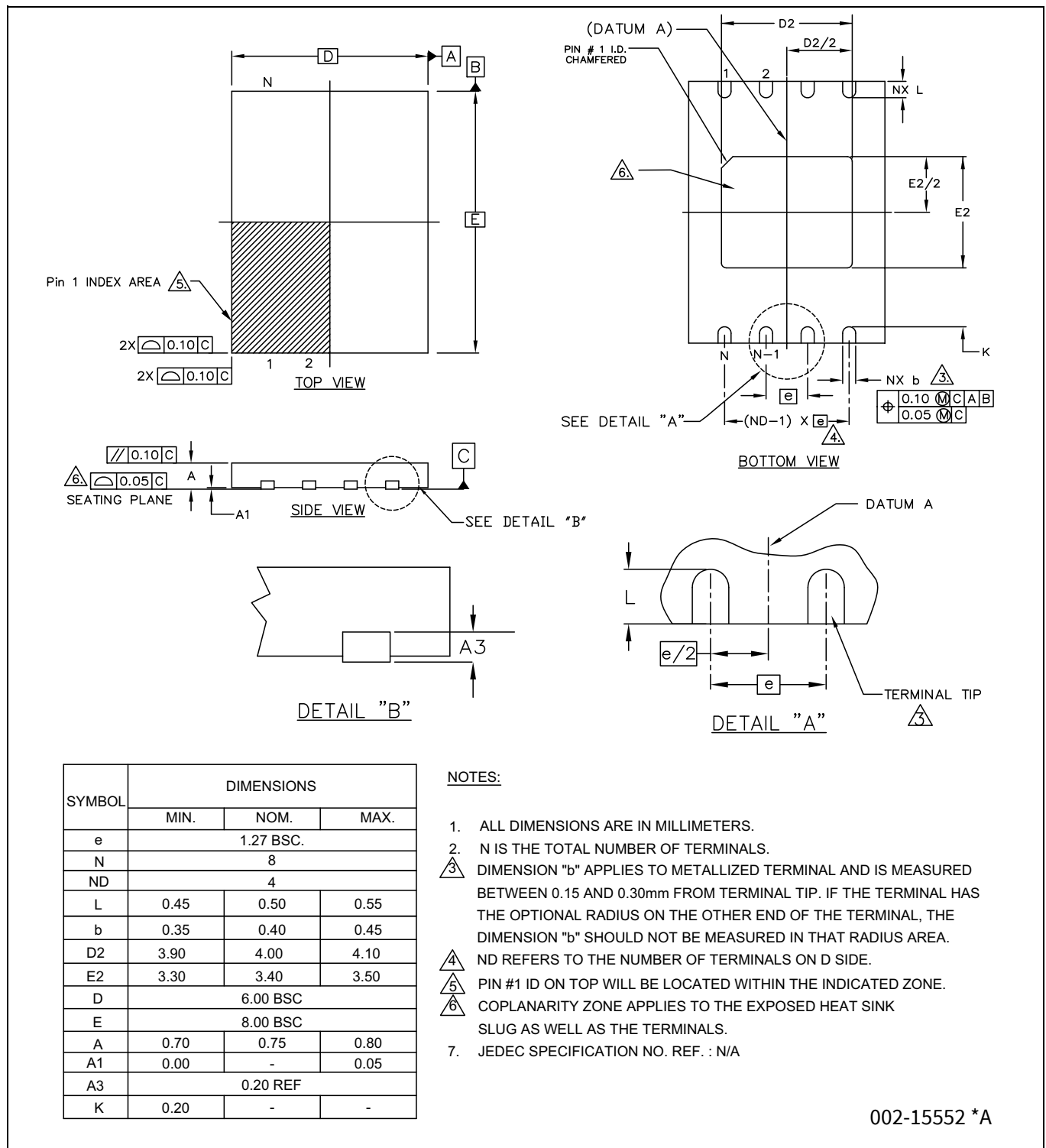
Figure 116 WSON 8-lead DFN 6.0 x 8.0 x 0.8 mm (WNH008) WNH008 4.0 x 3.4 mm E-Pad (SAWN)(PG-WSON-8)
