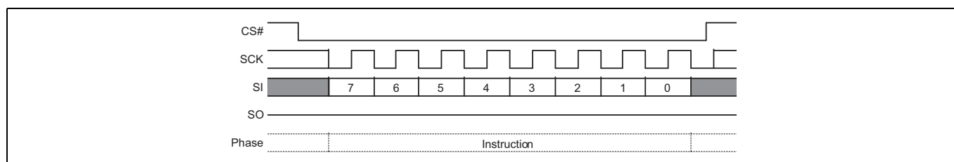
Figure 107 Software Reset command sequence
