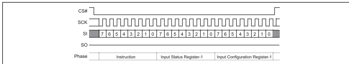
Figure 50 Write Registers (WRR) command sequence – 16 data bits
