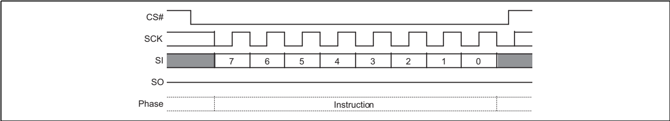
Figure 113 Release from Deep Power-Down command sequence
