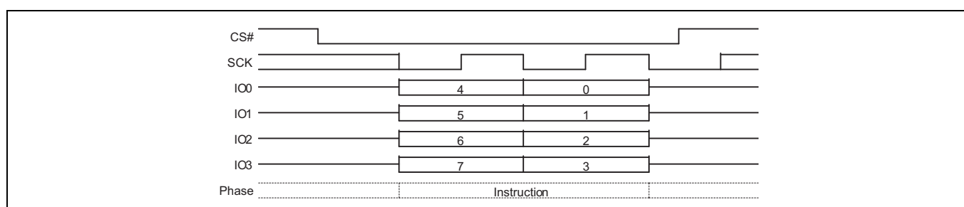
Figure 108 Software Reset command sequence QPI mode
