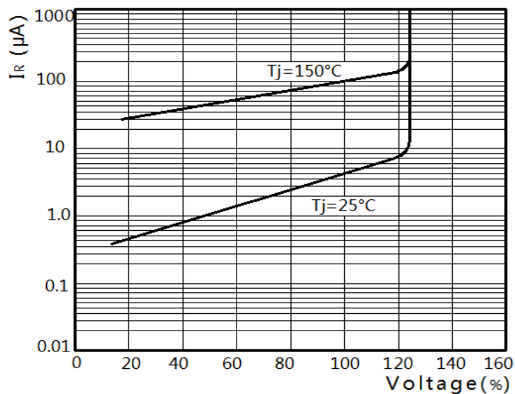
FIGURE 2. REVERSE CURRENT vs REVERSE VOLTAGE
