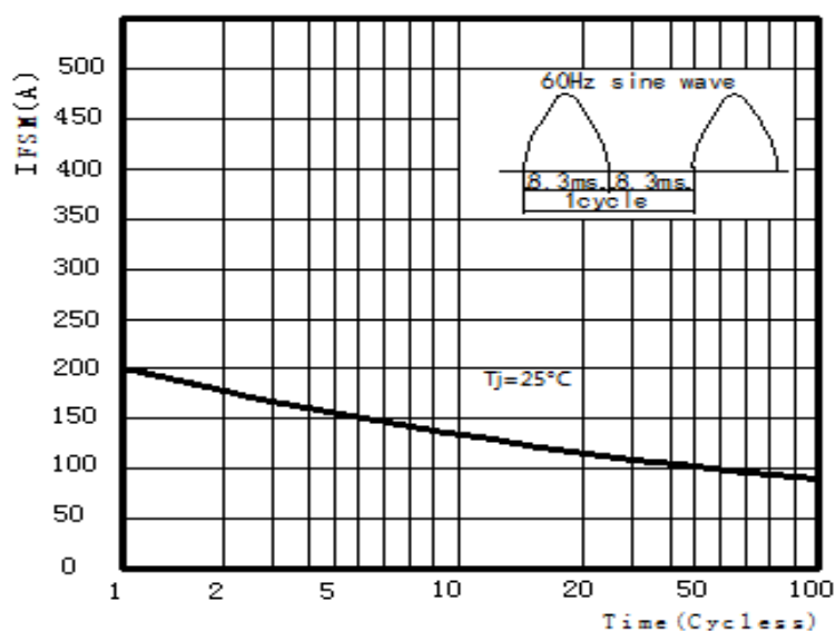
FIGURE 3. Peak Surge Forward Capability
