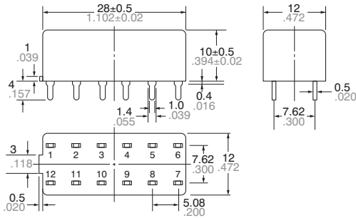
External dimensions
