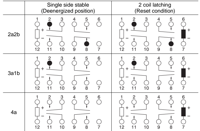
Schematic (Bottom view)
