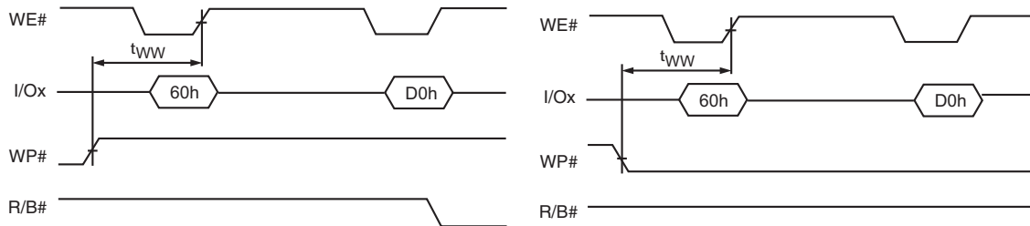
Figure 57. Erase Enabling / Disabling Through WP# Handling
