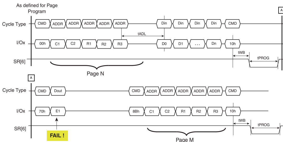
Figure 7. Page Reprogram
