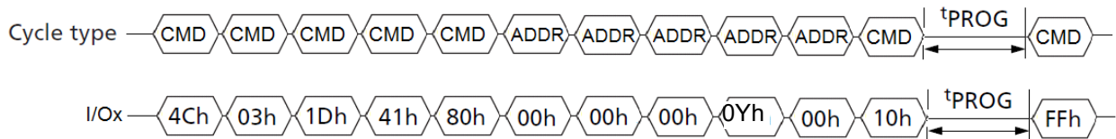
Figure 16. Timing Diagram for the PBP Sequence
