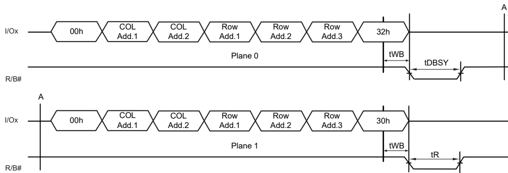
Figure 28. Multiplane Page Read Operation
