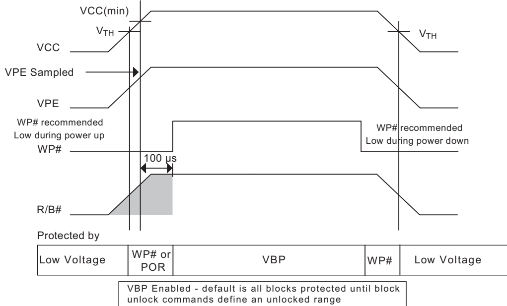
Figure 53. VPE High at Power up Timing
