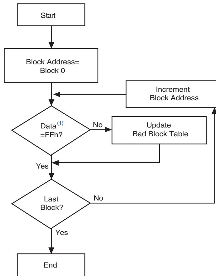
Figure 65. Bad Block Management Flowchart
