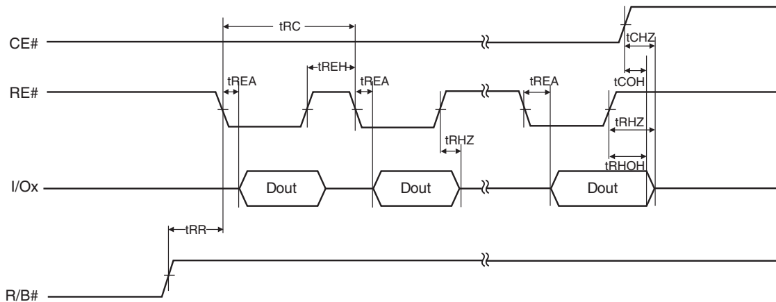
Figure 23. Data Output Cycle Timing
