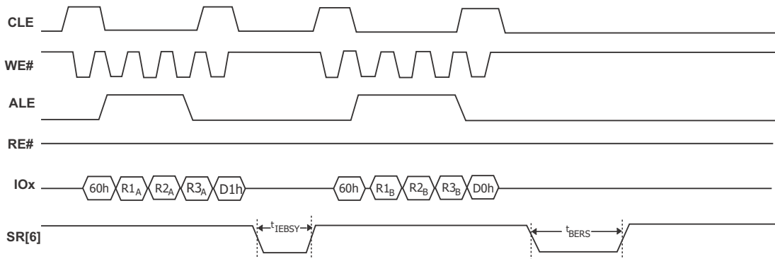
Figure 38. Multiplane Block Erase (ONFI 1.0 Protocol)
