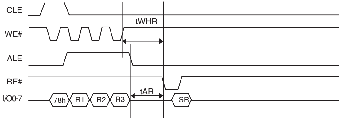
Figure 44. Read Status Enhanced Timing
