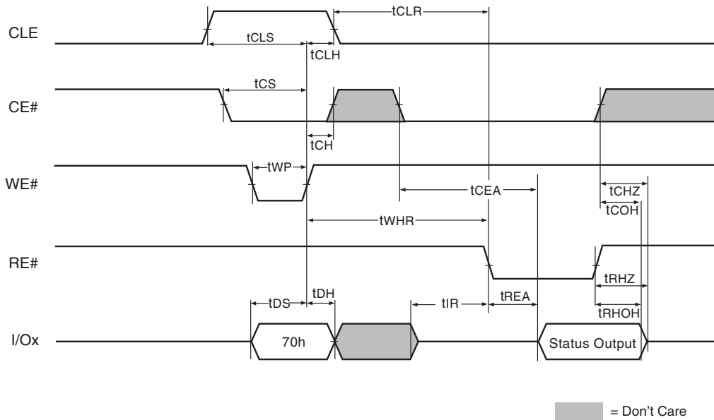
Figure 43. Read Status Cycle
