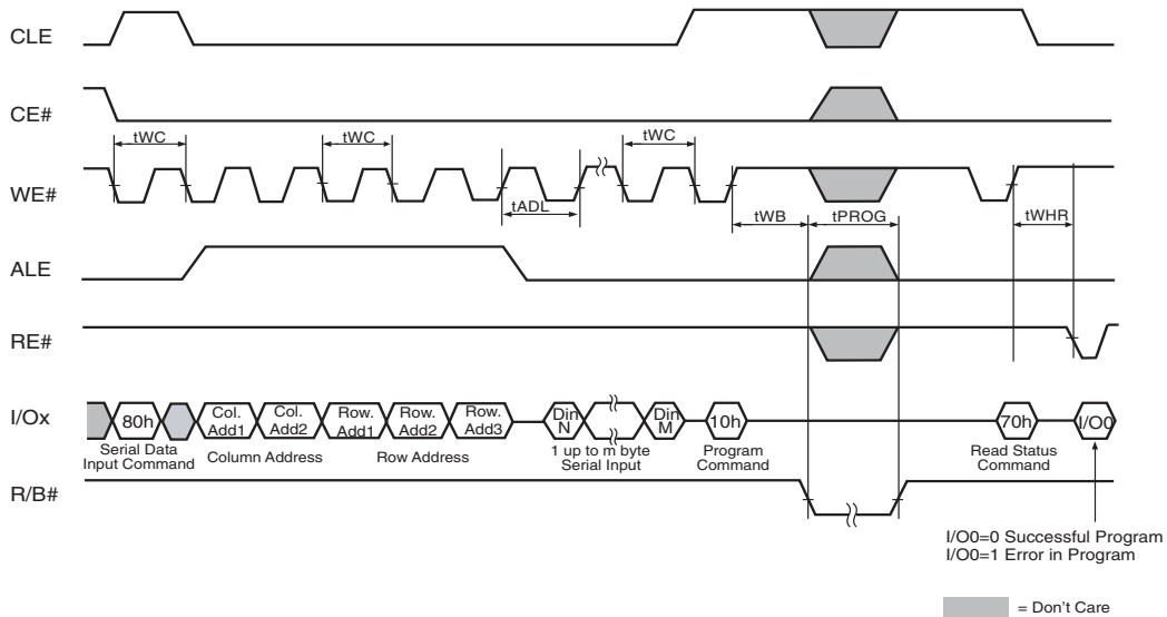
Figure 29. Page Program Operation
