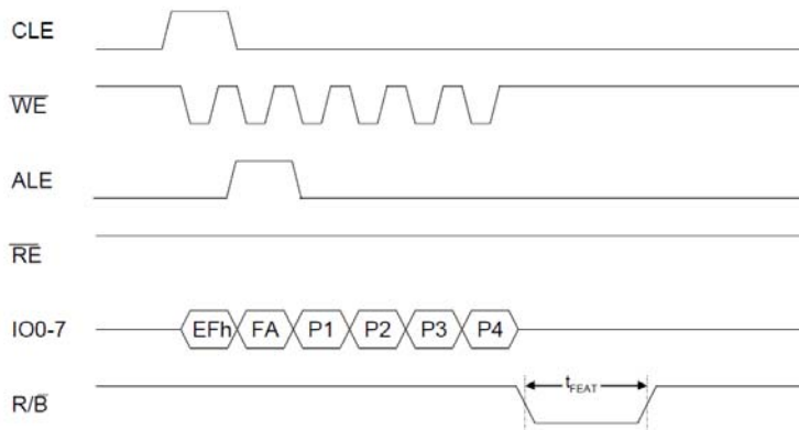
Figure 9. Set Features Timing
