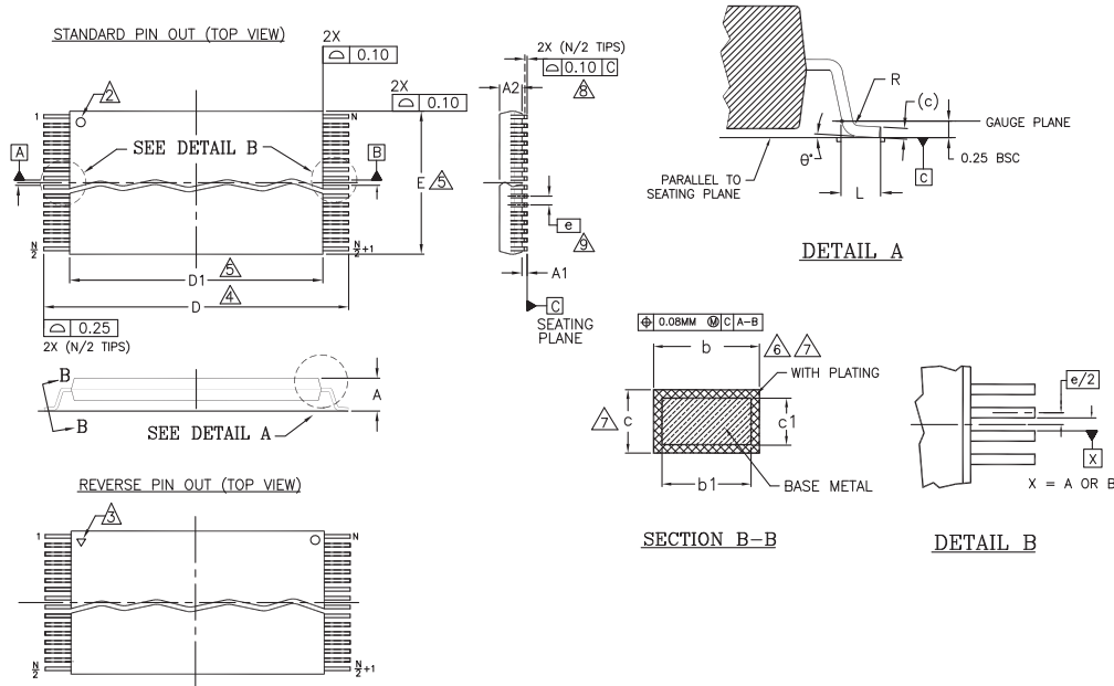
Figure 58. TS/TSR 48 — 48-lead Plastic Thin Small Outline, 12 x 20 mm, Package Outline
