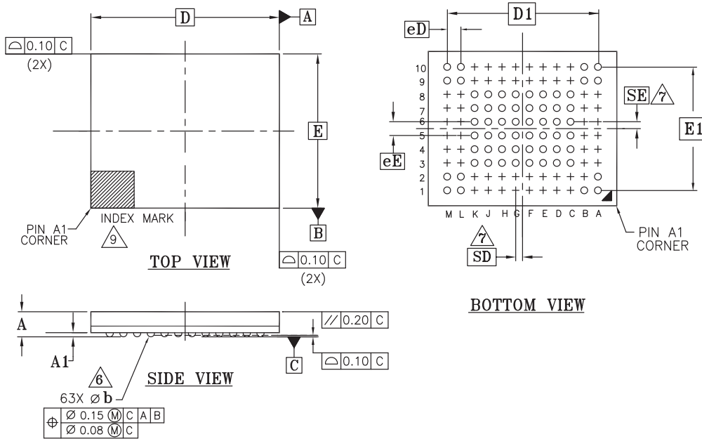
Figure 59. VBM063 — 63-Pin BGA, 11 mm x 9 mm Package
