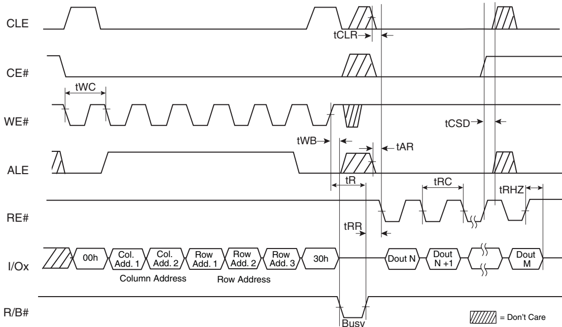
Figure 25. Page Read Operation (Read One Page)
