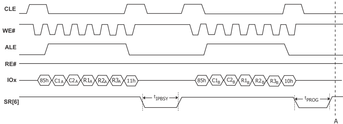
Figure 42. Multiplane Copy Back Program (ONFI 1.0 Protocol)
