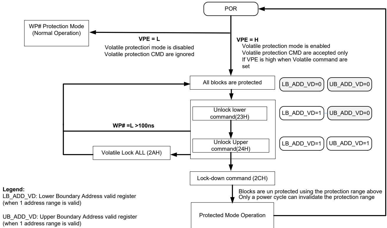
Figure 11. VBP Flowchart
