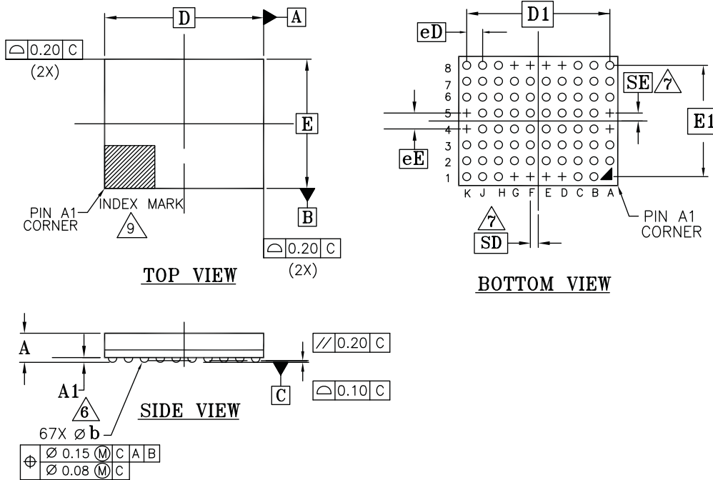
Figure 60. VBT067 — 67-Ball BGA, 8 x 6.5 mm Package
