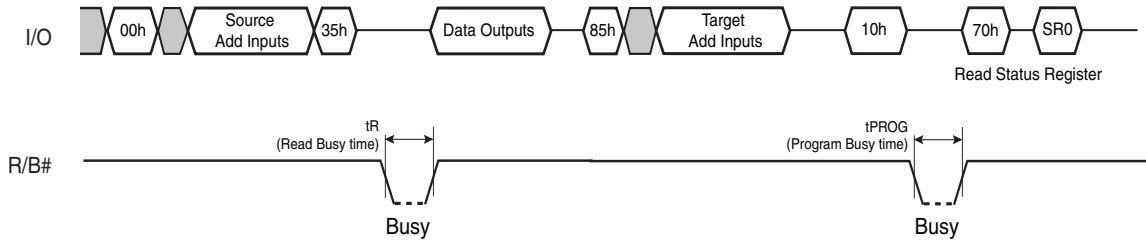
Figure 39. Copy Back Read with Optional Data Readout
