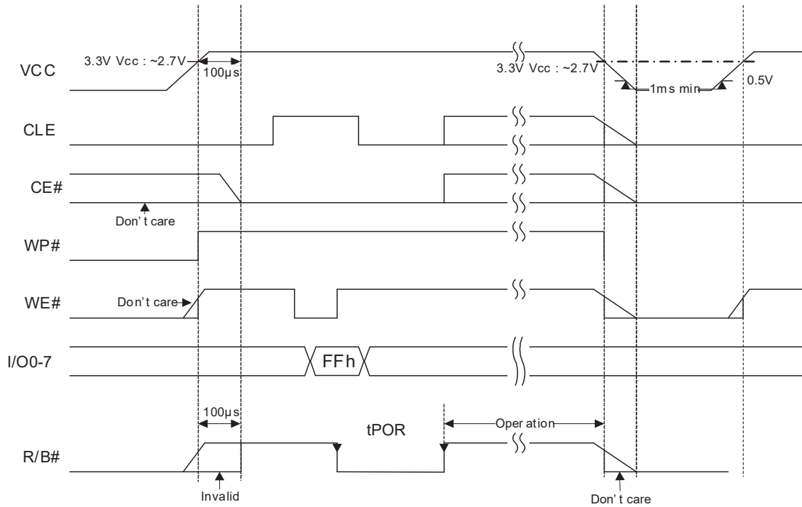
Figure 55. Device Initialization
