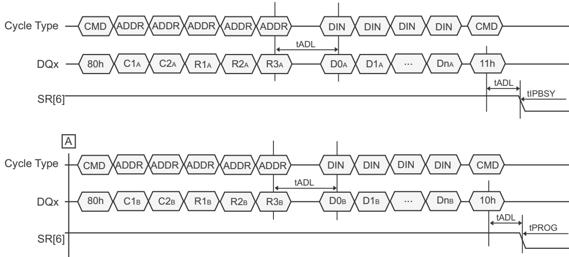
Figure 35. Multiplane Page Program (ONFI 1.0 Protocol)
