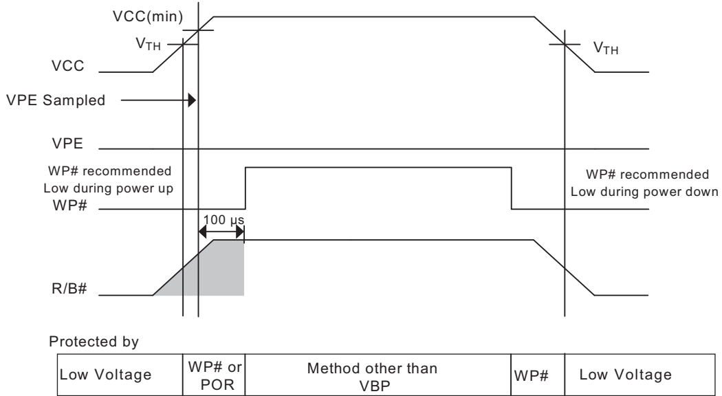
Figure 54. VPE LOW at Power up Timing
