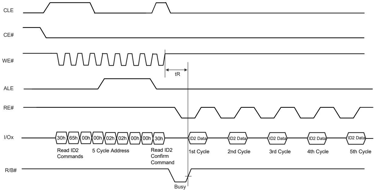
Figure 47. Read ID2 Operation Timing
