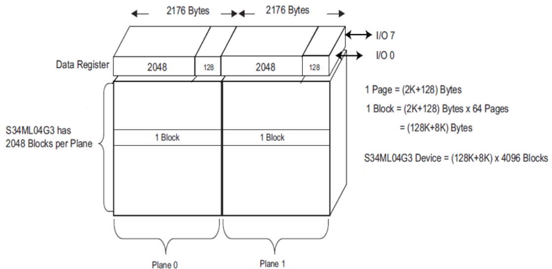
Figure 6. Array Organization
