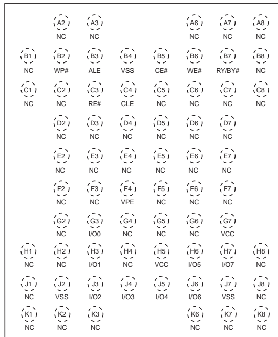
Figure 4. 67-BGA Contact (Balls Down, Top View)
