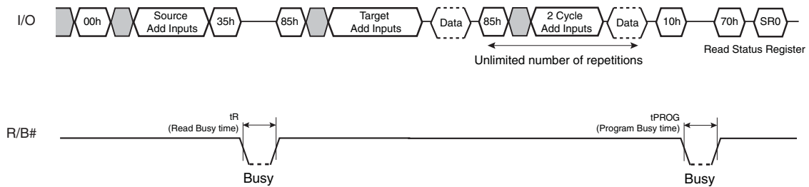
Figure 40. Copy Back Program with Random Data Input
