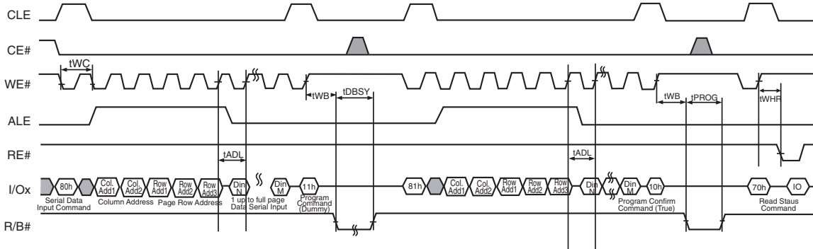
Figure 34. Multiplane Page Program
