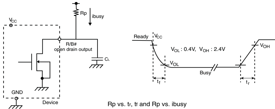
Figure 18. Ready/Busy Pin Electrical Application
