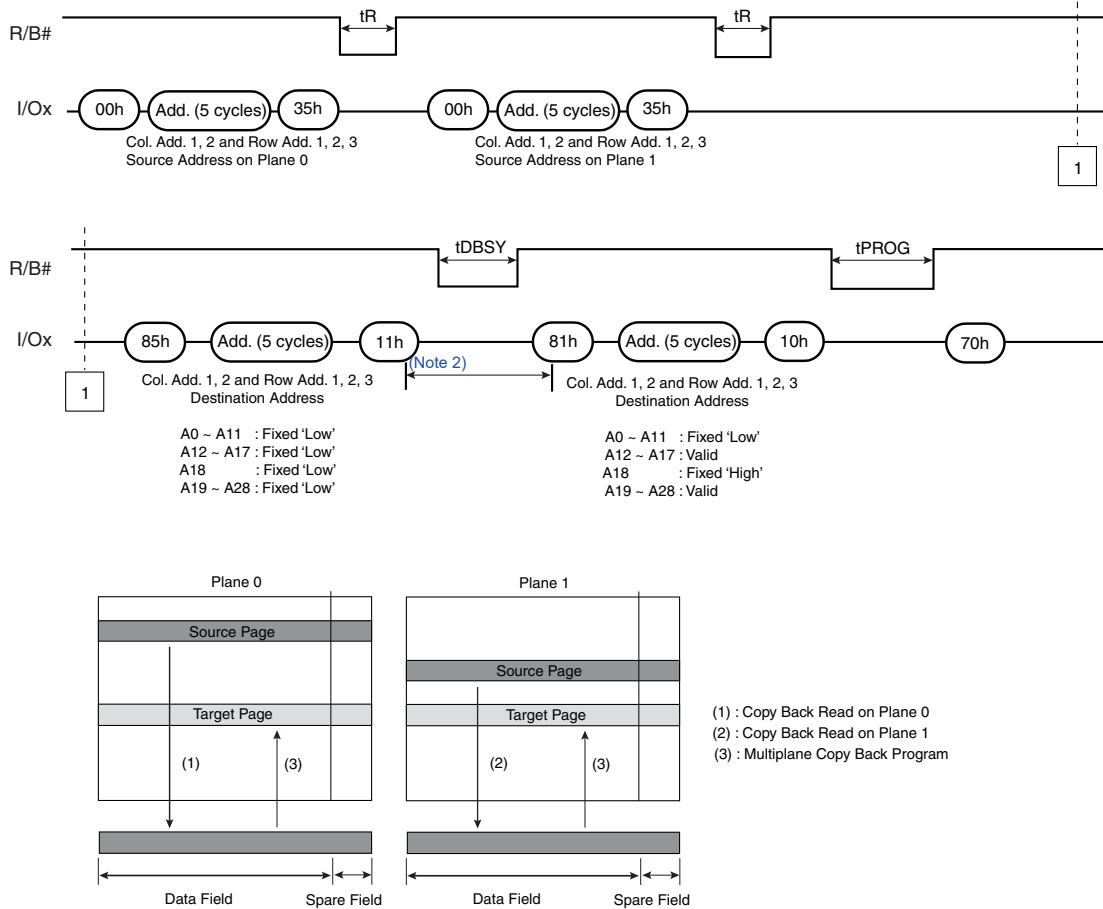
Figure 41. Multiplane Copy Back Program
