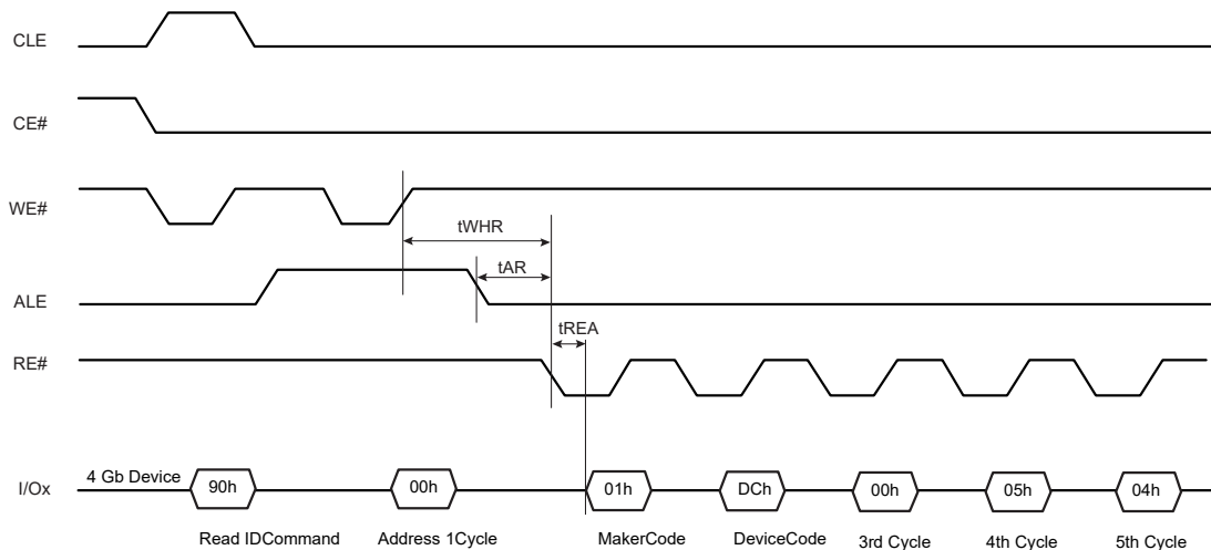
Figure 46. Read ID Operation Timing
