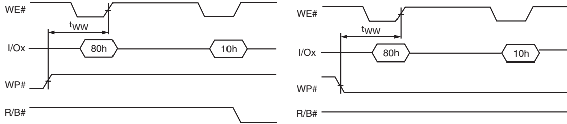
Figure 56. Program Enabling / Disabling Through WP# Handling
