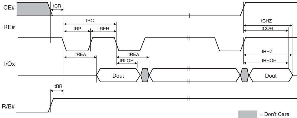
Figure 24. Data Output Cycle Timing (EDO)
