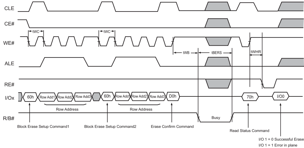
Figure 37. Multiplane Block Erase
