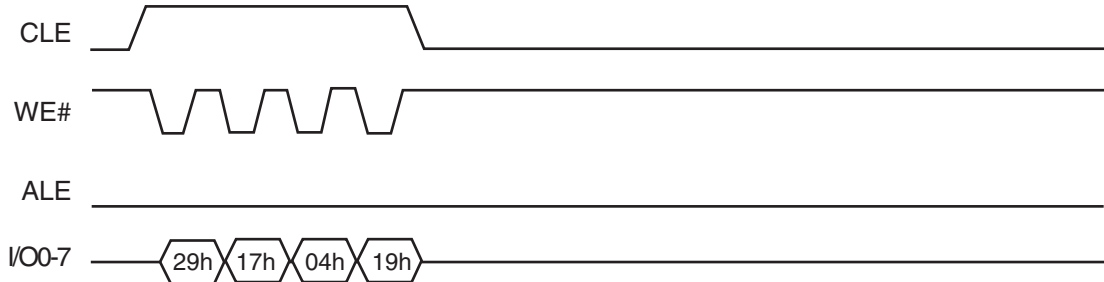
Figure 51. OTP Entry Timing
