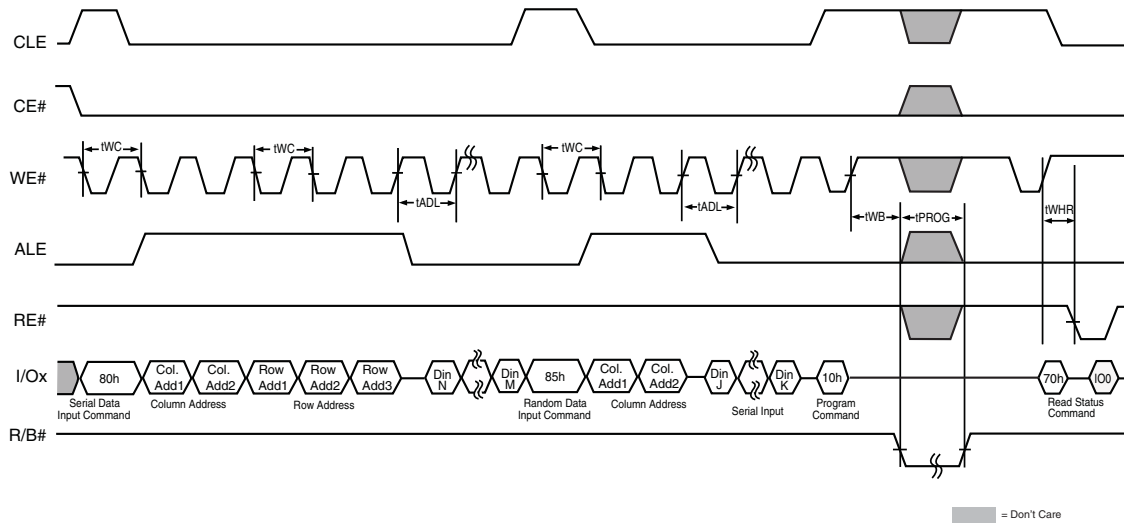
Figure 32. Random Data Input
