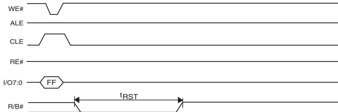
Figure 45. Reset Operation Timing
