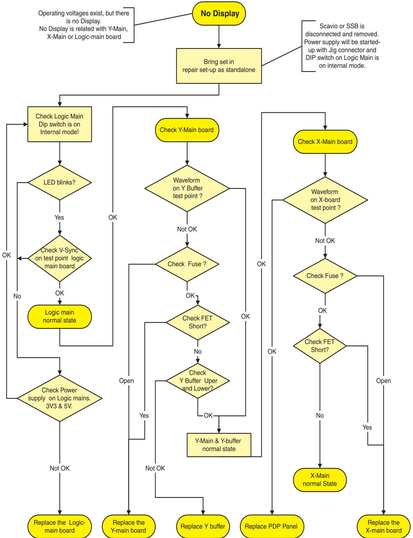
Figure 5-13 Fault symptom: "No Display"
