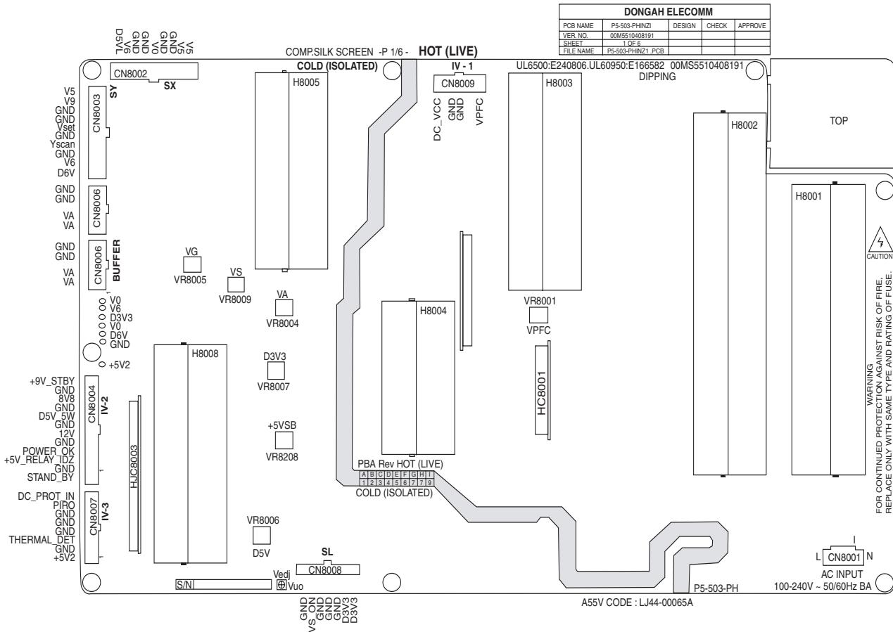
Figure 6-15 PSU layout
