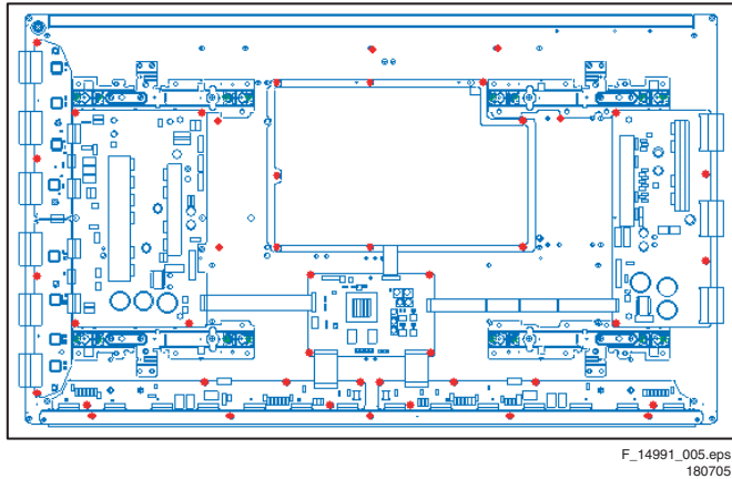
Figure 1-8 Points of screw mount (42" SD v4)
