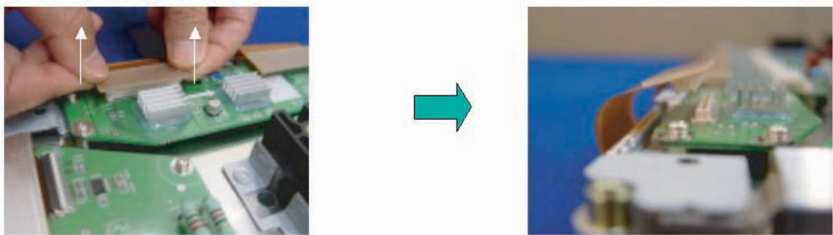
Figure 4-1 Dis-assembly FPC of Y-buffer
