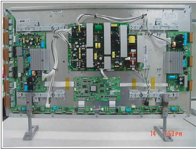
Figure 1-11 External view (42" HD v4)
