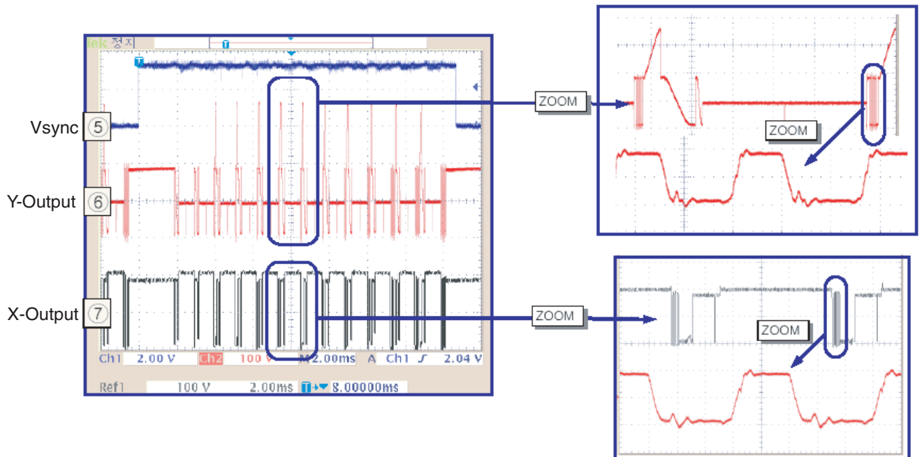
Figure 8-11 Waveform of X- and Y-board (42" SD v2)
