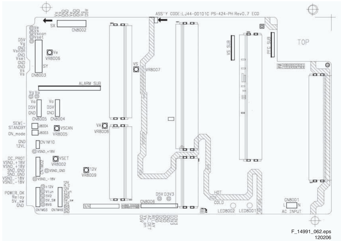
Figure 6-14 PSU layout
