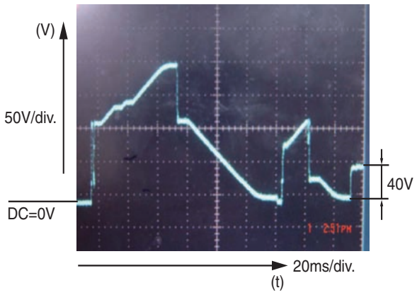
Figure 8-16 Rising ramp
