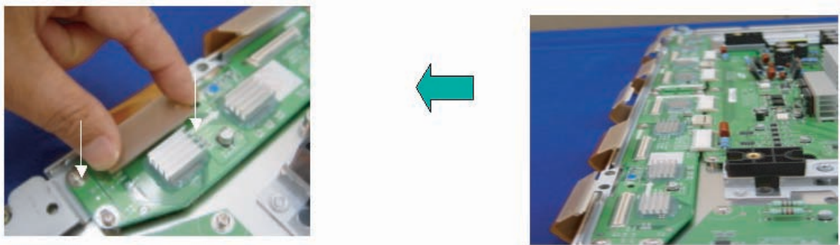
Figure 4-2 Re-assembly FPC of Y-buffer
