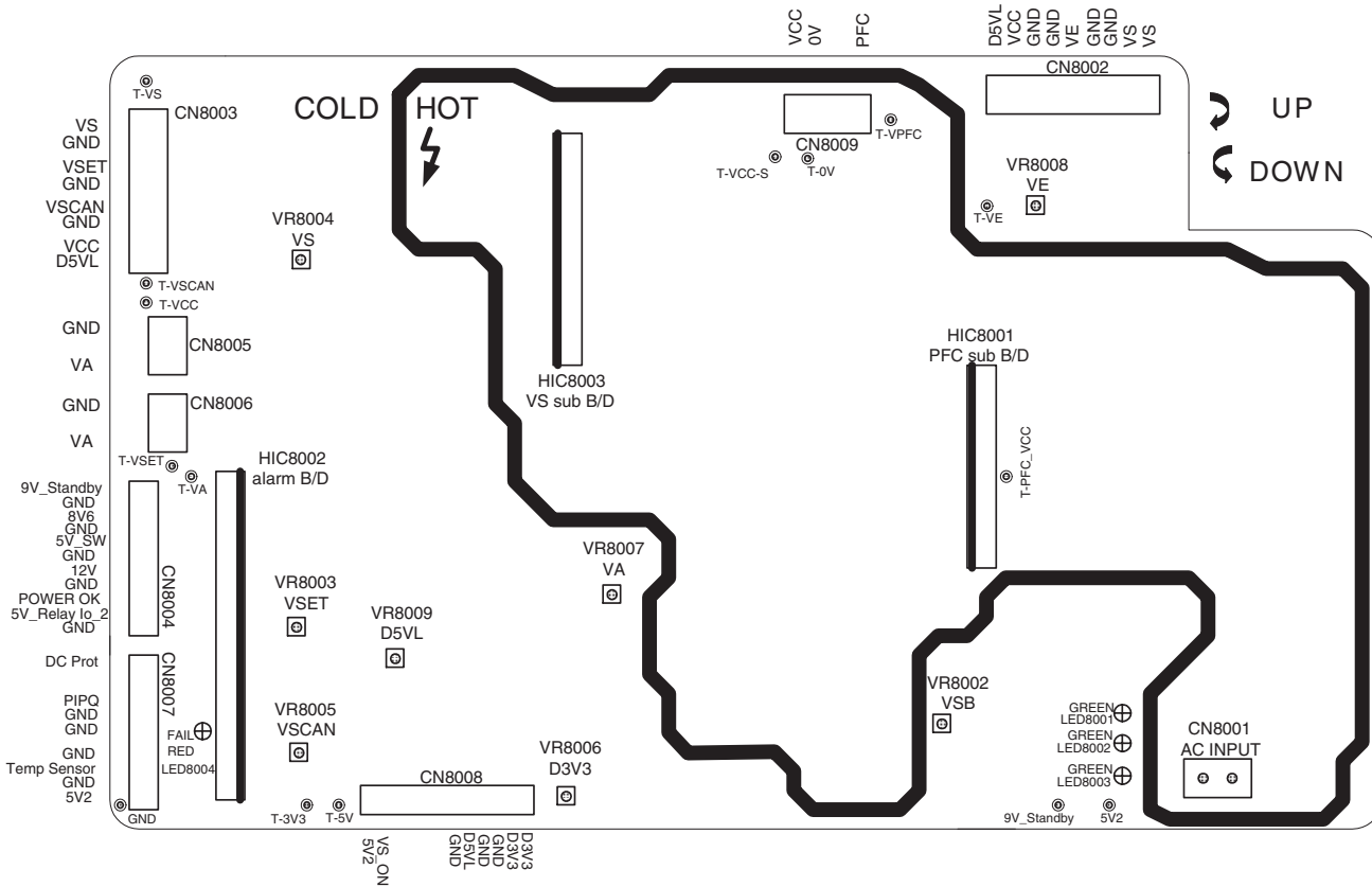
Figure 6-11 PSU layout
