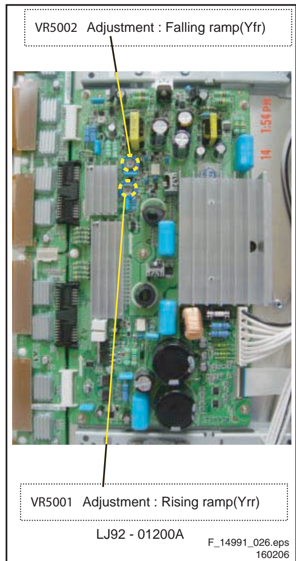
Figure 8-36 Potentiometer locations
