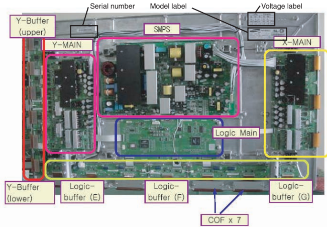
Figure 1-3 External view (42" SD v2)
