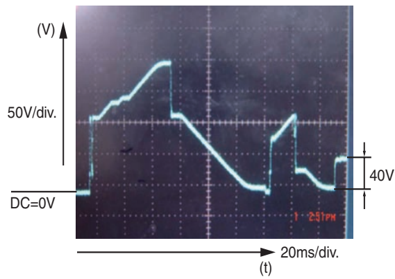
Figure 8-24 Rising ramp
