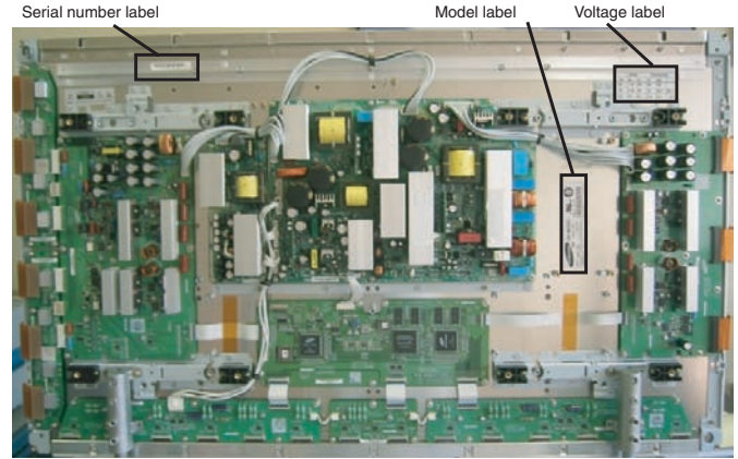
Figure 1-5 External view (42" SD v3)
