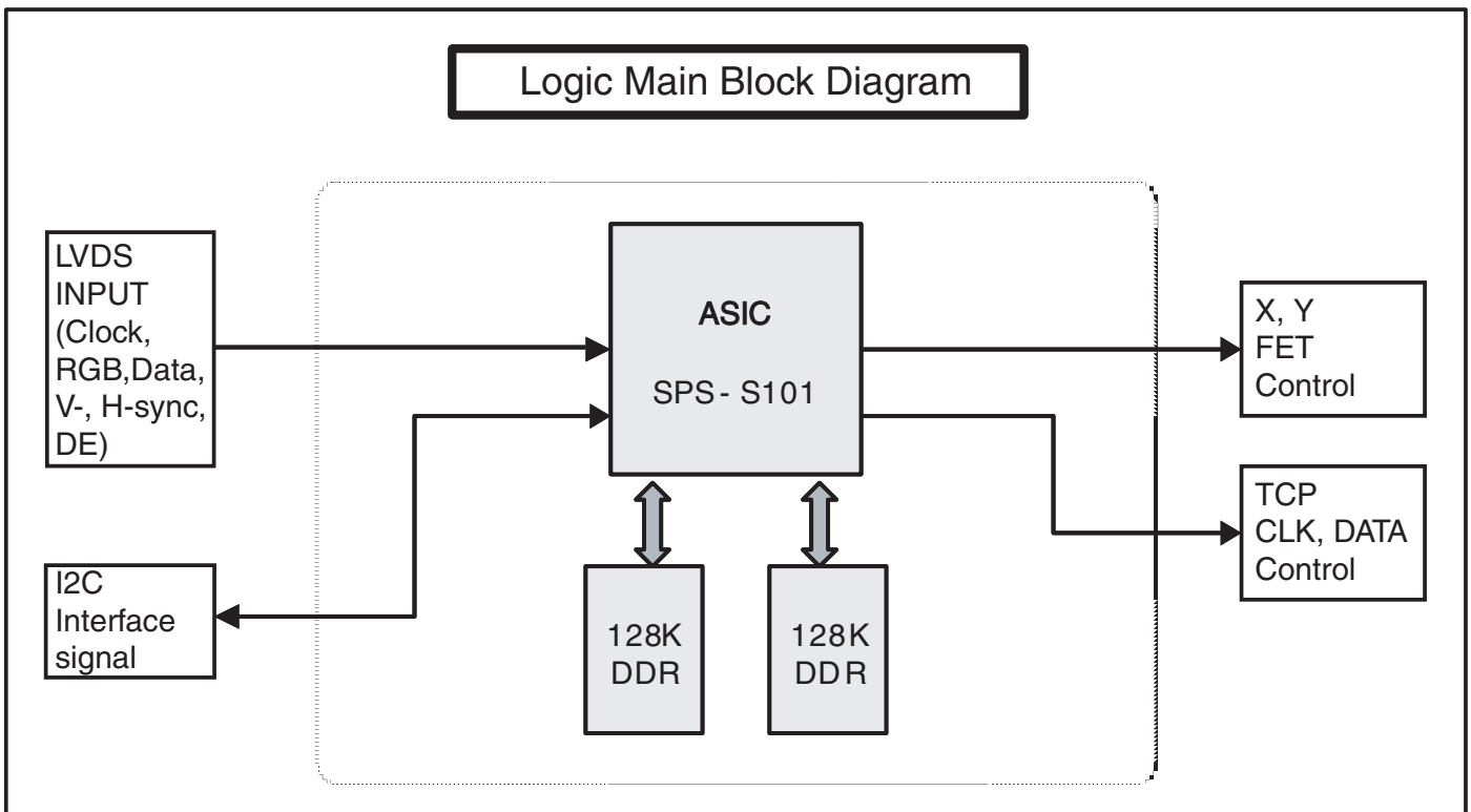
Figure 6-3 Block diagram (42" SD v3)
