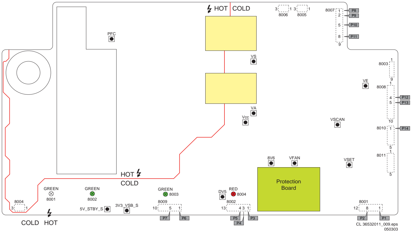
Figure 6-10 PSU layout
