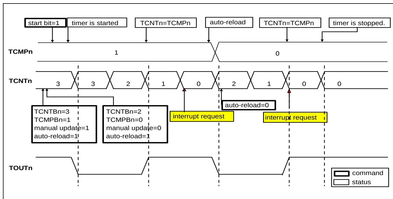
Figure 7-2. Timer operations
