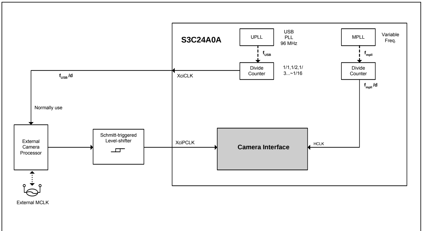
Figure 21-6. Clock Generation
