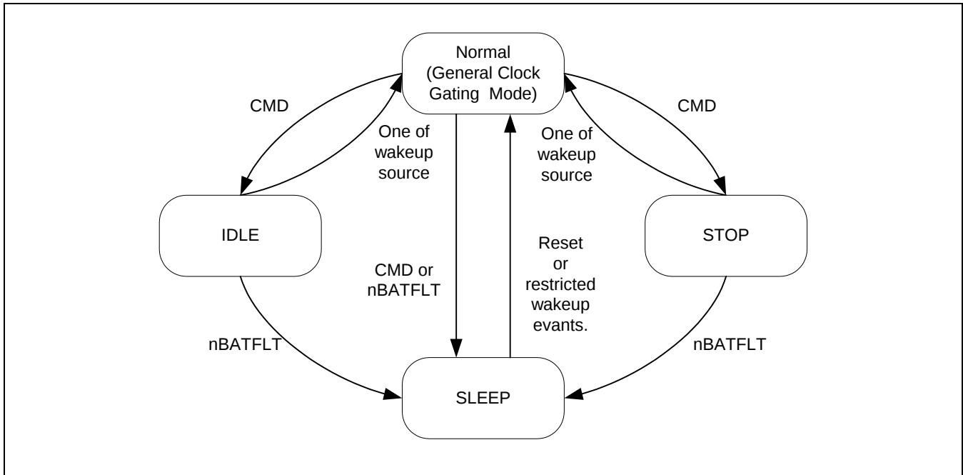
Figure 33-7. Power mode state diagram
