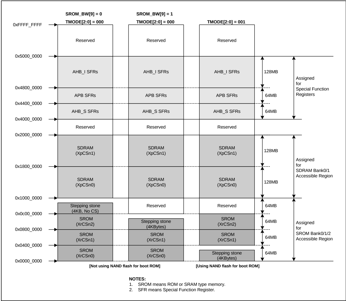
Figure 1-3. Address Map
