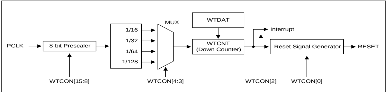
Figure 8-1. Watchdog Timer Block Diagram
