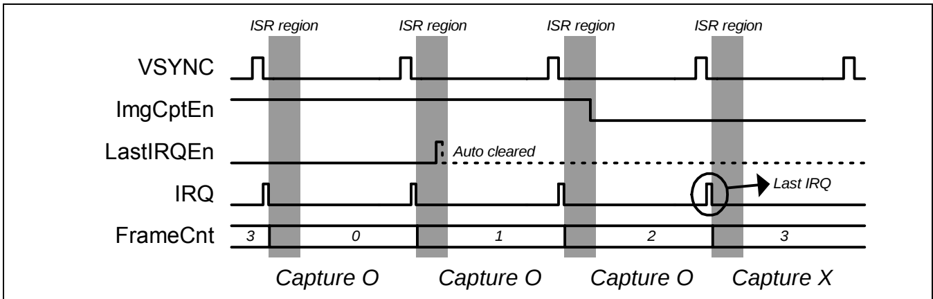
Figure 21-10. Timing Diagram for Last IRQ
