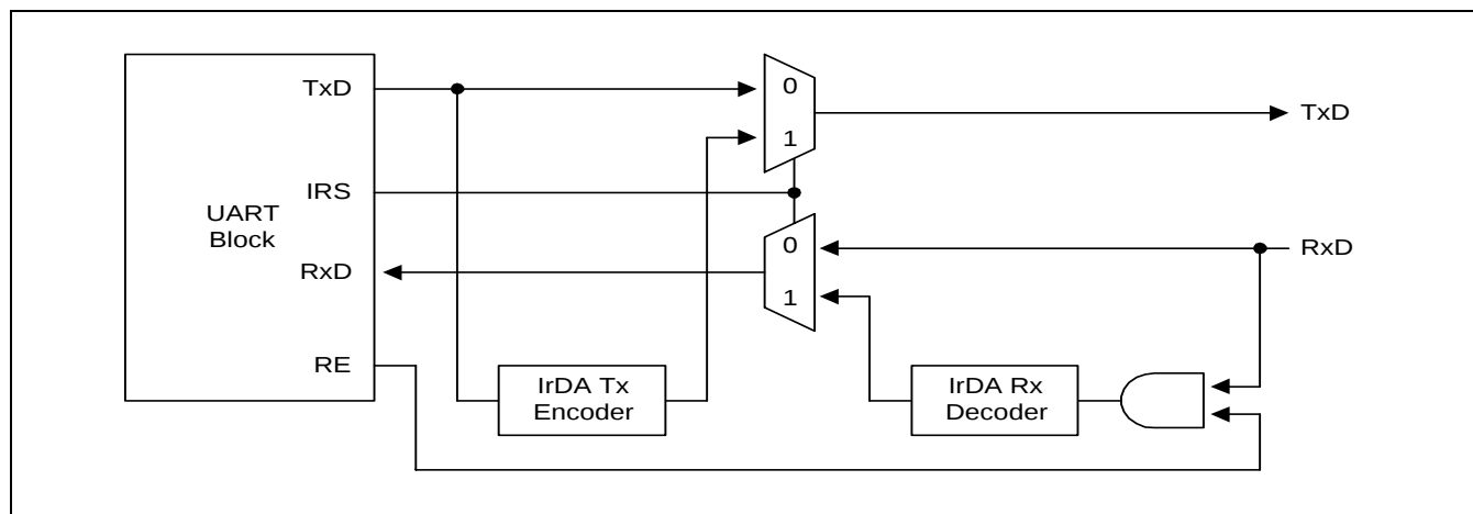
Figure 11-4. IrDA Function Block Diagram
