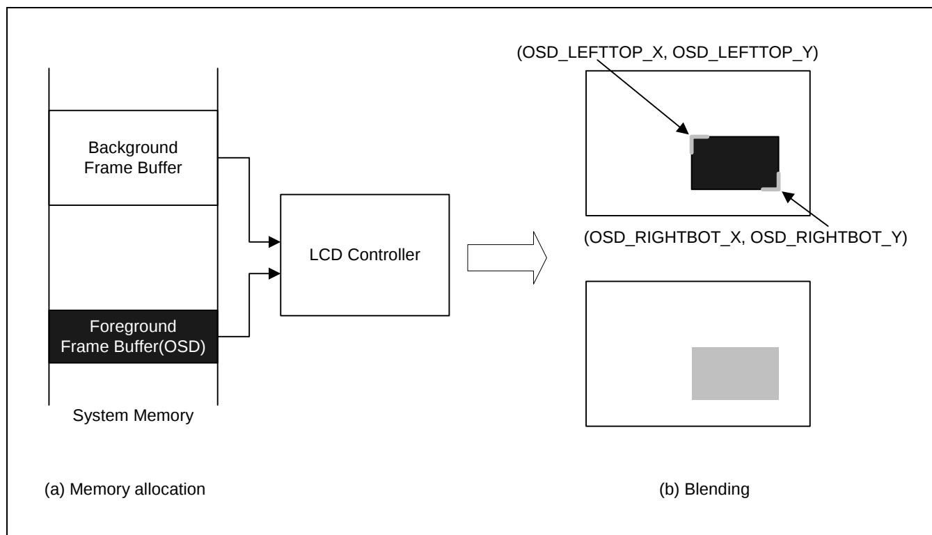
Figure 28-3. OSD Procedure
