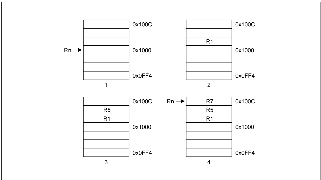
Figure 3-20. Pre-Increment Addressing
