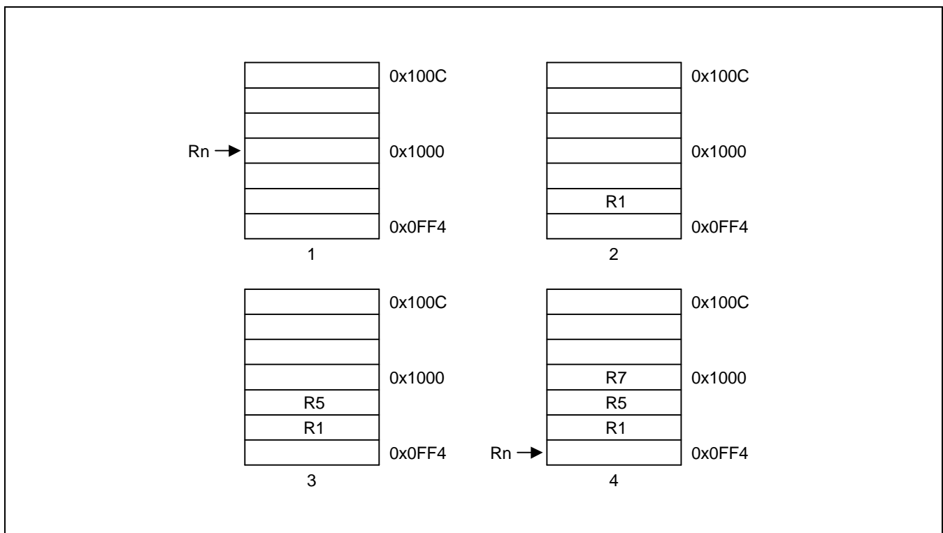
Figure 3-21. Post-Decrement Addressing
