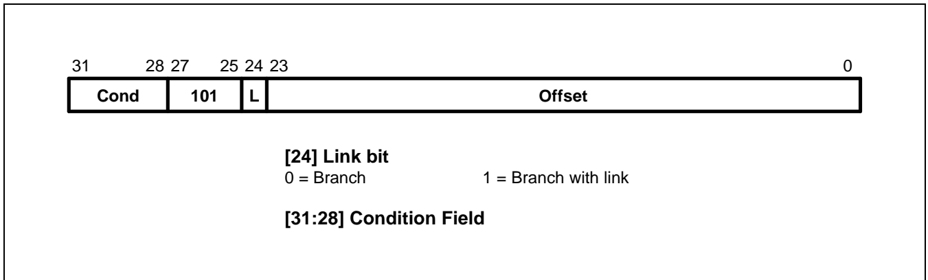
Figure 3-3. Branch Instructions
