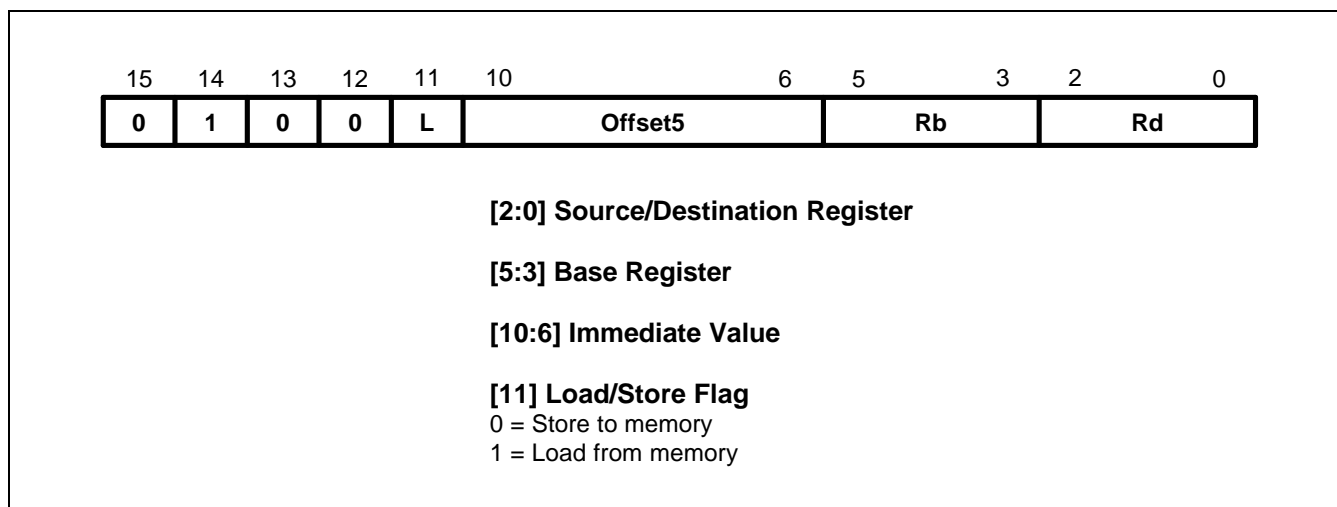
Figure 3-39. Format 10
