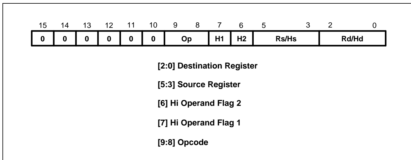
Figure 3-34. Format 5
