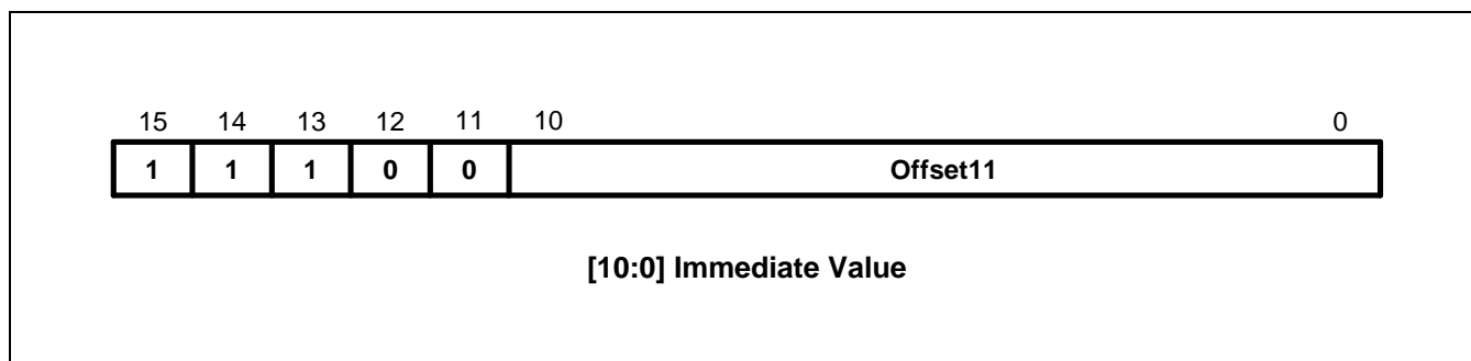
Figure 3-47. Format 18
