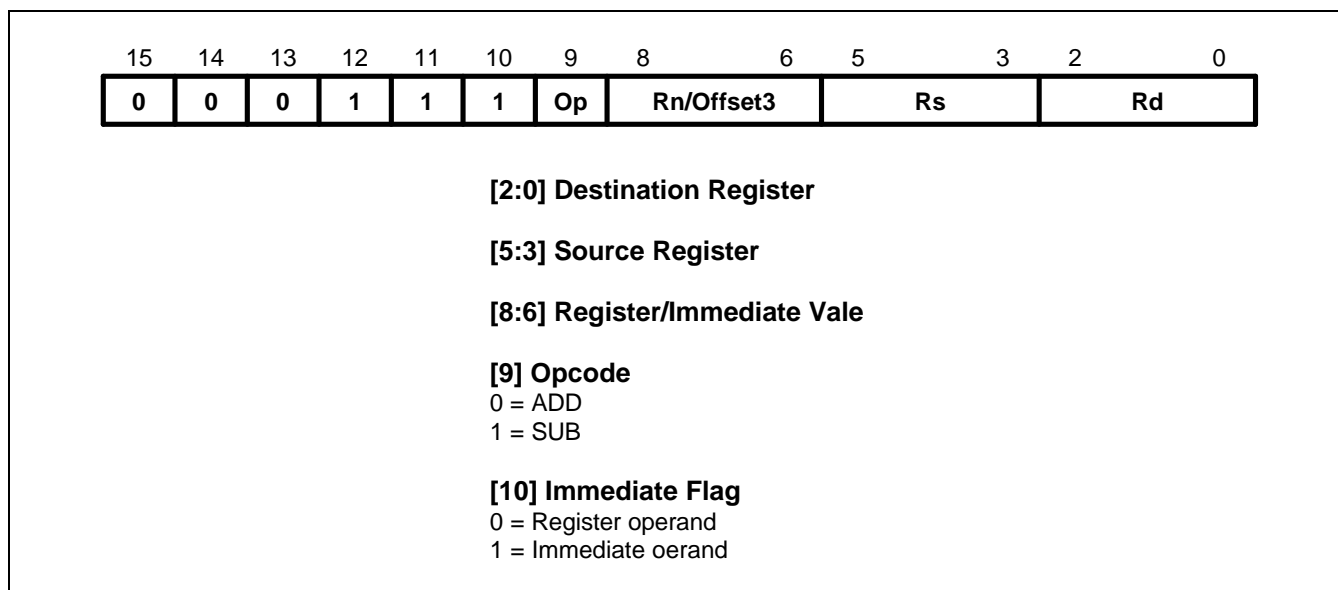
Figure 3-31. Format 2
