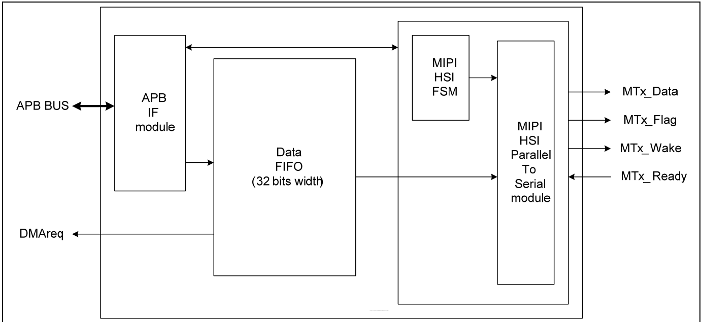
Figure 28-3. MIPI HSI interface controller Tx module Top Block Diagram
