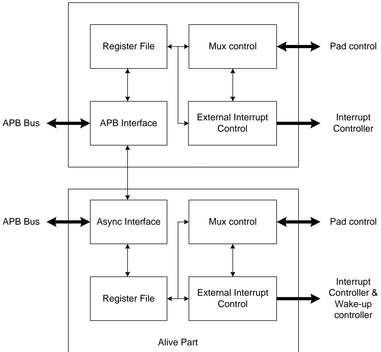
Figure 10-1 GPIO block diagram
