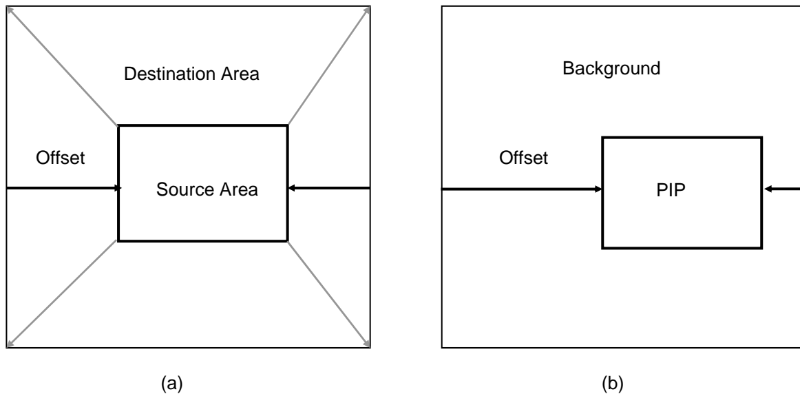
Figure 15-7 Offset address for (a) Source image for zoom in/out operation and (b) Destination image for PIP applications
