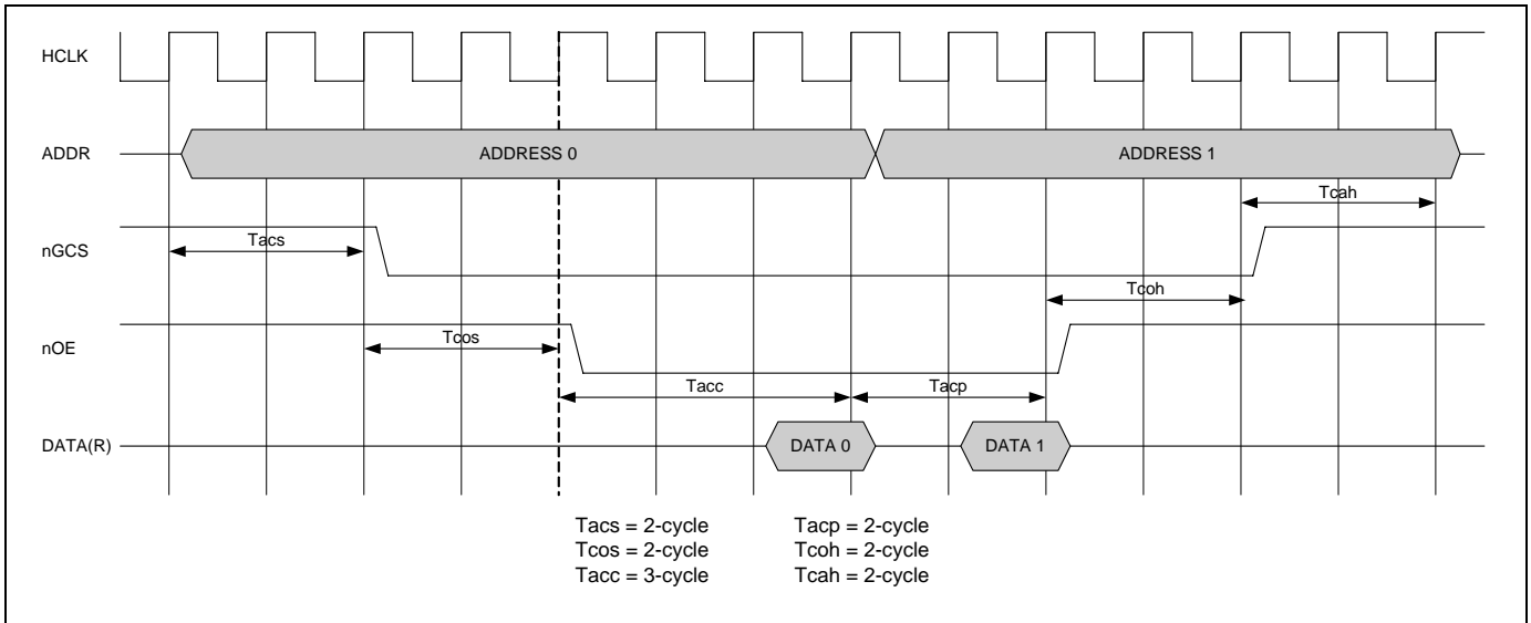
Figure 6-3 SROM Controller Read Timing Block Diagram
