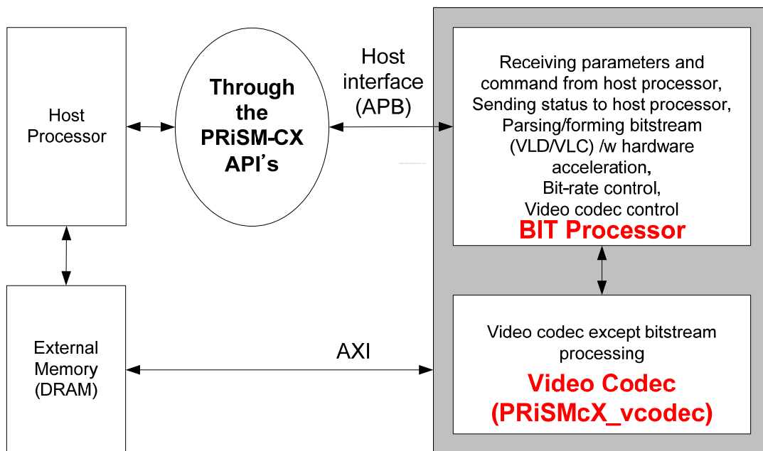
Figure 21.2. Roles of the BIT processor and the video codec module
