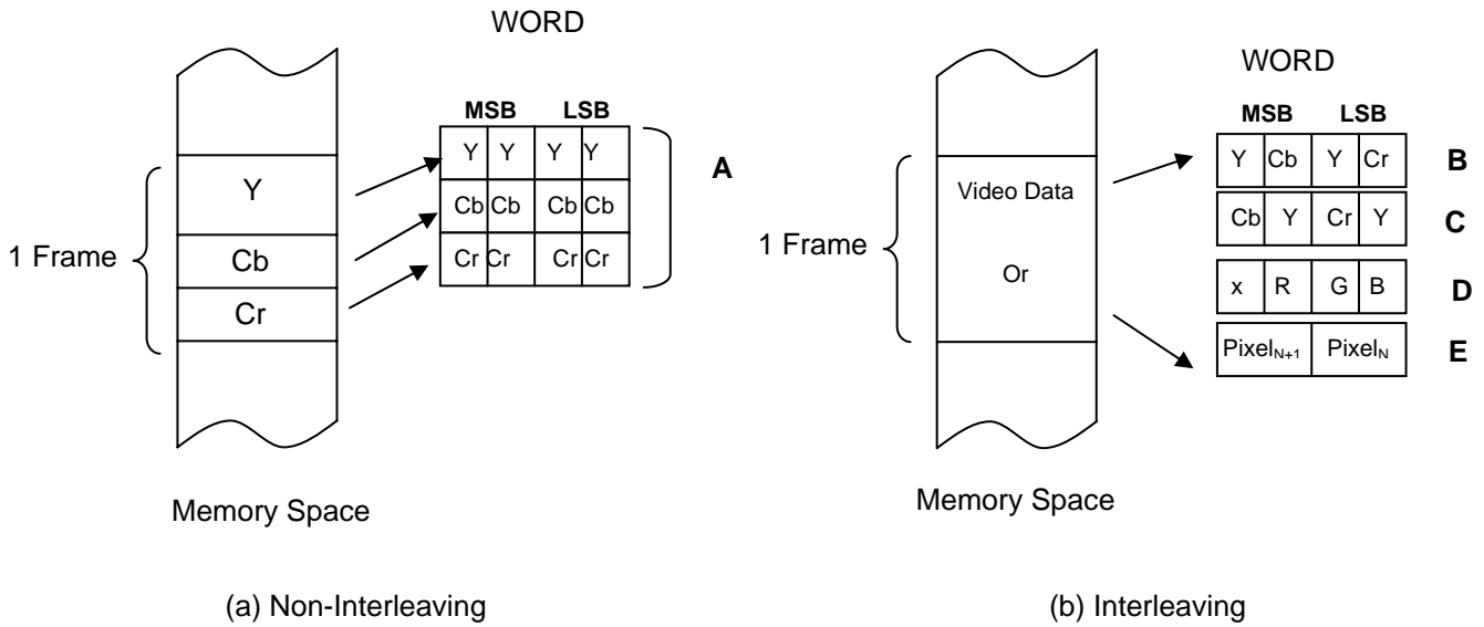
Figure 16-3 Data format stored in external
