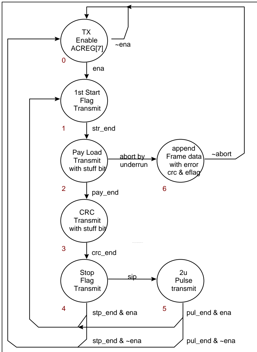
Figure 38-5 MIR modulation process.
