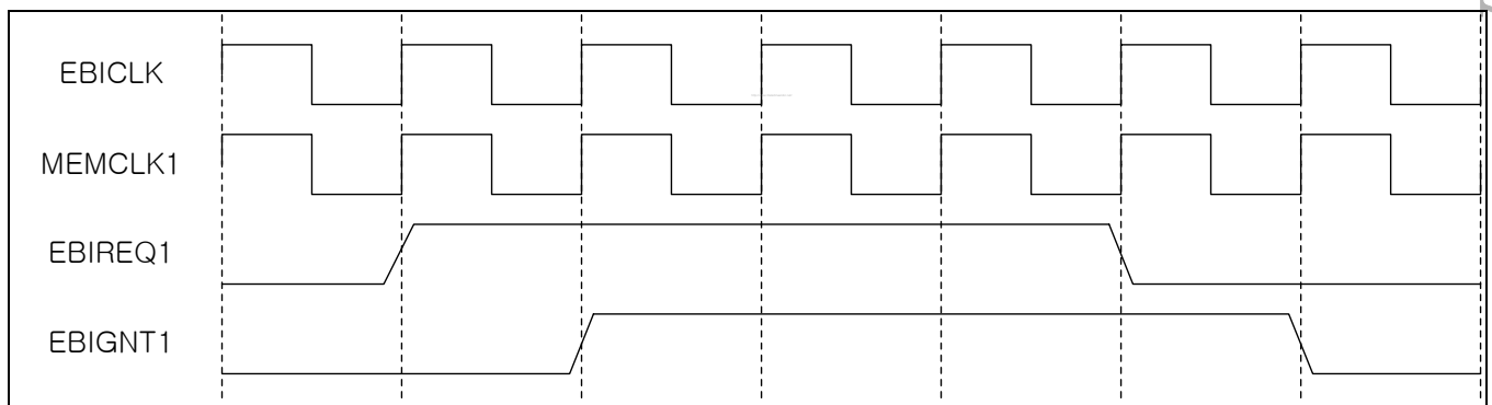
Figure 4-3. EBIREQ, EBIGANT signals
