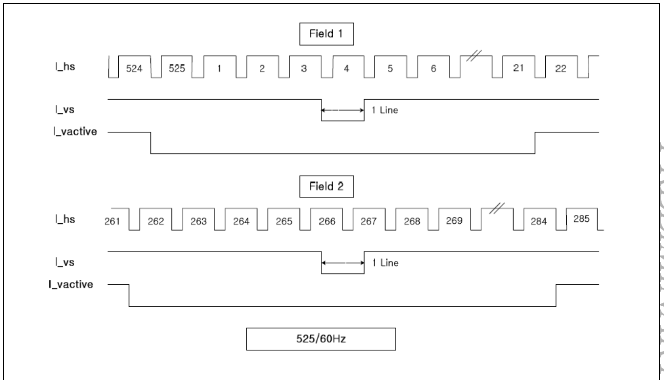
Figure 17-8. Requested Vertical Timing Diagram in 60Hz
