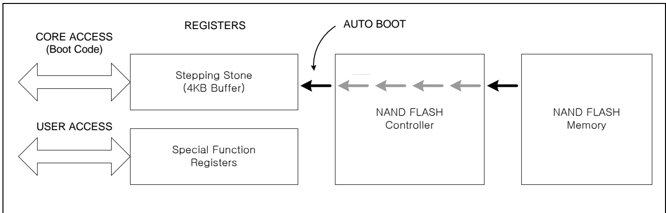
Figure 8-2 NAND Flash Controller Boot Loader Block Diagram
