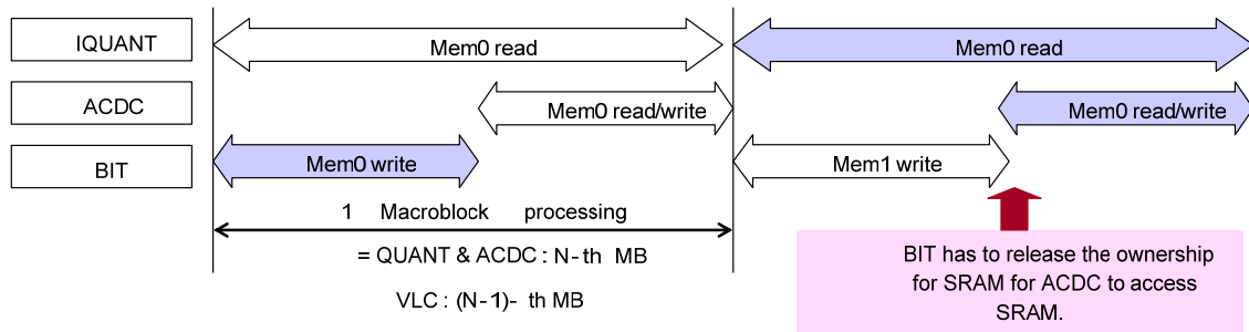
Figure 21.39 MPEG-4 decoding case
