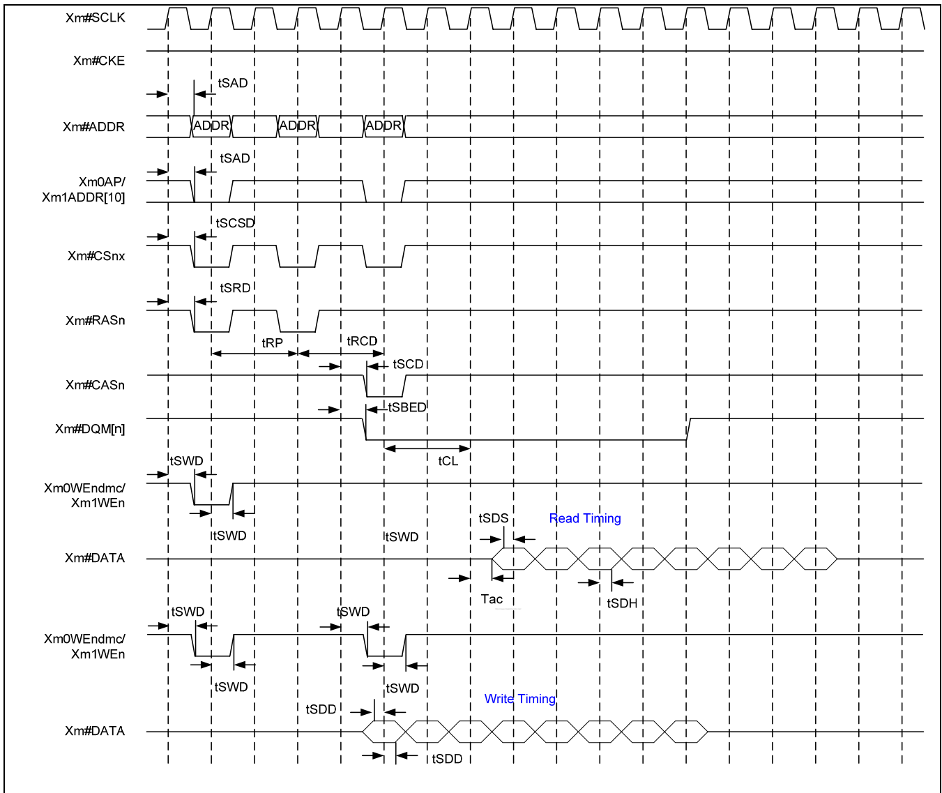
Figure 41-10. SDR SDRAM READ / WRITE Timing ( T_{rp} = 2 , T_{rcd} = 2 , T_{cl} = 2 , DW = 16-bit)
