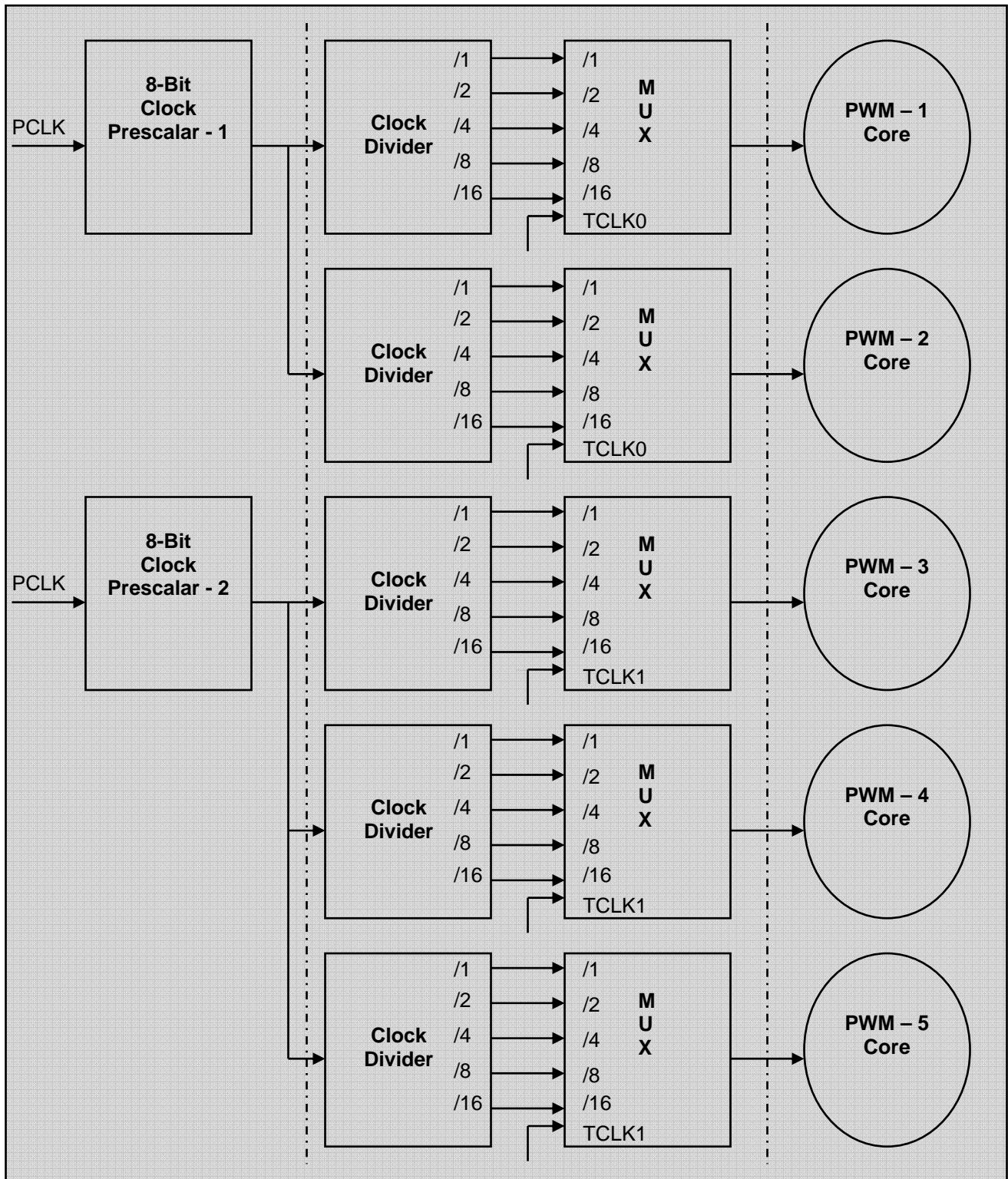
Figure 32-4: PWMTIMER Detailed Clock Tree Diagram
