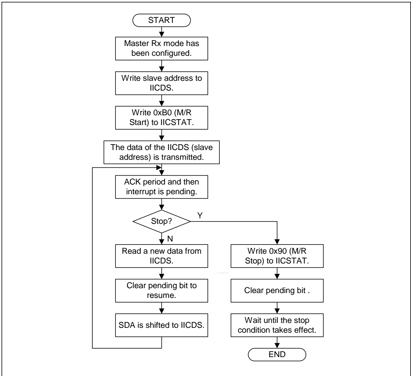
Figure 30-6. Operations for Master/Receiver Mode
