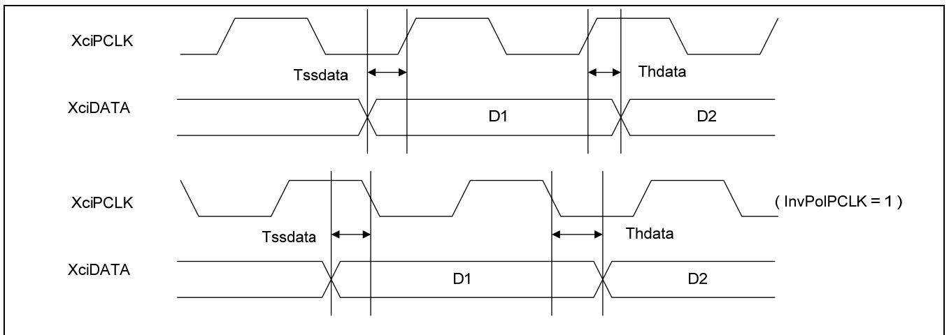
Figure 41-20. Camera Interface Data Timing
