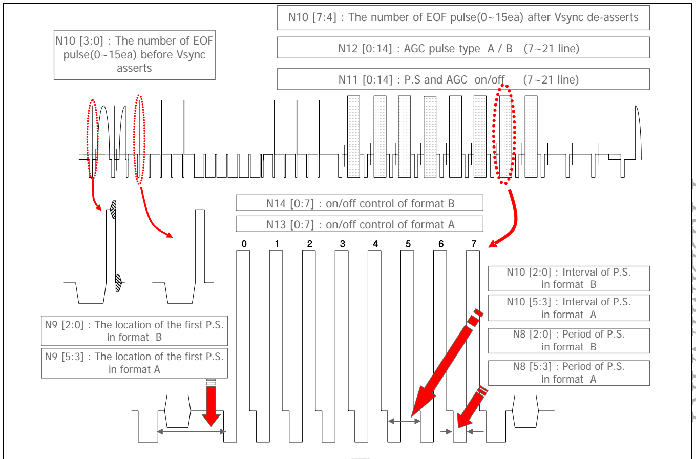
Figure 17-12. Vertical Timing Diagram for pseudo sync and AGC pulse (macrovision control)
