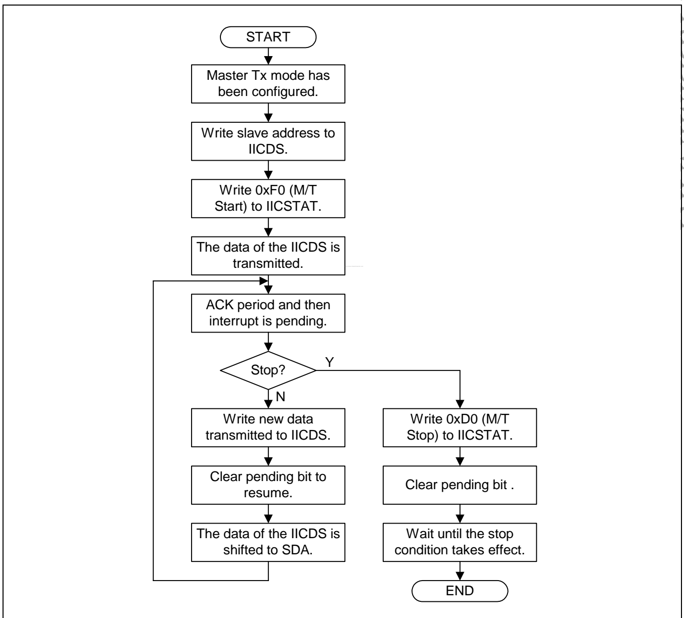
Figure 30-5. Operations for Master/Transmitter Mode
