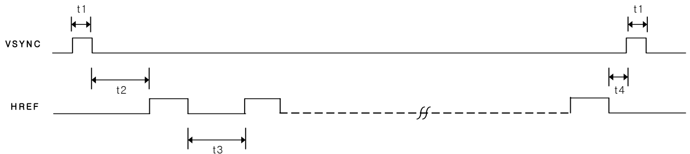
Figure 20-4. Sync signal timing diagram
