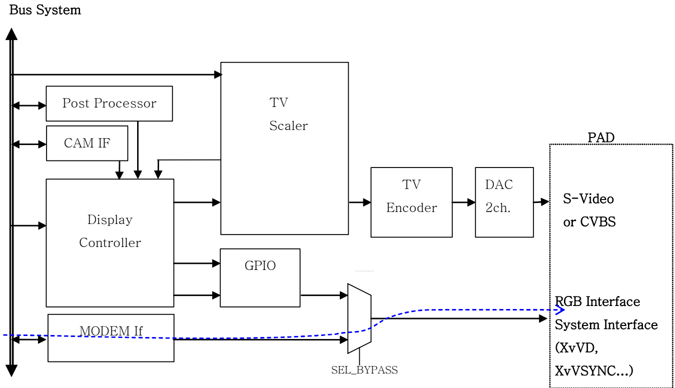
Figure 14-10. By-Pass Mode (Initial LCD Output Pass)
