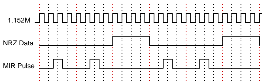
Figure 38-4 Pulse modulation in MIR mode
