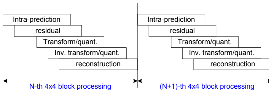
Figure 21.27 H.264 encoding pipeline
