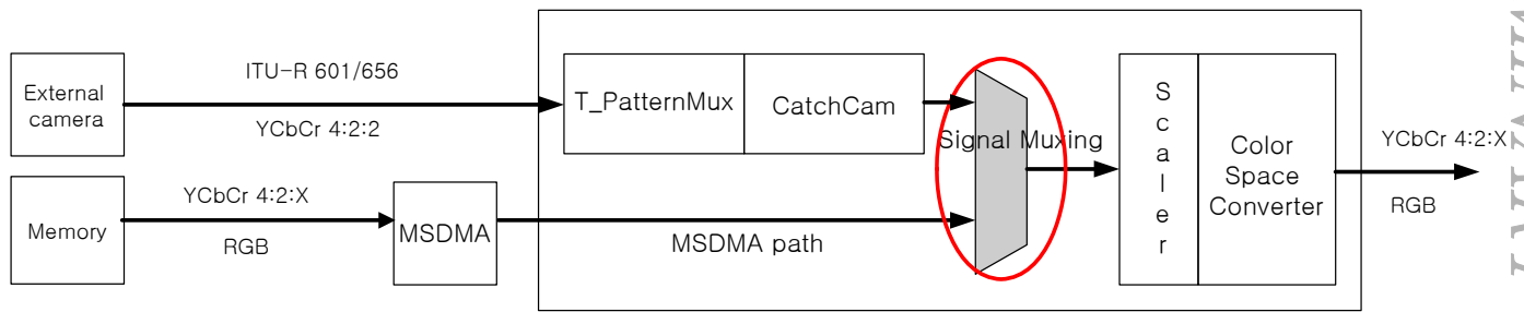
Figure 20-15. MSDMA or External Camera interface
