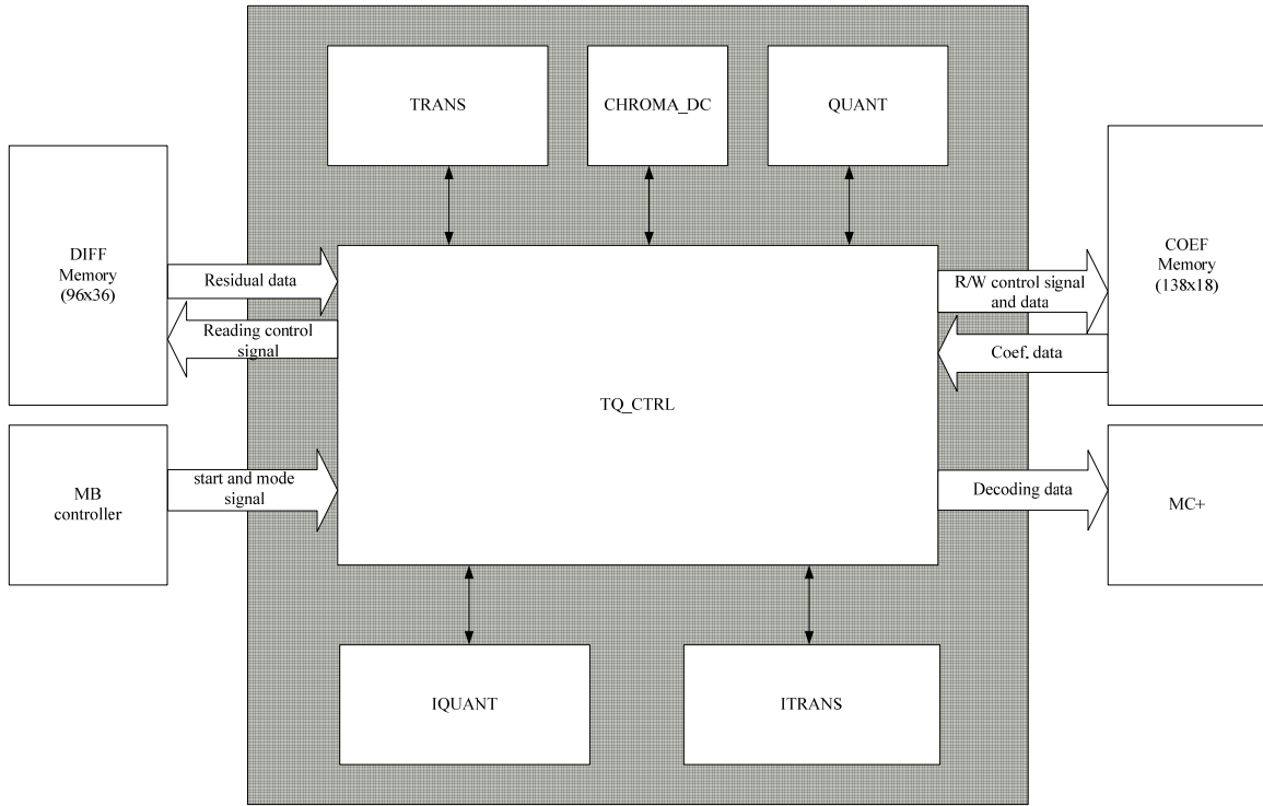
Figure 21.25. H.264 tranform/quantization block diagram
