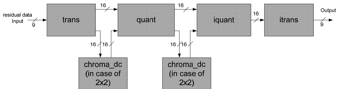
Figure 21.24. H.264 transform/quantization data flow
