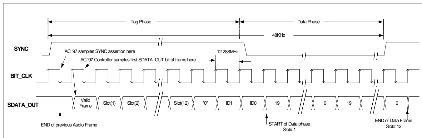
Figure 35-5. AC-link Output Frame
