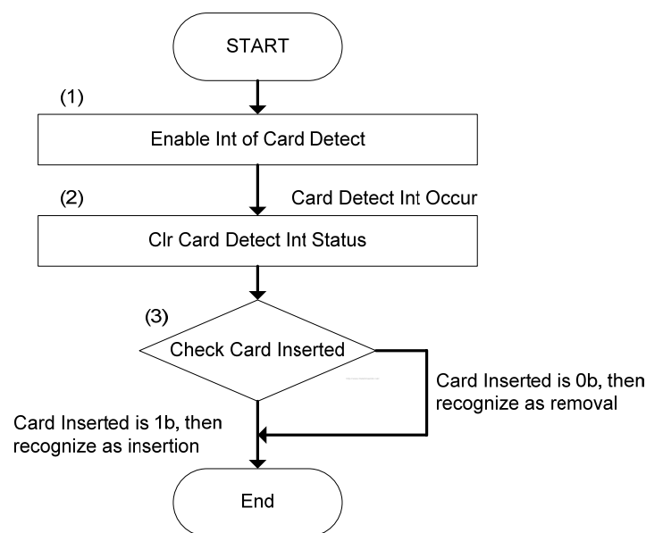
Figure 27-2. SD Card Detect Sequence
