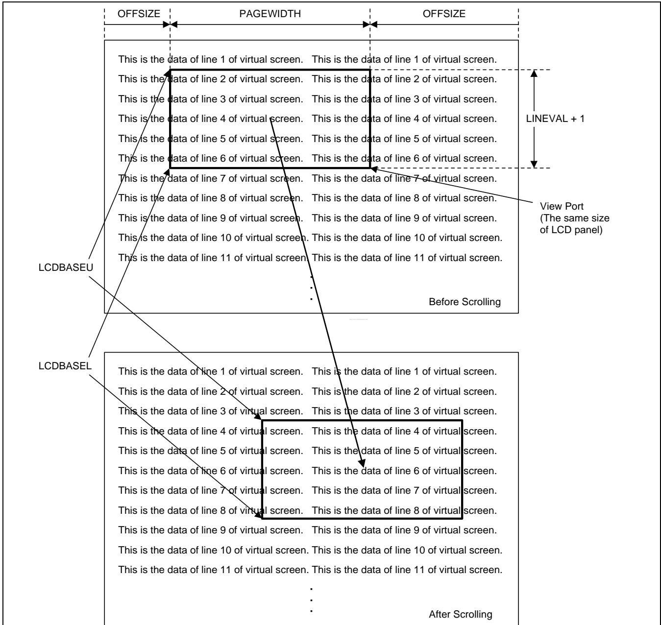
Figure 14-7. Example of Scrolling in Virtual Display
