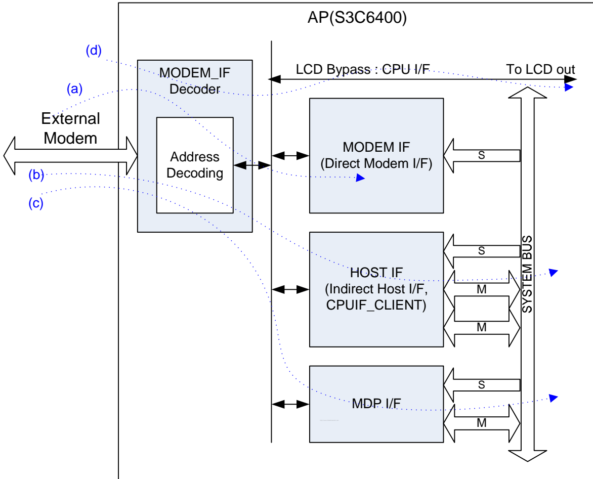
Figure 24-2 Data flow of the the External Host device (MODEM) and the AP
