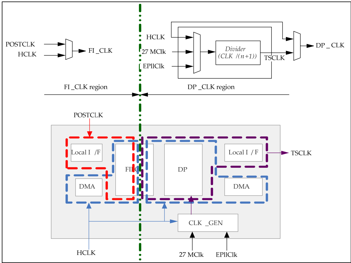
Figure 15-10 Internal clock scheme Block Diagram
