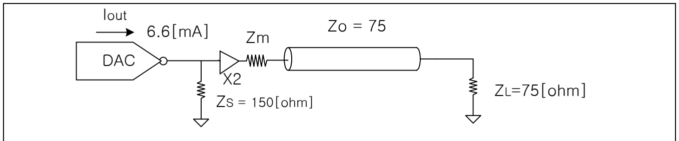
Figure 17-13. DAC Board Guide
