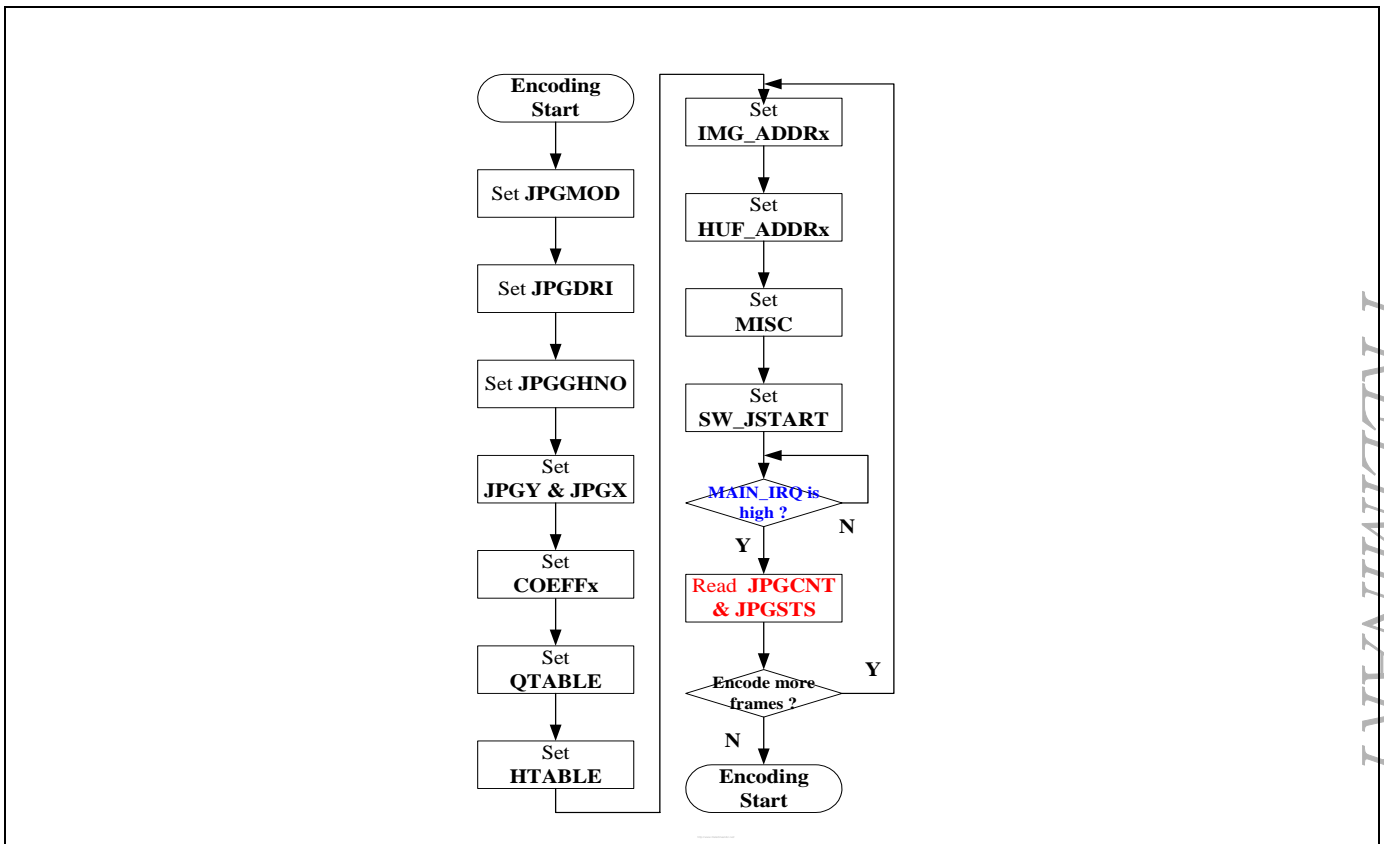
Figure 22-4. Example flow chart of basic encoding
