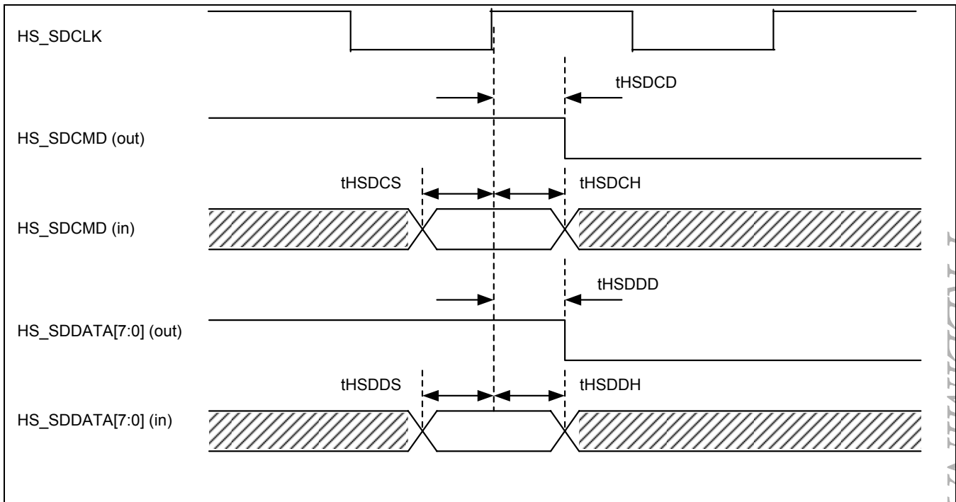
Figure 41-21. High Speed SDMMC Interface Timing
