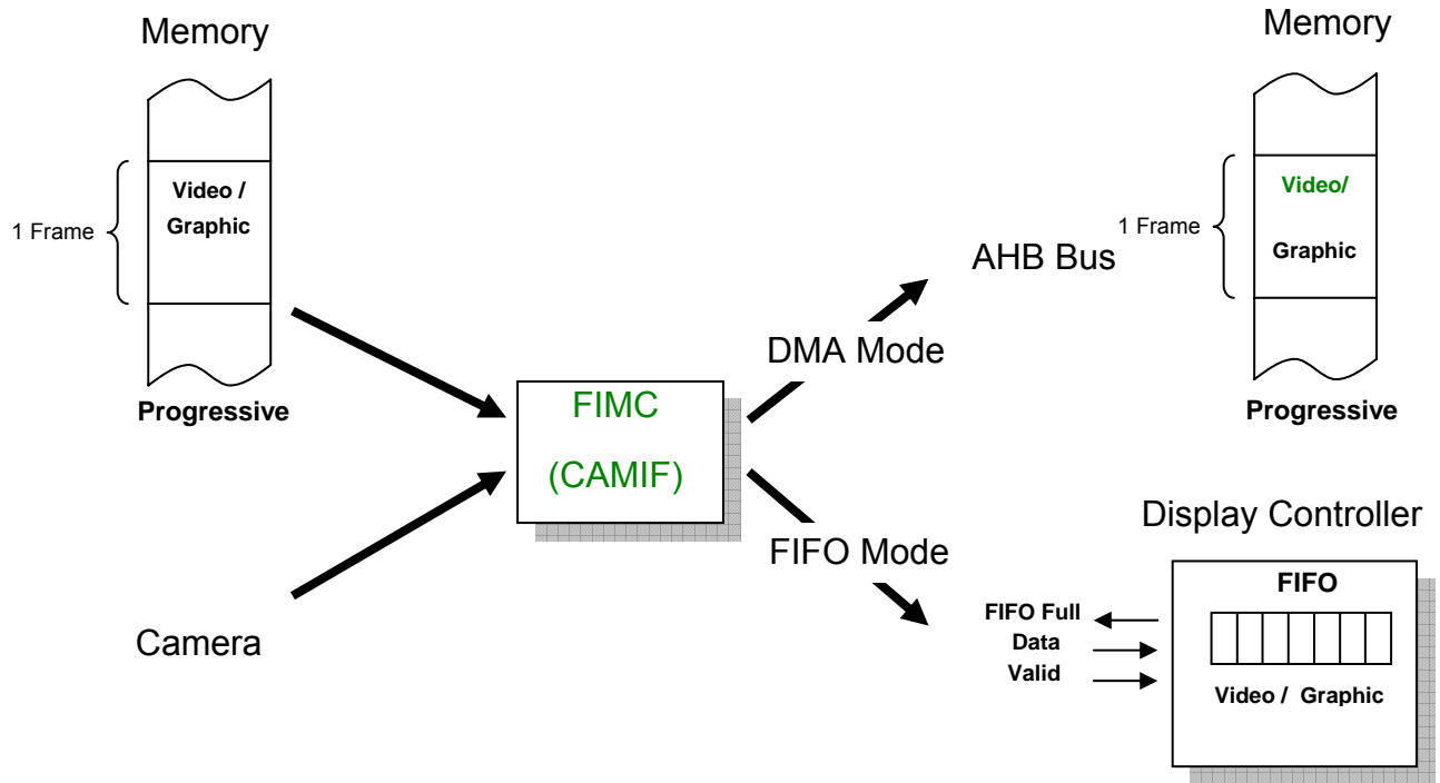
Figure 20-21 . Two input & Two output modes in FIMC
