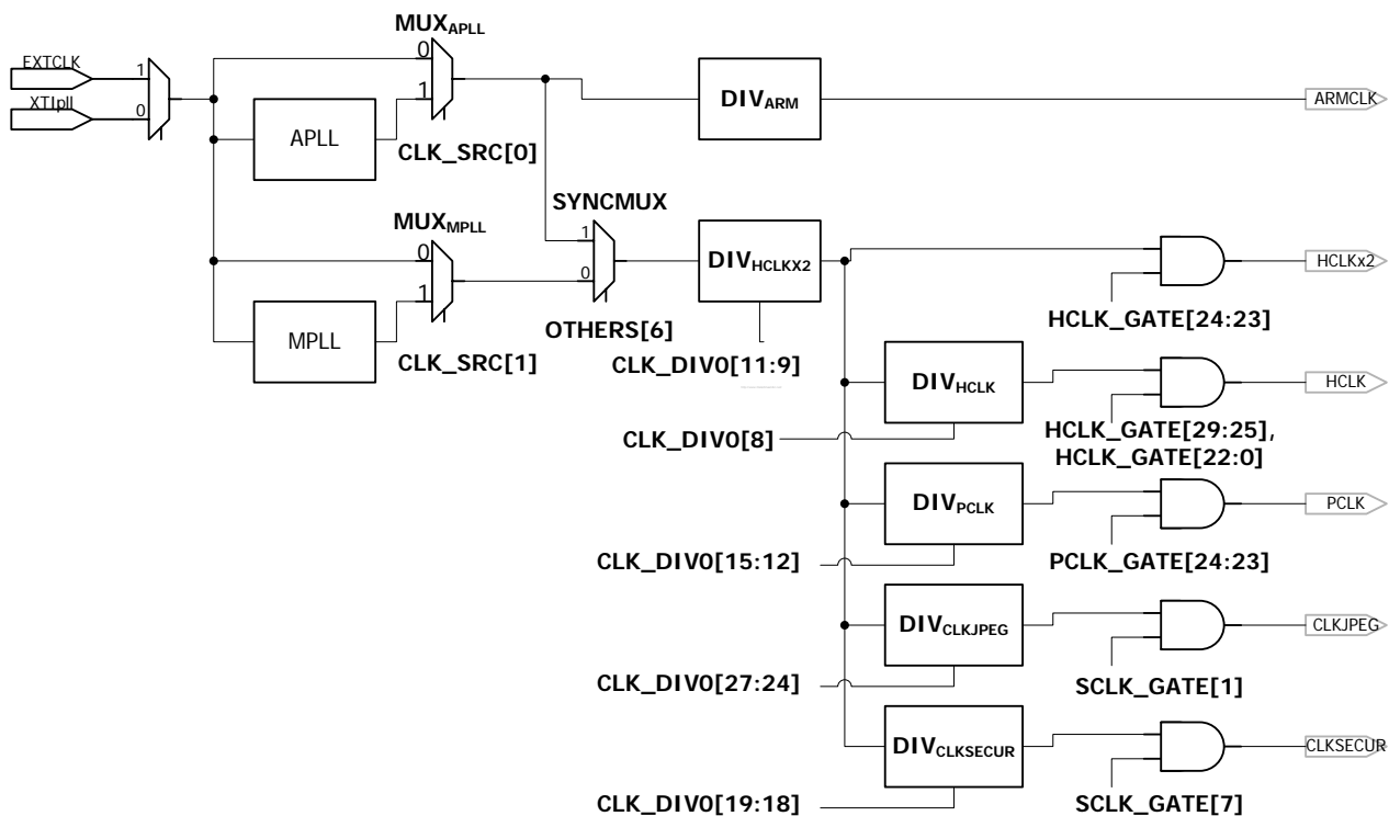
Figure 3-5. ARM and Bus clock generation
