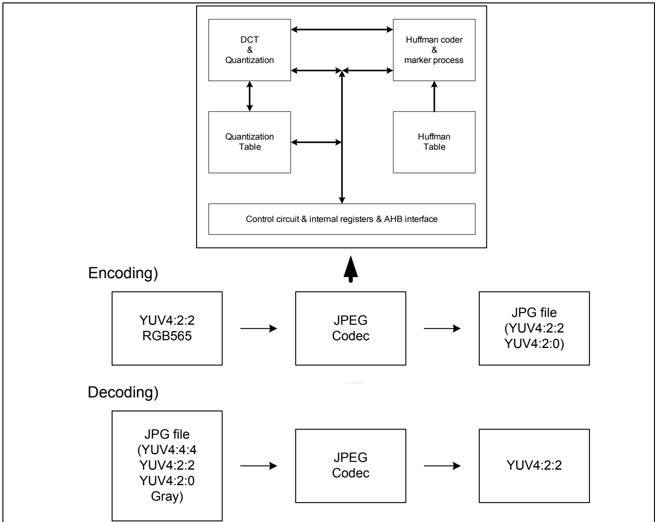
Figure 22-1. JPEG Codec Block Diagram
