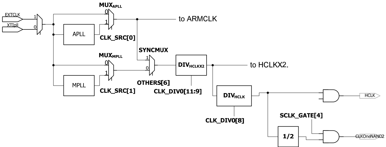
Figure 3-7. OneNAND clock generation
