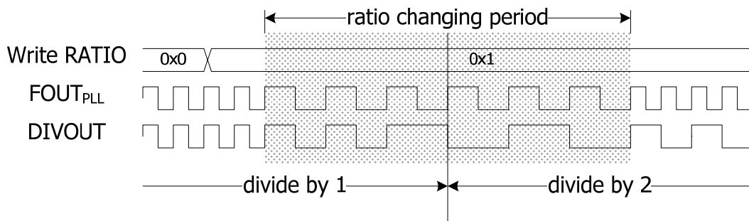
Figure 3-6. Waveform during system clock ratio is changing.
