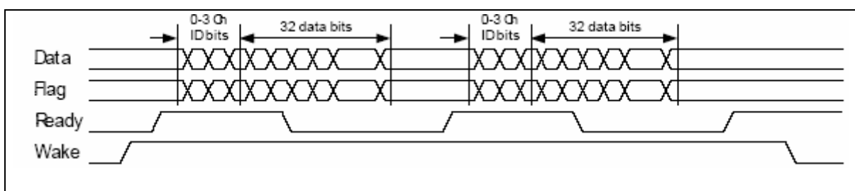
Figure 28-9 Example of Stream mode Block Diagram
