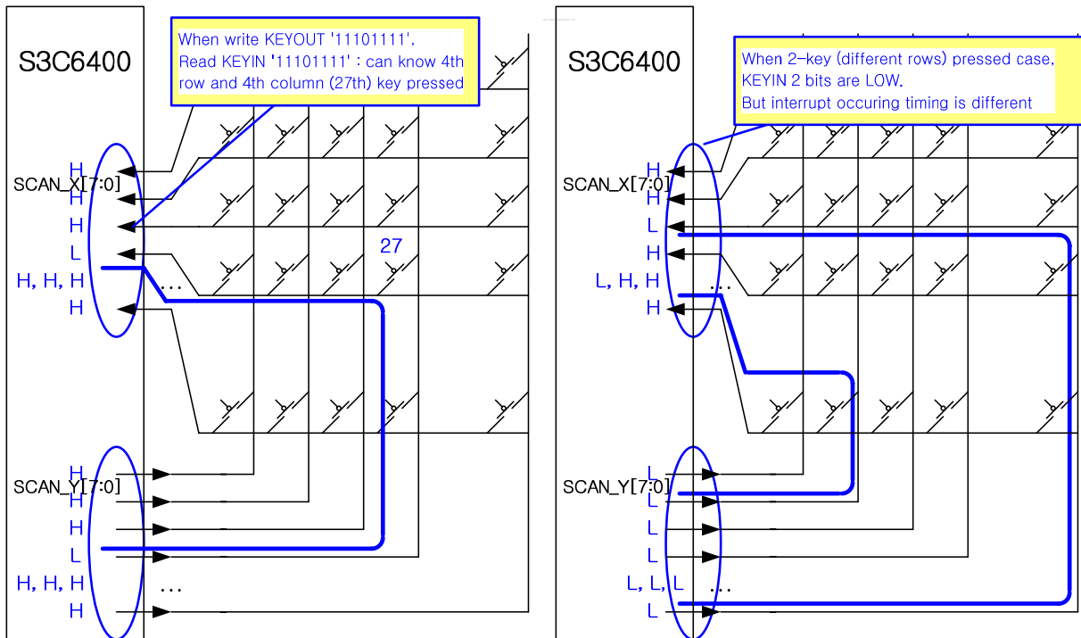
Figure 40-5 Keypad scanning procedure III
