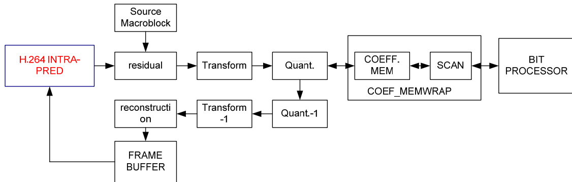
Figure 21.21 (b) H.264 Intra prediction data flow
