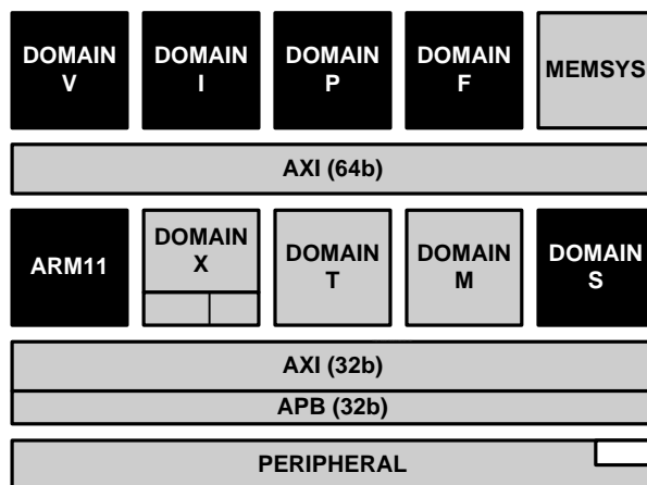
Figure 3-16. Power domains at DEEP-STOP mode (ARM11 is OFF and lost internal state)
