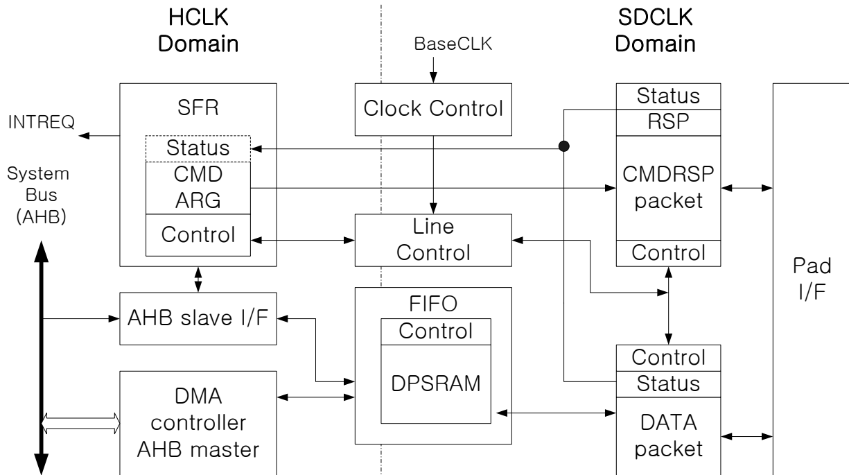
Figure 27-1. HSMC block diagram
