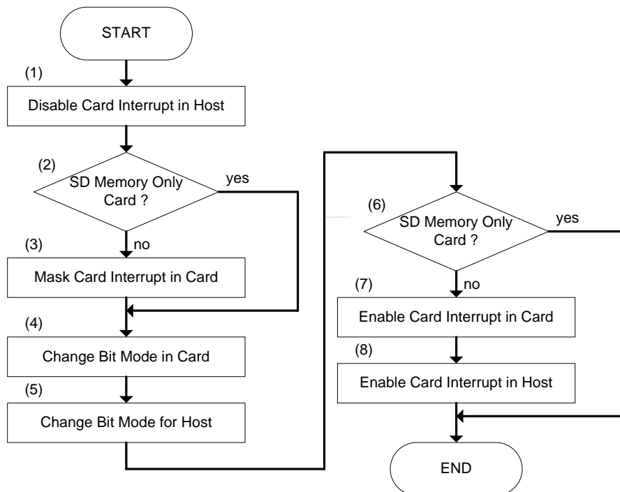
Figure 27-7. Change Bus Width Sequence
