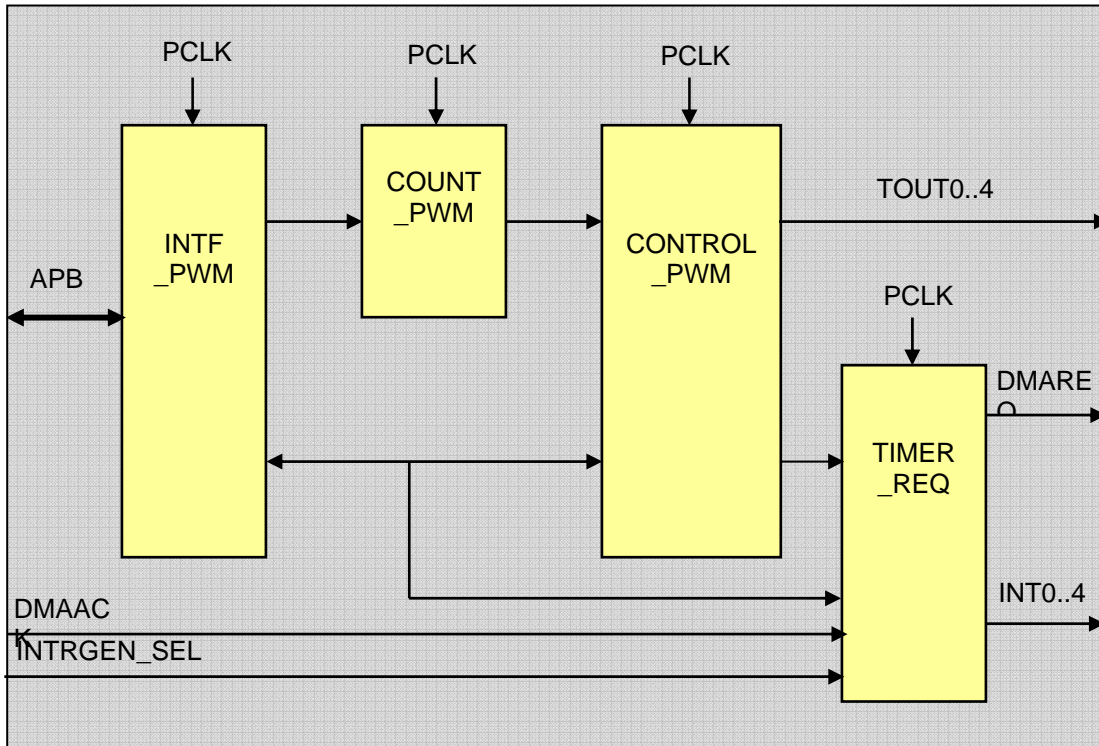
Figure 32-2: PWMTIMER Block Diagram
