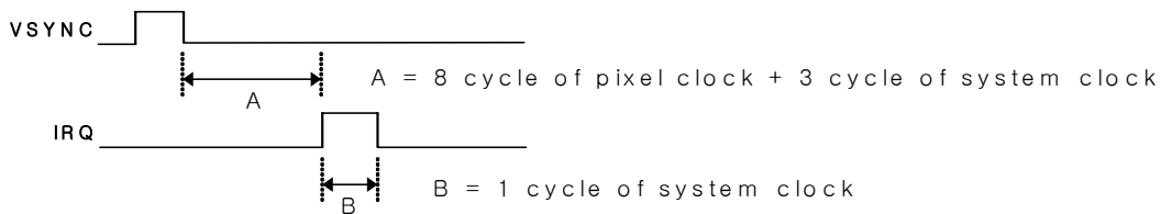
Figure 20-13. VSYNC & IRQ signals timing requirement
