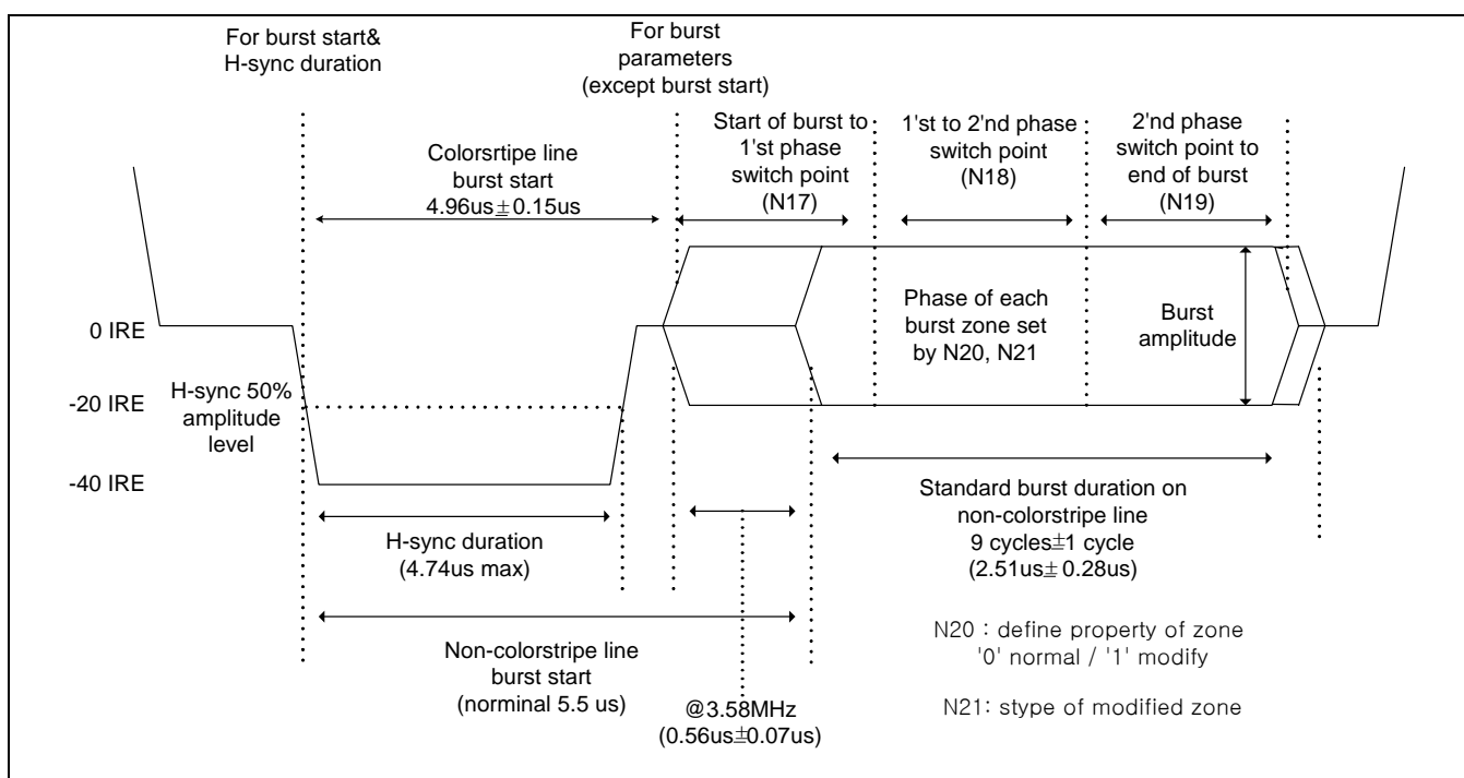
Figure 17-11. Horizontal Timing Diagram for color stripe (macrovision control)
