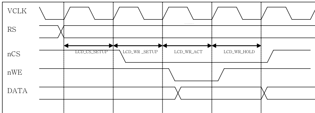
Figure 14-9. I80 CPU system interface WRITE Cycle Timing
