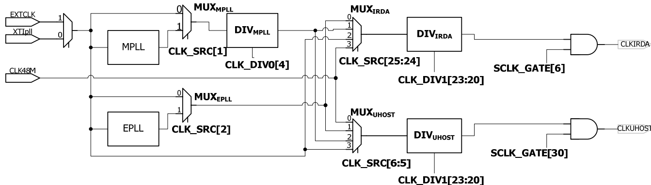
Figure 3-13. IrDA/USB host clock generation
