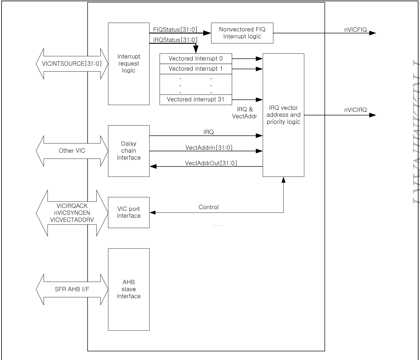
Figure 12-2 Vectored Interrupt Controller block diagram
