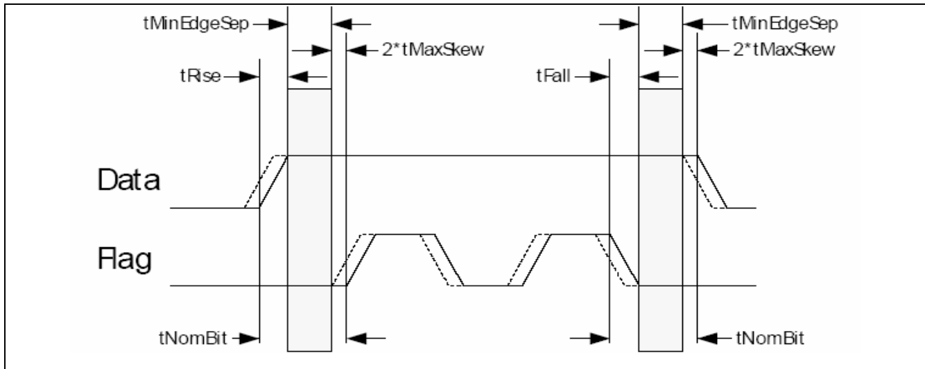
Figure 41-23. MIPI HSI Timing Diagram
