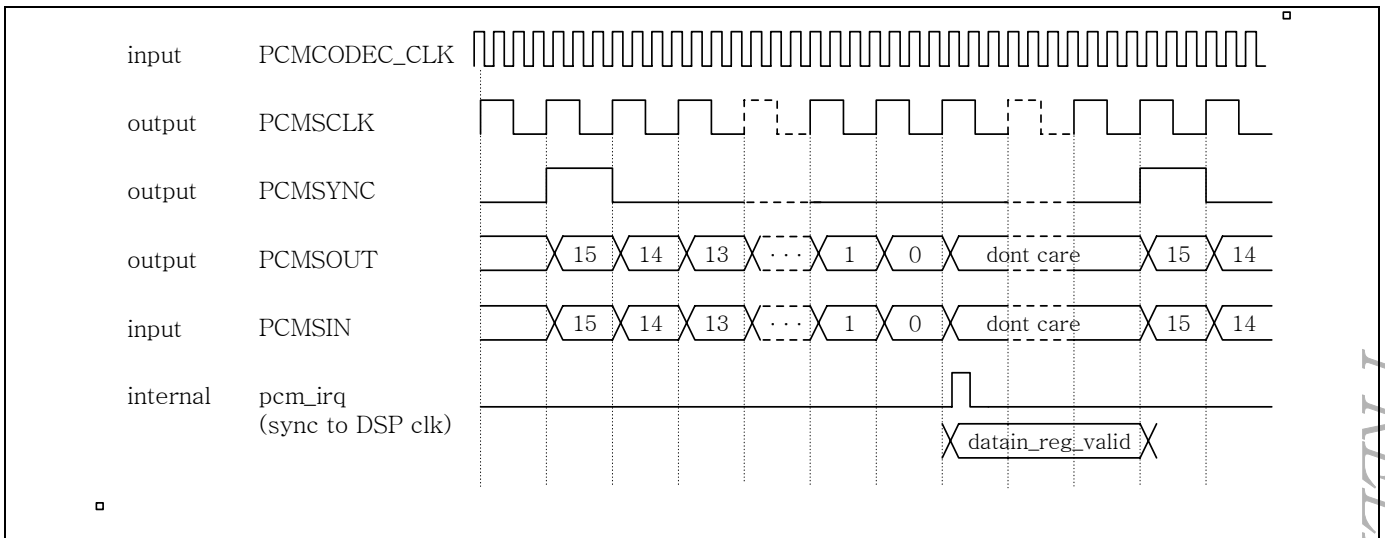
Figure 37-1 PCM timing, POS_MSB_WR/RD = 0
