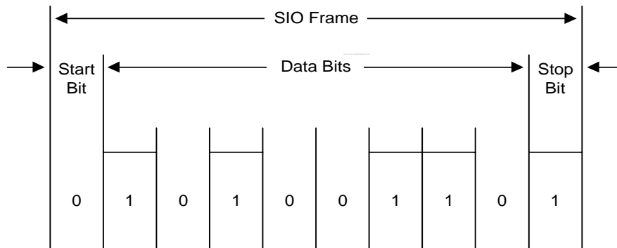
Figure 31-5 Serial I/O Frame Timing Diagram (Normal UART)
