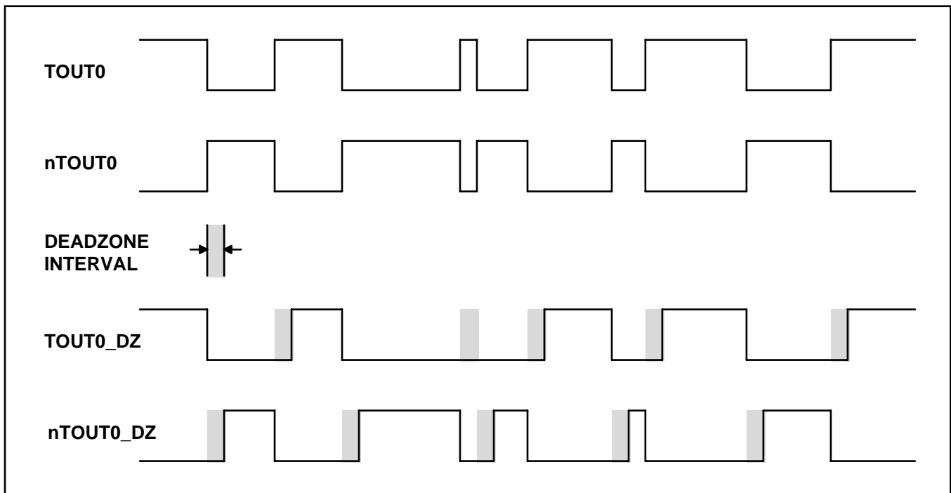
Figure 32-10: The waveform when a deadzone feature is enabled.
