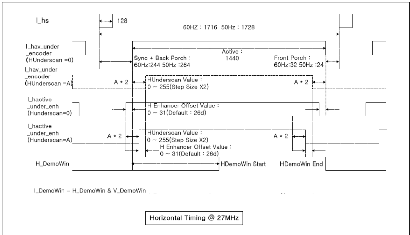
Figure 17-7. Requested Horizontal Timing Diagram
