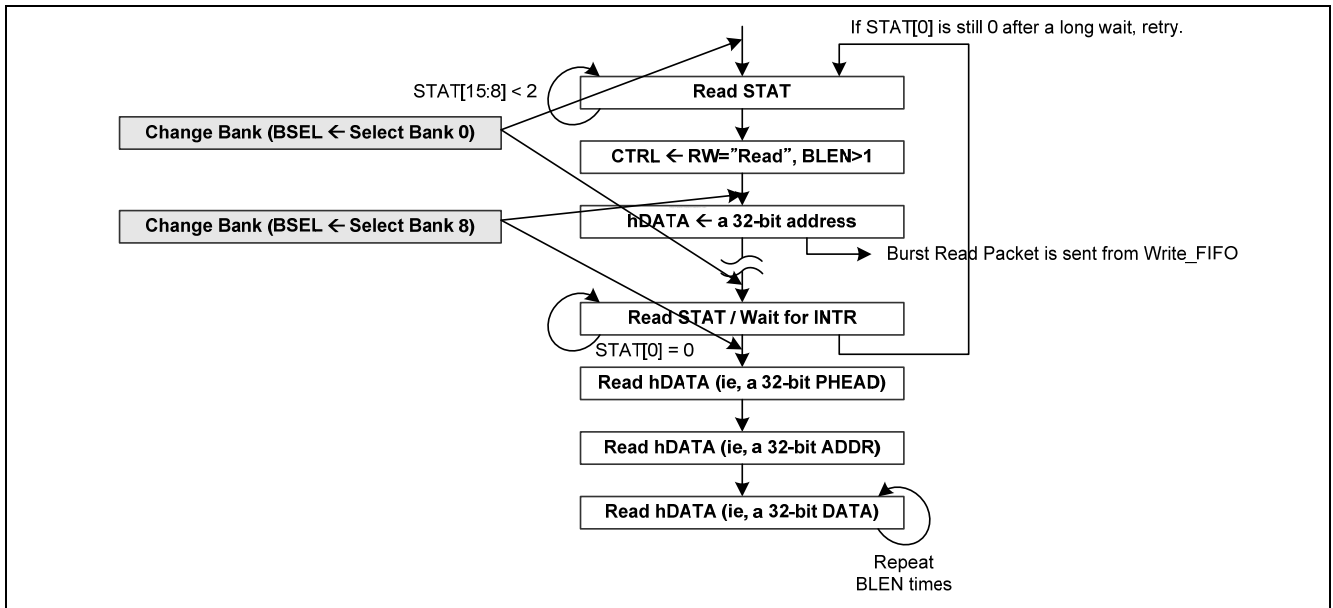
Figure 24-7. Burst Read Procedure
