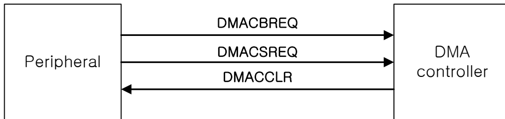
Figure 11-2. Peripheral-to-memory transaction comprising bursts and single requests
