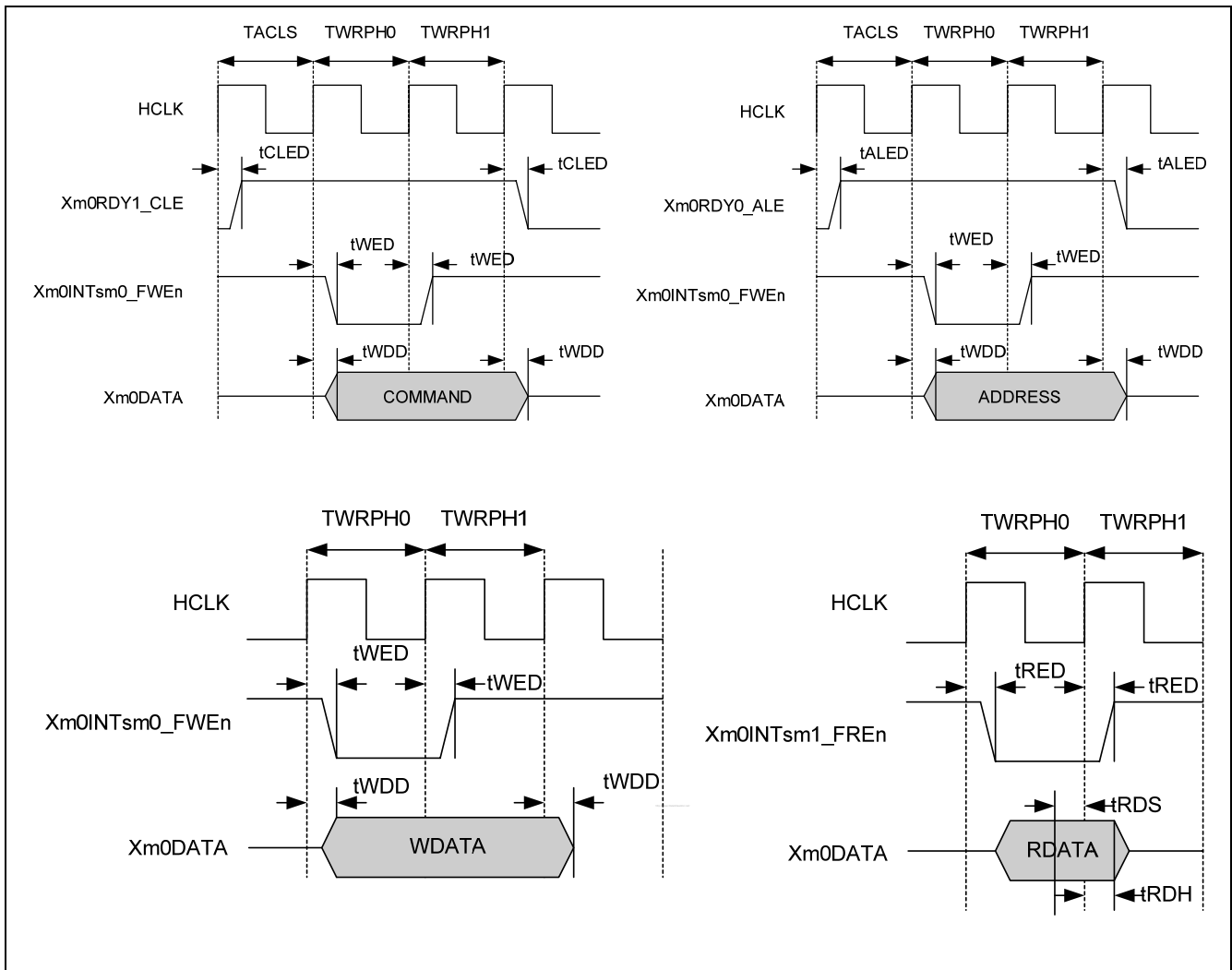
Figure 41-9. Nand Flash Timing
