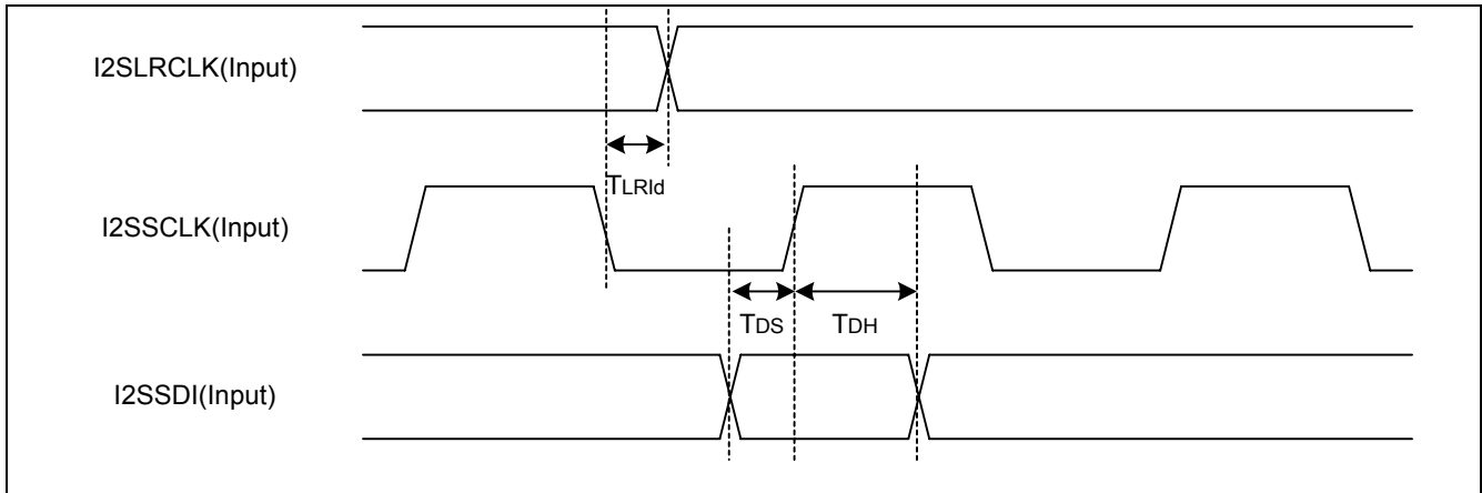
Figure 41-25. IIS Interface Timing (Slave / RX)
