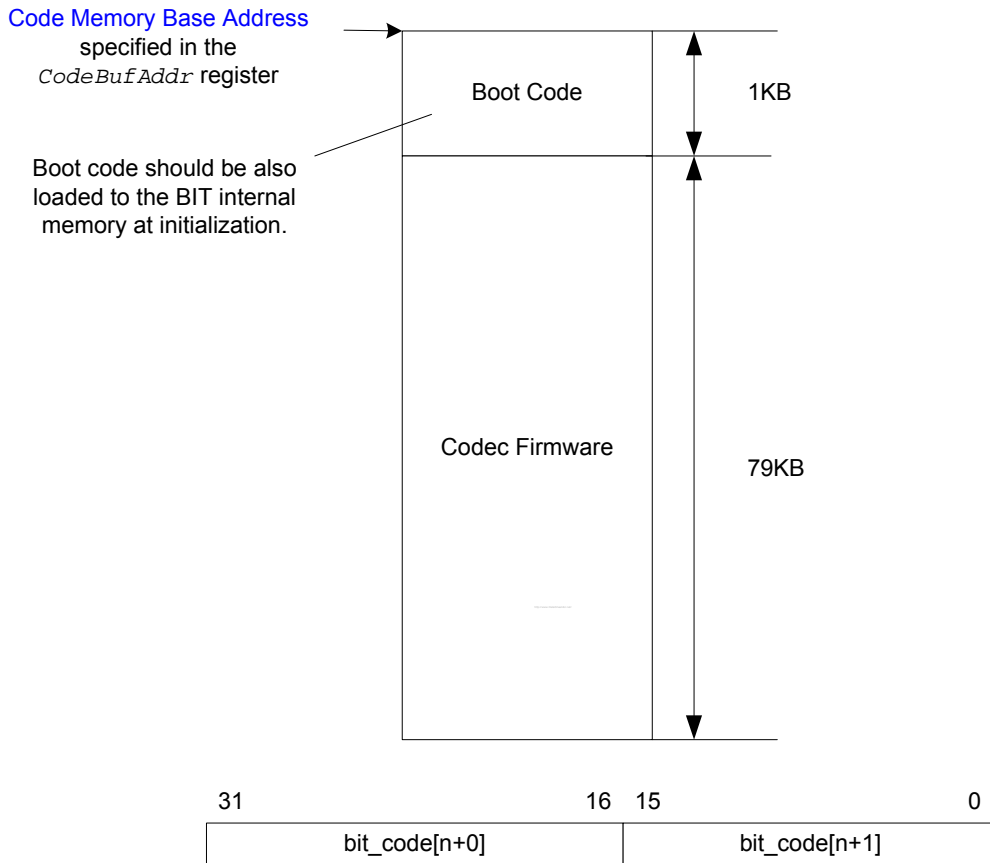
Figure 21.4 Memory space for the BIT firmware
