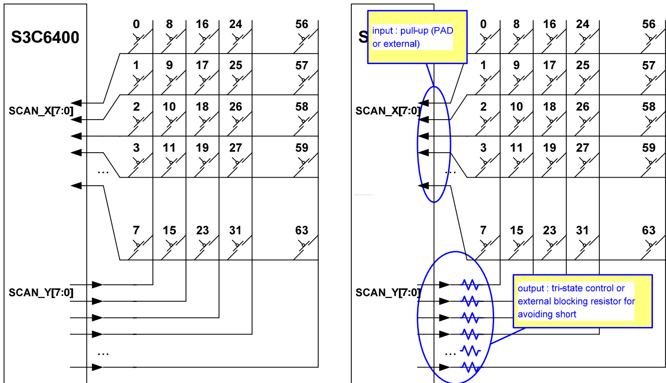
Figure 40-3 Keypad scanning procedure I
