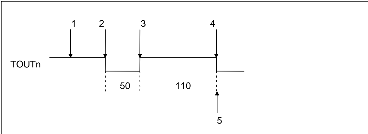
Figure 32-1: Simple Example of PWM Cycle Block Diagram
