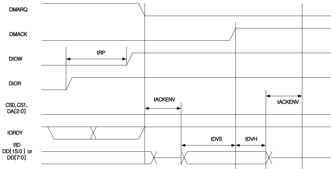
Figure 9-7: UDMA - In Operation (terminated by host)
