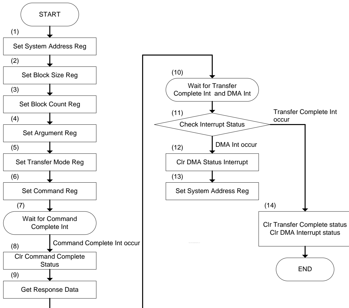
Figure 27-12. Transaction Control with Data Transfer Using DAT Line Sequence (Using DMA)
