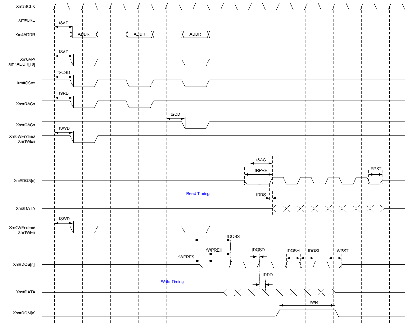
Figure 41-11. DDR SDRAM READ / WRITE Timing ( T_{rp} = 2 , T_{rcd} = 2 , T_{cl} = 2 , DW = 16-bit)
