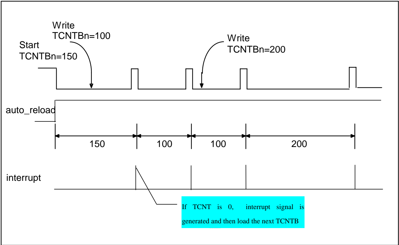
Figure 32-6: Example of Double Buffering Feature Block Diagram
