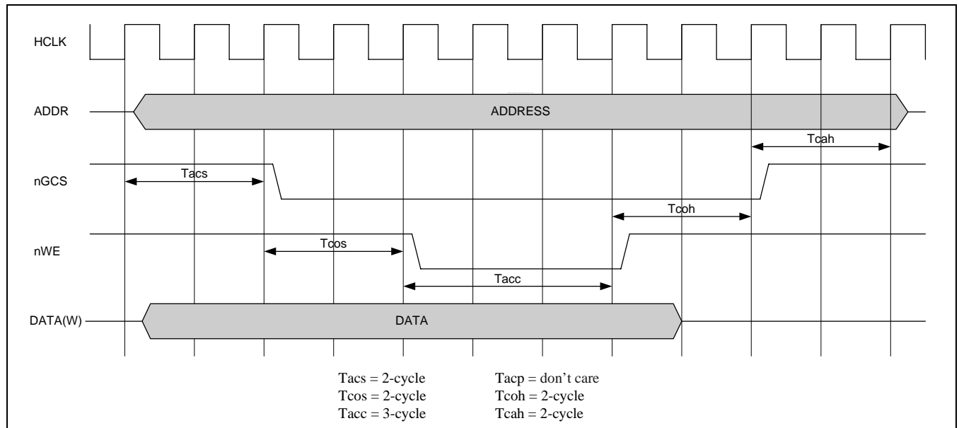
Figure 6-4 SROM Controller Write Timing Block Diagram
