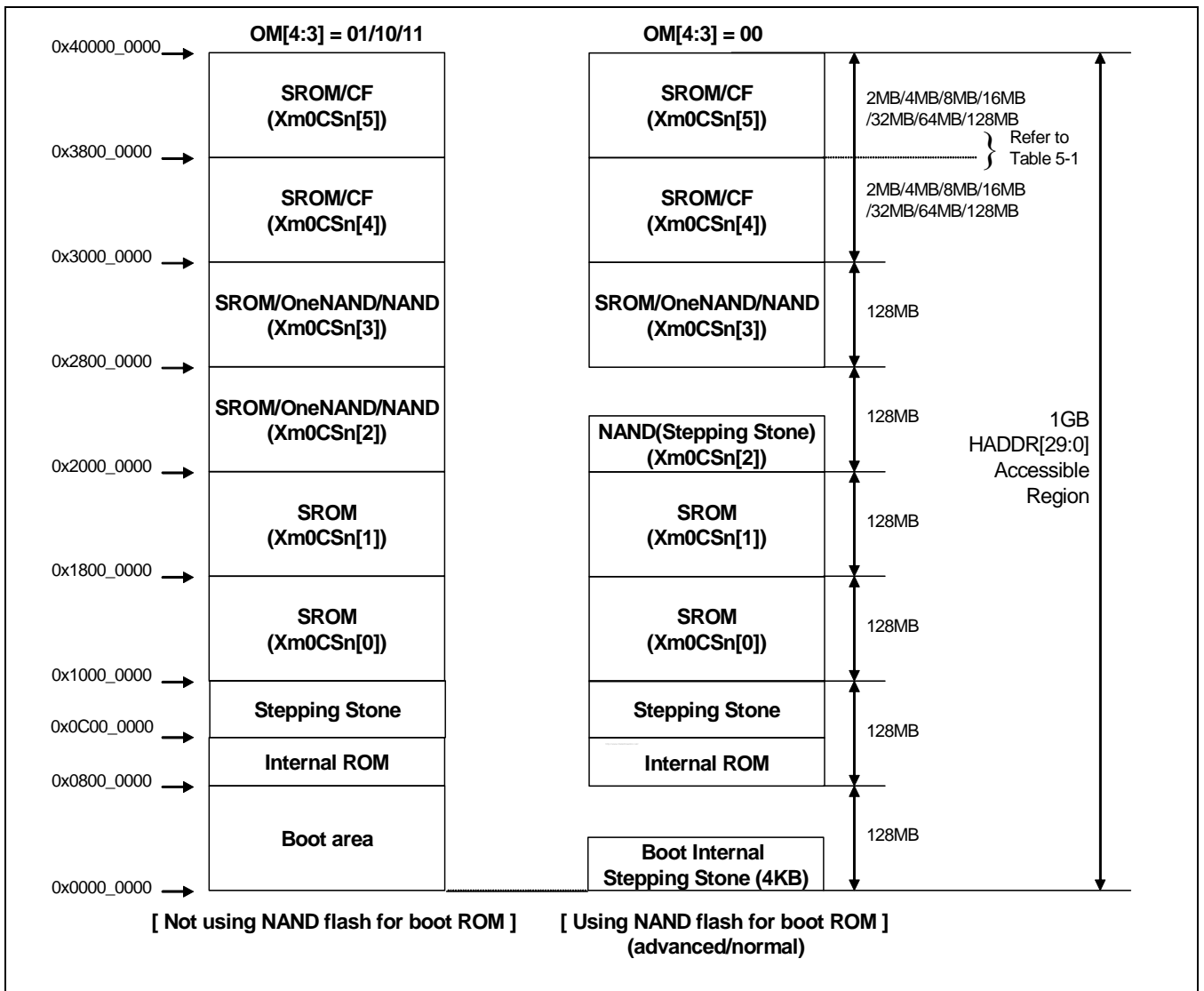
Figure 8-5. NAND Flash Memory Mapping Block Diagram
