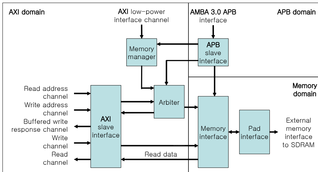
Figure 5-1 DRAM Controller Block Diagram
