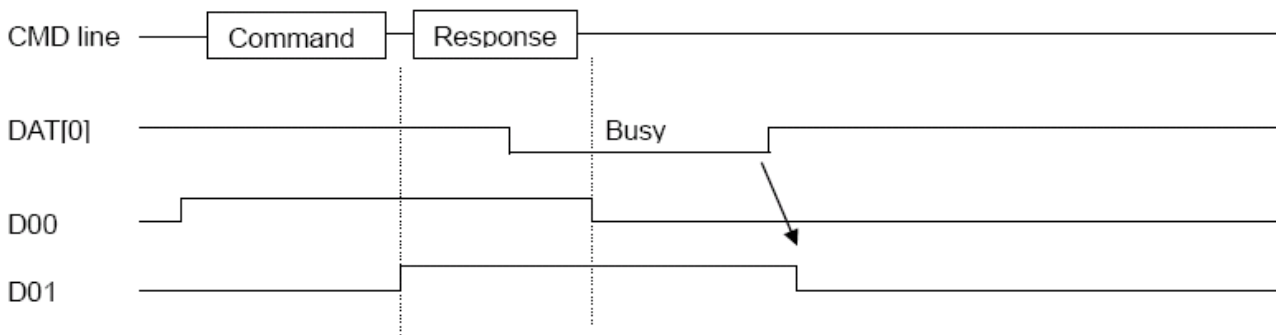
Figure 27-4. Timing of Command Inhibit (DAT) for the case of response with busy
