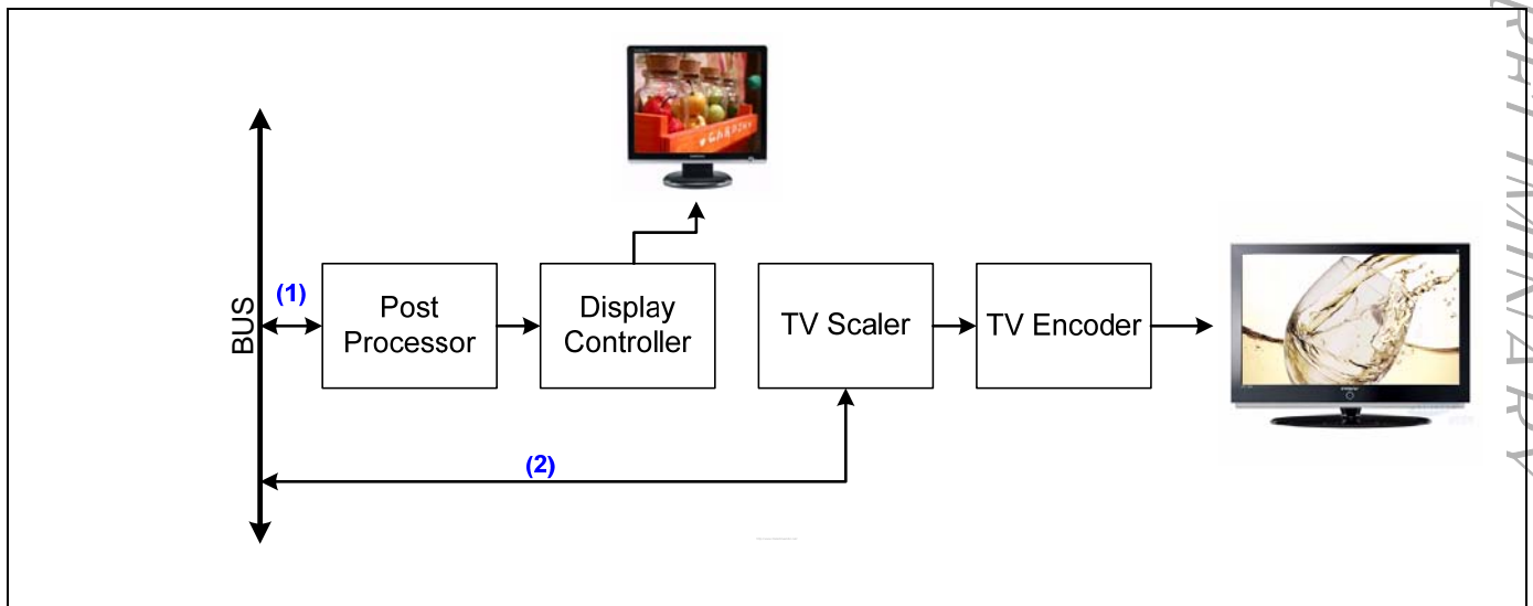
Figure 17-2. TV Encoder Data Path Concept
