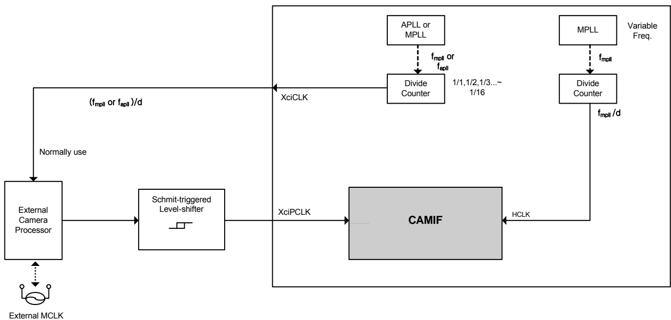
Figure 20-7. CAMERA INTERFACE clock generation
