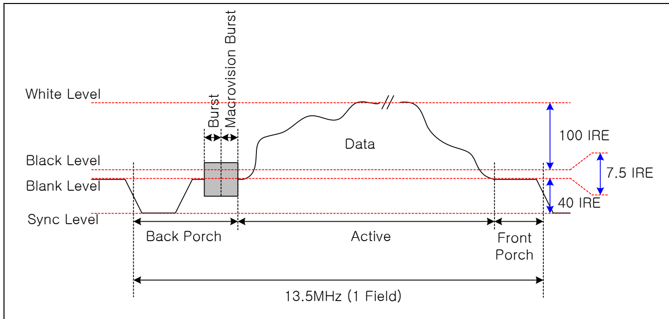
Figure 17-3. Composition of Analog Composite Signal
