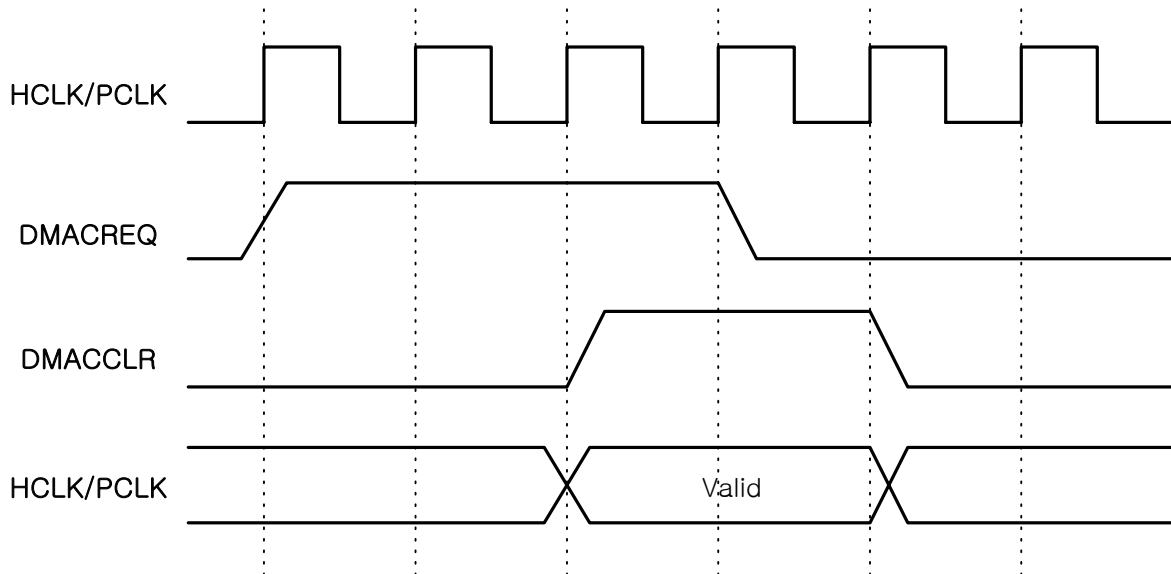
Figure 11-6. DMA interface timing
