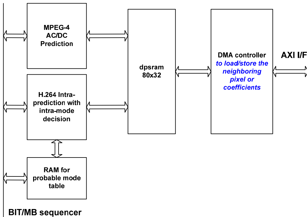
Figure 21.22. Intra-prediction block diagram
