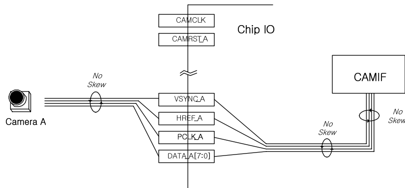
Figure 20-5. IO connection guide
