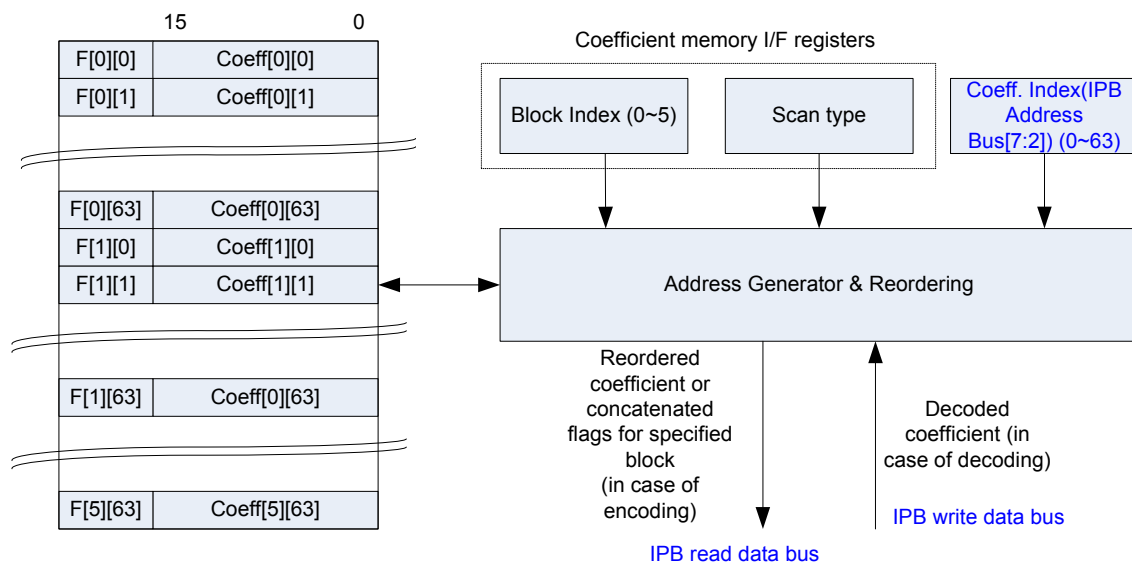
Figure 21.36 Coefficient memory access
