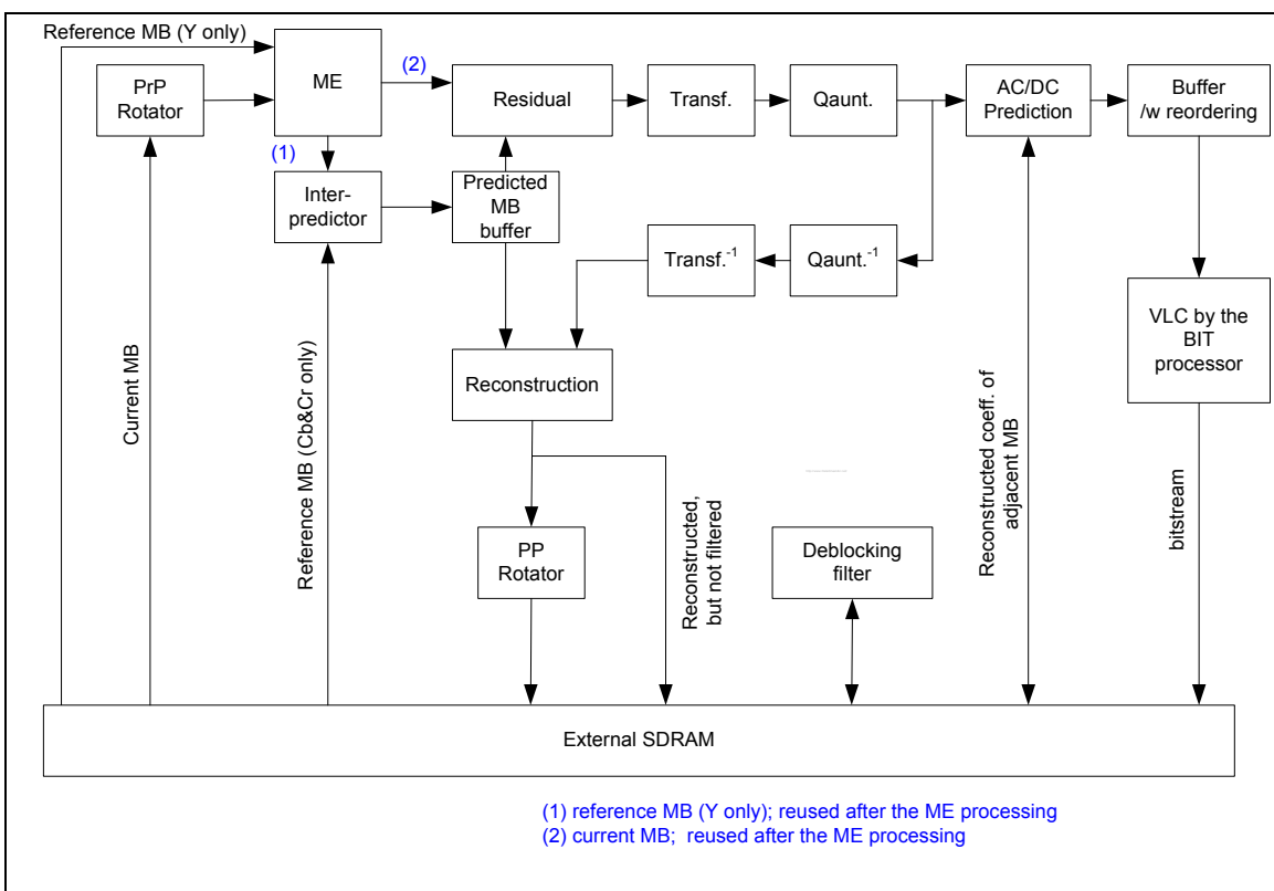
Figure 21.7 MPEG-4 encoder data flow
