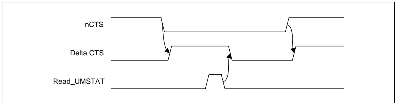
Figure 31-8 nCTS and Delta CTS Timing Diagram
