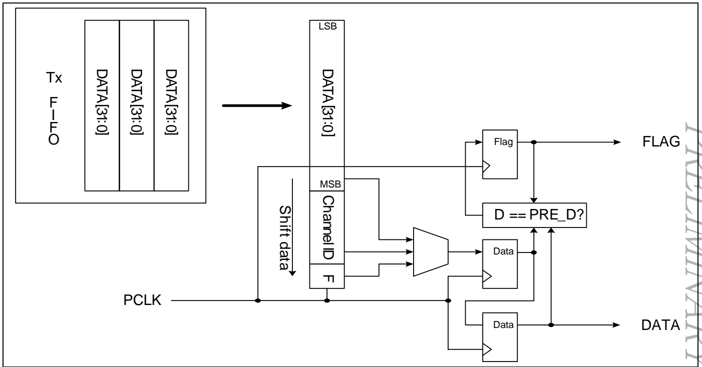
Figure 28-5 Parallel -to- Serial block (Tx module Part)
