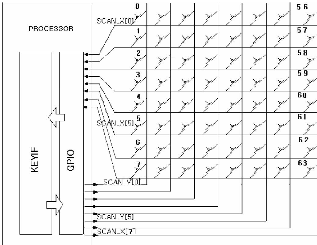
Figure 40-1 Key Matrix Interface External Connection Guide
