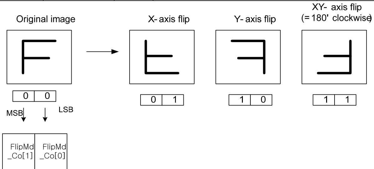
Figure 20-18. Codec image mirror
