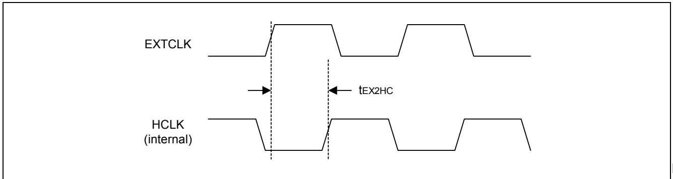
Figure 41-3. EXTCLK/HCLK in case that EXTCLK is used without the PLL
