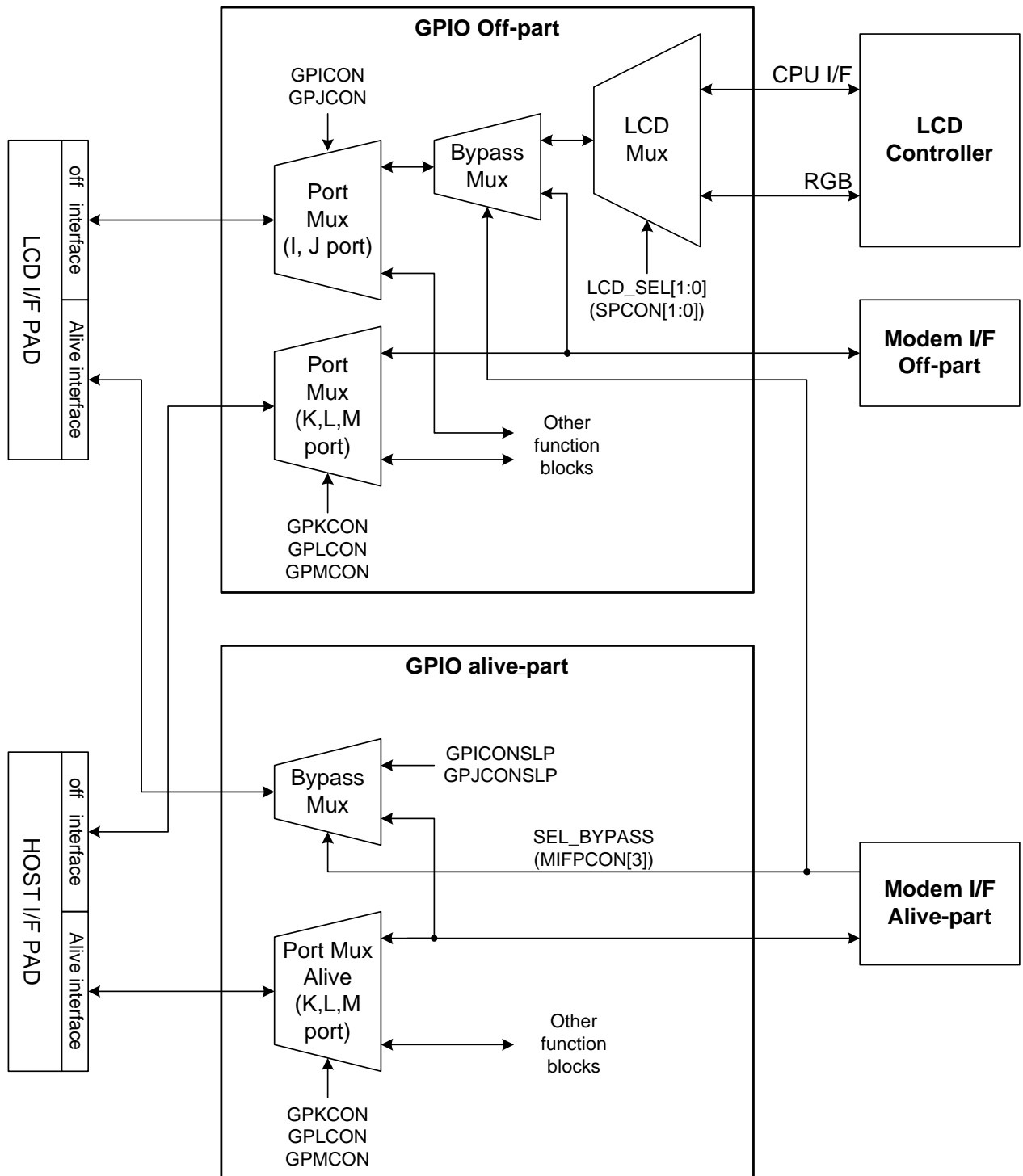
Figure 10- 3 Diagram of LCD bypass logic
