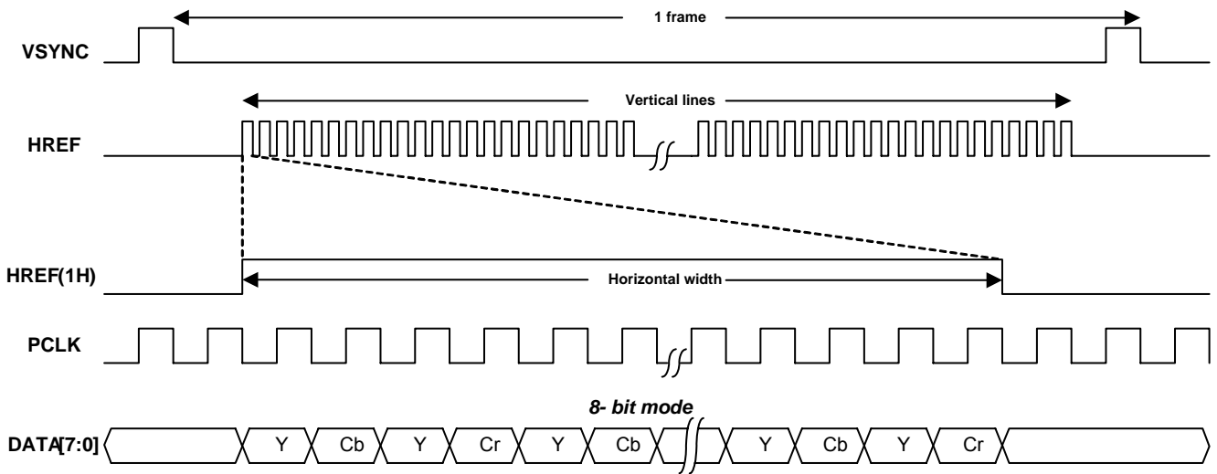
Figure 20-2. ITU-R BT 601 Input timing diagram
