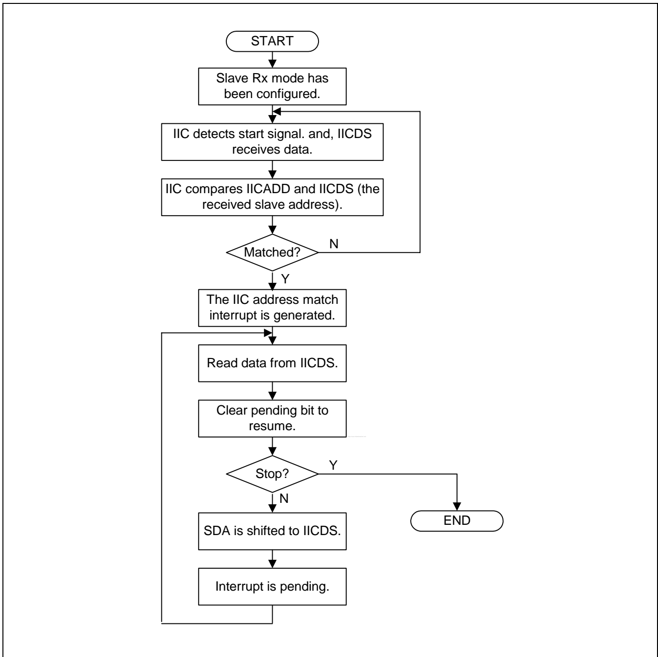
Figure 30-8. Operations for Slave/Receiver Mode
