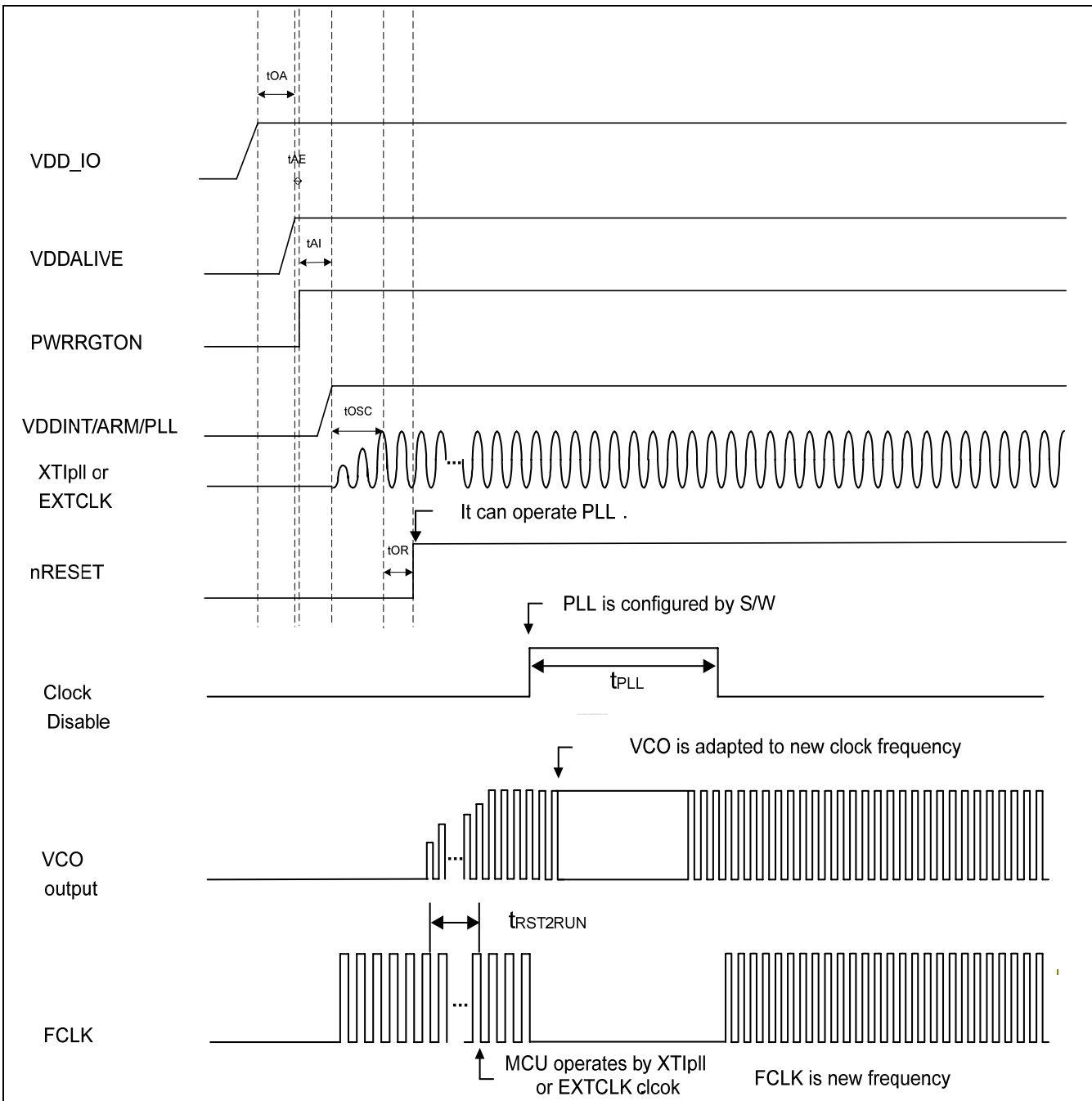
Figure 41-5. Power-On Oscillation Setting Timing
