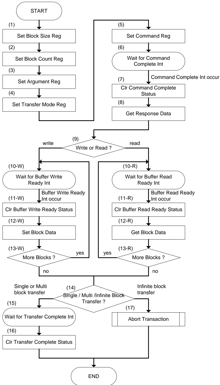
Figure 27-11. Transaction Control with Data Transfer Using DAT Line Sequence (Not using DMA)
