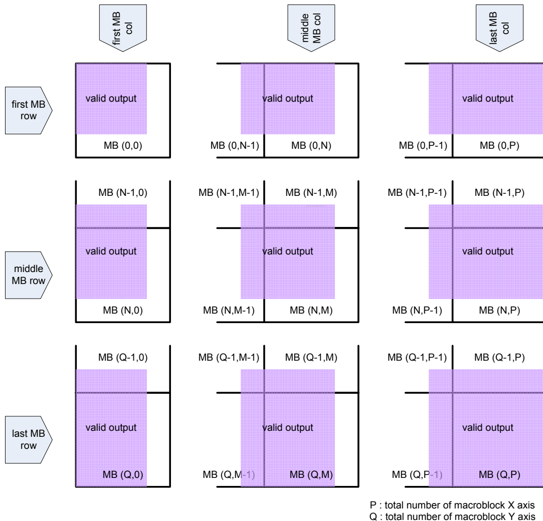
Figure 21.31 valid output data of deblocking filter in H.264 mode
