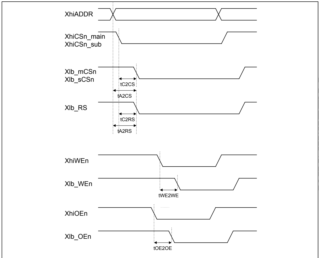
Figure 41-16. LCD Bypass Control signal timing diagram
