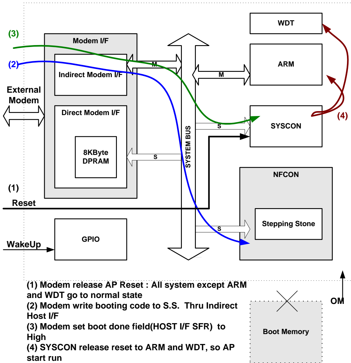
Figure 24-10. Modem Boot procedure
