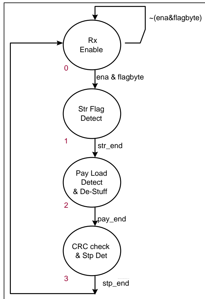
Figure 38-6 MIR demodulation process
