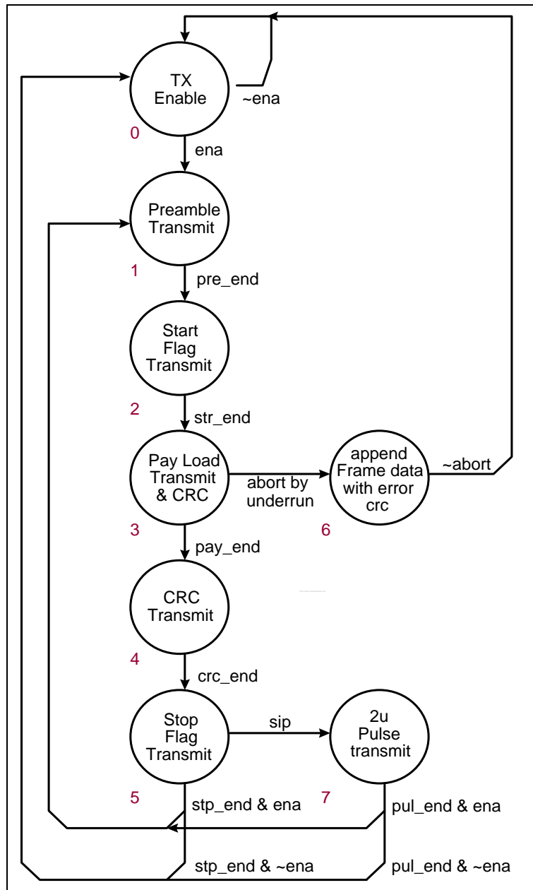
Figure 38-2 FIR modulation process
