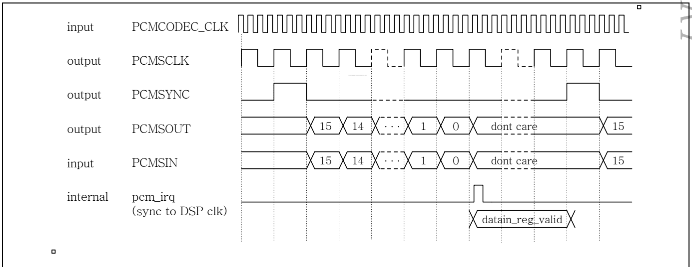
Figure 37-2 PCM timing, POS_MSB_WR/RD = 1
