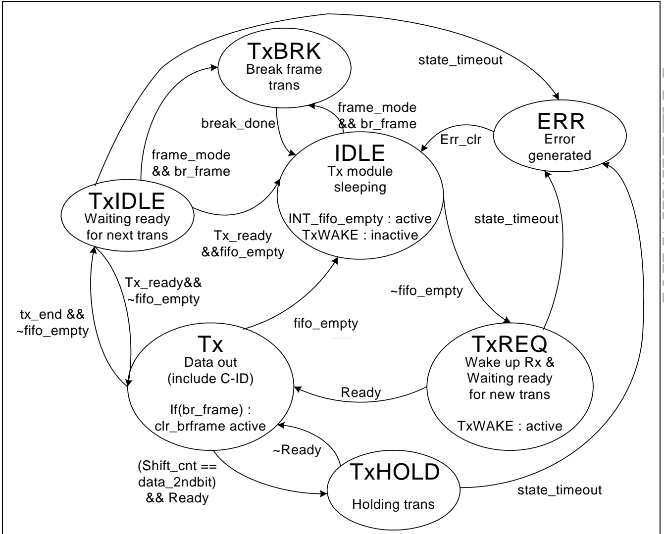
Figure 28-12 FSM of Tx module Part Block Diagram
