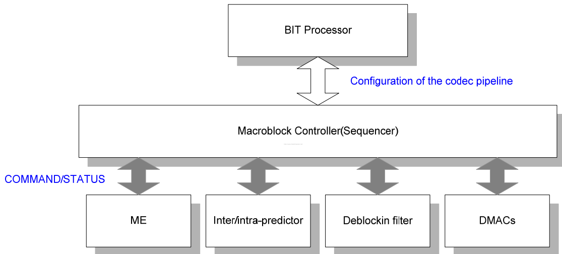
Figure 21.40. Macroblock controller connectivity
