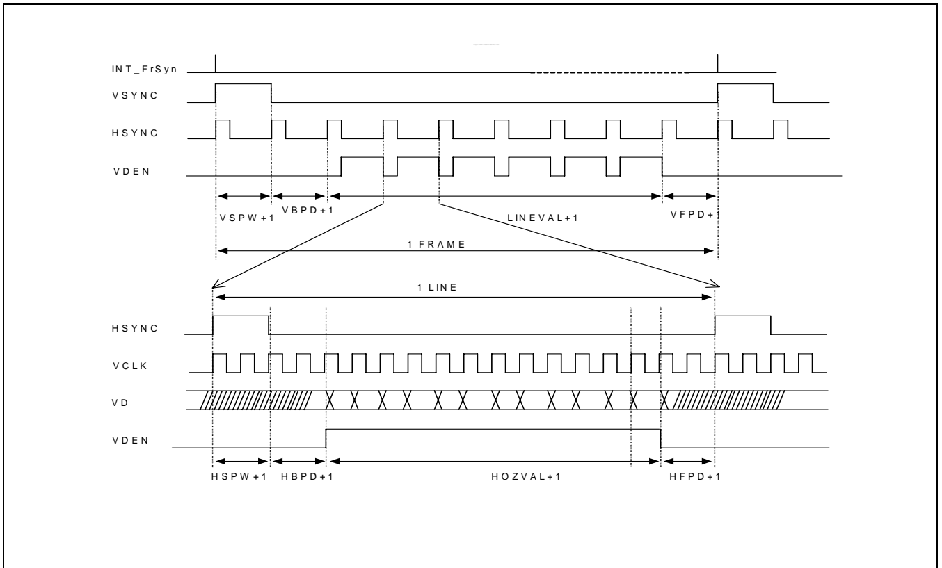
Figure 14-8. LCD RGB interface Timing
