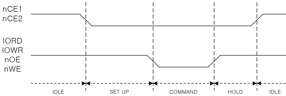
Figure 9-4: PC Card State Definition
