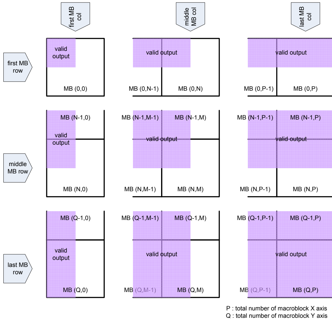
Figure 21.34 valid output data of VC-1 deblocking filter
