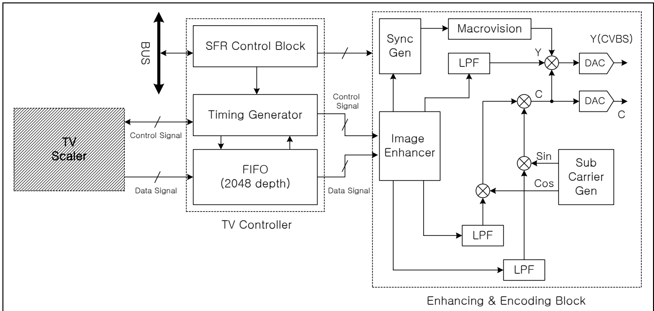
Figure 17-1. TV Encoder Block Diagram
