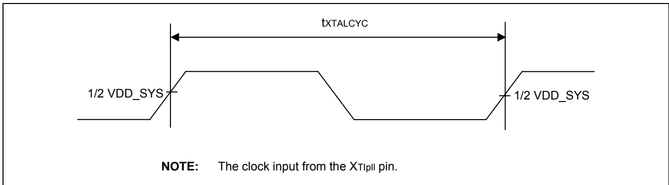
Figure 41-1. XT1pll Clock Timing
