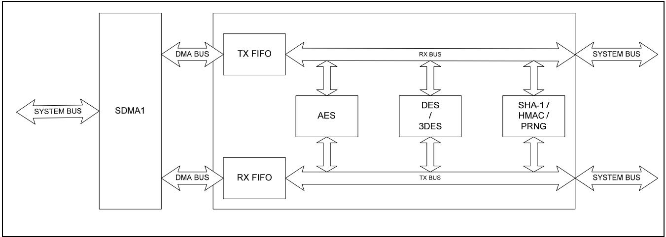
Figure 13-1, Block Diagram of the Security Sub-System
