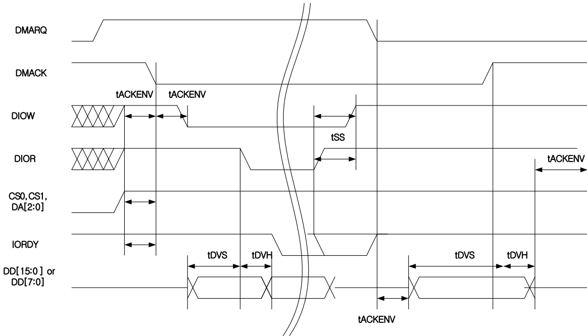
Figure 9-8: UDMA - Out Operation (terminated by device)
