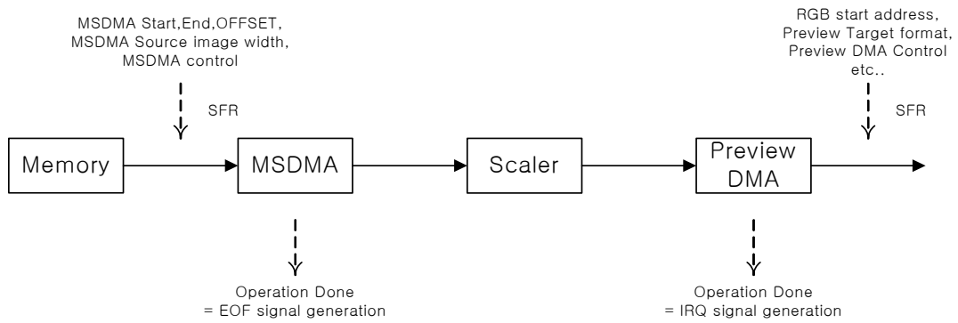
Figure 20-25. SFR & Operation (related each DMA when selected MSDMA input path)
