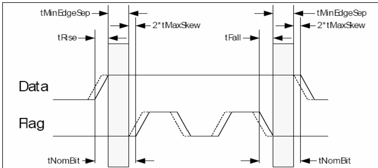
Figure 28-7 Waveform Block Diagram
