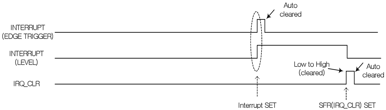
Figure 20-17. Interrupt generation scheme
