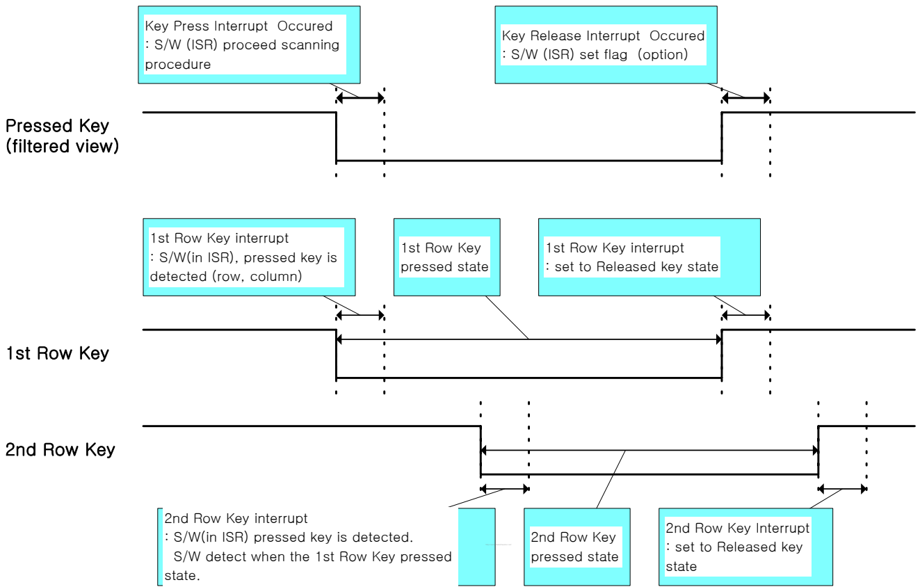
Figure 40-6 Keypad Scanning Procedure when the two-key pressed with different row
