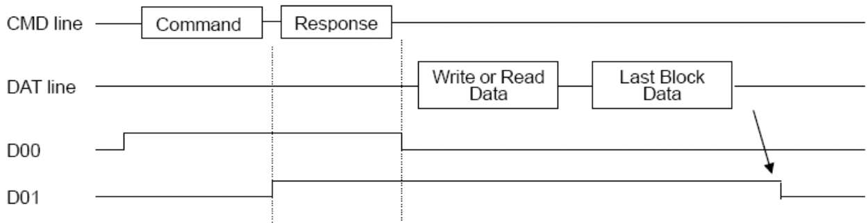
Figure 27-3. Timing of Command Inhibit (DAT) and Command Inhibit (CMD) with data transfer
