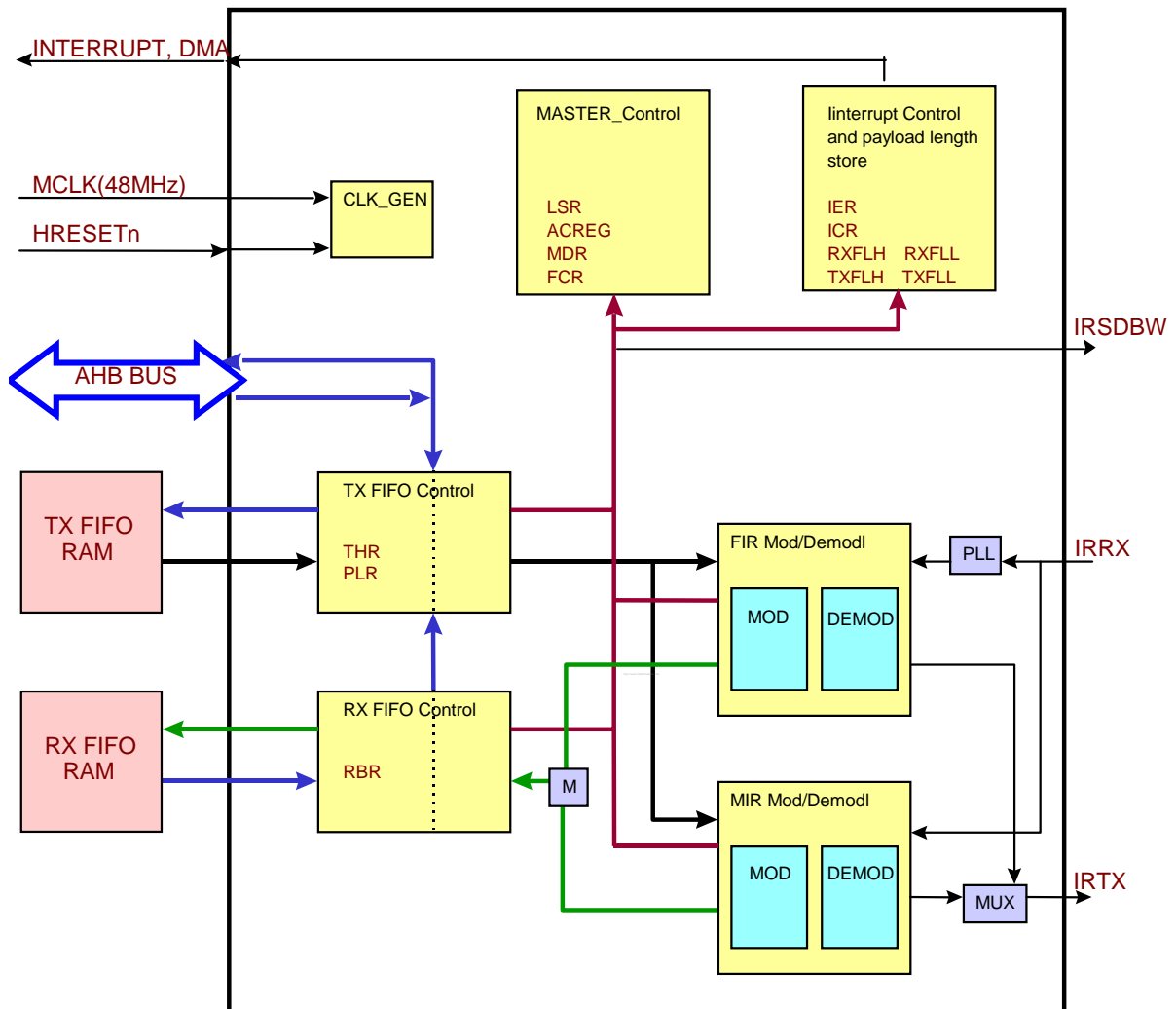
Figure 38-1 Block Diagram
