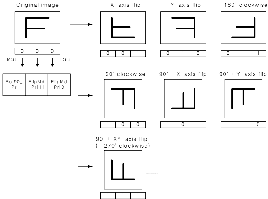
Figure 20-22 Preview image mirror and rotation
