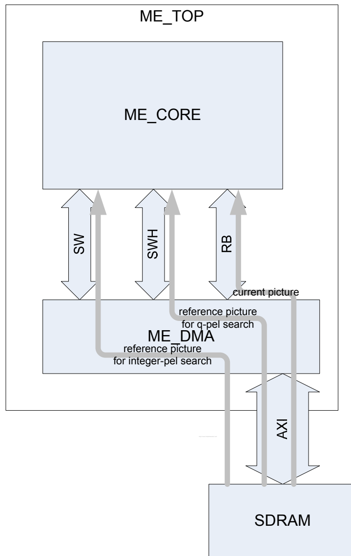
Figure 21.13. Motion Estimation Block Diagram
