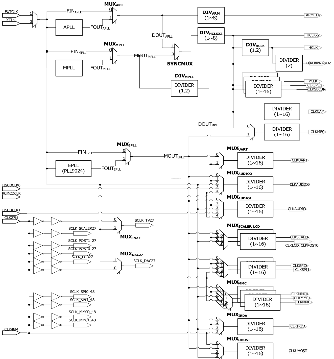
Figure 3-2. The block diagram of clock generator
