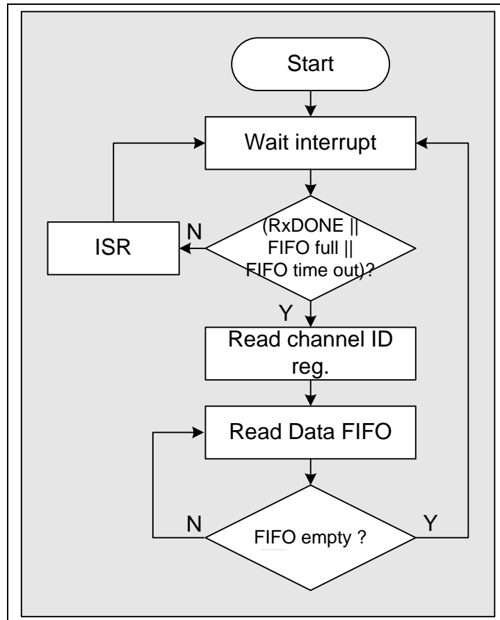
Figure 28-15 Basic Rx module programming flow chart
