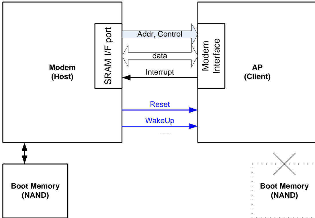
Figure 24-9. Modem Boot connection diagram
