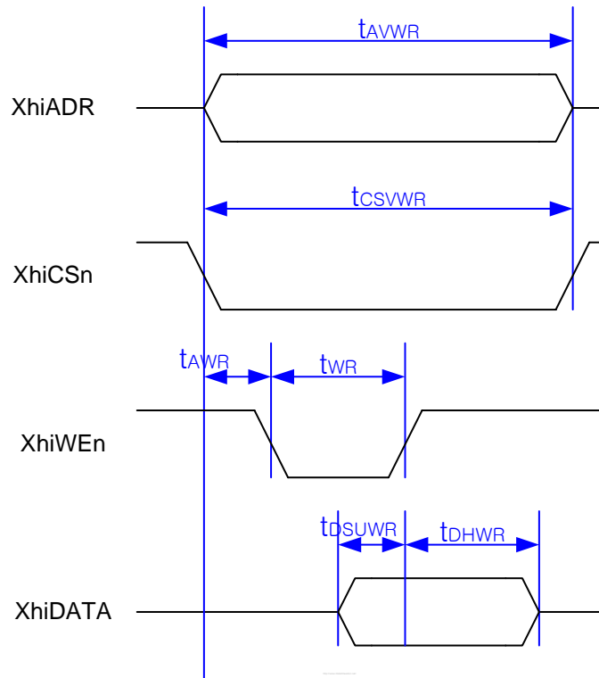
Figure 23-5 Modem interface write timing diagram
