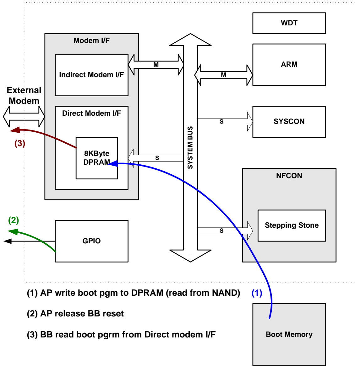
Figure 23-3 AP Booting for MODEM boot procedure
