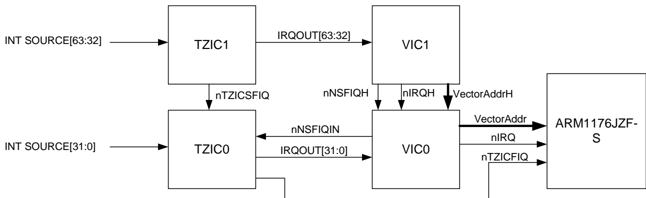
Figure 12-1 Interrupt Controller in S3C6400X
