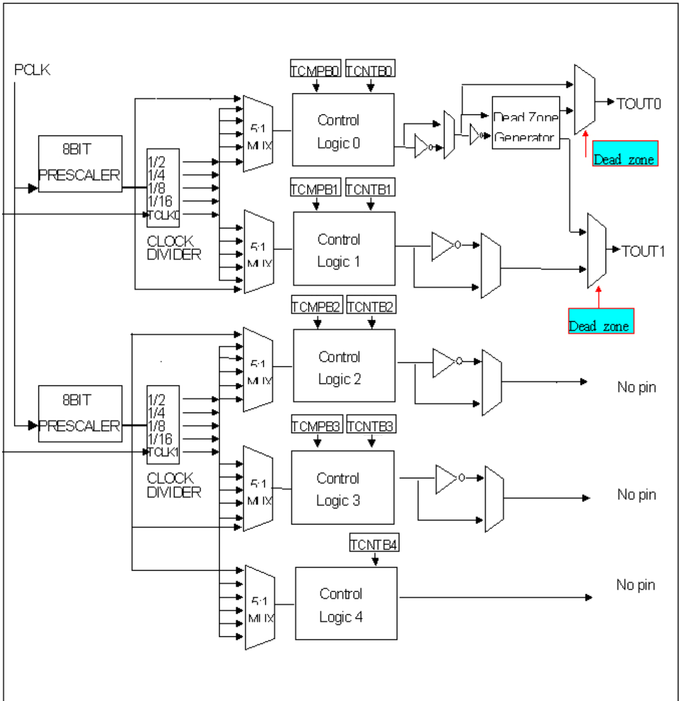
Figure 32-3: PWMTIMER Clock Tree Diagram
