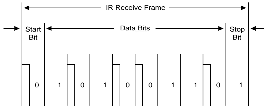
Figure 31-7 Infra-Red Receive Mode Frame Timing Diagram
