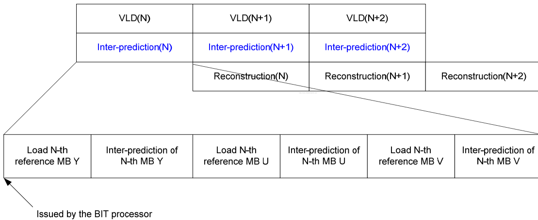
Figure 21.19 Inter-prediction pipeline of encoding case
