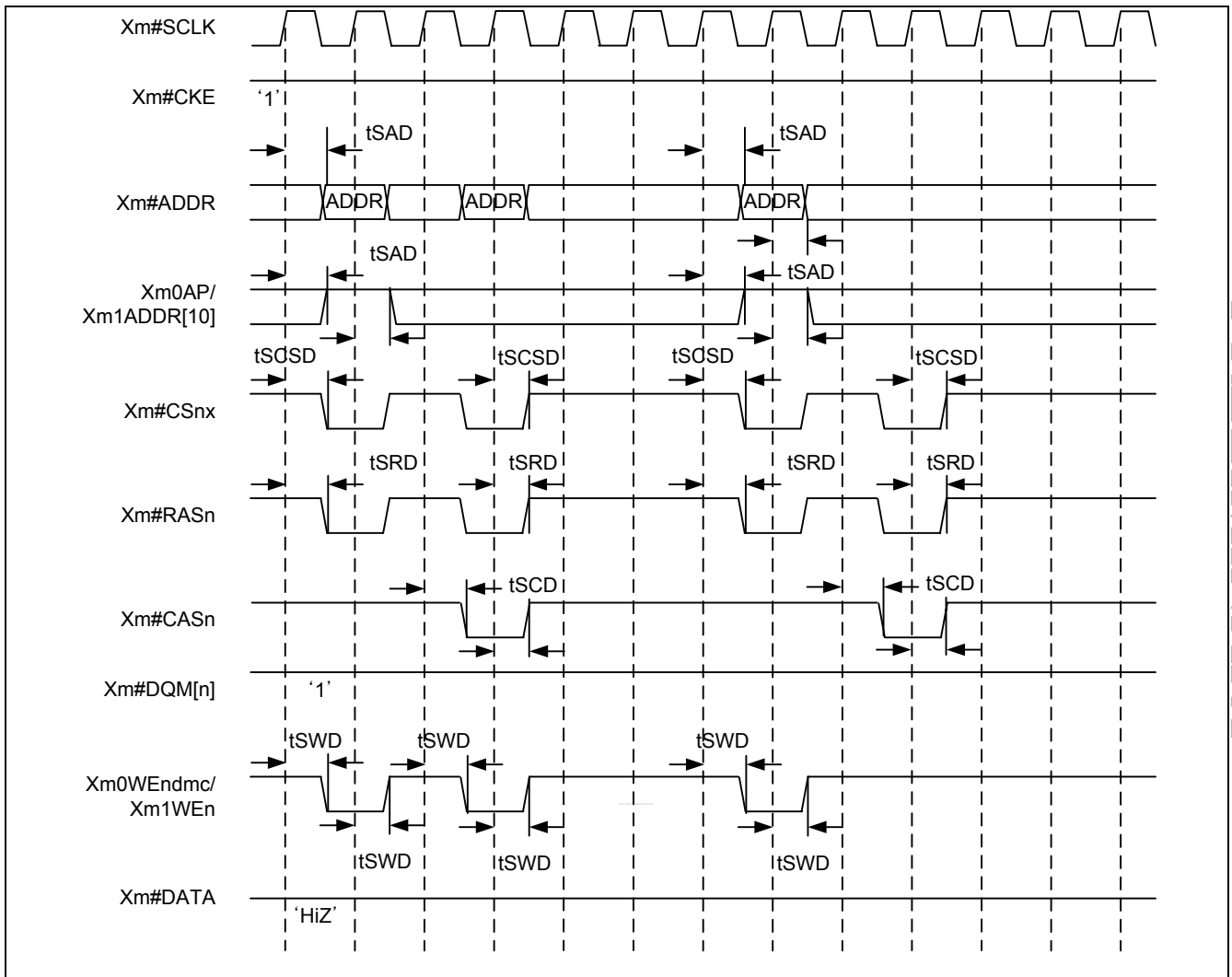
Figure 41-12. SDRAM MRS Timing and Auto Refresh Timing (Trp = 2, Trc = 4)
