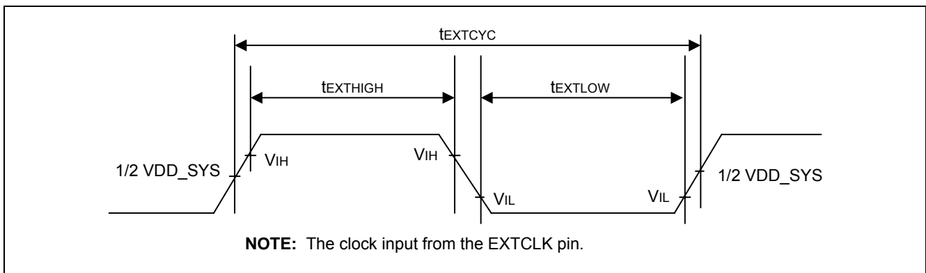
Figure 41-2. EXTCLK Clock Input Timing
