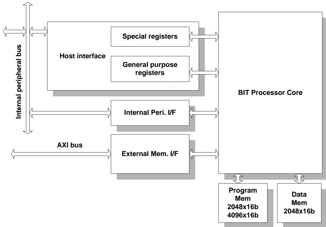
Figure 21.3. BIT processor block diagram
