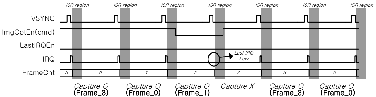
Figure 20-12. Timing diagram for last IRQ (LastIRQEn is disabled)
