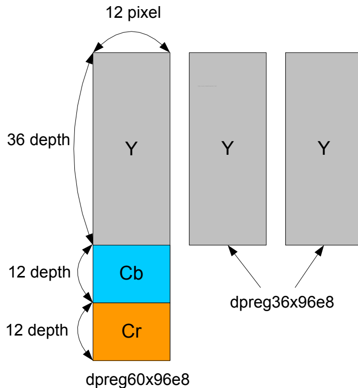
Figure 21.17. The local buffer memory configuration
