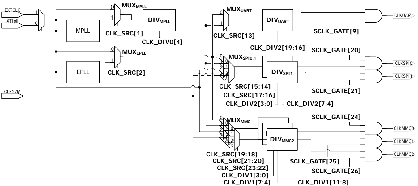
Figure 3-12. UART/SPI/MMC clock generation
