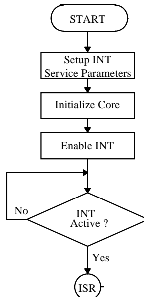
Figure 38-7 General Program Flowchart
