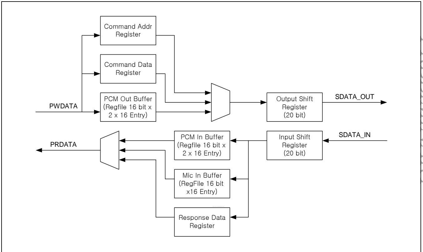
Figure 35-2. Internal Data Path
