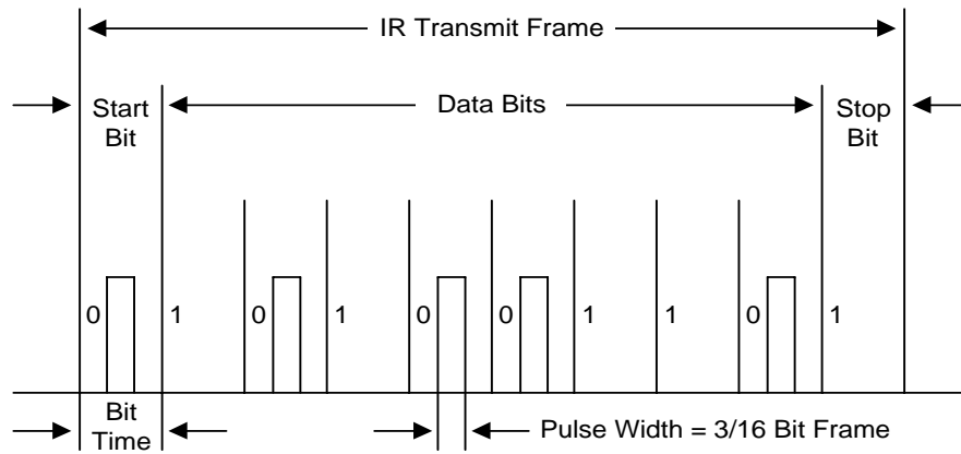
Figure 31-6 Infra-Red Transmit Mode Frame Timing Diagram
