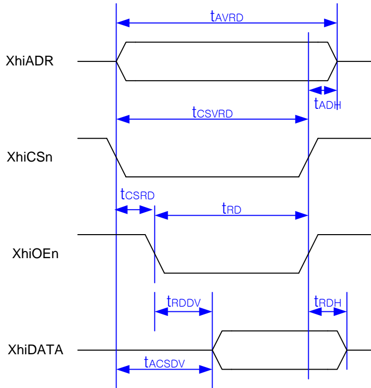
Figure 23-6 Modem interface read timing diagram
