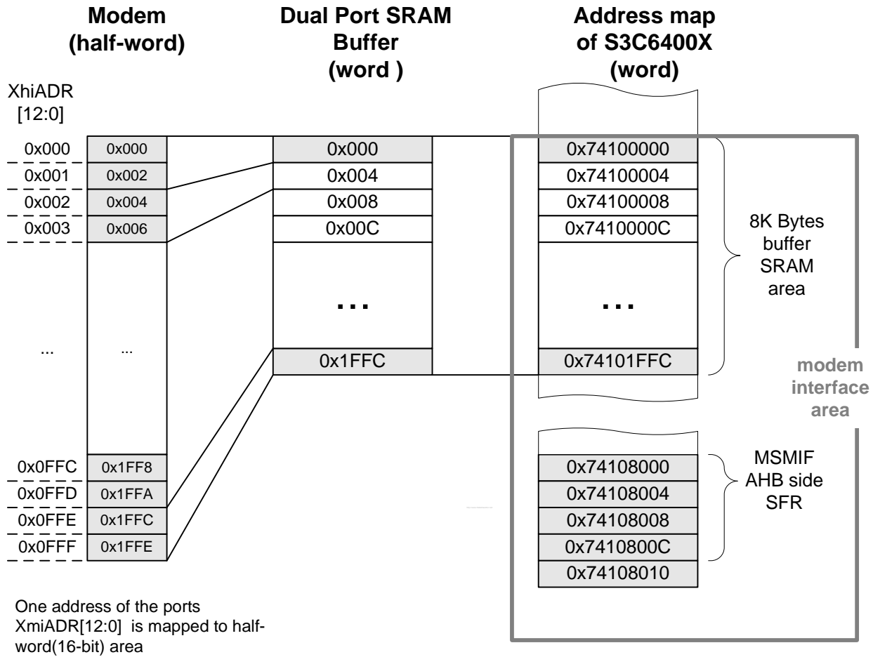
Figure 23-4 MODEM interface address mapping
