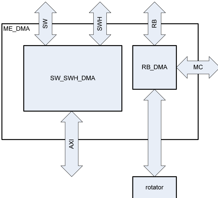
Figure 21.15. Motion Estimation DMA Block Diagram
