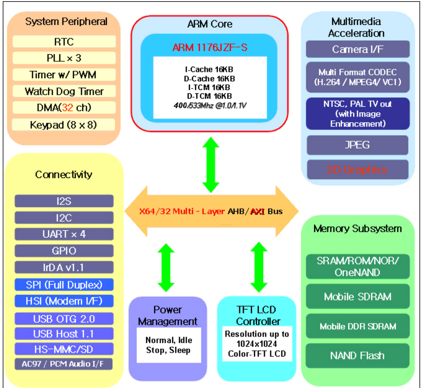
Figure 1-1 S3C6400 block diagram
