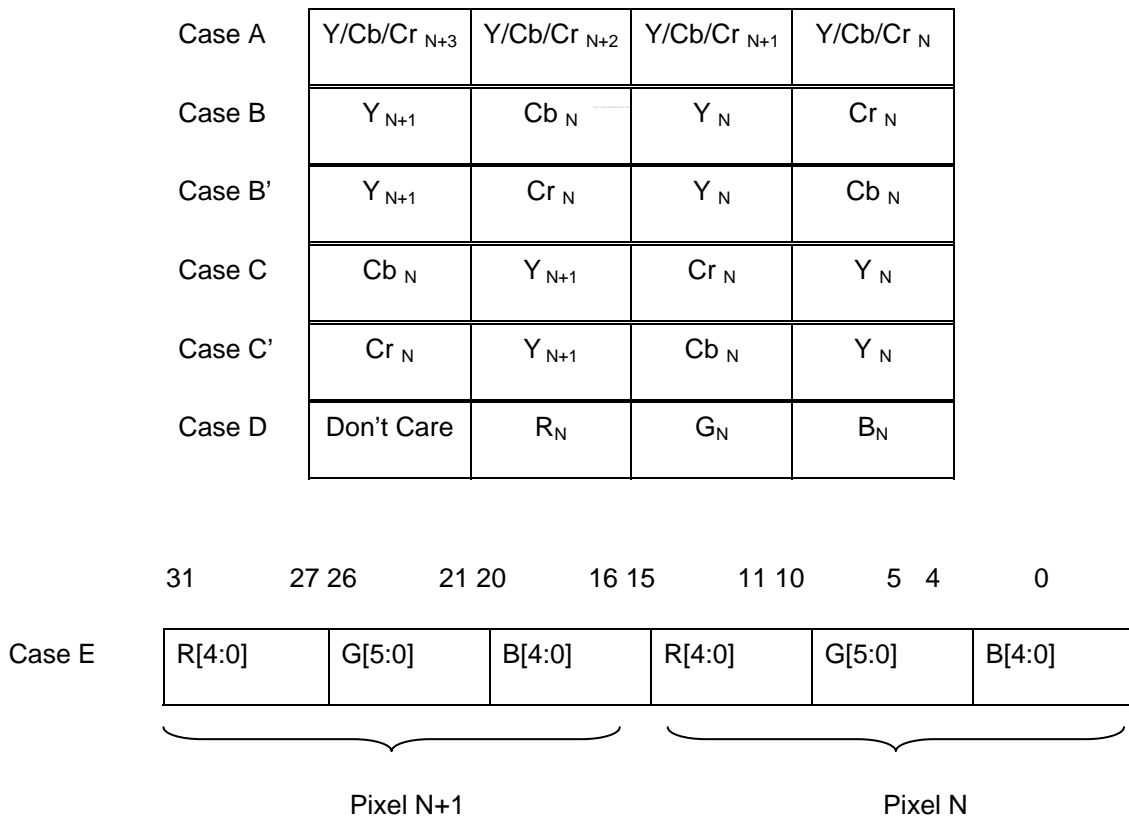
Figure 15-4 Byte and half-word organization Block Diagram
