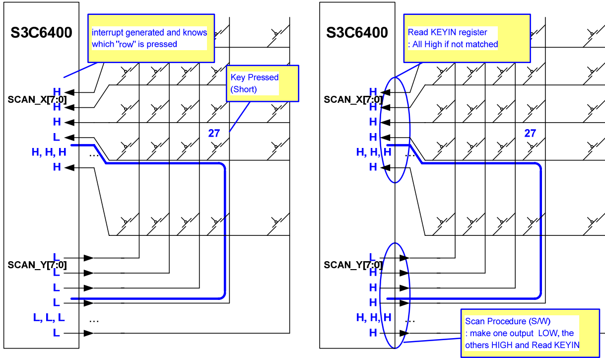
Figure 40-4 Keypad scanning procedure II
