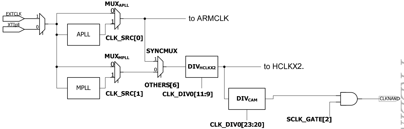
Figure 3-9. Camera I/F clock generation
