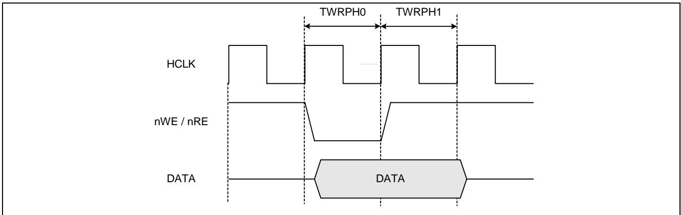
Figure 8-4 nWE & nRE Timing (TWRPH0=0, TWRPH1=0) Block Diagram
