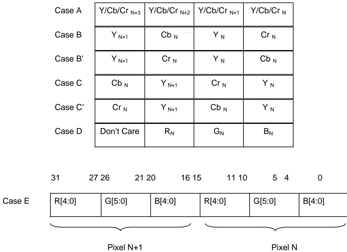
Figure 16-4 Byte and half-word organization Block Diagram
