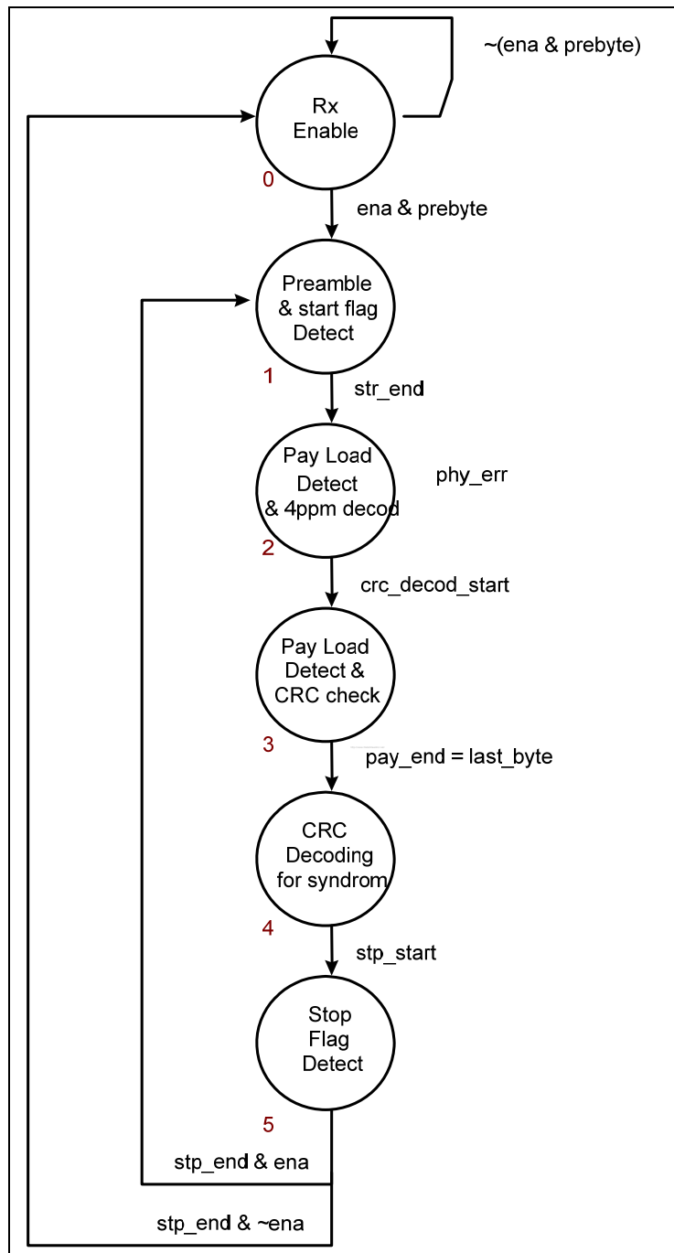
Figure 38-3 FIR demodulation process
