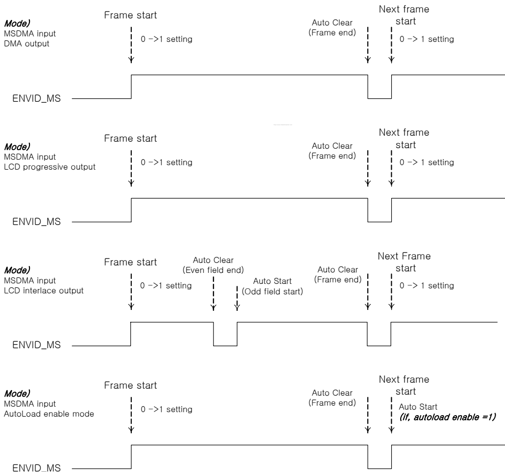
Figure 20-24. ENVID_MS SFR setting when DMA start to read memory data
