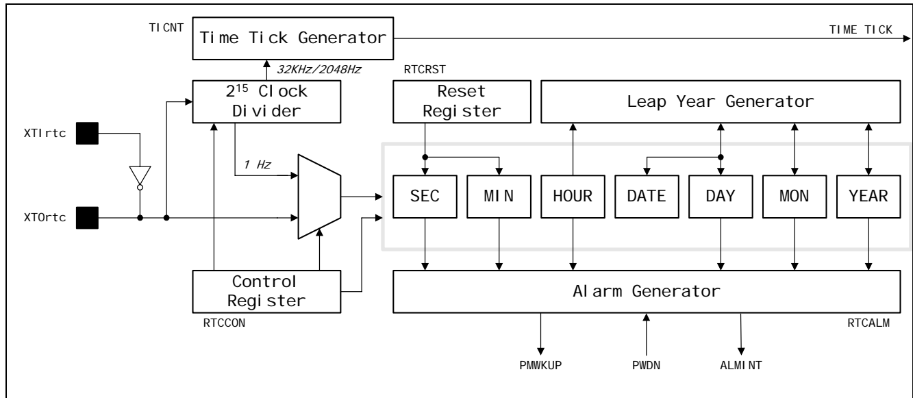
Figure 33-1. Real Time Clock Block Diagram
