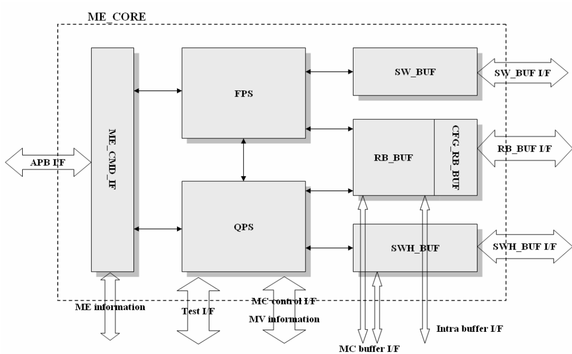
Figure 21.14. Motion Estimation Core Block Diagram
