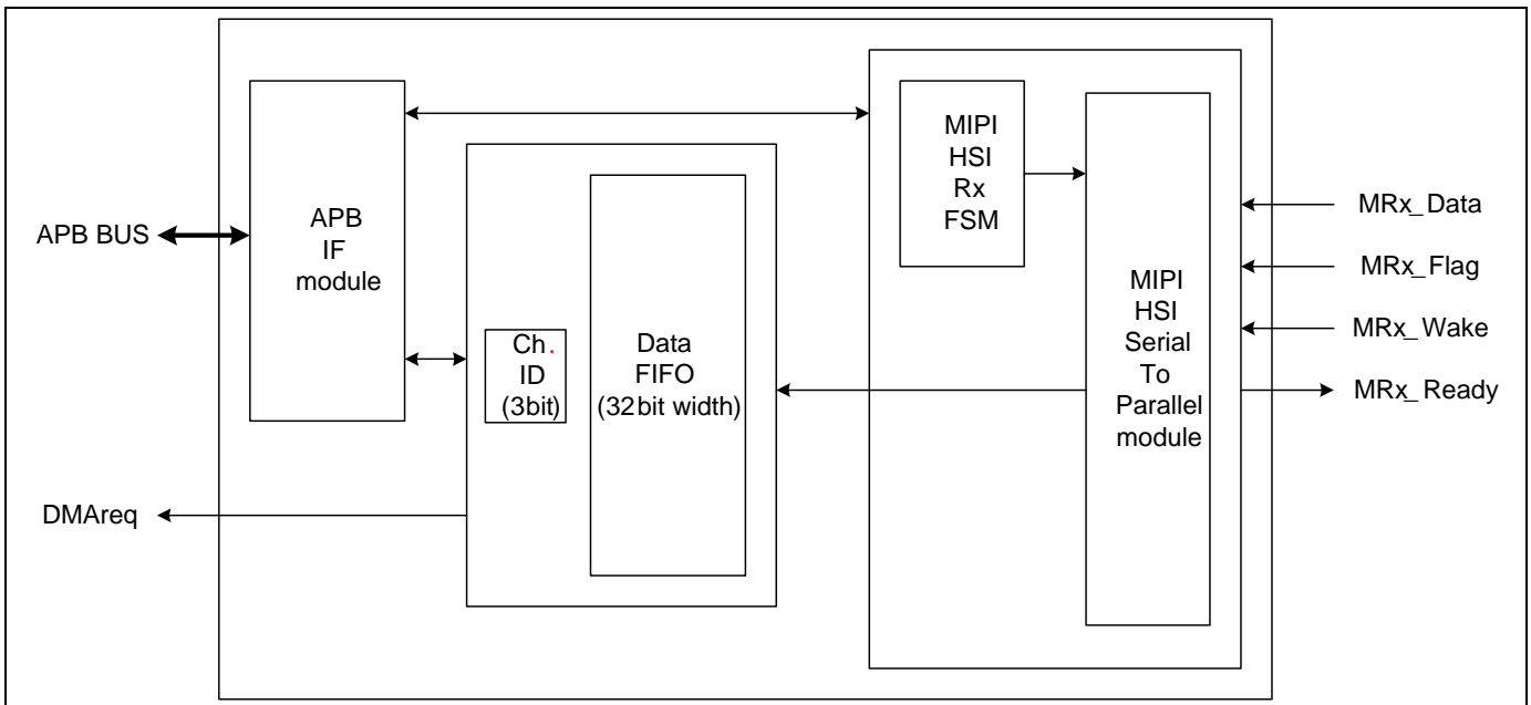
Figure 28-4 MIPI HSI interface controller Rx module Top Block Diagram
