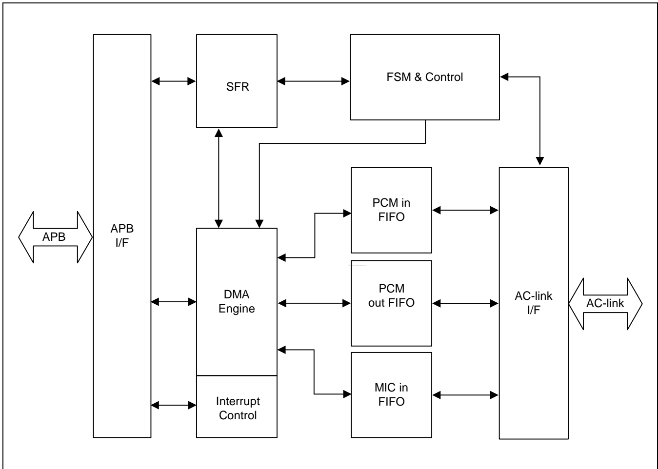
Figure 35-1. AC97 Block Diagram
