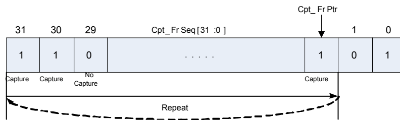
Figure 20-23. Capture frame control
