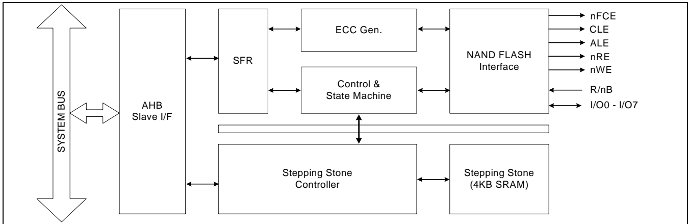
Figure 8-1 NAND Flash Controller Block Diagram
