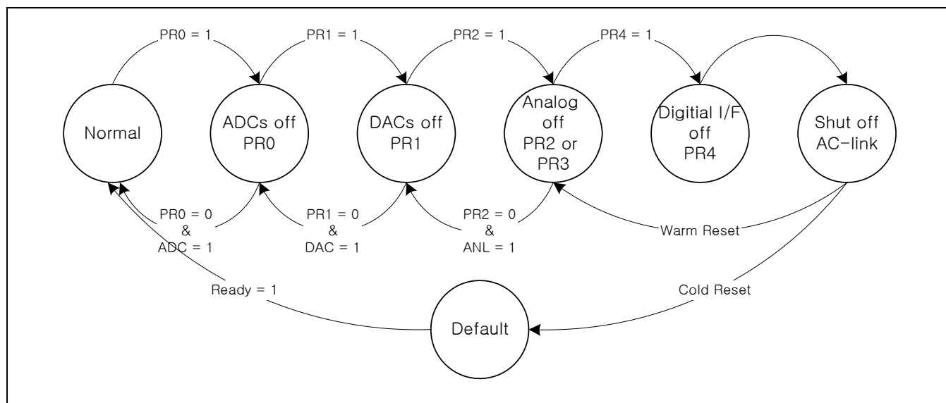
Figure 35-8 AC97 Power down/Power up Flow
