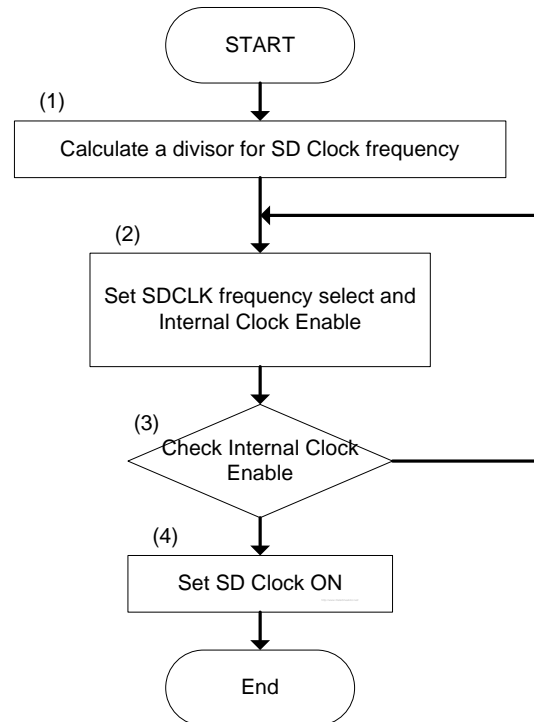
Figure 27-3. SD Clock Supply Sequence
