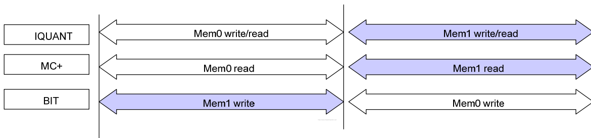
Figure 21.39 H.264 decoding case
