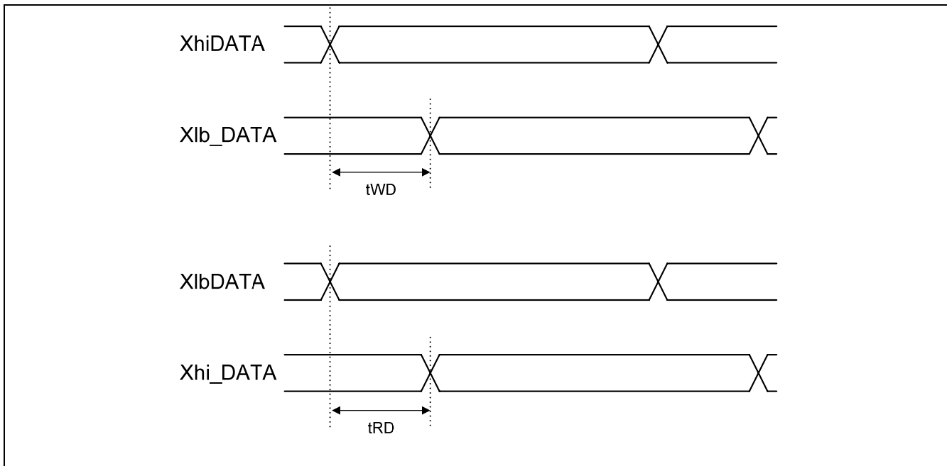
Figure 41-17. LCD Bypass Data for write and read timing diagram
