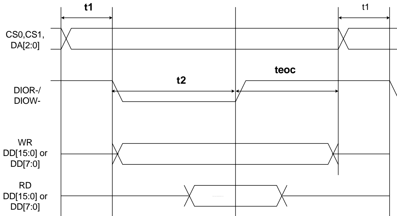
Figure 9-5: PIO Mode Waveform
