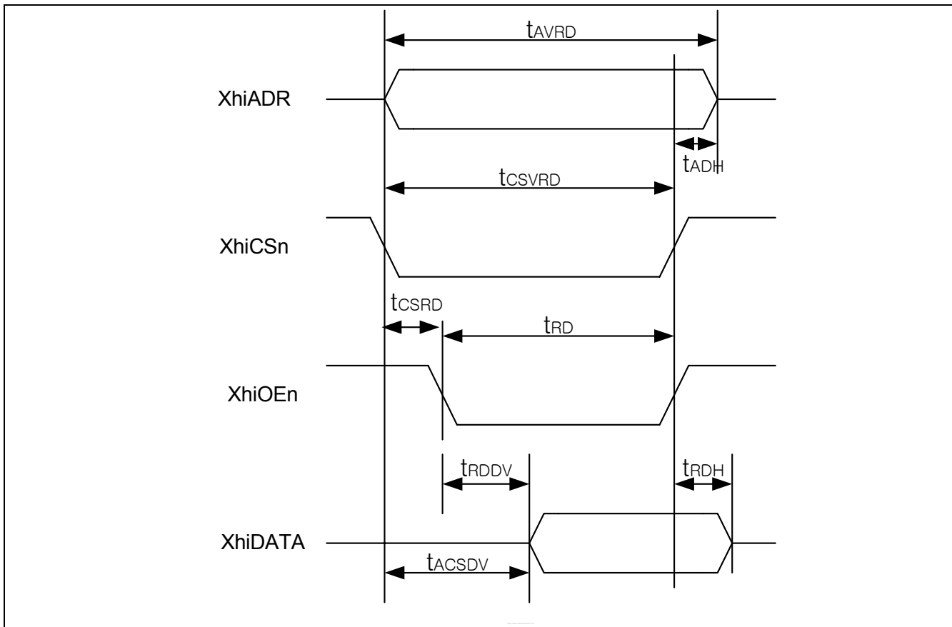
Figure 41-15. Modem interface read timing diagram
