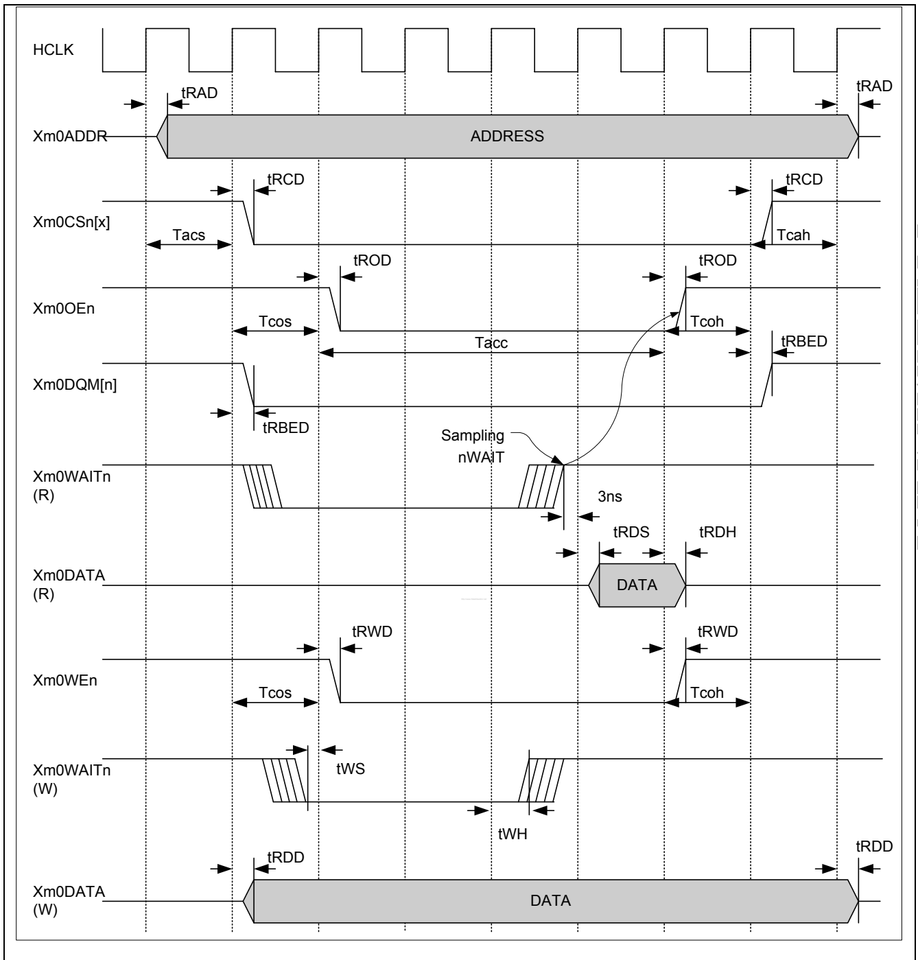
Figure 41-7. ROM/SRAM Timing (Tacs = 0, Tcos = 0, Tacc = 2, Tcoh = 0, Tcah = 0, PMC = 0, ST = 0, DW = 16-bit)
