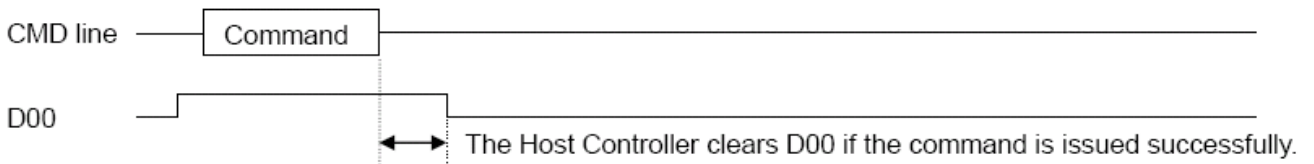
Figure 27-5. Timing of Command Inhibit (CMD) for the case of no response command
