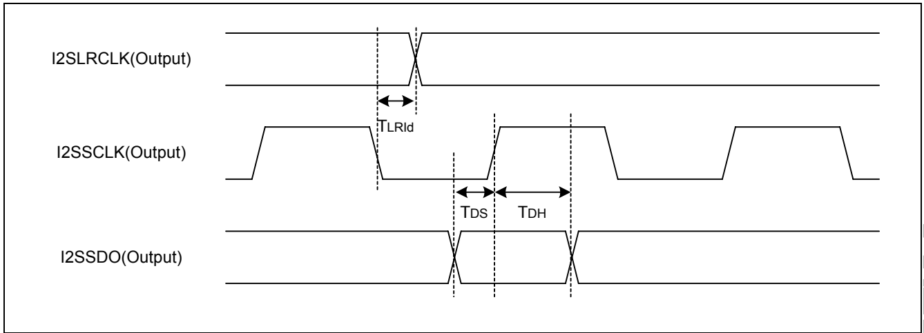
Figure 41-24. IIS Interface Timing (Master / TX)
