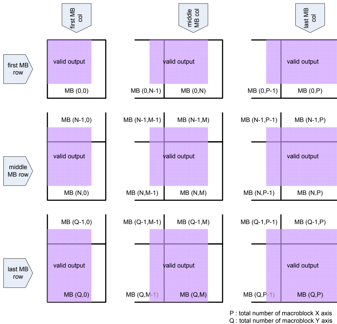
Figure 21.32 valid output data of deblocking filter in H.263 Annex J mode
