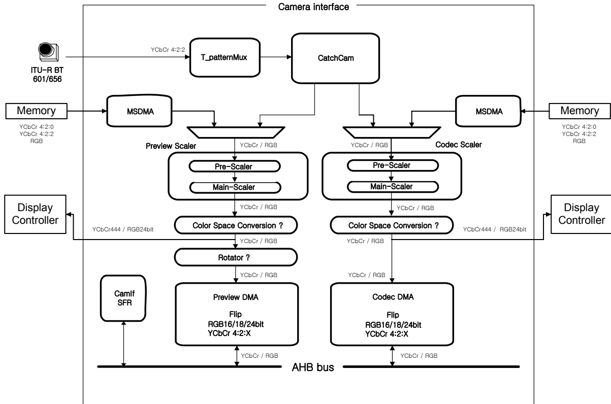
Figure 20-1. Camera interface overview
