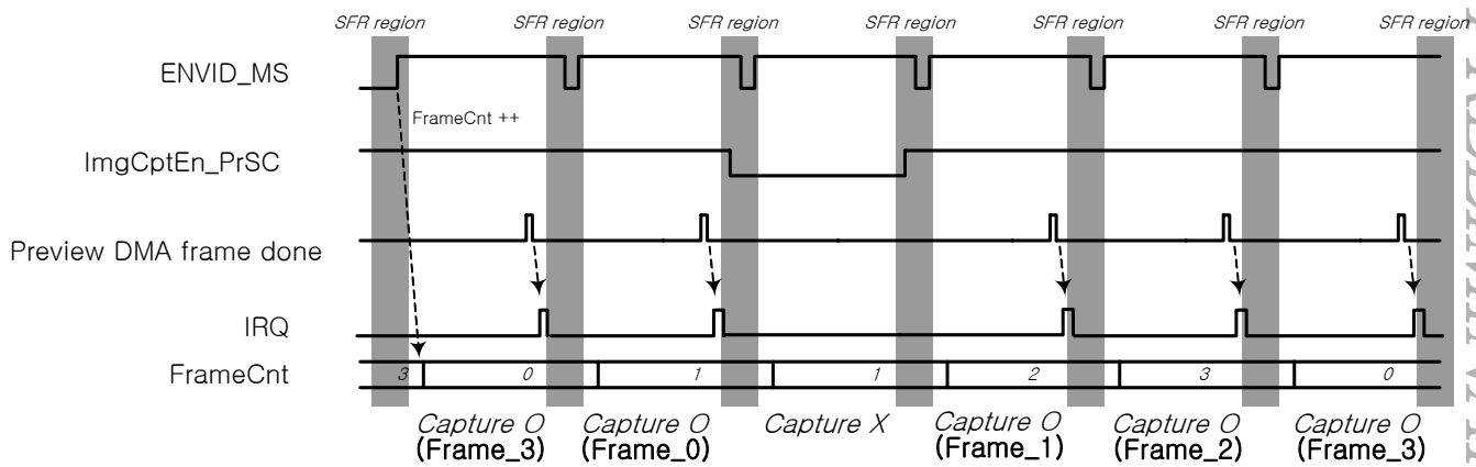
Figure 20-14. Timing diagram for IRQ (MSDMA path)
