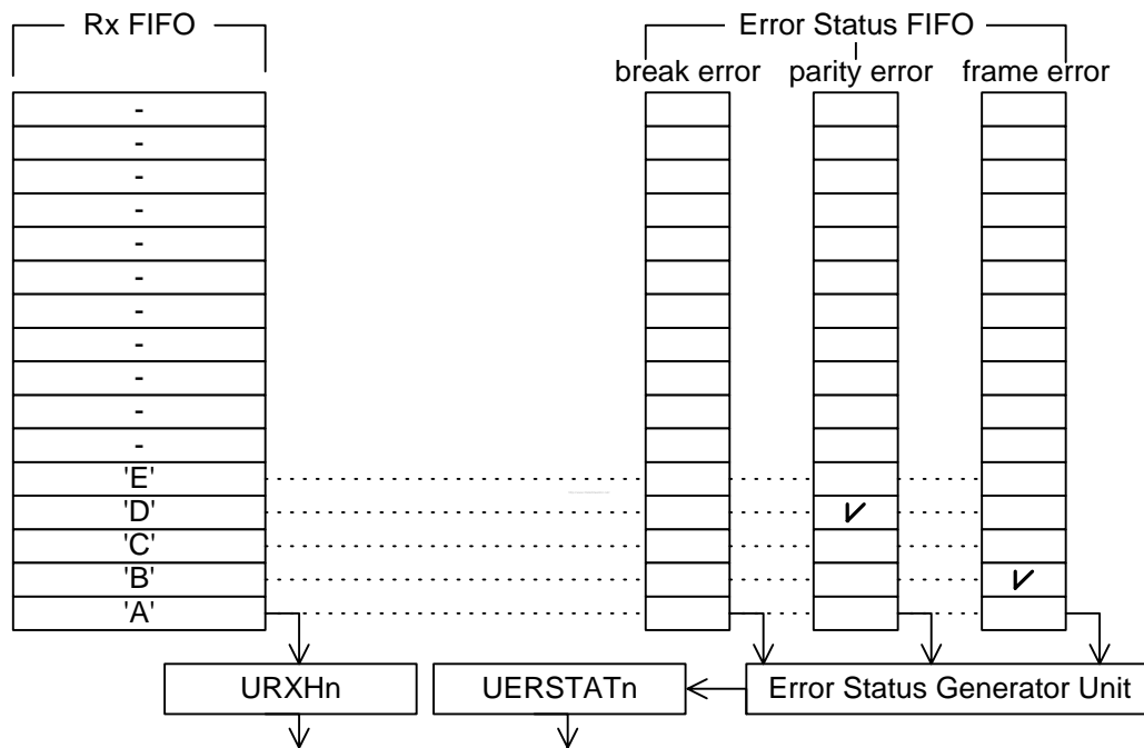
Figure 31-3 Example showing UART Receiving 5 Characters with 2 Errors
