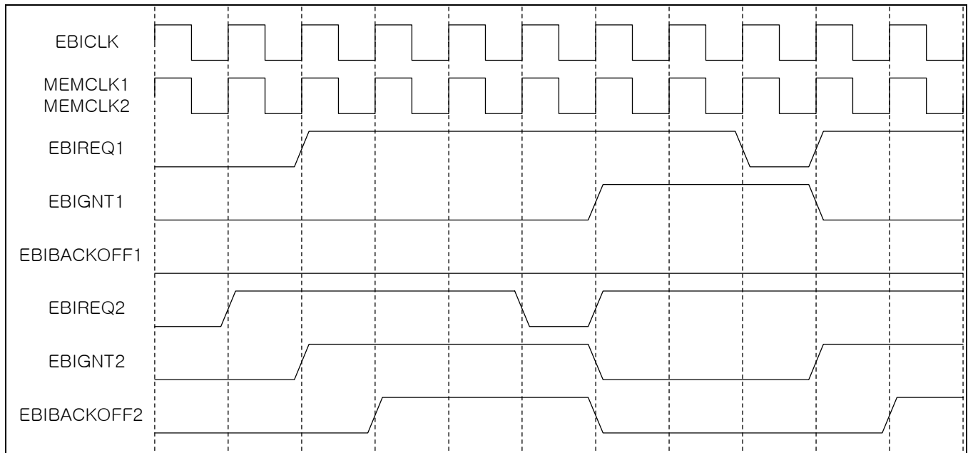
Figure 4-4. EBIBACKOFF signal
