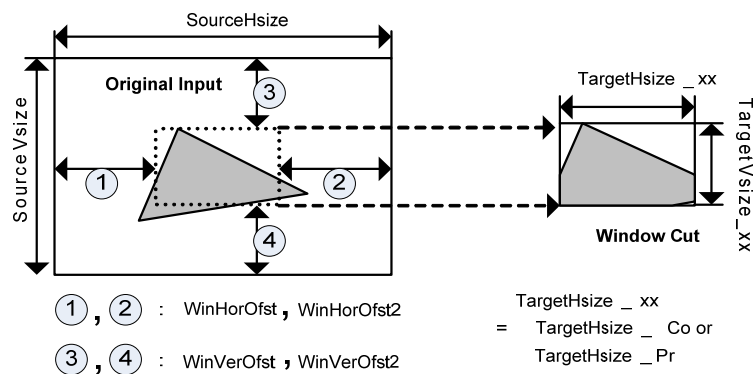
Figure 20-16. Window offset scheme
