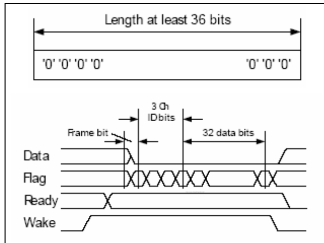
Figure 28-11 Break frame Block Diagram
