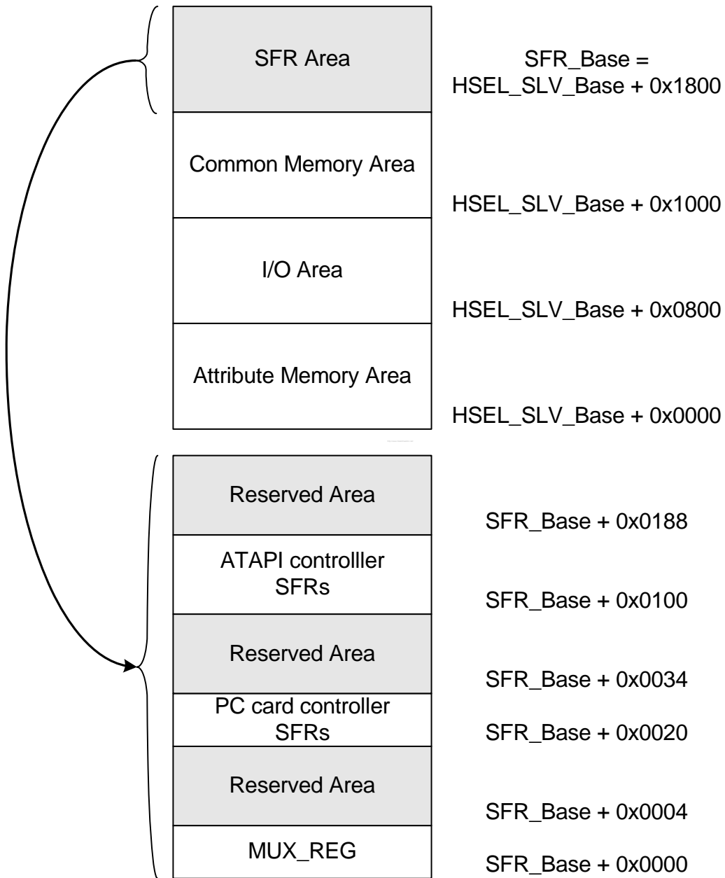
Figure 9-10: Memory Map Diagram
