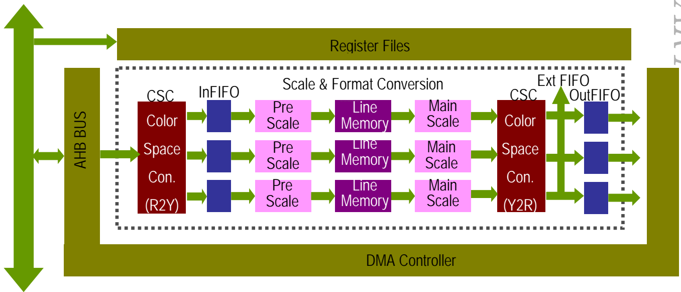
Figure 15-1. Block Diagram of Post Processor
