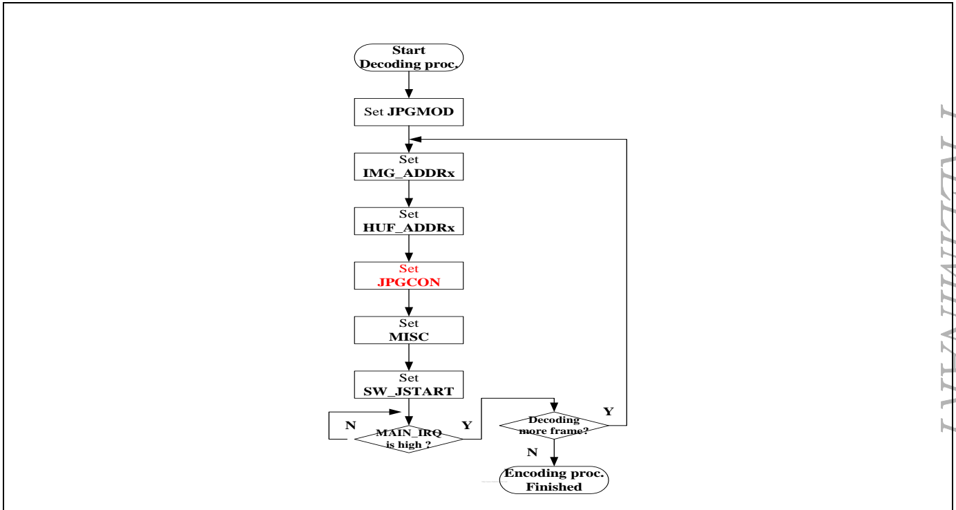
Figure 22-6. Example flow chart of hardware controlled decoding
