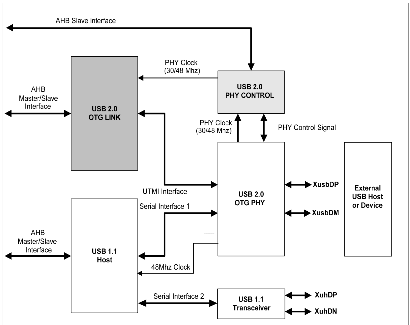
Figure 26-1. System Level Block Diagram
