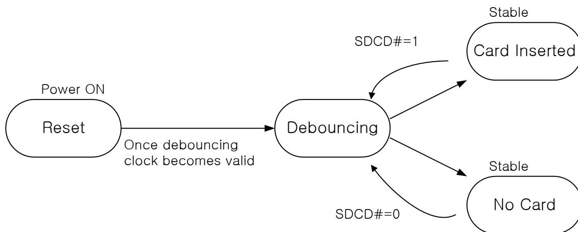
Figure 27-2. Card Detect State
