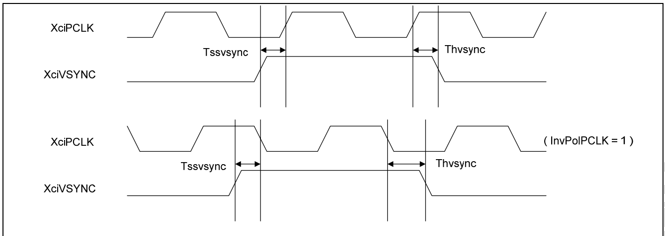
Figure 41-18. Camera Interface VSYNC Timing
