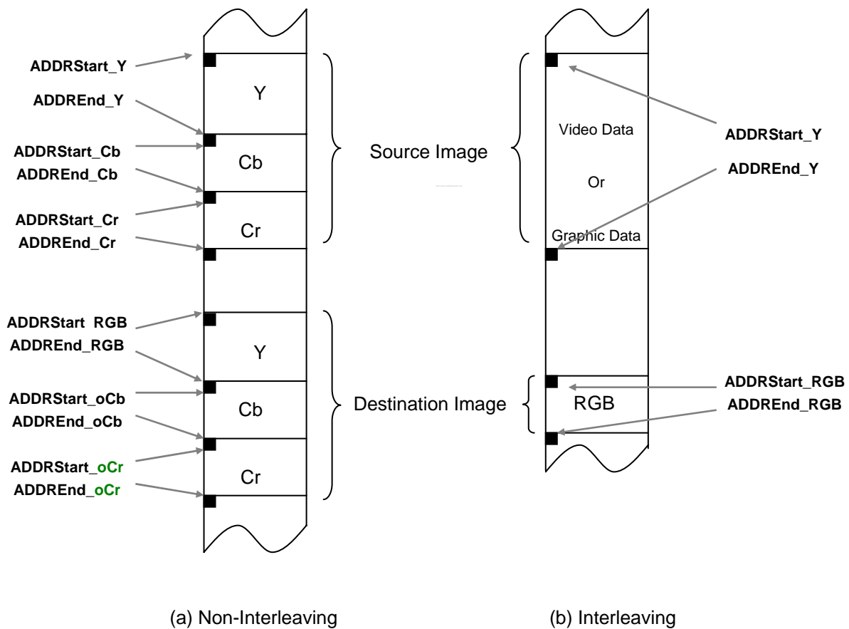
Figure 16-6 Start and end address set according to memory allocation type
