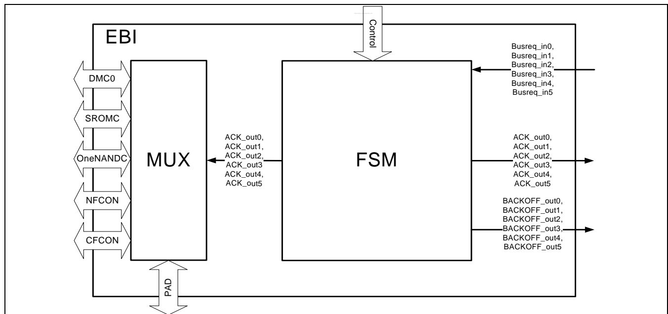
Figure 4-1. EBI Block Diagram
