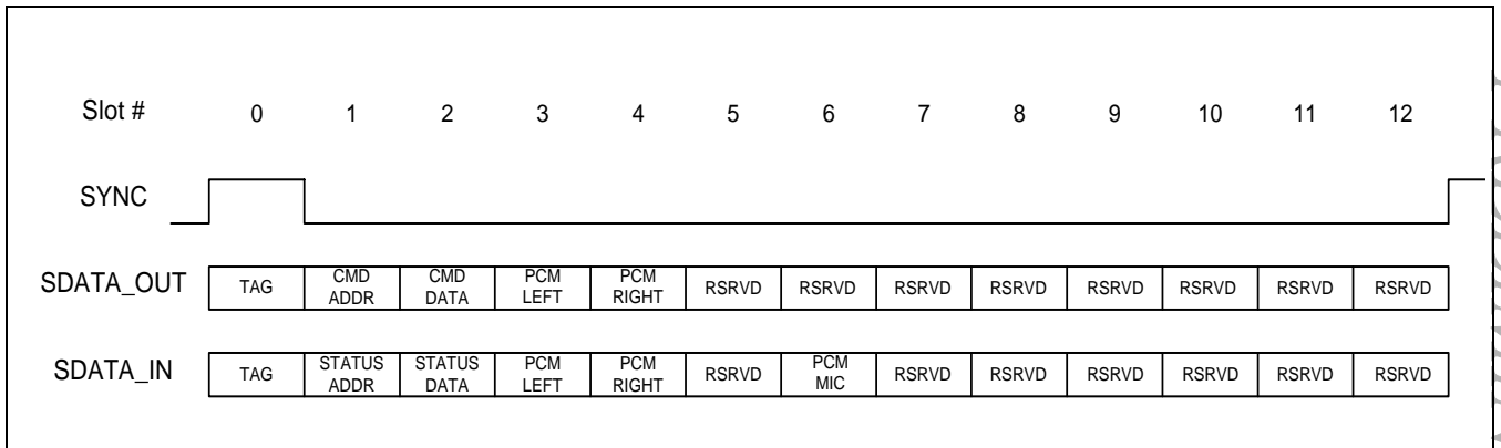
Figure 35-4. Bi-directional AC-link Frame with Slot Assignments
