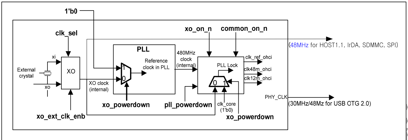
Figure 26-3. OTG PHY Clock Path
