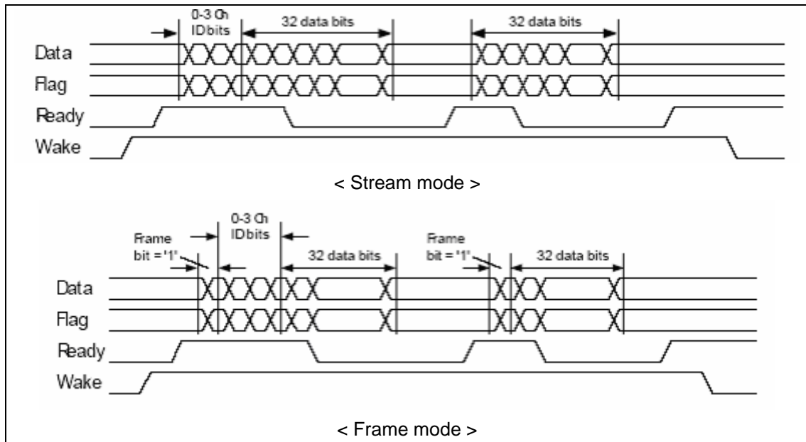
Figure 28-8 Example of Burst channel ID mode Block Diagram
