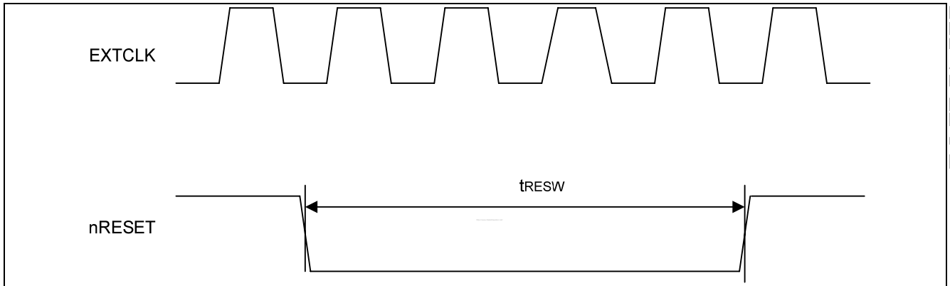
Figure 41-4. Manual Reset Input Timing
