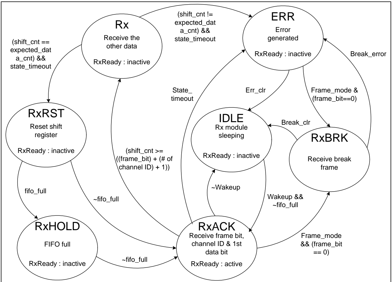
Figure 28-13 FSM of Rx module Part
