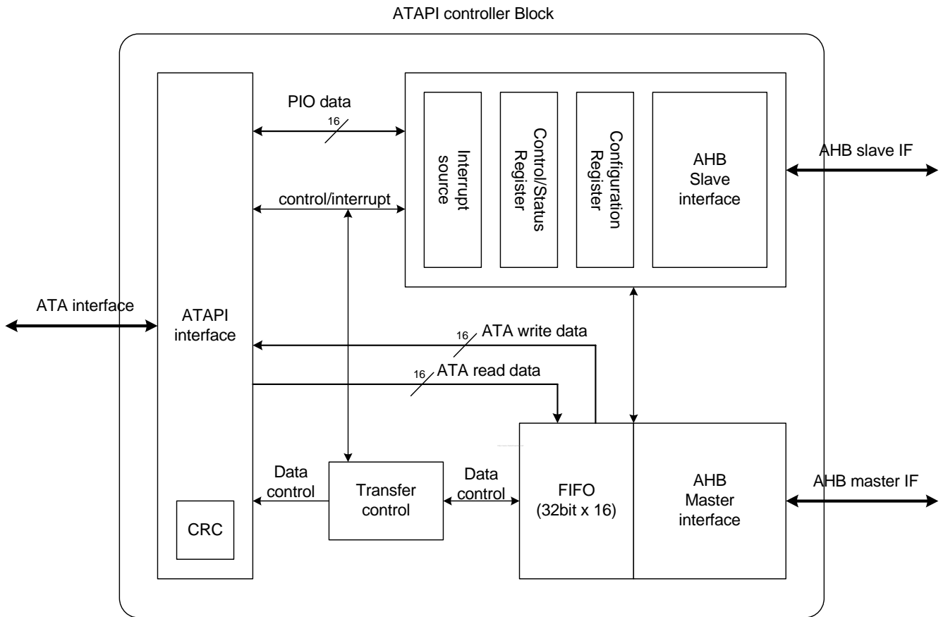
Figure 9-3: ATAPI Controller Top Block Diagram
