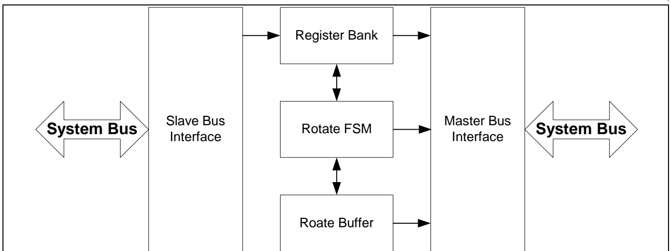
Figure 19-1 Image Rotator Block Diagram
