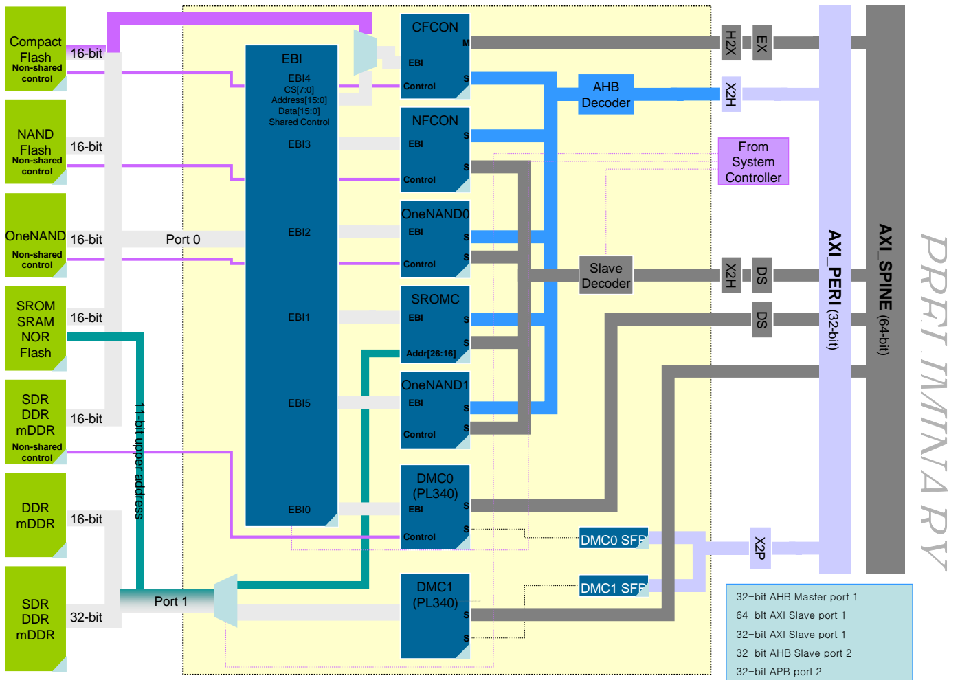
Figure 4-2. Memory interface through EBI
