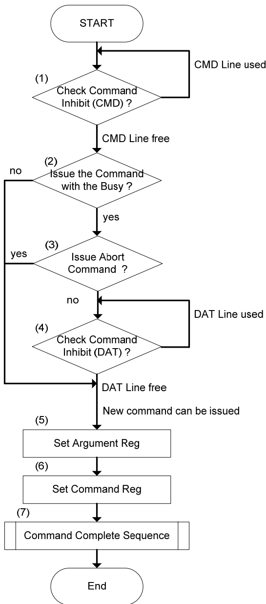
Figure 27-9. Timeout Setting Sequence
