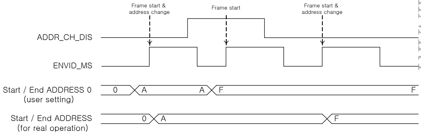
Figure 20-26. ADDRESS Change timing (related MSDMA)
