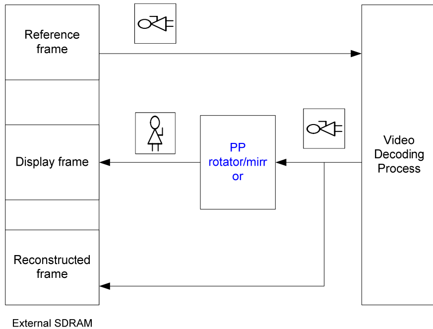
Figure 21.12. PP rotator data flow
