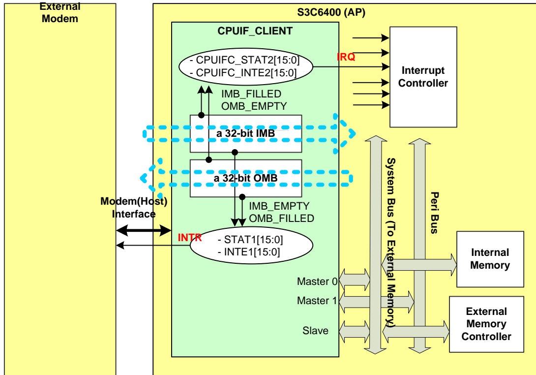
Figure 24-11. In/Out Mailbox between Modem and AP
