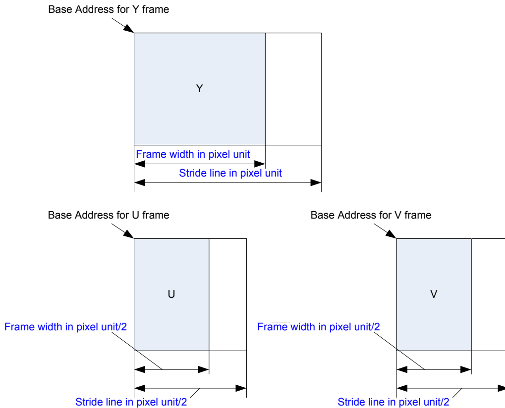
Figure 21.9. Frame buffer configuration
