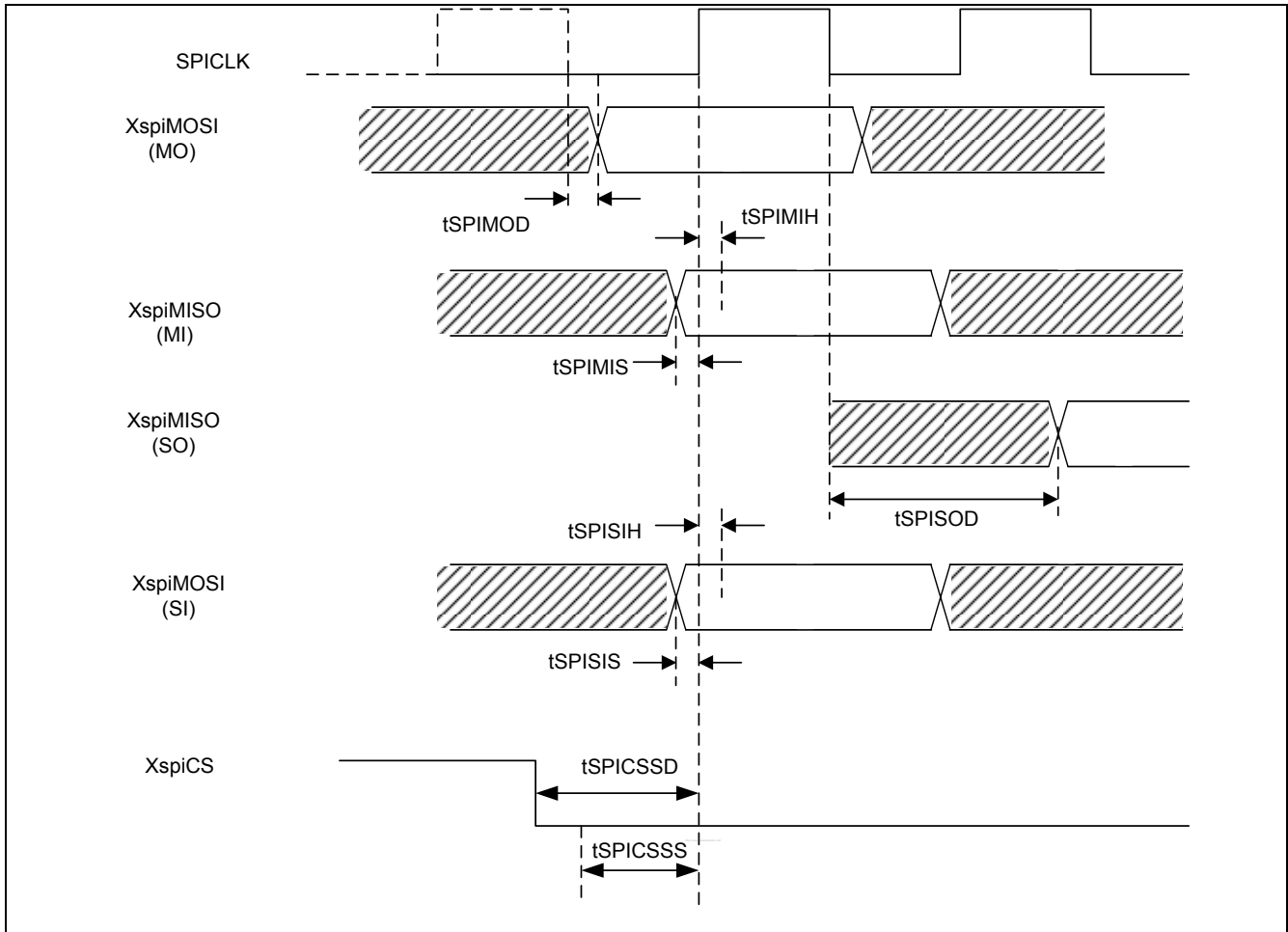
Figure 41-22. SPI Interface Timing (CPHA = 0, CPOL = 0)
