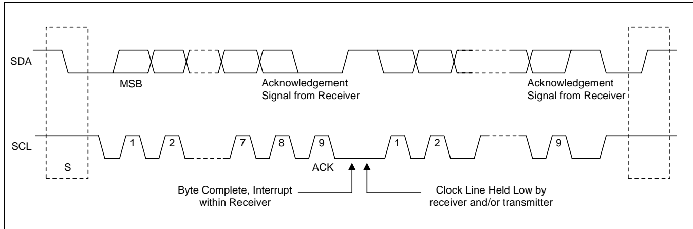
Figure 30-3. Data Transfer on the IIC-Bus Block Diagram
