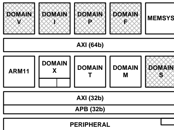
Figure 3-14. Power domains at NORMAL/IDLE mode (grey colored domain can be ON/OFF by NORMAL_CFG configuration register)
