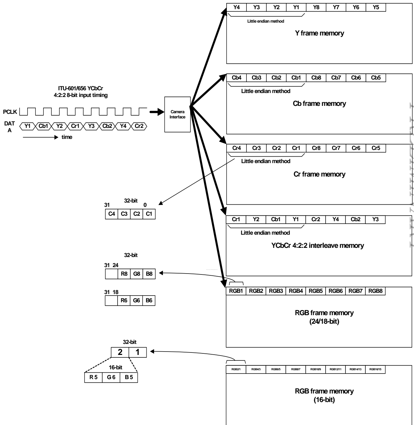
Figure 20-9. Memory storing style
