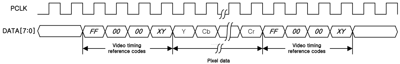
Figure 20-3. ITU-R BT 656 Input timing diagram
