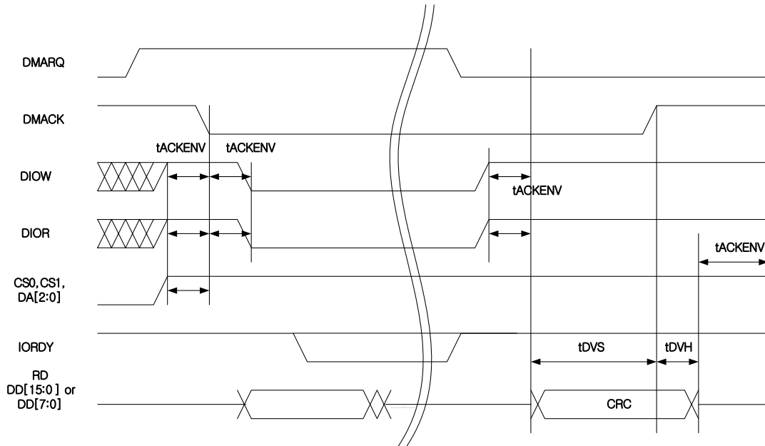
Figure 5-6: UDMA - In operation (terminated by device)
