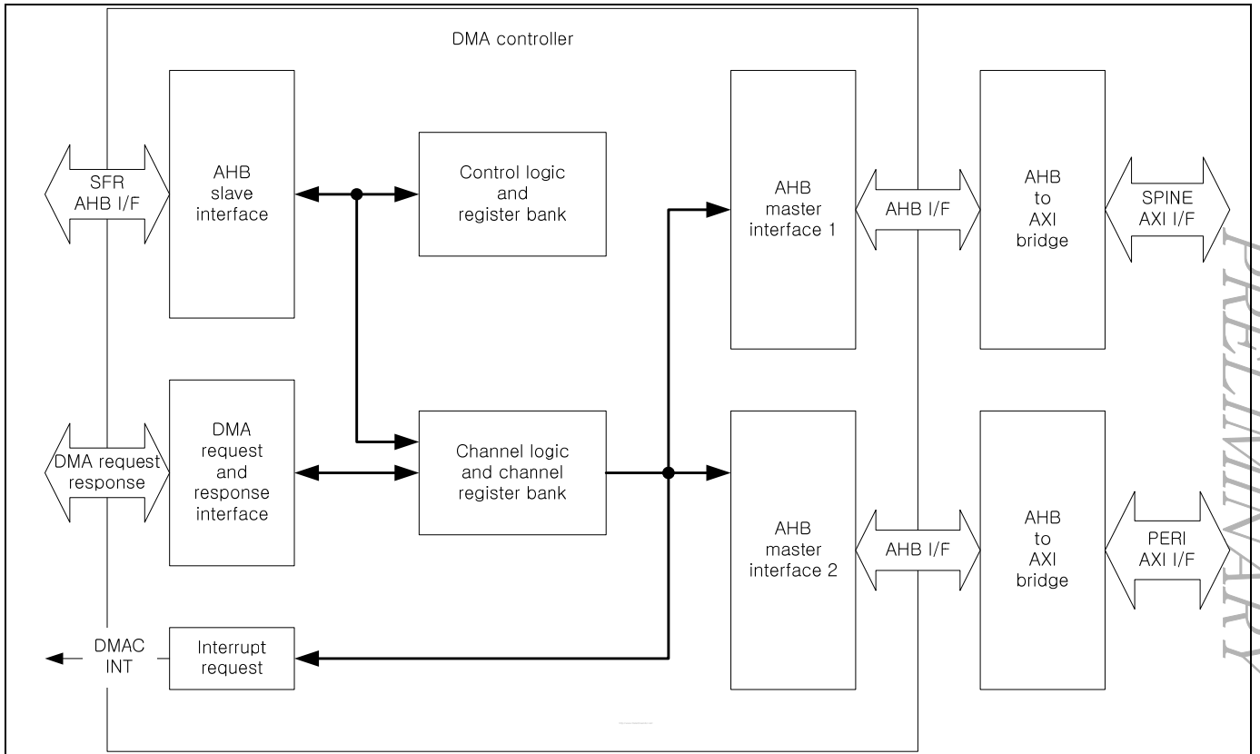
Figure 11-1. DMAC block diagram
