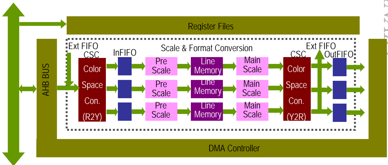
Figure 16-1. Block Diagram of TV Scaler
