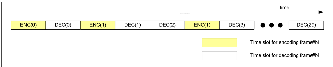
Figure 21.8 full-duplex codec processing
