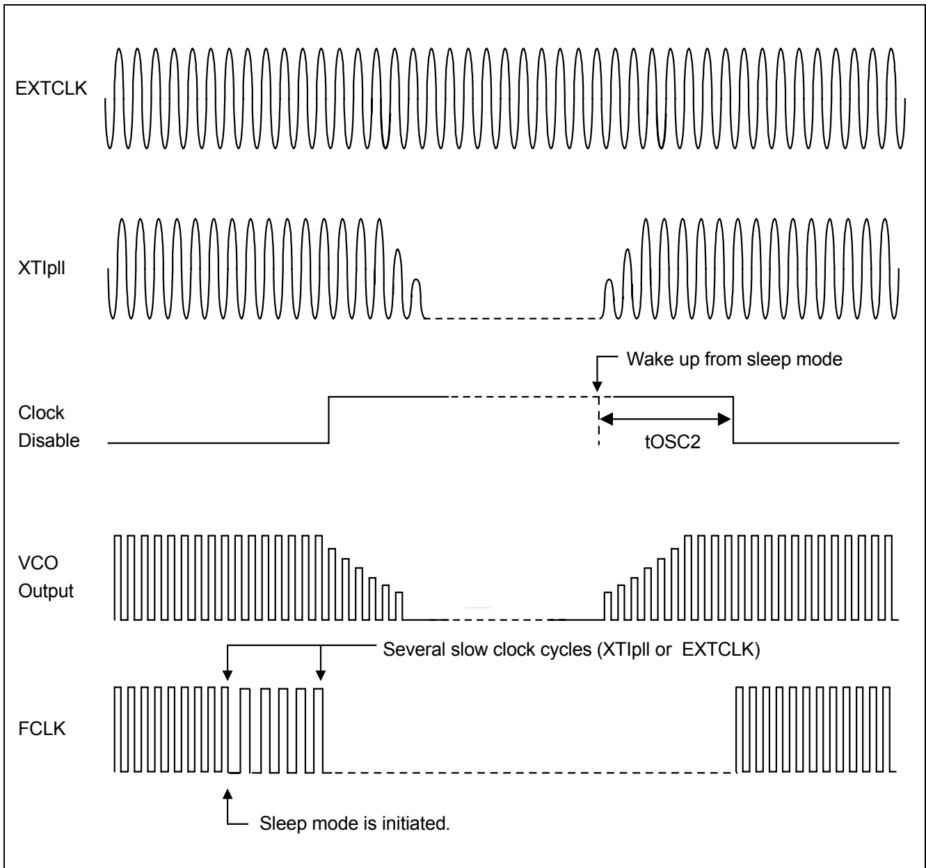
Figure 41-6. Sleep Mode Return Oscillation Setting Timing
