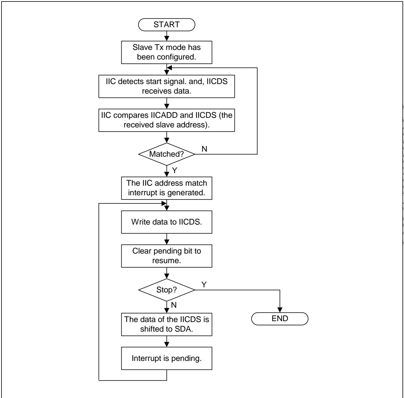
Figure 30-7. Operations for Slave/Transmitter Mode
