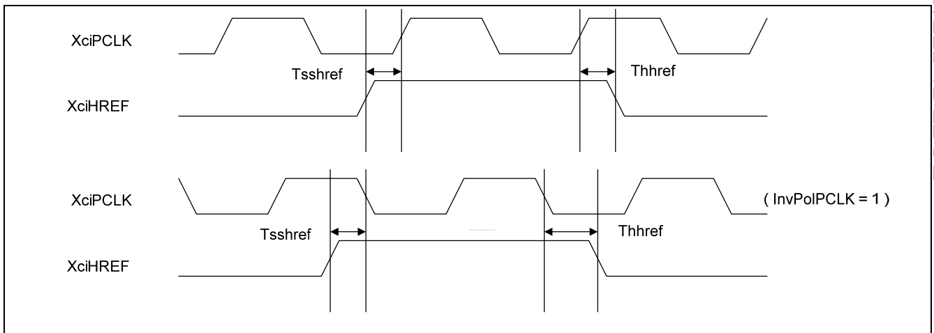
Figure 41-19. Camera Interface HREF Timing
