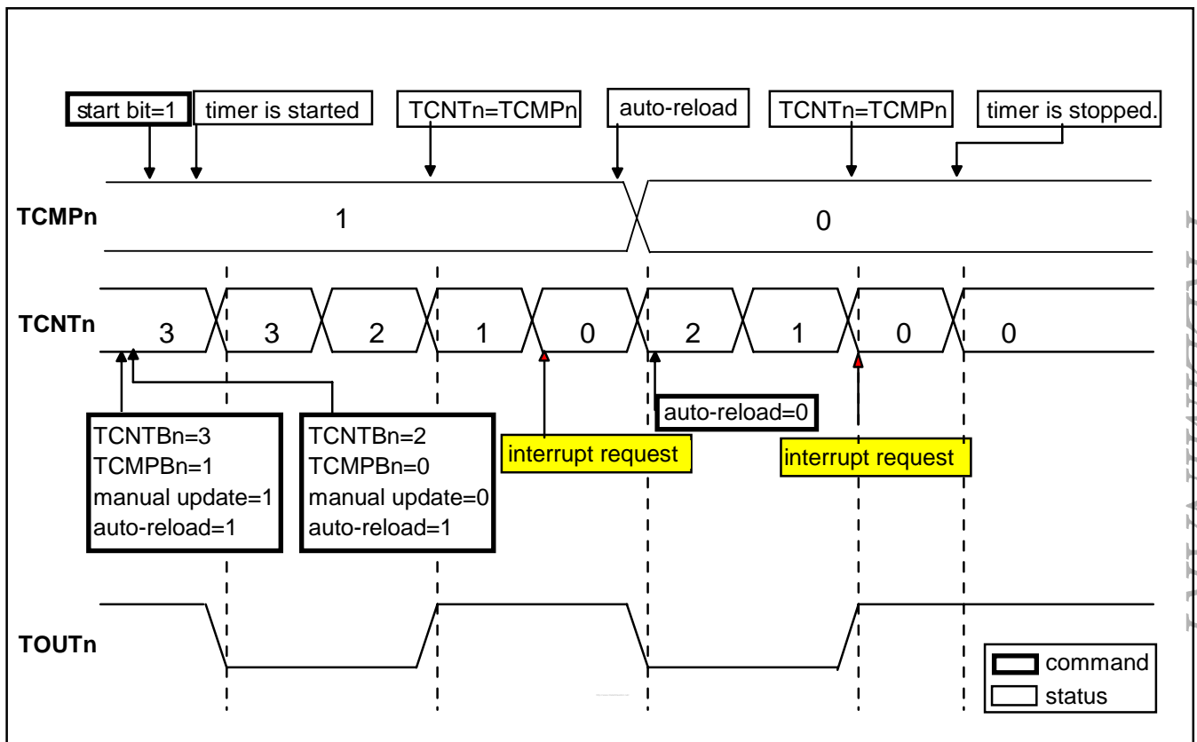
Figure 32-5: Timer operations
