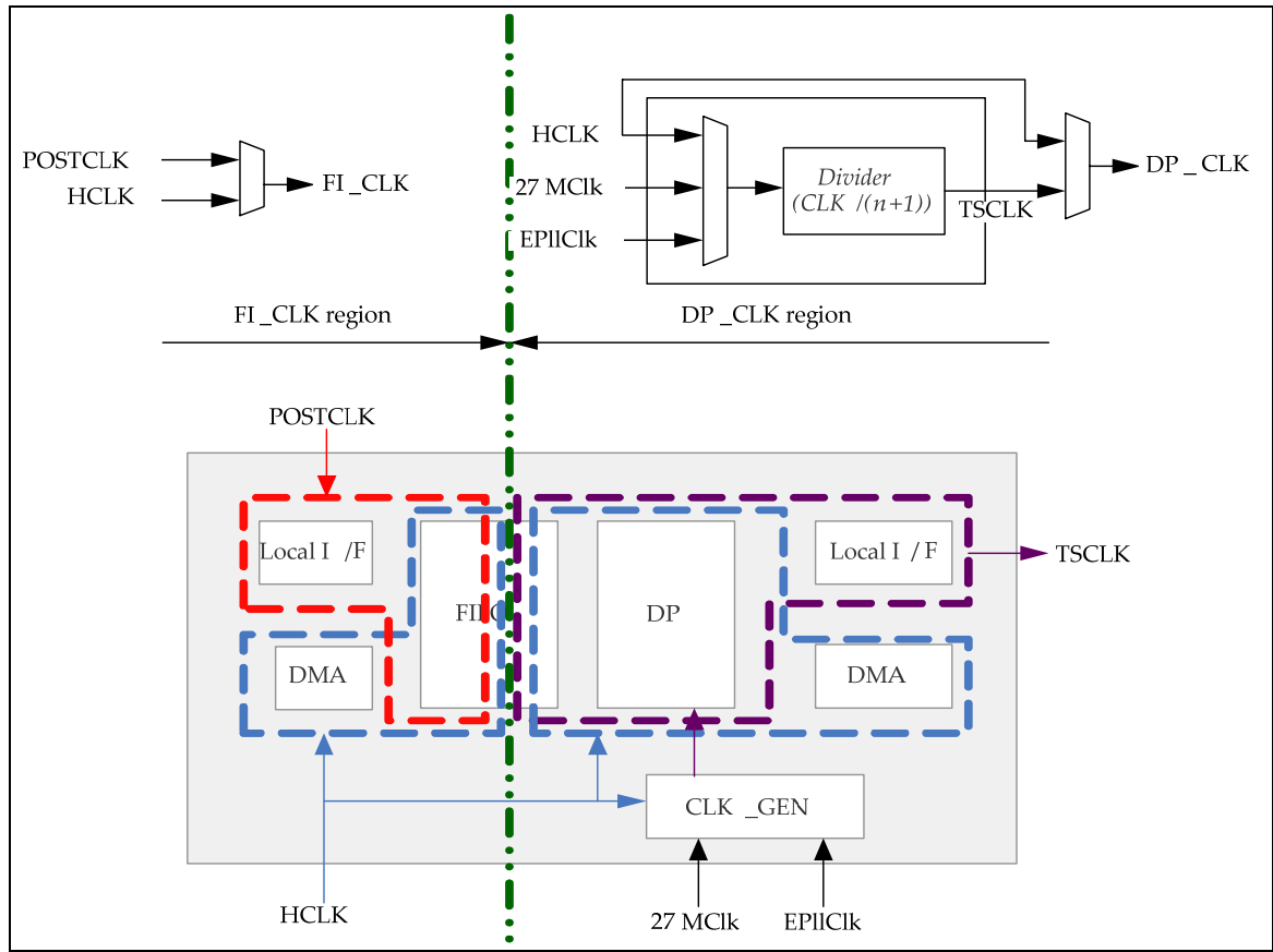
Figure 16-10 Internal clock scheme Block Diagram
