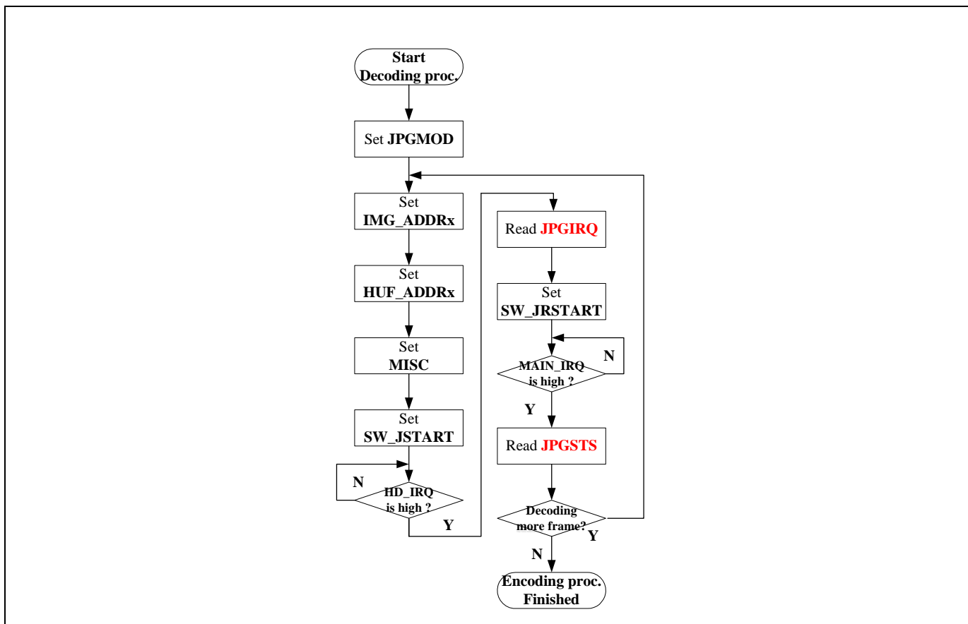
Figure 22-5. Example flow chart of software controlled decoding
