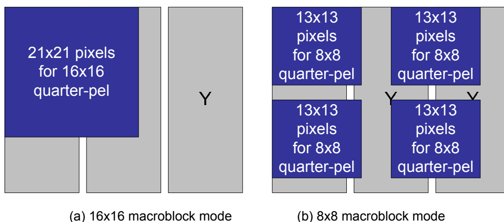
Figure 21.18. The example of the stored reference pixels in 16x16 mode and 8x8 mode
