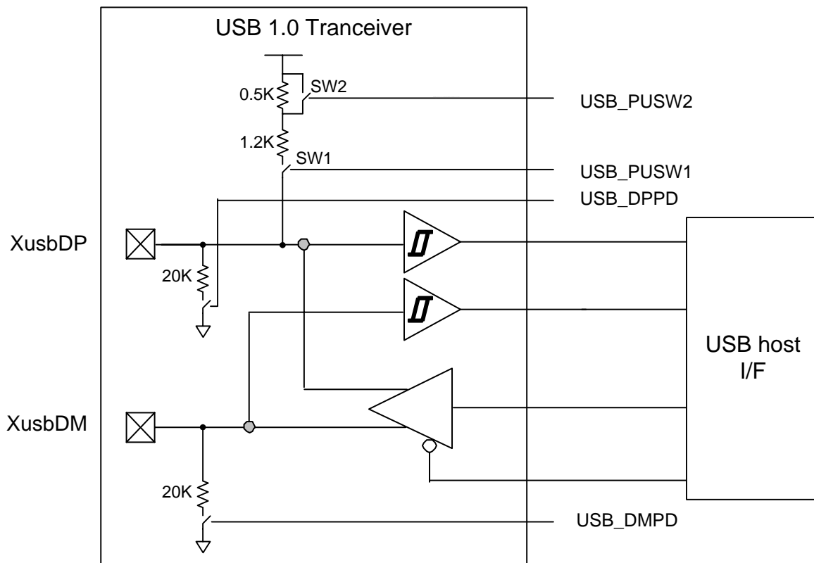
Figure 10- 2 USB transceiver block diagram
