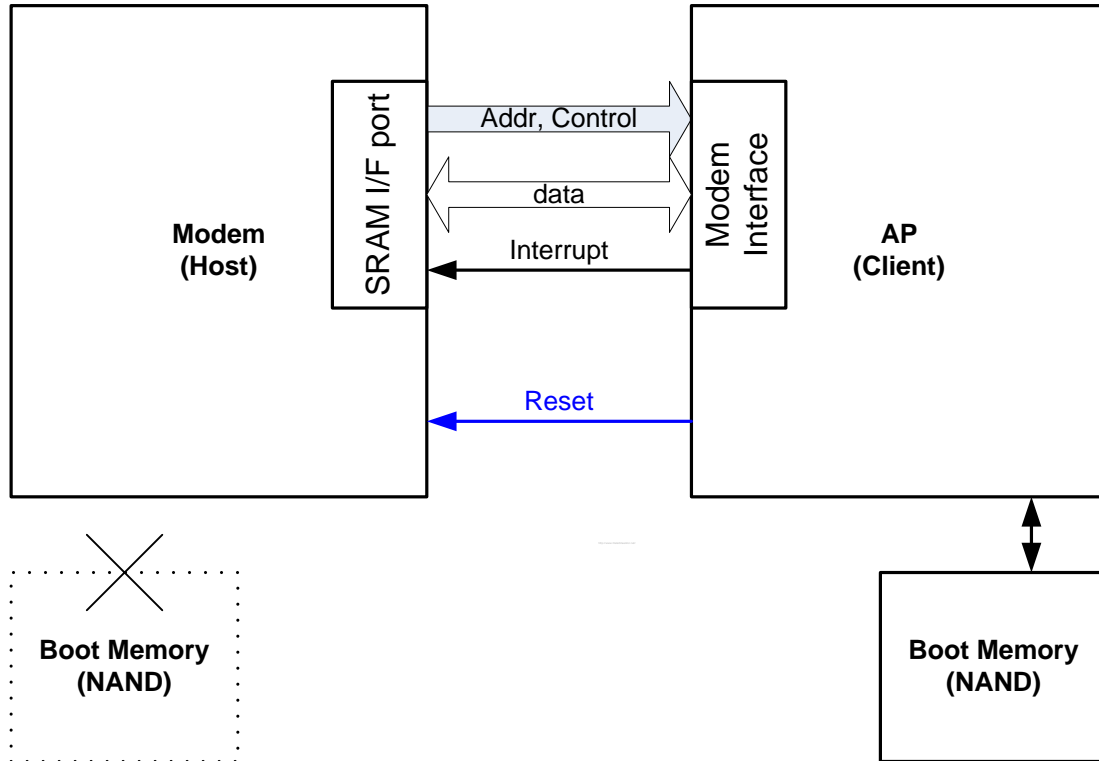
Figure 23-2 MODEM interface for AP Booting for MODEM
