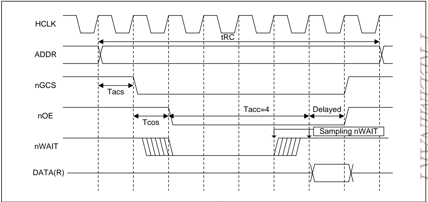
Figure 6-2 SROM Controller nWAIT Timing Block Diagram
