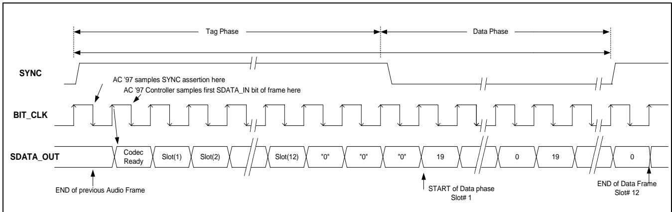
Figure 35-6. AC-link Input Frame
