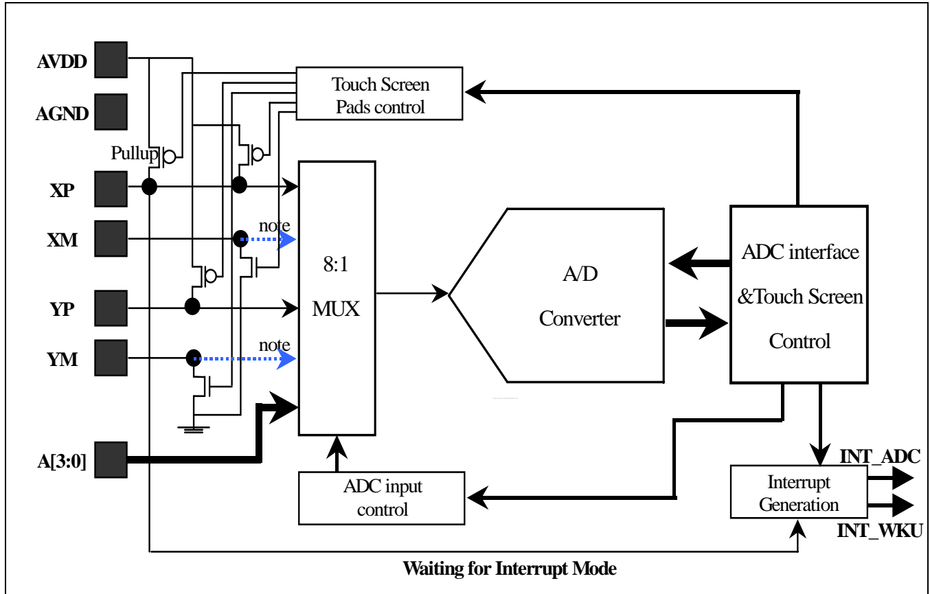
Figure 39-1. ADC and Touch Screen Interface Functional Block Diagram
