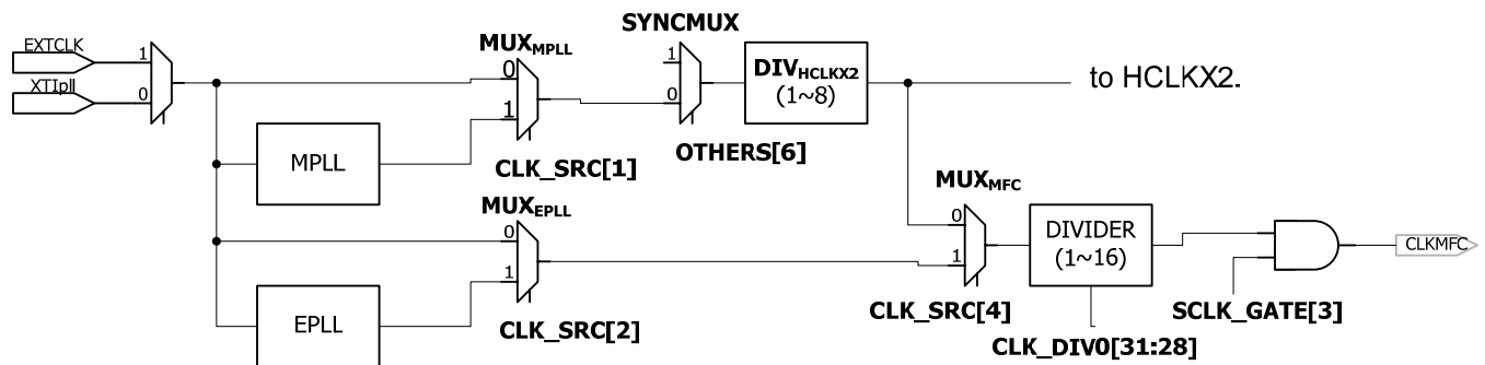
Figure 3-8. MFC clock generation
