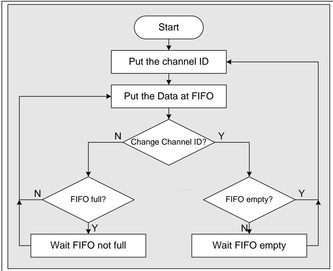
Figure 28-14 Basic Tx module programming flow chart
