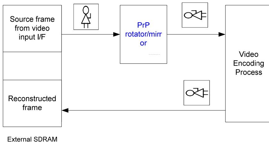
Figure 21.11. PrP rotator data flow
