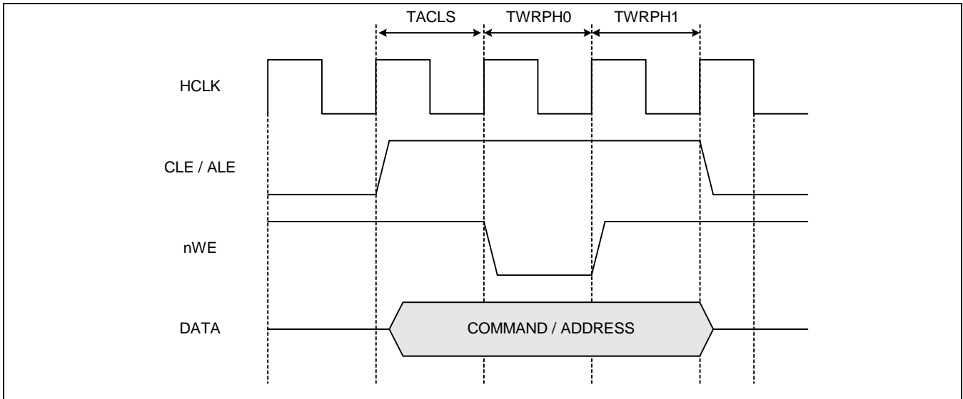
Figure 8-3. CLE & ALE Timing (TACLS=1, TWRPH0=0, TWRPH1=0) Block Diagram
