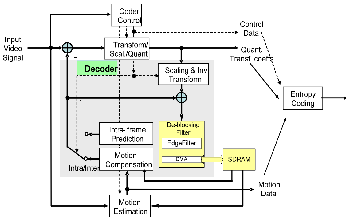
Figure 21.28. H.264 deblocking filter data flow
