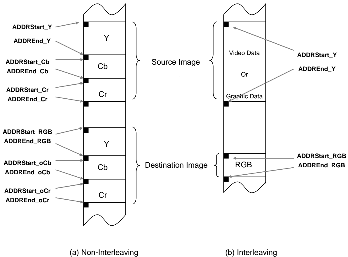
Figure 15-6 Start and end address set according to memory allocation type Block Diagram
