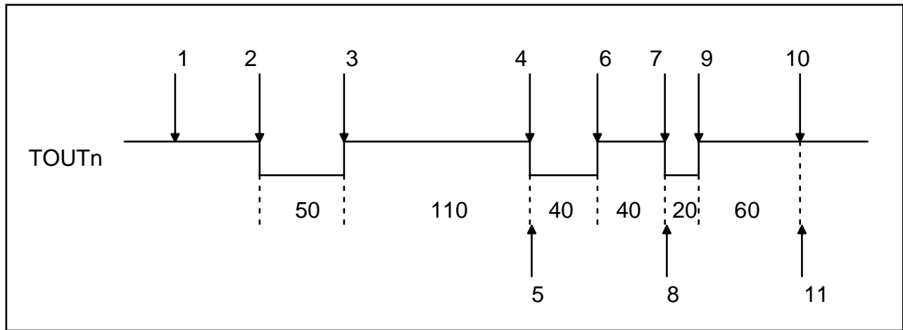
Figure 32-7: Example of a Timer Operation
