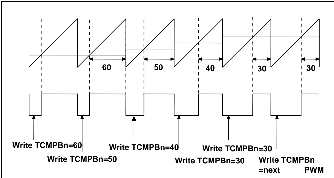
Figure 32-8: Example of PWM
