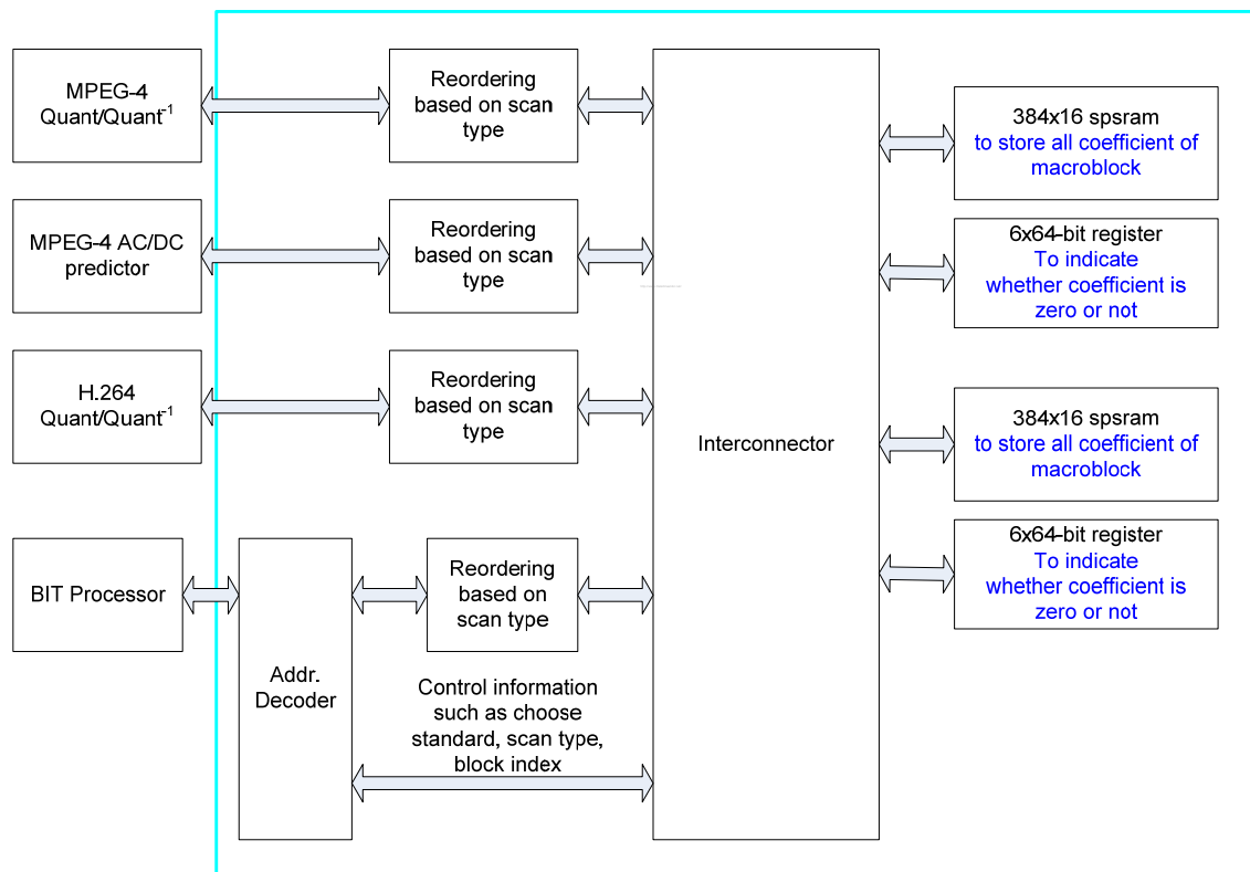
Figure 21.35 Coefficient memory interface block diagram
