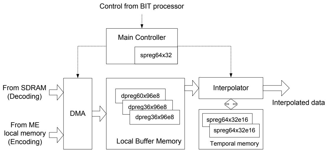
Figure 21.16. The Block Diagram of Inter-prediction
