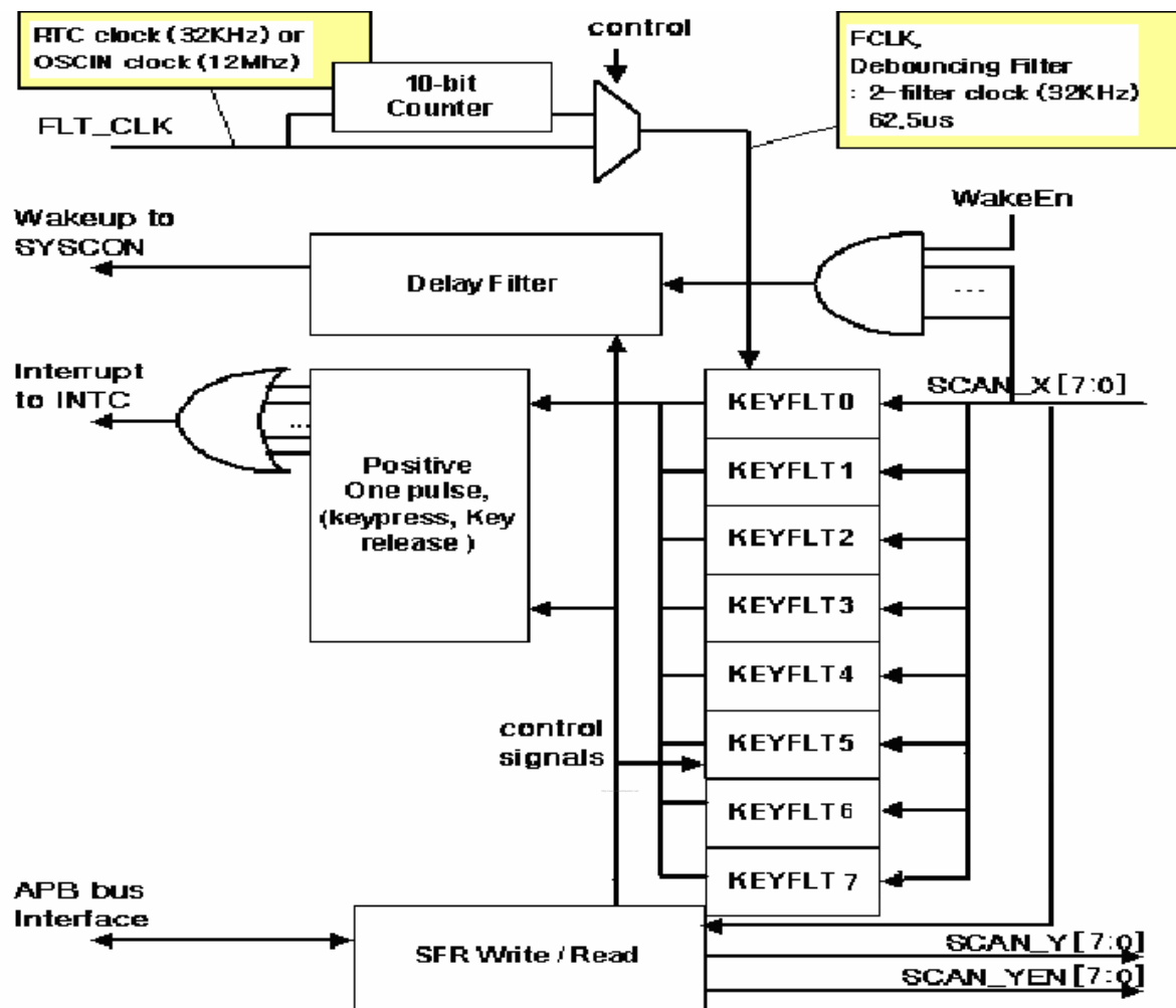
Figure 40-7 Keypad I/F block diagram
