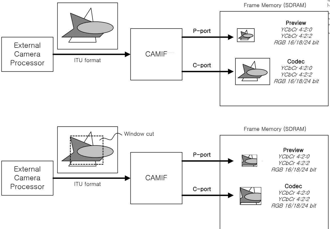
Figure 20-6. DMA ports through Camera processor data
