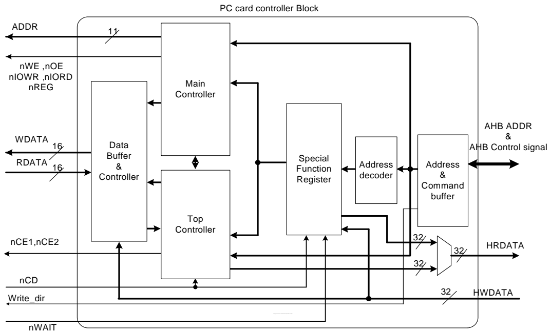
Figure 9-2: PC Card Controller Top Block Diagram
