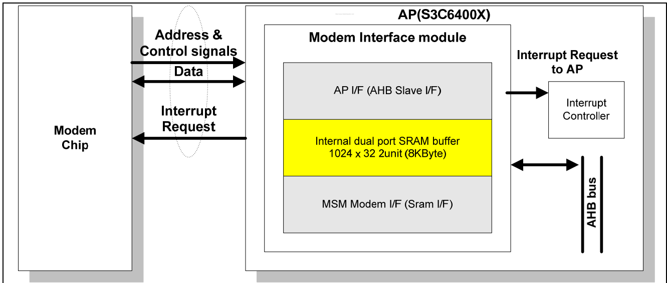
Figure 23-1 The interface with the Modem chip and the MSM I/F block diagram
