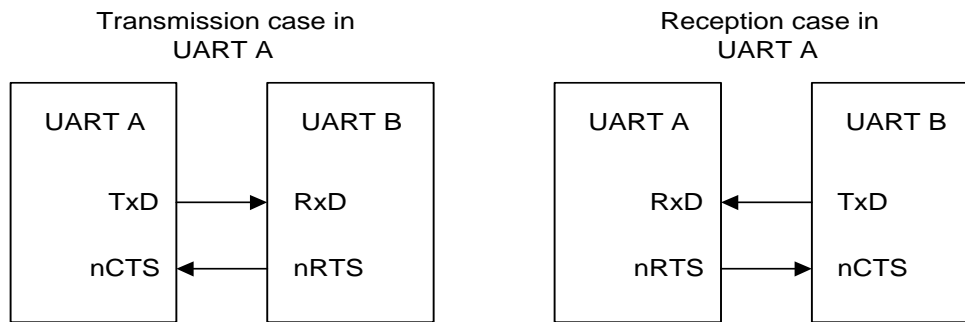
Figure 31-2 UART AFC interface
