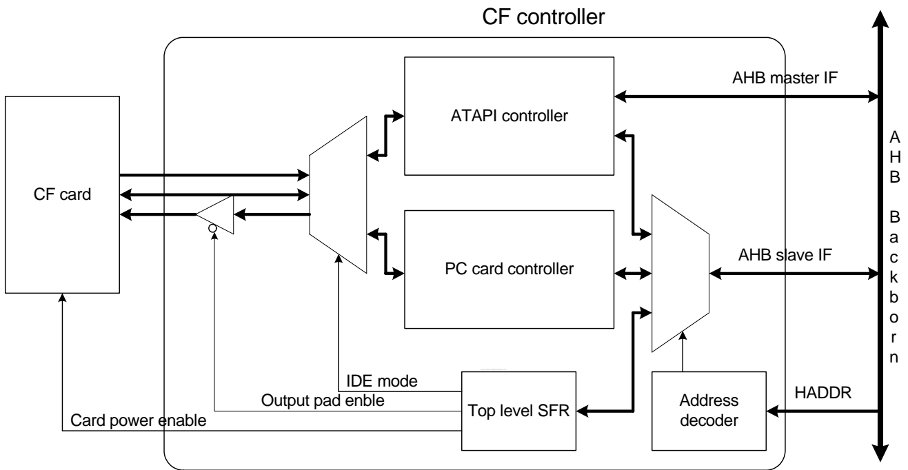
Figure 9-1: CF Controller Top Block Diagram
