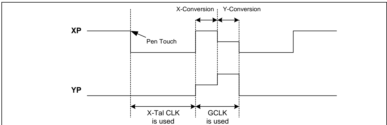
Figure 39-2 ADC and Touch Screen Operation signal
