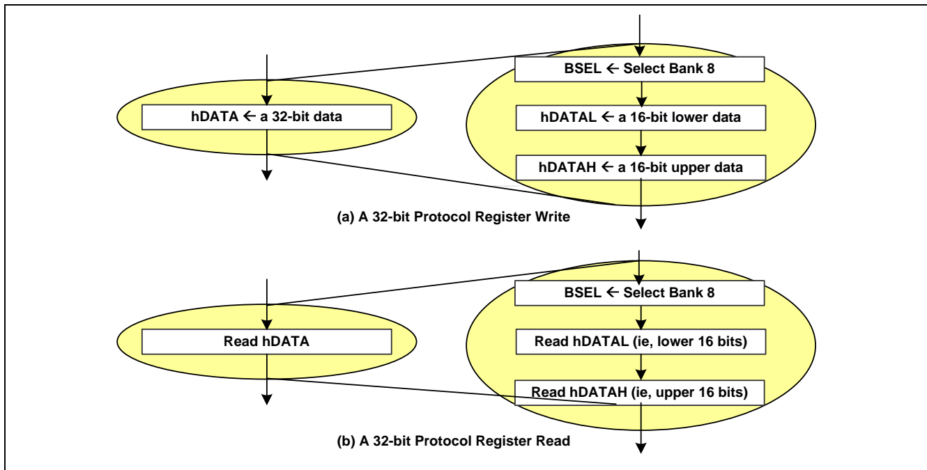
Figure 24-3. A 32-bit Protocol Register Access by Using Two 16-bit Read/Write
