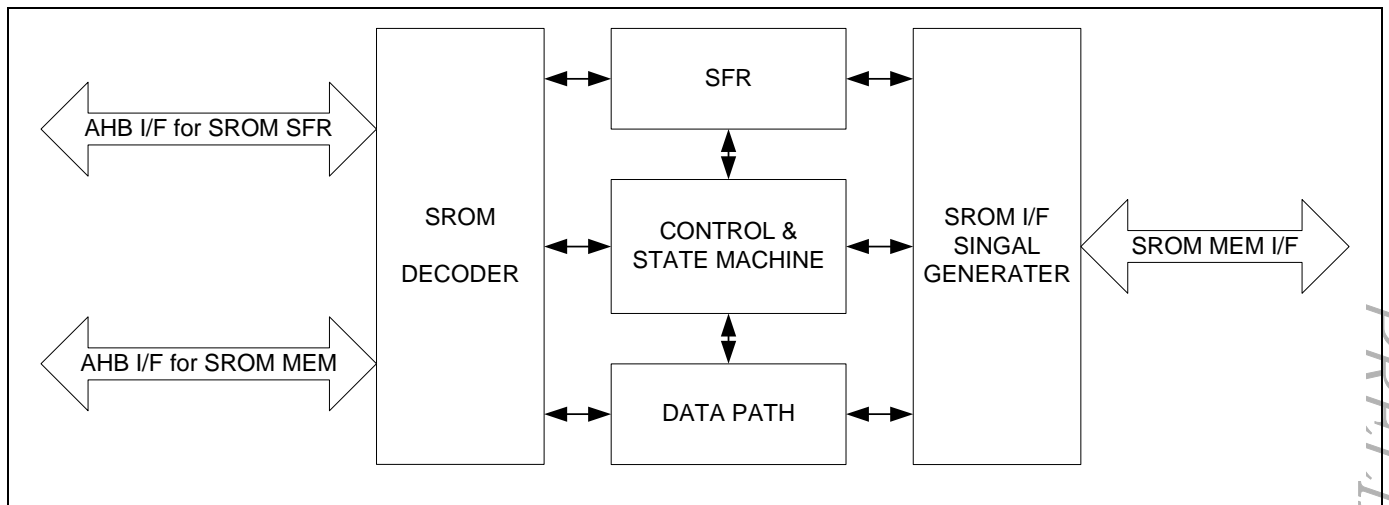
Figure 6-1 SROM Controller Block Diagram
