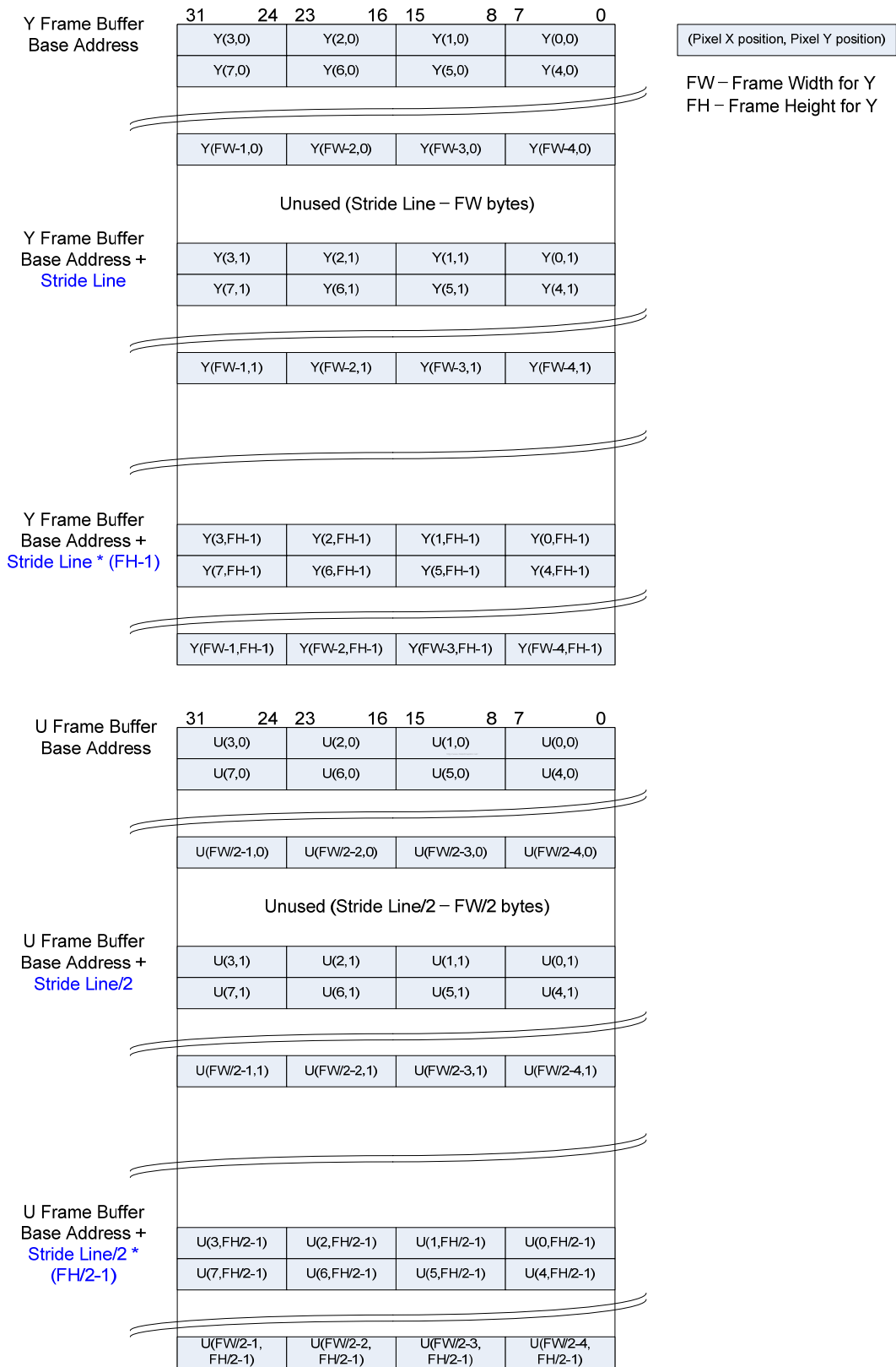
Figure 21.10. Frame buffer address map in little endian
