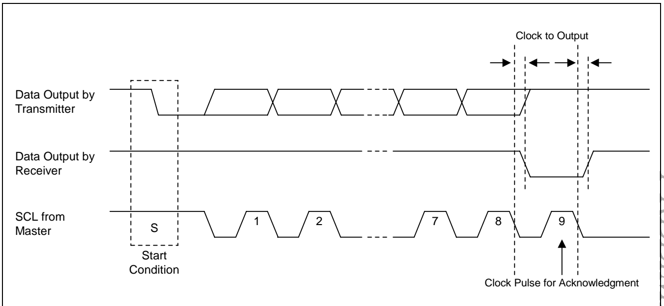
Figure 30-4. Acknowledge on the IIC-Bus Block Diagram
