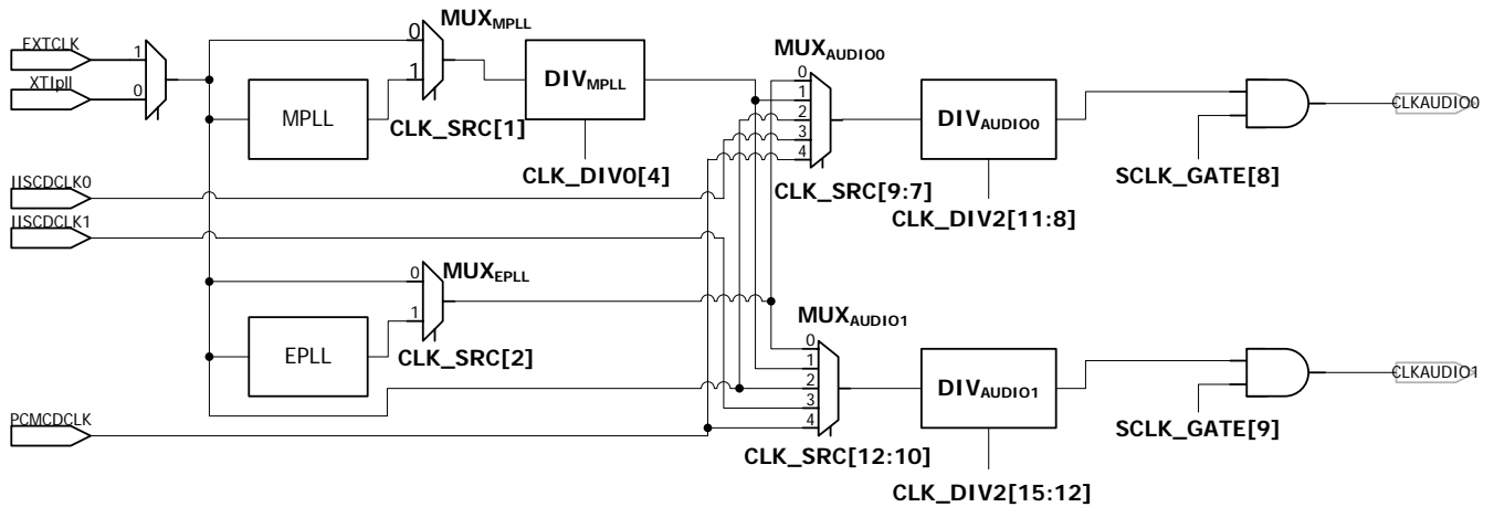
Figure 3-11. Audio clock generation
