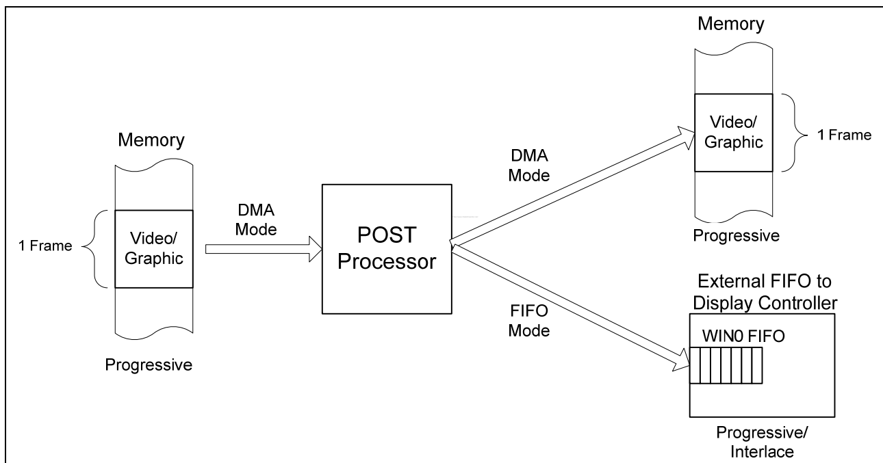
Figure 15-2. Two input and output modes in POST Processor Block Diagram
