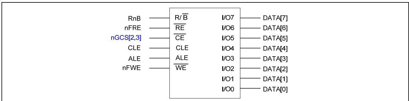
Figure 8-6 A 8-bit NAND Flash Memory Interface Block Diagram
