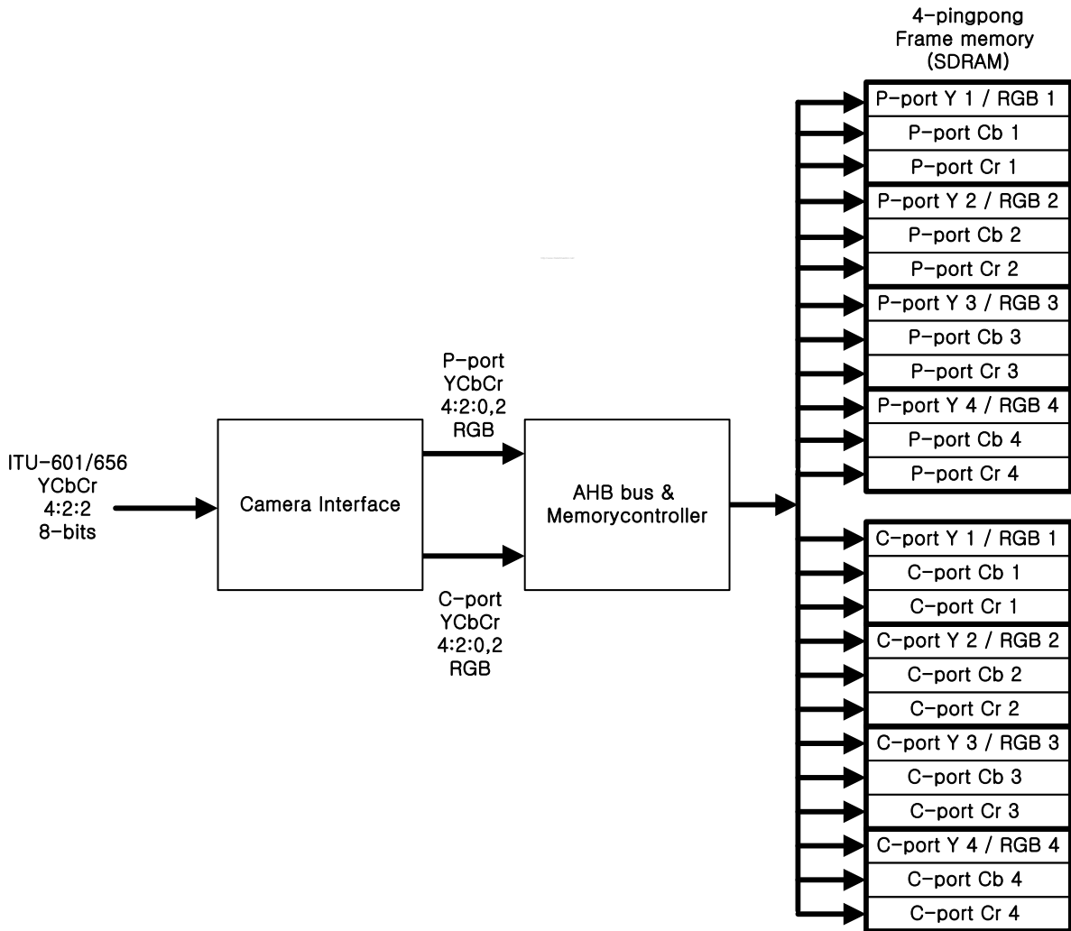
Figure 20-8. Ping-pong memory hierarchy
