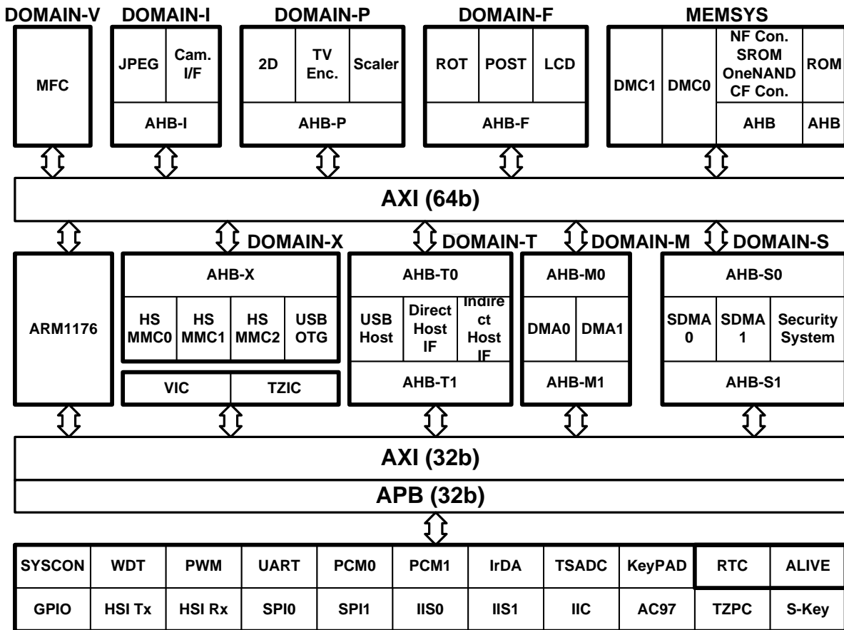
Figure 3-1. S3C6400X block diagram
