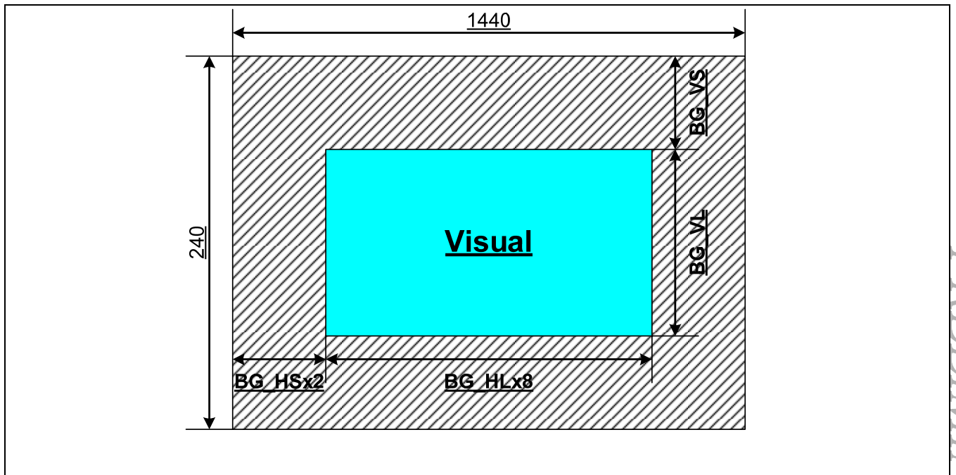
Figure 17-14. The Calculation Method of Back-ground
