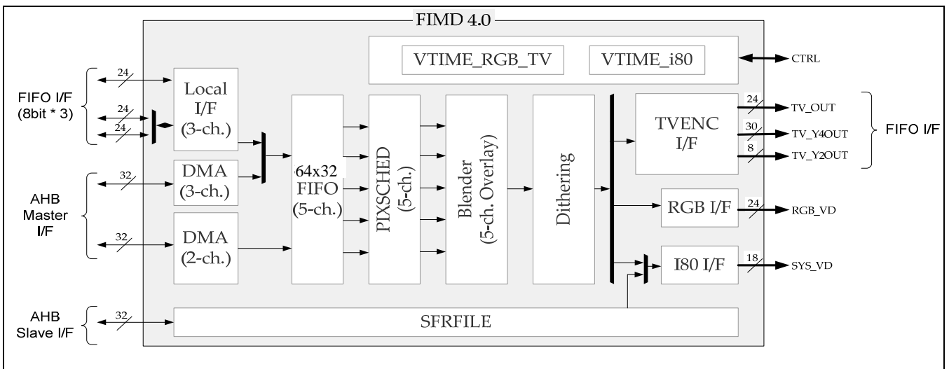
Figure 14-1. Top block diagram Display Controller
