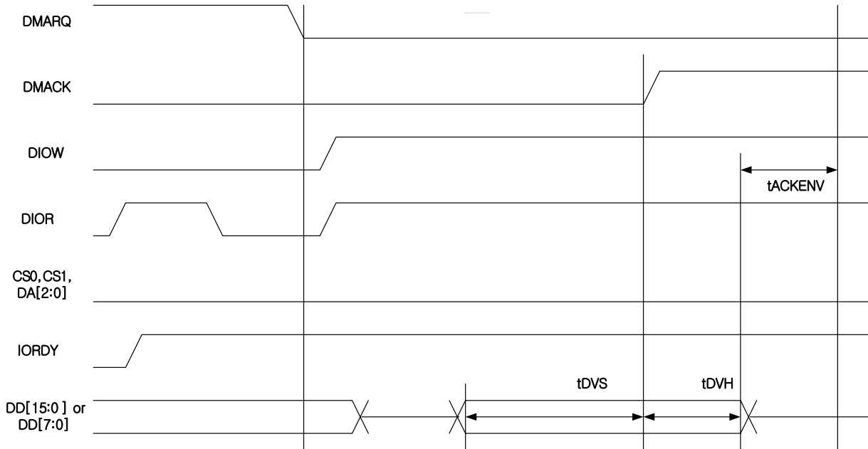
Figure 9-9: UDMA - Out Operation (terminated by host)
