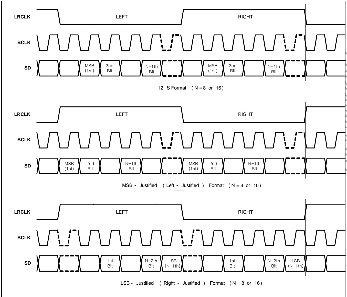
Figure 36-3. IIS Audio Serial Data Formats
