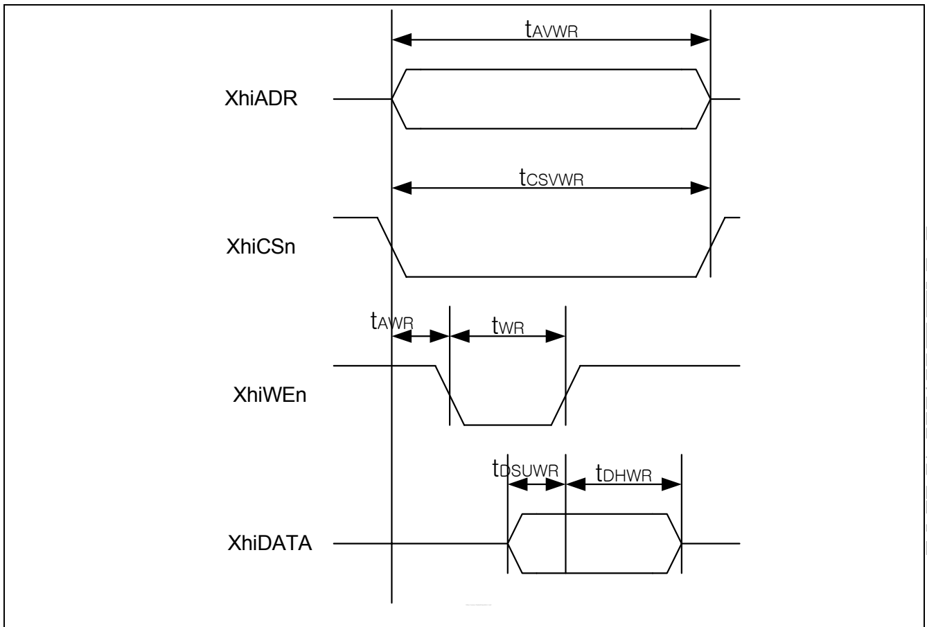
Figure 41-14. Modem interface write timing diagram
