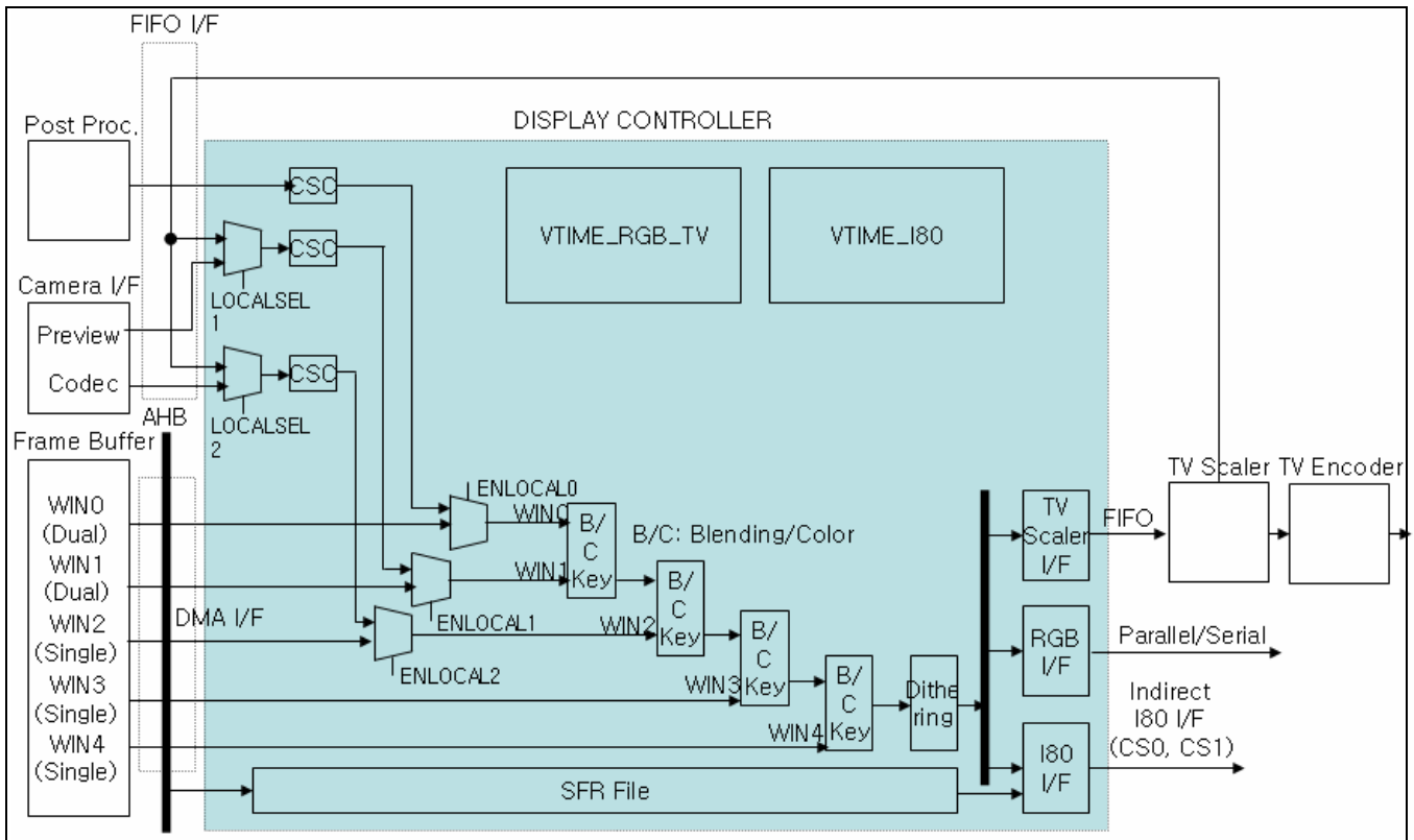
Figure 14-2. Block diagram of the Data Flow
