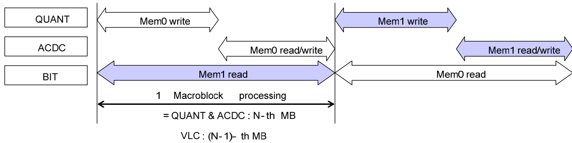
Figure 21.37 MPEG-4 encoding case
