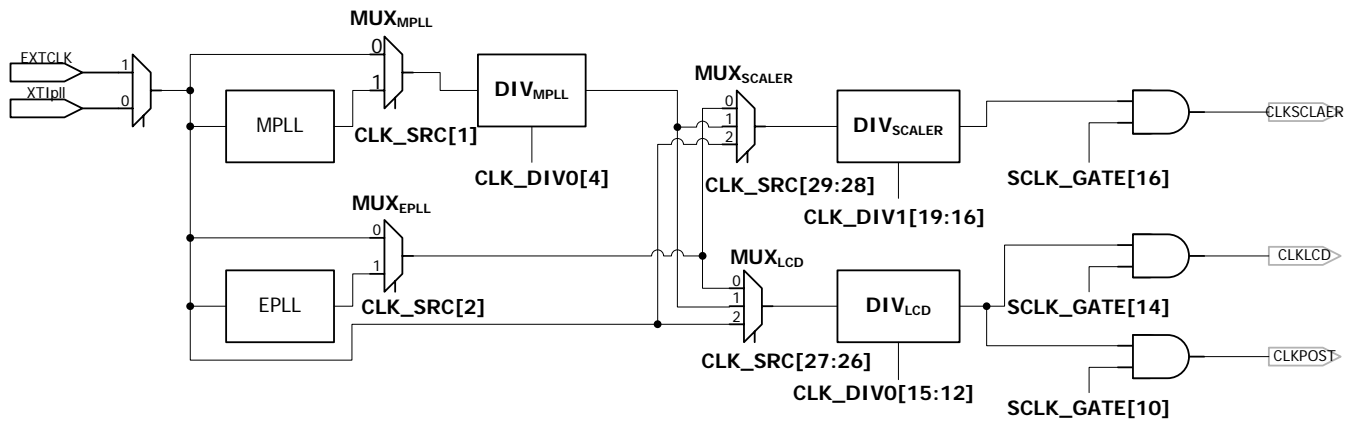
Figure 3-10. Display clock generation
