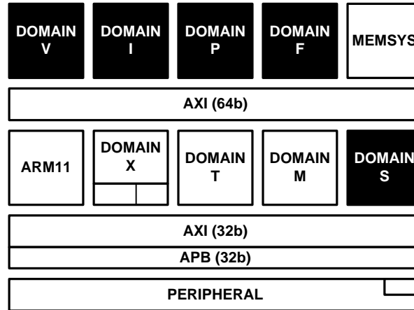
Figure 3-15. Power domains at STOP mode (Domains highlighted in white represent clock-off domain and domains highlighted in black represent power-gating domain)
