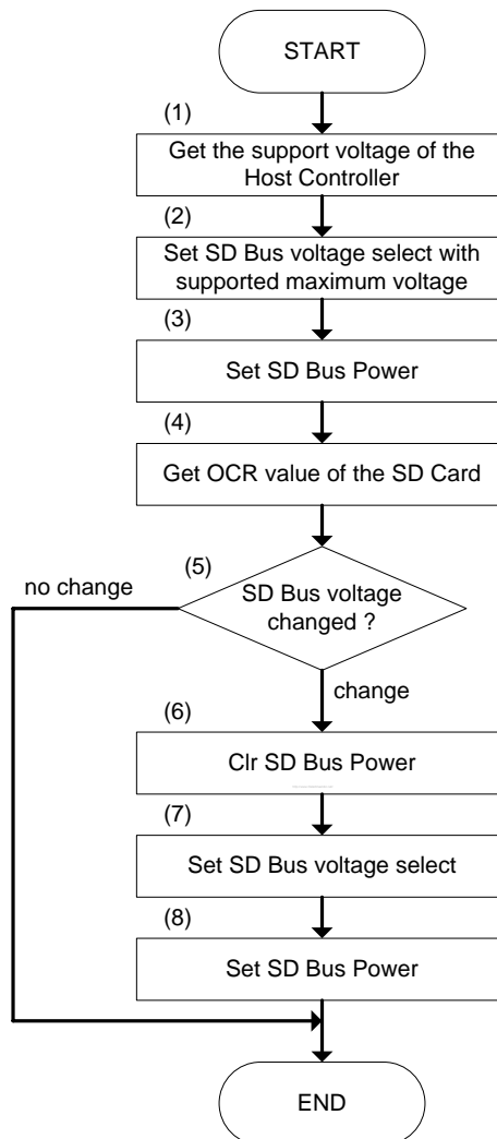
Figure 27-6. SD Bus Power Control Sequence
