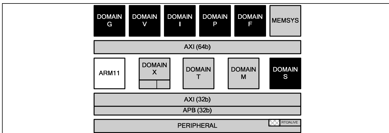
Figure 3-14. Power domains at STOP mode (grey domains represent state-retained domain and black domains represent power-gating domain)
