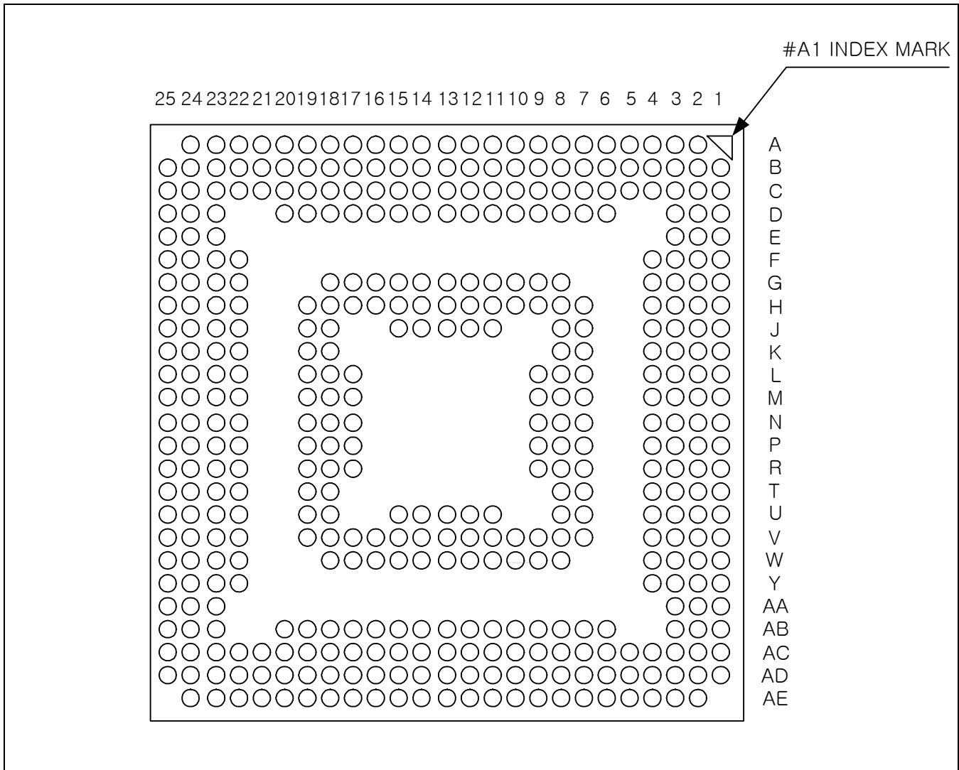
Figure 1-2. Pin Assignments
