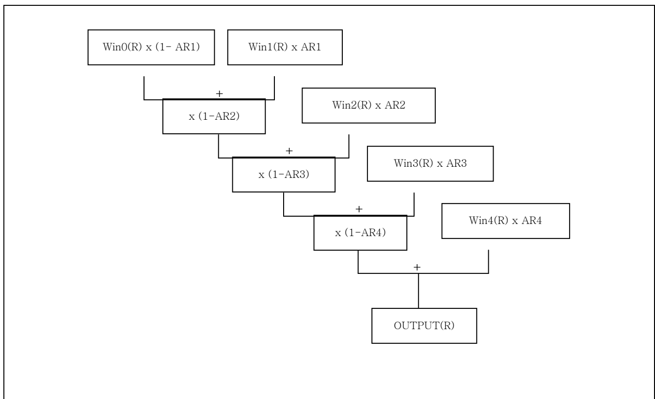
Figure 14-5. Blending diagram
