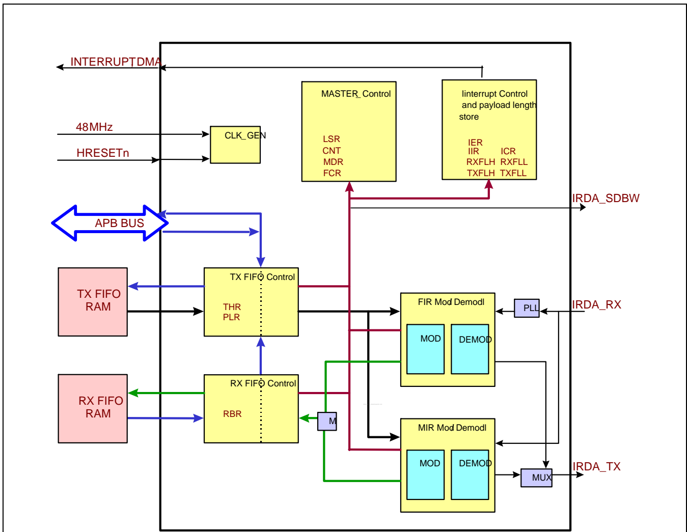
Figure 38-1. Block Diagram
