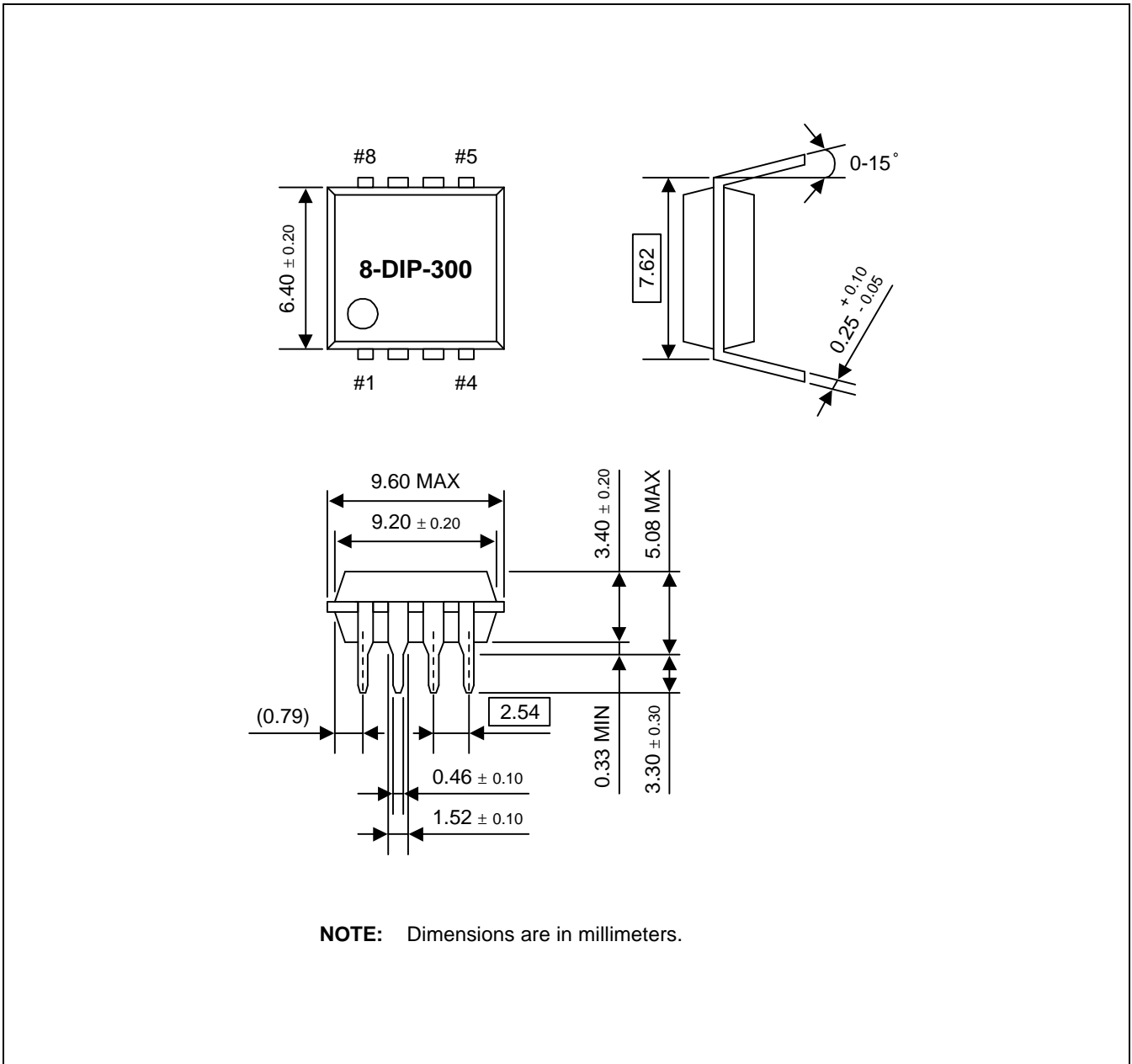
Figure 14-4. 8-DIP-300 Package Dimensions
