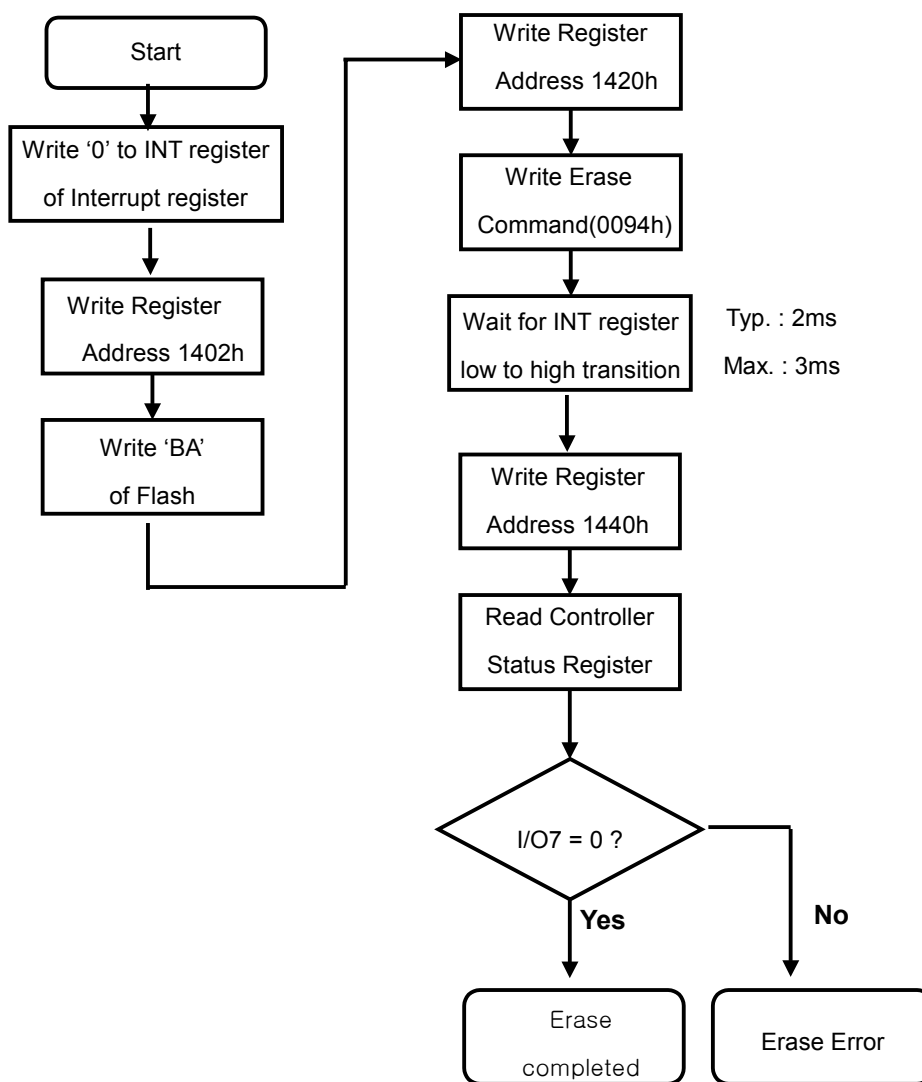
Figure 21. Flow Chart of Erase Operation
