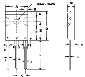
TO-247 (3P)
