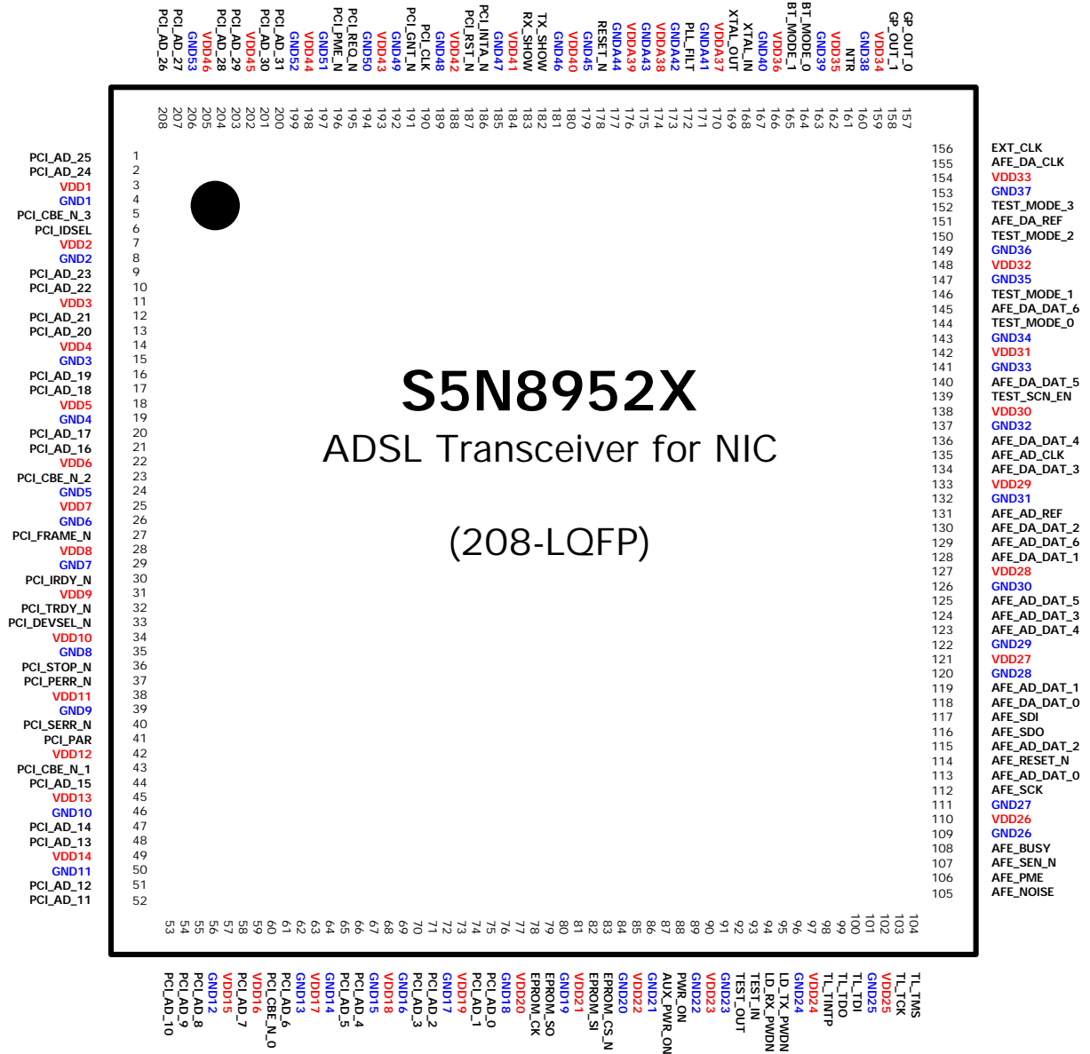
Figure 3: Pin Configuration of the S5N8952X
