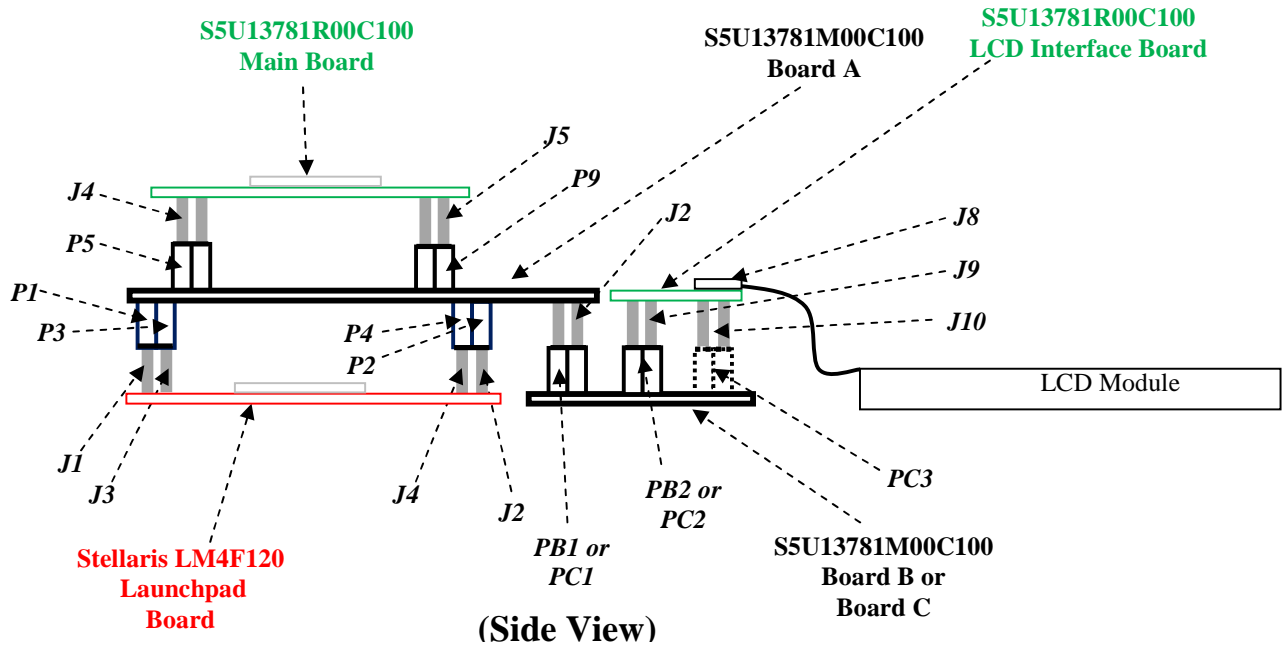
Figure 3 – Board Connections Diagram
