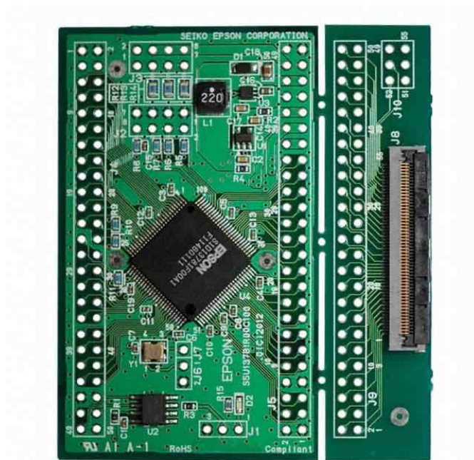
Figure 1 – S5U13781R00C100 Reference Board Set
