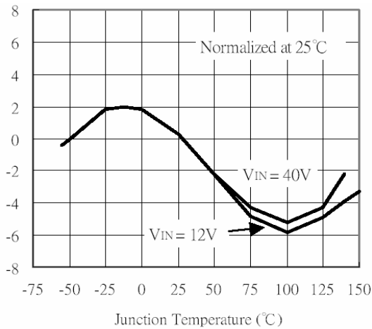
Oscillator Frequency
