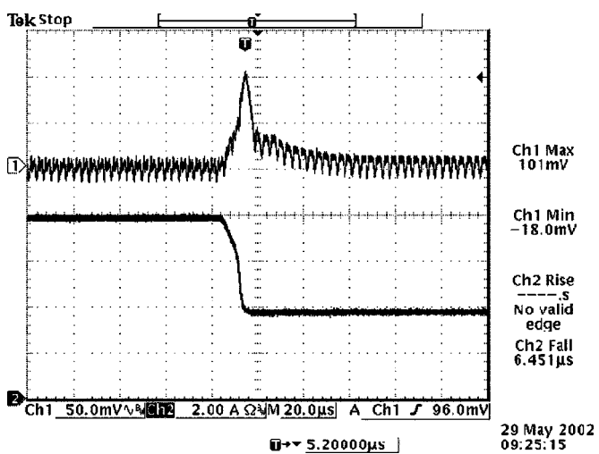
DataSheet4U.com Vout=1.2V 100% to 50% load transients at 5V input and Ta=25° C
