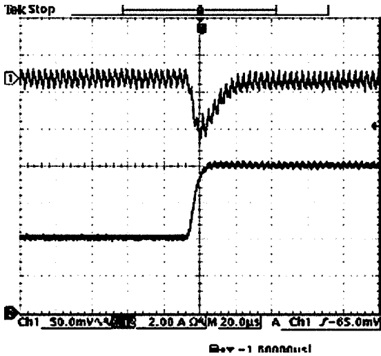
Vout=1.8V 50% to 100% load transients at 5V input and Ta=25° C
