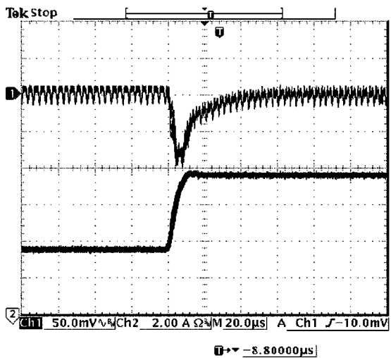
Vout=1.2V 50% to 100% load transients at 5V input and Ta=25° C
