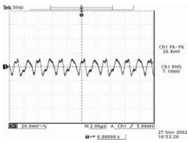
Ripple and noise at full load and 8Vdc input, 1.8Vdc output and Ta=25° C
