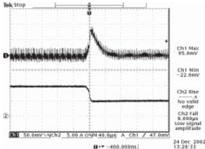
DataSheet4U.com Vout=1.0V 100% to 50% load transients at 8V input and Ta=25° C
