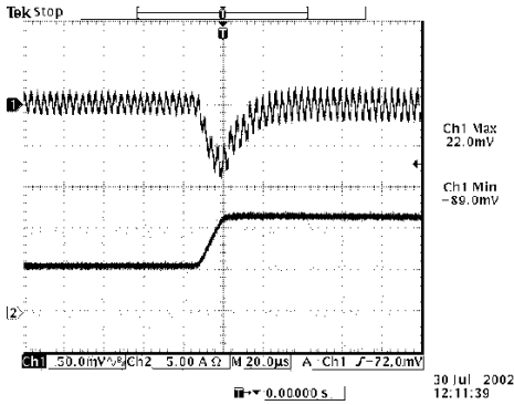
Vout=1.2V 50% to 100% load transients at 3.3V input and Ta=25° C
