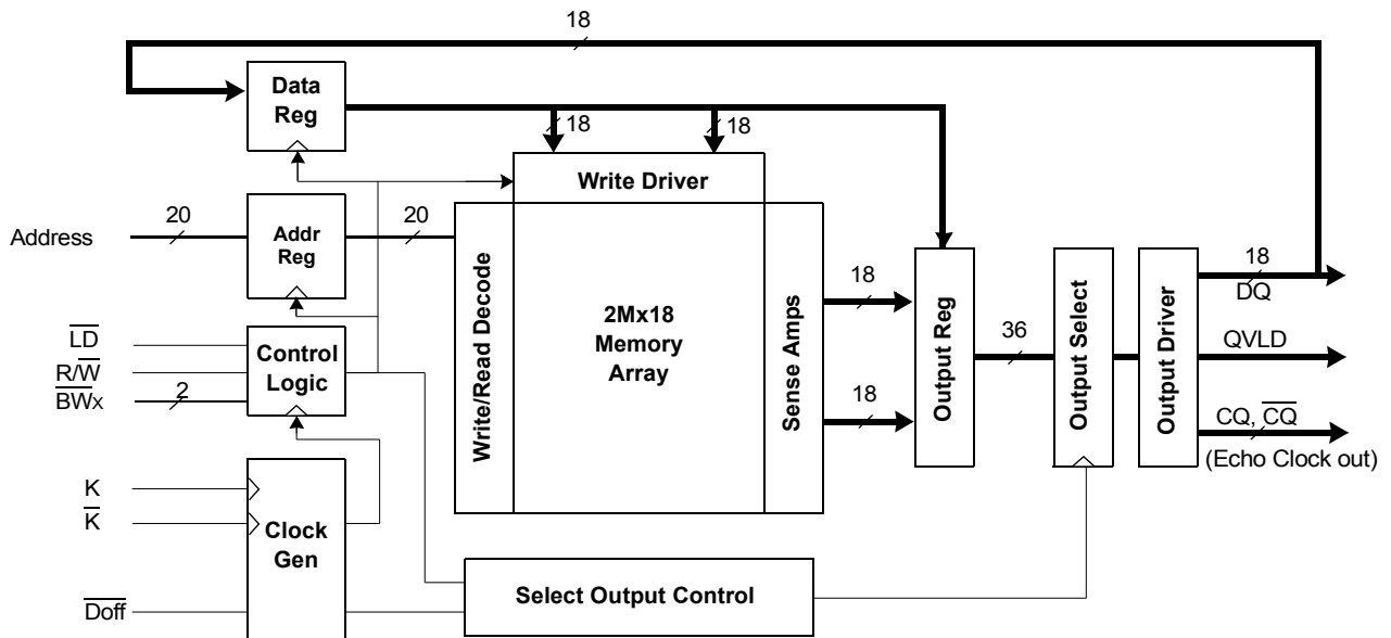
Logic Block Diagram - S7L3218U2M (2M x 18)
